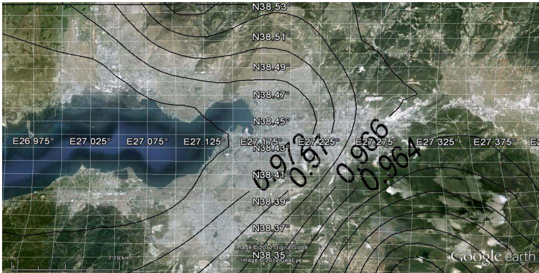
Figure E.9 (MAP 9): Attenuation relationship: Campbell & Bozorgnia (2008). Probability of exceedance in 50 years: 2% Values: Ground Acceleration (g) (Median +Standard Deviation). Spectral period T=0.2s V_{s30}=760 m/s
