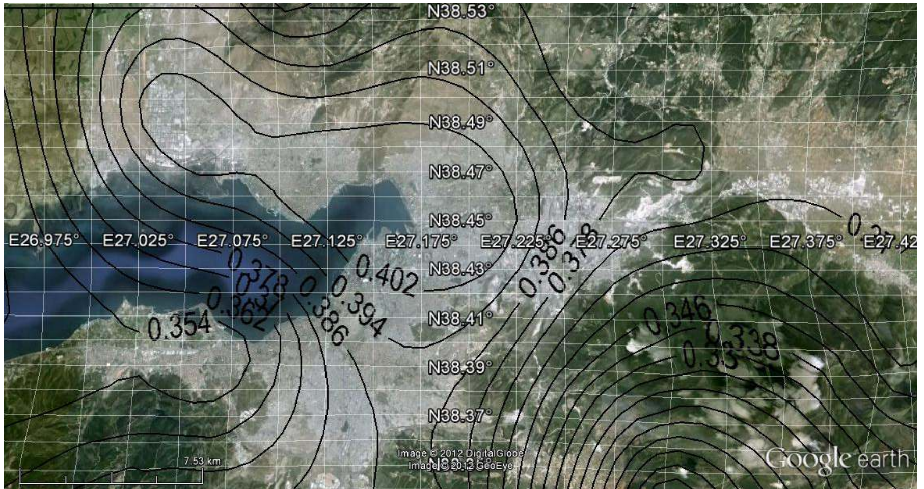
Figure E.15 (MAP 15): Attenuation relationship: Brian et al.(2008). Probability of exceedance in 50 years: 2% Ground Acceleration (g) (Median) Spectral period T=1 s V_{s30}=760 m/s
