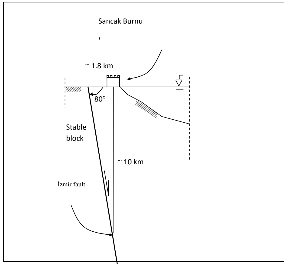
Figure 2.10 The geometric analysis of the epicenter of earthquake occurred near İzmir fault in 1688 (Özden et al., 2011).
