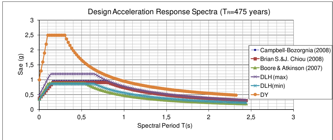
Figure 4.10 Design Spectra for site_2 (Return period T=475 ) (Mavişehir)
