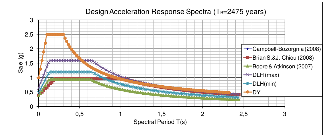
Figure 4.9 Design Spectra for site_1 (Return period T=2475 ) (Manavkuyu)
