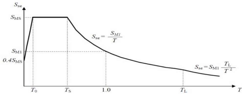
Figure 4.7 Formation of Design Spectra
