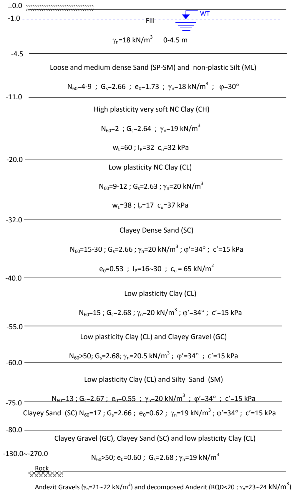
Figure 2.12 Idealized soil profile for Mavişehir Coastal Zone (Özden et al., 2011).
