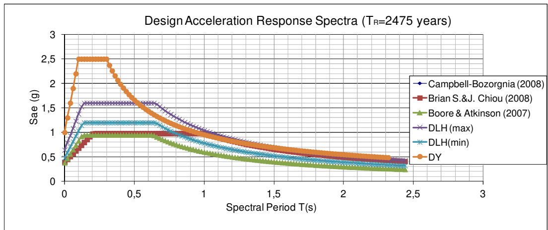
Figure 4.11 Design Spectra for site_2 (Return period T=2475 ) (Mavişehir)
