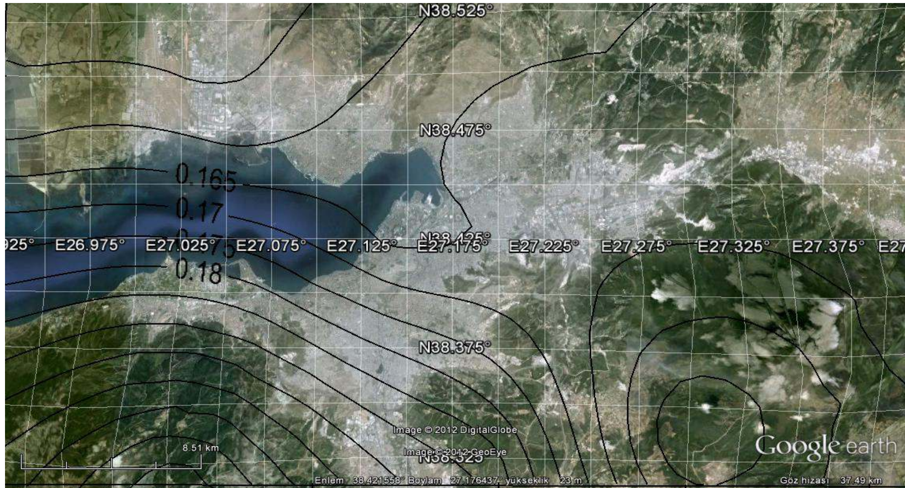
Figure E.34 (MAP 34): Attenuation relationship: Boore & Atkinson (2007). Probability of exceedance in 50 years: 50%
