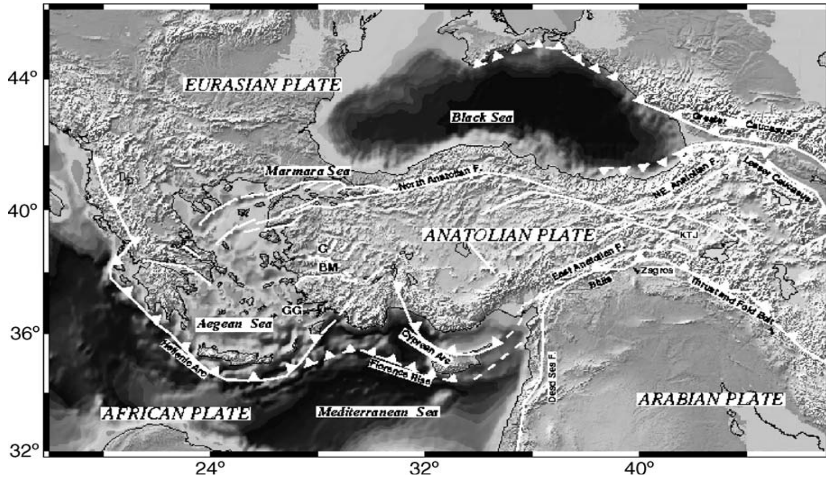
Figure 2.3 General tectonic map of Anatolia and its surroundings. (Aktuğ & Kılıçoğlu, 2006)
