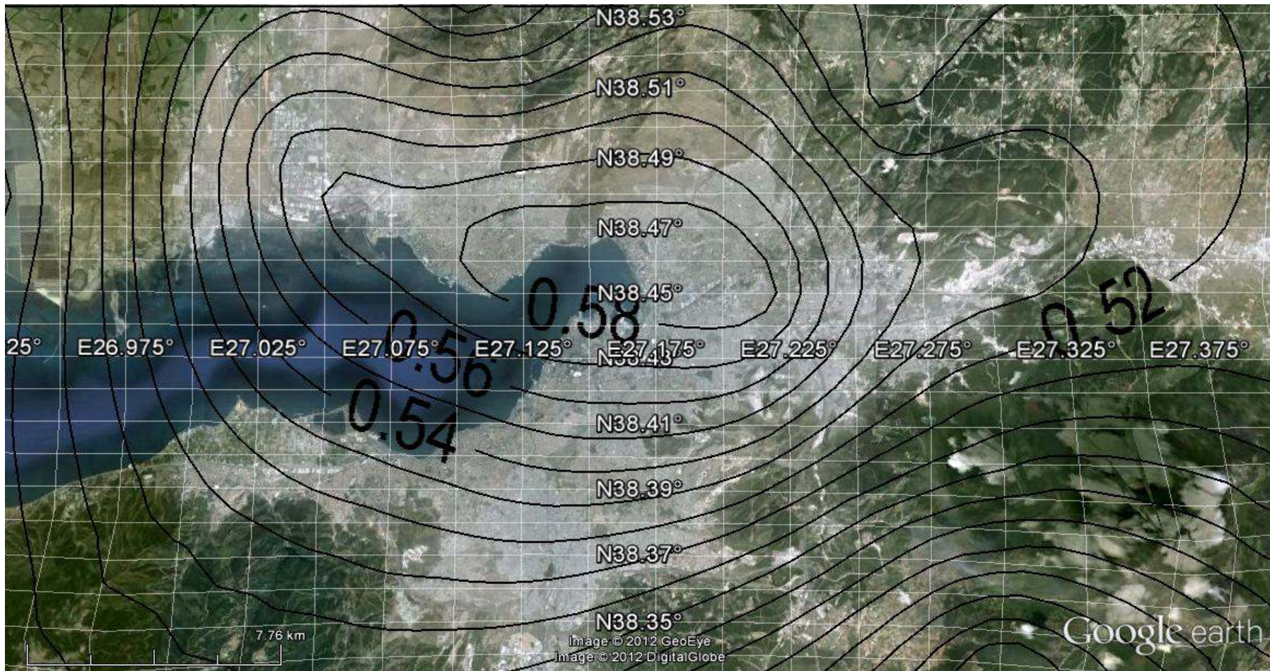
Figure E.11 (MAP 11): Attenuation relationship: Campbell & Bozorgnia (2008). Probability of exceedance in 50 years: 10%
