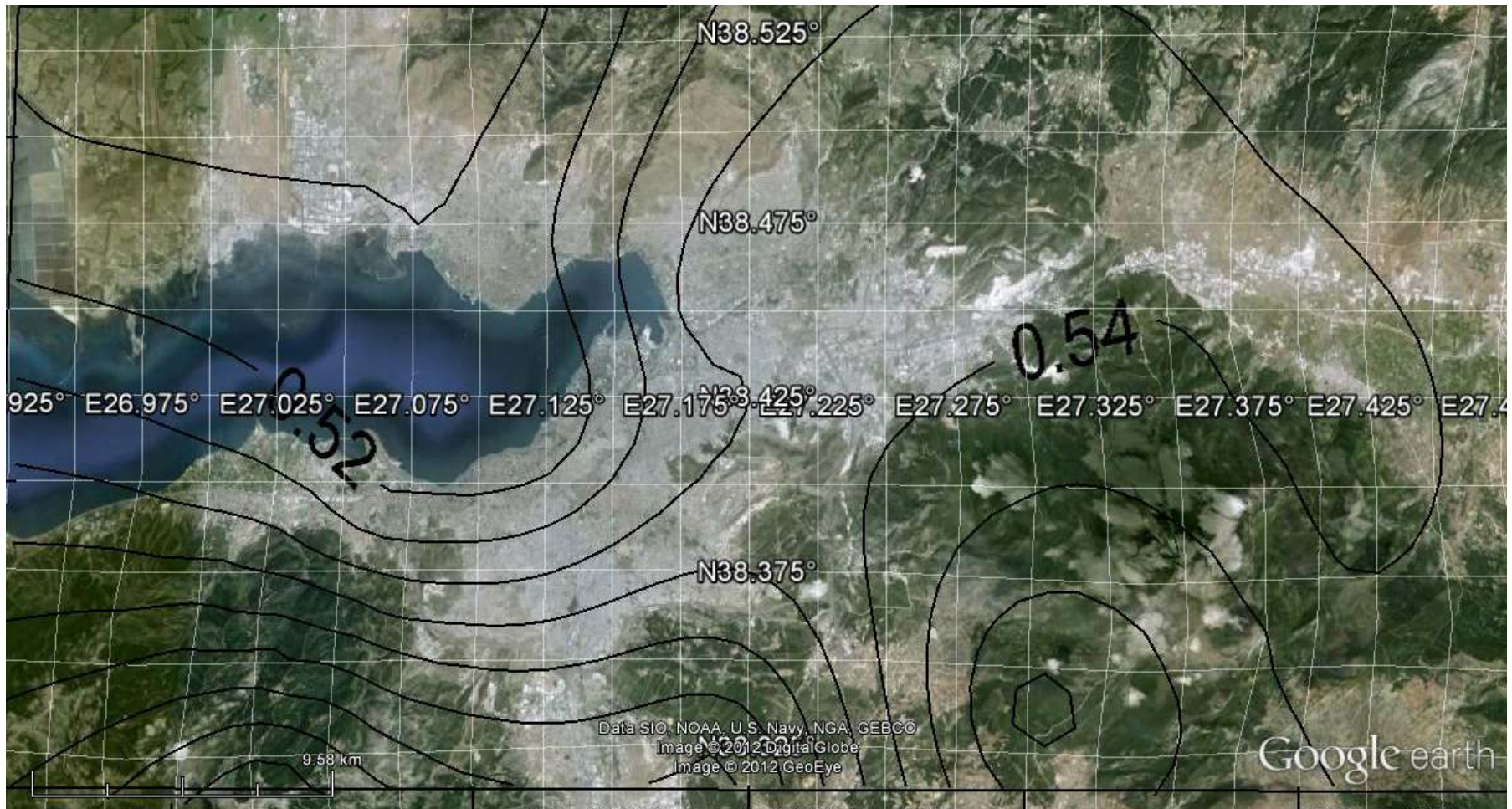
Figure E.31 (MAP 31): Attenuation relationship: Boore & Atkinson (2007). Probability of exceedance in 50 years: 50%
