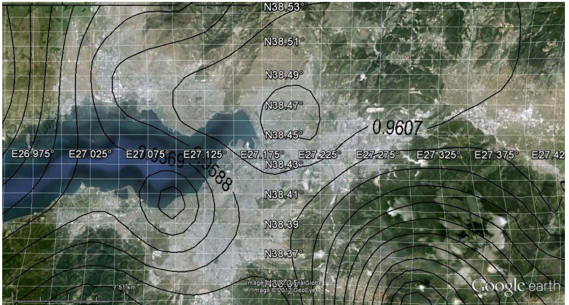
Figure E.21 (MAP 21): Attenuation relationship: Brian et al. (2008). Probability of exceedance in 50 years: 2% Ground Acceleration (g) (Median +Standard Deviation) Spectral period T=0.2 s V_{s30}=760 m/s
