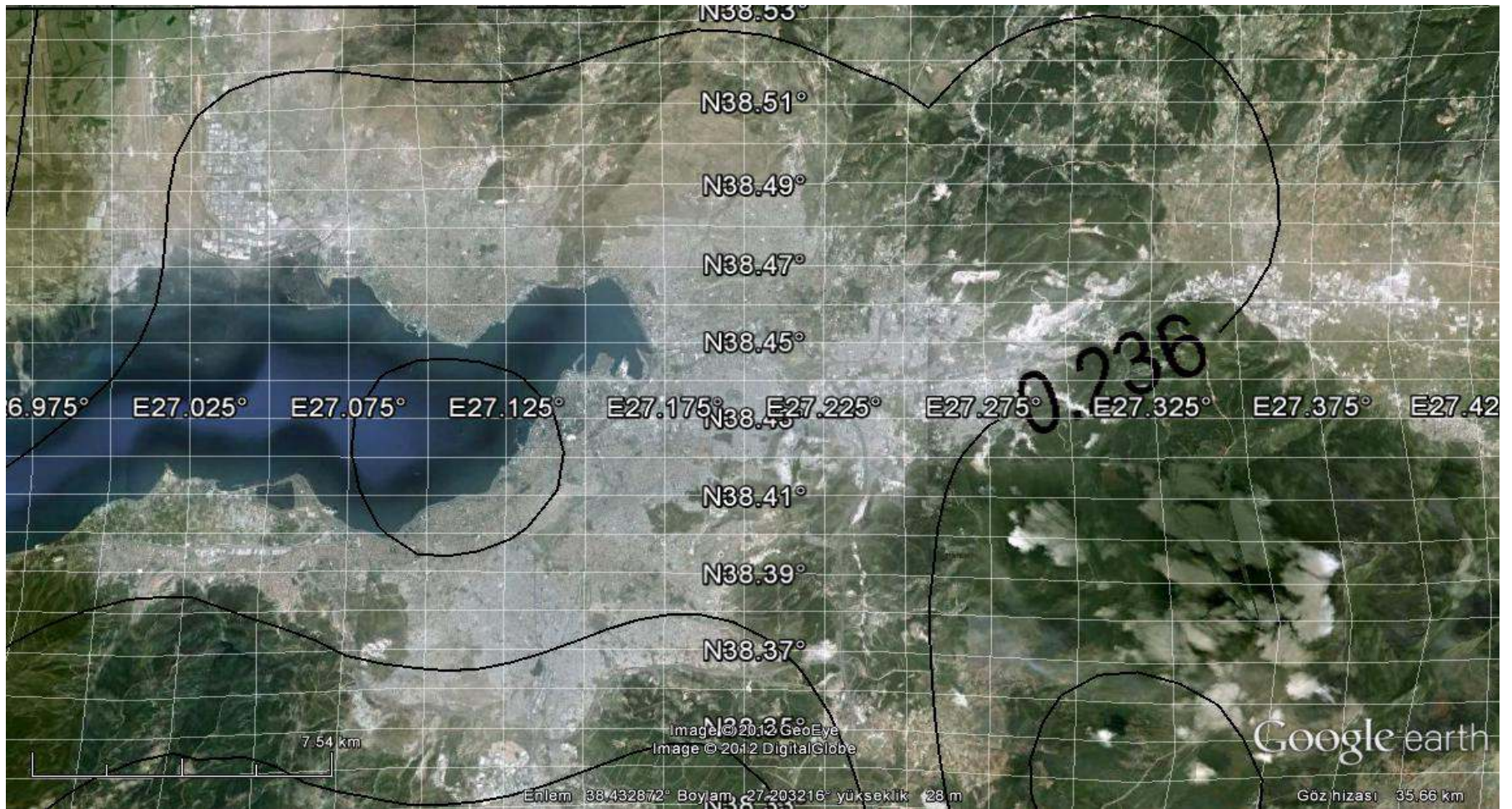
Figure E.27 (MAP 27): Attenuation relationship: Boore & Atkinson (2007). Probability of exceedance in 50 years: 2%
