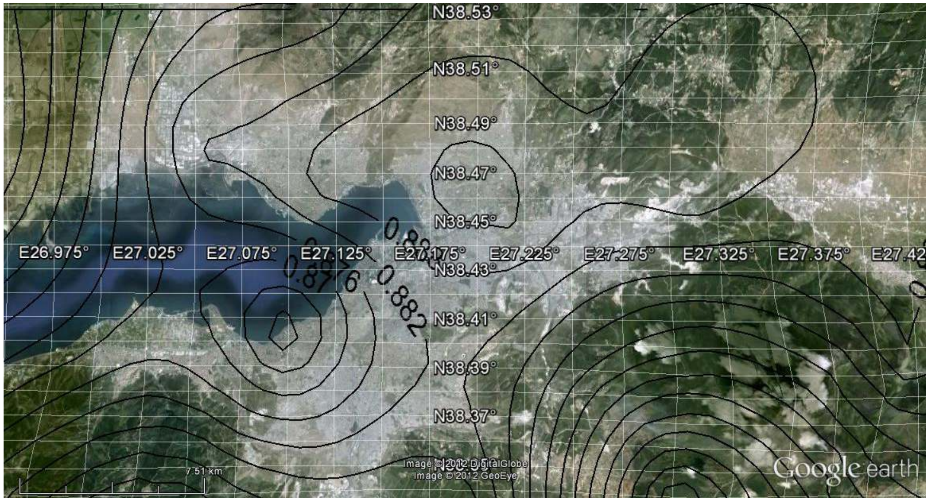
Figure E.20 (MAP 20): Attenuation relationship: Brian et al. (2008). Probability of exceedance in 50 years: 10% Ground Acceleration (g) (Median +Standard Deviation) Spectral period T=0.2 s V_{s30}=760 m/s
