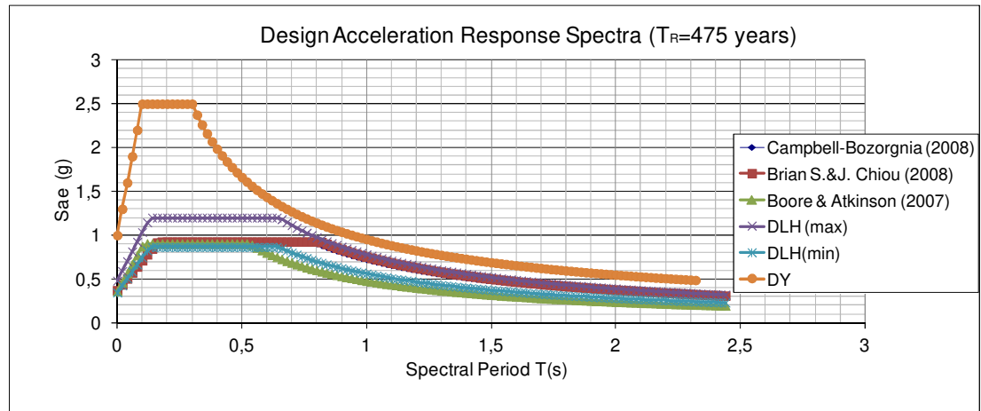
Figure 4.8 Design Spectra for site_1 (Return period T=475 ) (Manavkuyu)
