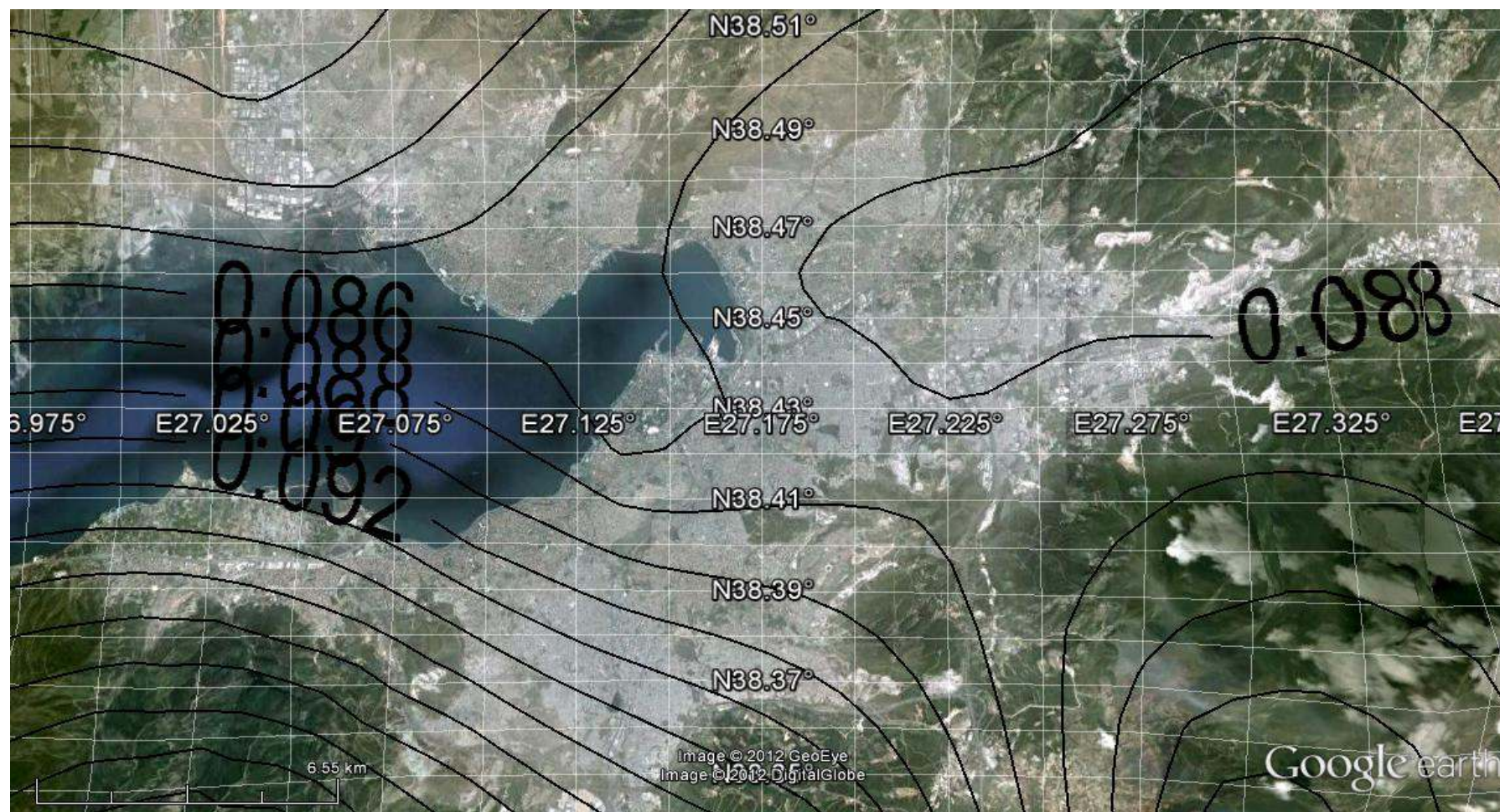
Figure E.25 (MAP 25): Attenuation relationship: Boore & Atkinson (2007). Probability of exceedance in 50 years: 50% Values: Ground Acceleration (g) (Median) Spectral period T=1 s V_{s30}=760 m/s
