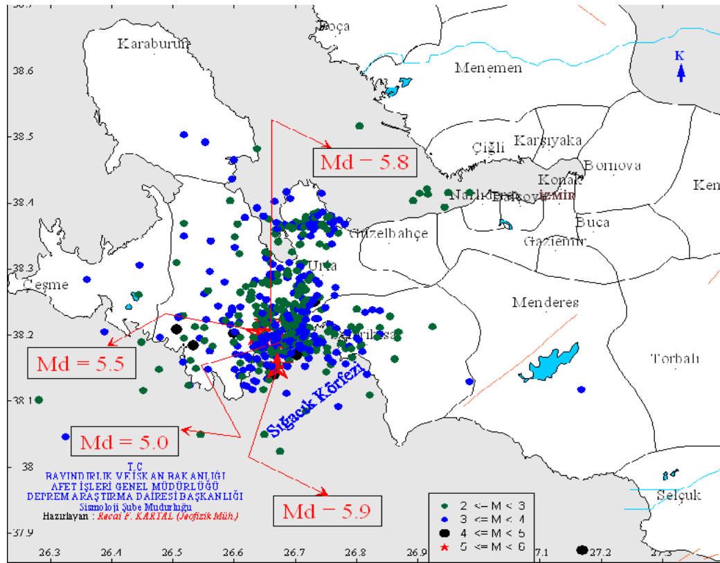
Figure 2.11 Location of epicenters of earthquakes occurred in Gulf of Sığacık and Seferihisar in October 2005 (Özden et al., 2011).
