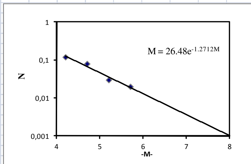
Figure D.5 Recurrence relationship for Source Zone 5
