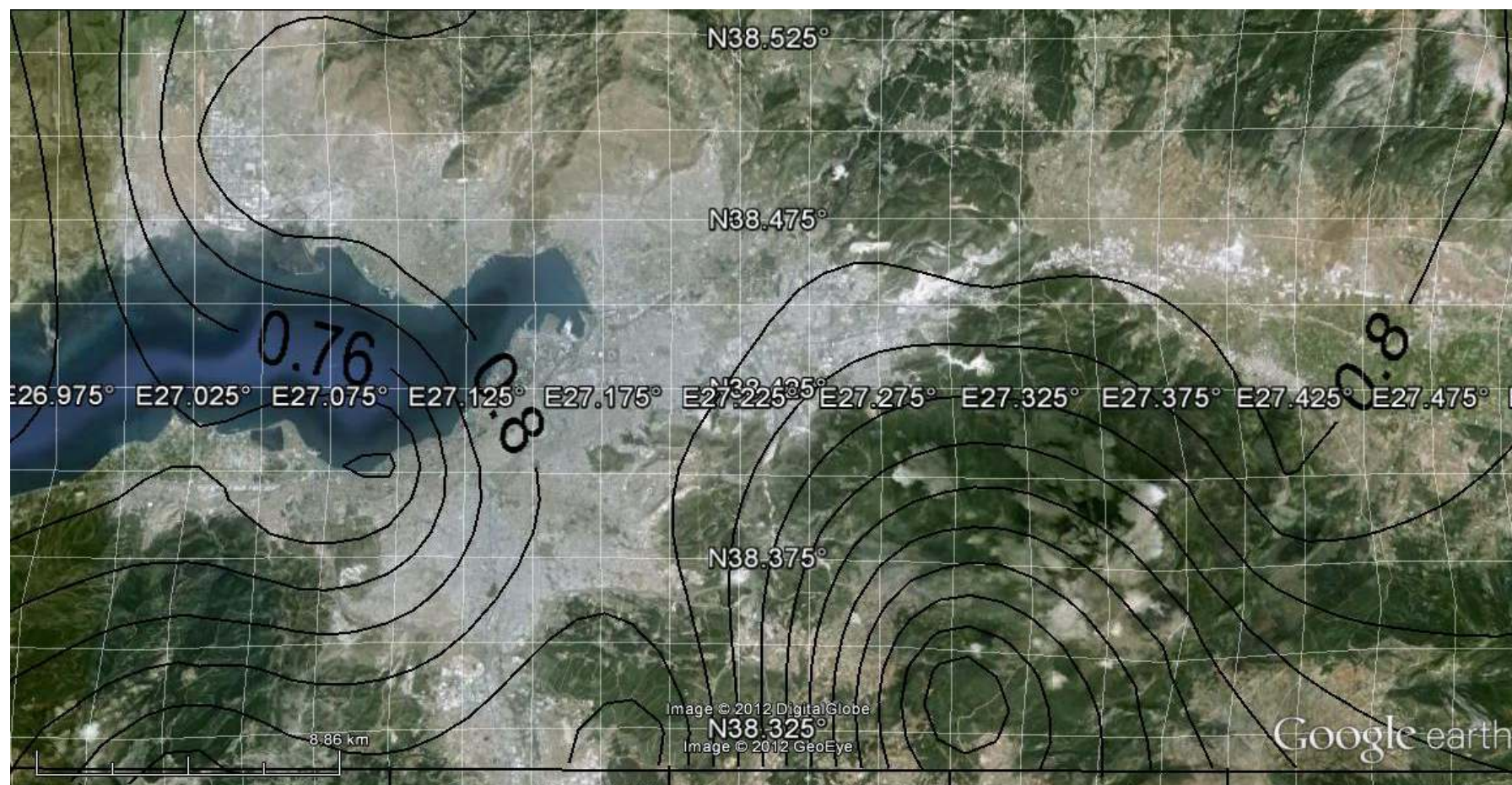
Figure E.30 (MAP 30): Attenuation relationship: Boore & Atkinson (2007). Probability of exceedance in 50 years: 2%
