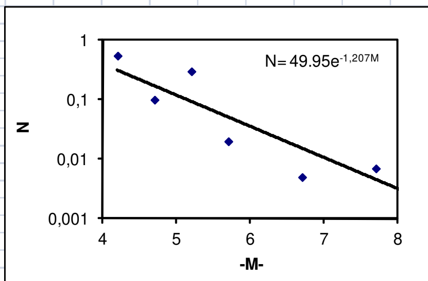
Figure D.1 Recurrence relationship for Source Zone 1
