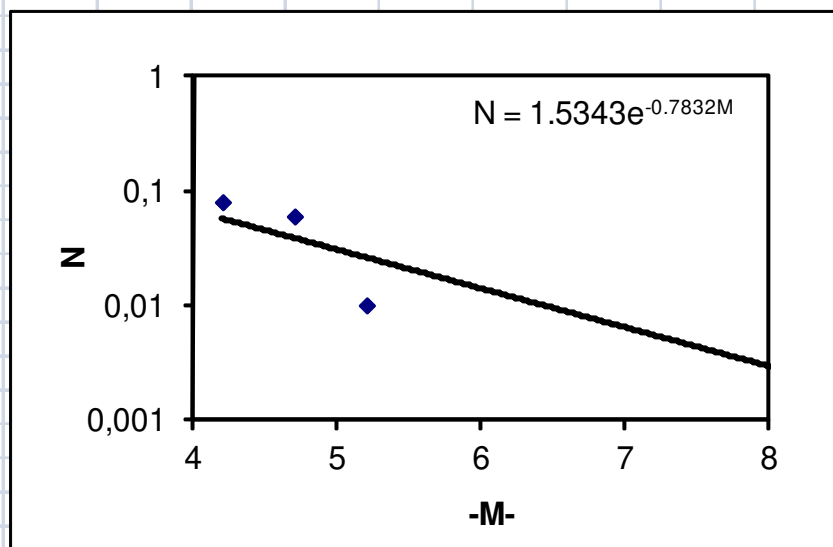
Figure D.2 Recurrence relationship for Source Zone 2
