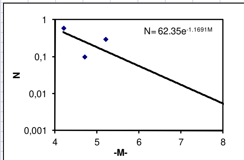
Figure D.3 Recurrence relationship for Source Zone 3
