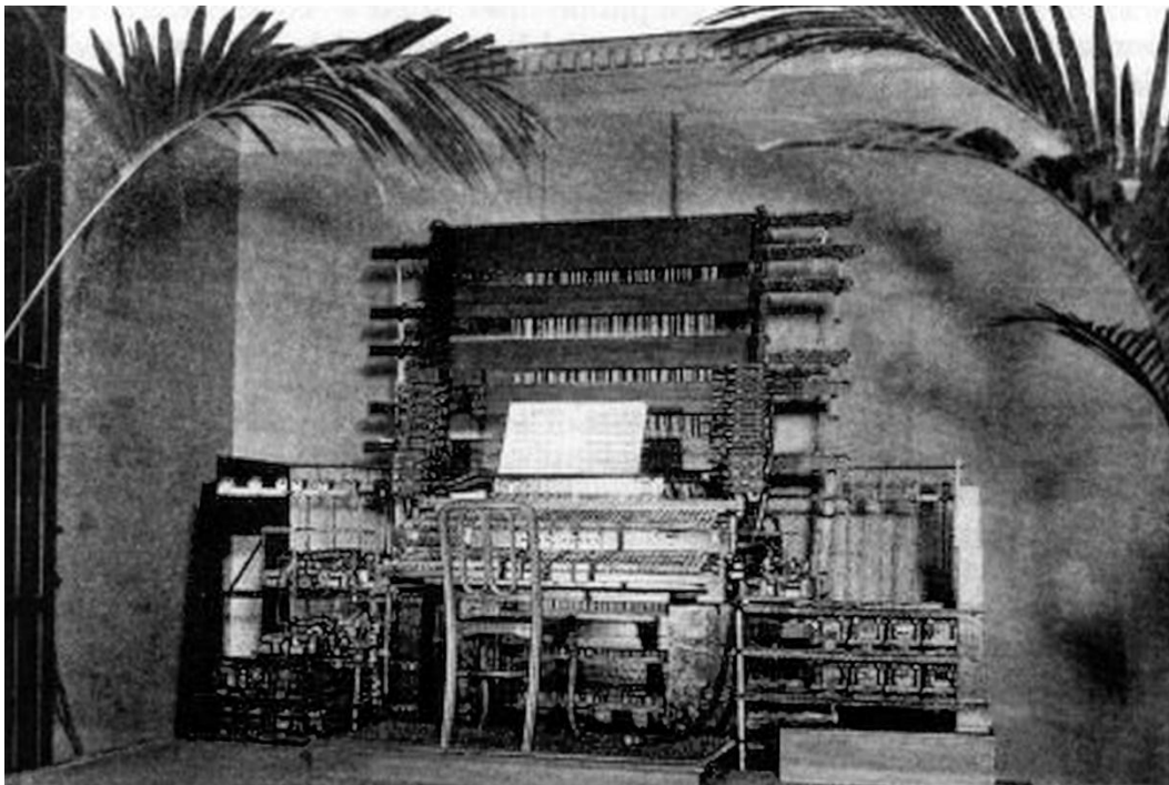
Figure 1.1 Telharmonium console by Thaddeus Cahill, 1897
