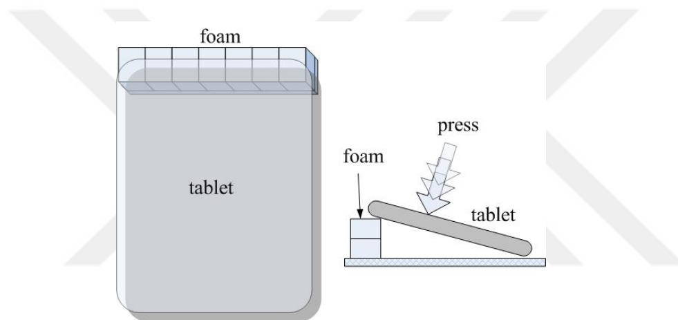
Figure 2.28 Typical fortissimo setup, from a top view (left) and side view (right) (Park and Nieto, 2013)
