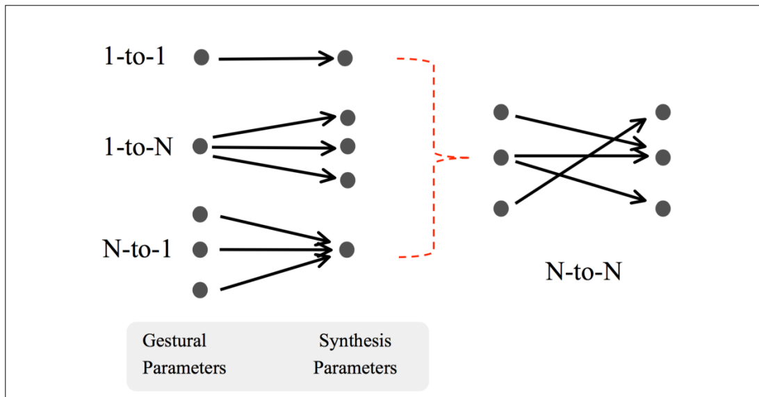
Figure 2.16 Types of mapping strategies (reproduced from Fels and Lyons, 2009).
