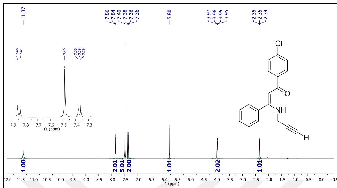
Figure 91. ^1\text{H} NMR spectrum of compound 26q.
