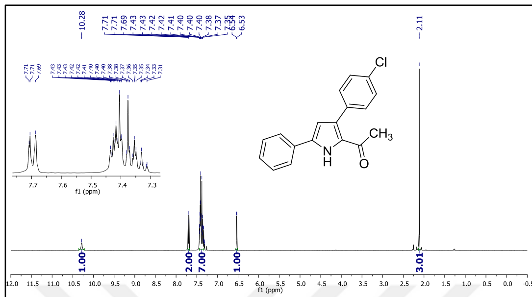
Figure 171. 1 H NMR spectrum of compound 46q .
