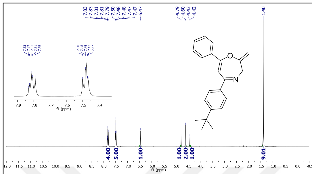
Figure 115. 1 H NMR spectrum of compound 37i.
