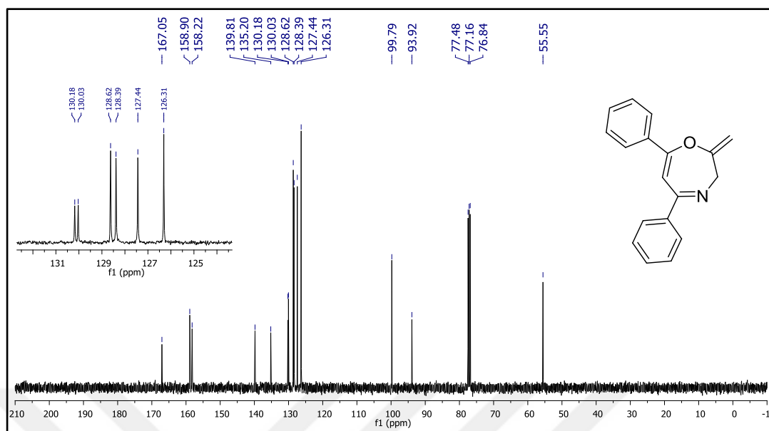
Figure 16. ^{13}\text{C} NMR spectrum of 2-methylene-5,7-diphenyl-2,3-dihydro-1,4-oxazepine ( 37a ).
