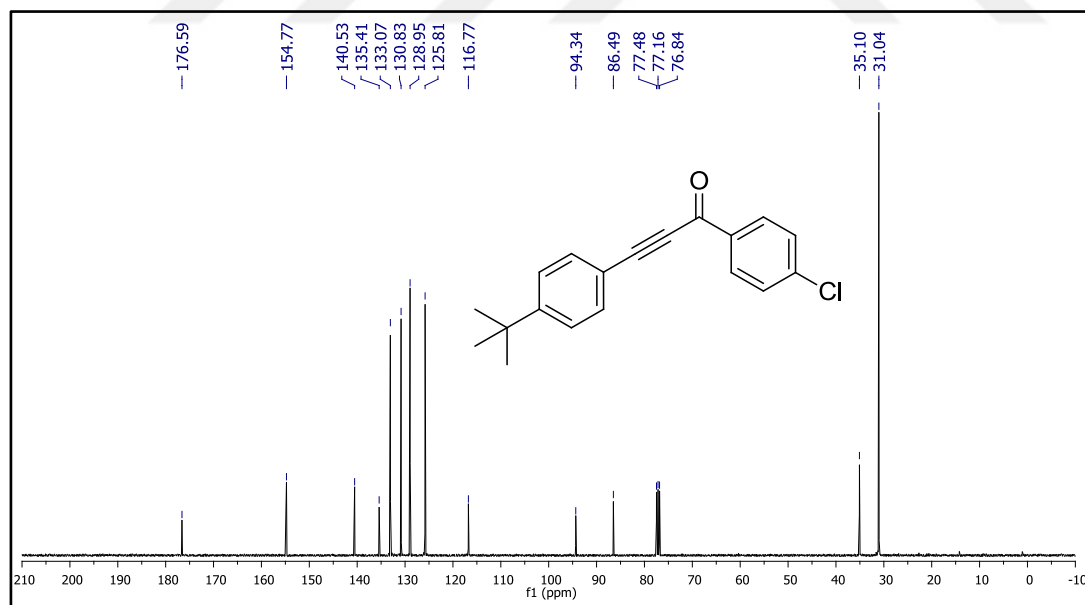
Figure 48. ^{13}\text{C} NMR spectrum of compound 49o .
