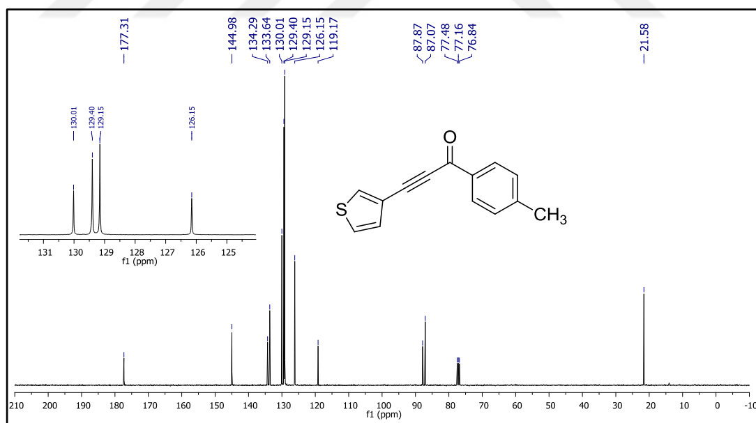
Figure 54. 13 C NMR spectrum of compound 49r.
