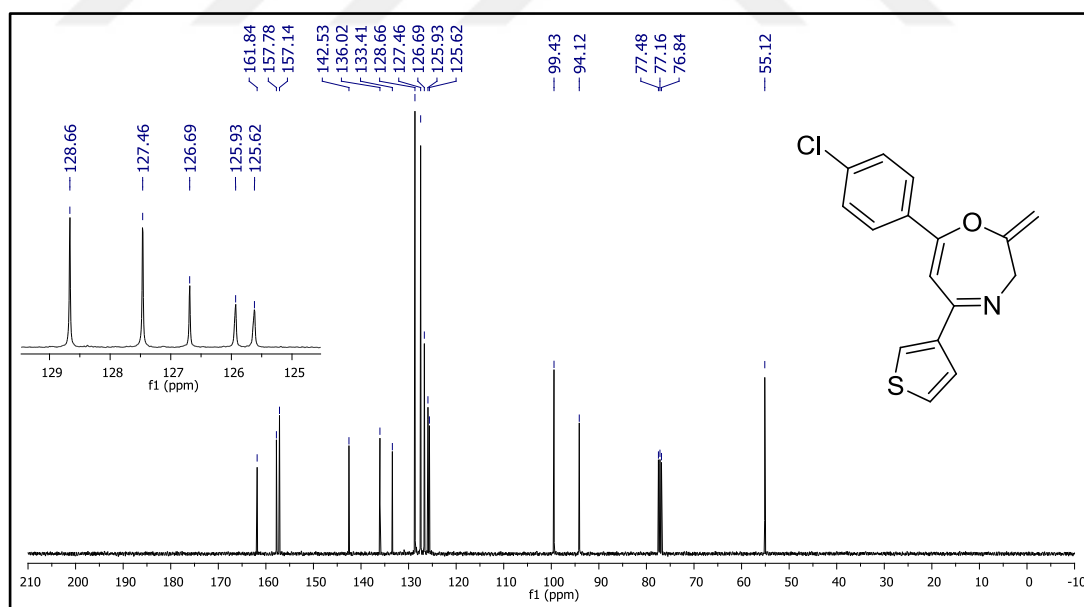
Figure 126. 13 C NMR spectrum of compound 37n.
