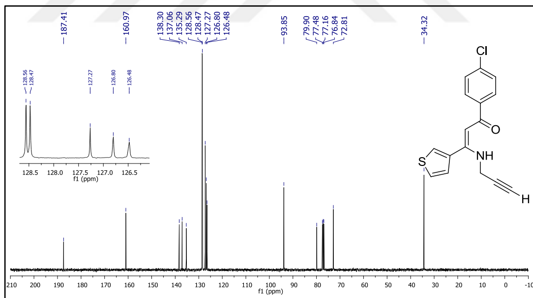
Figure 86. 13 C NMR spectrum of compound 26n.
