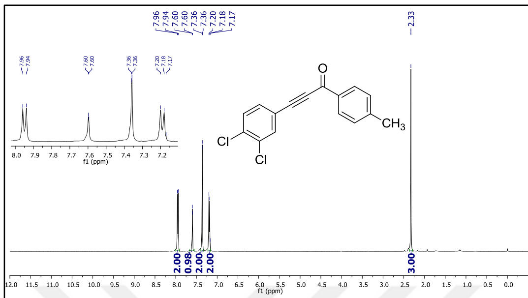
Figure 55. ^1\text{H} NMR spectrum of compound 49s.
