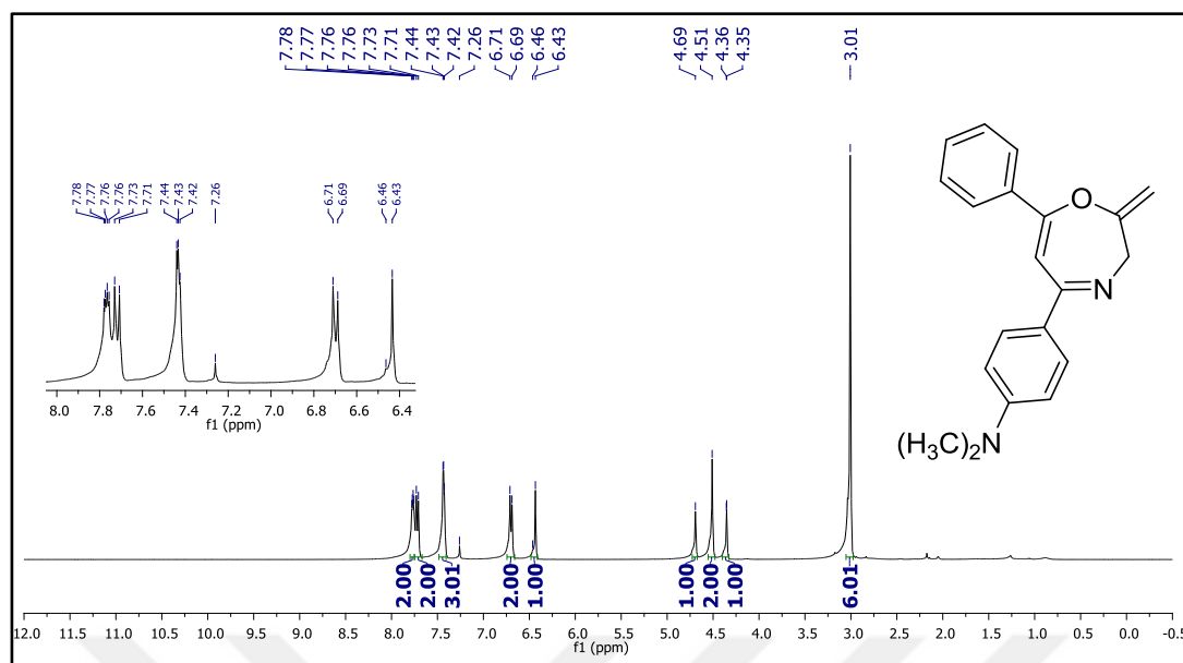
Figure 103. ^1\text{H} NMR spectrum of compound 37c.
