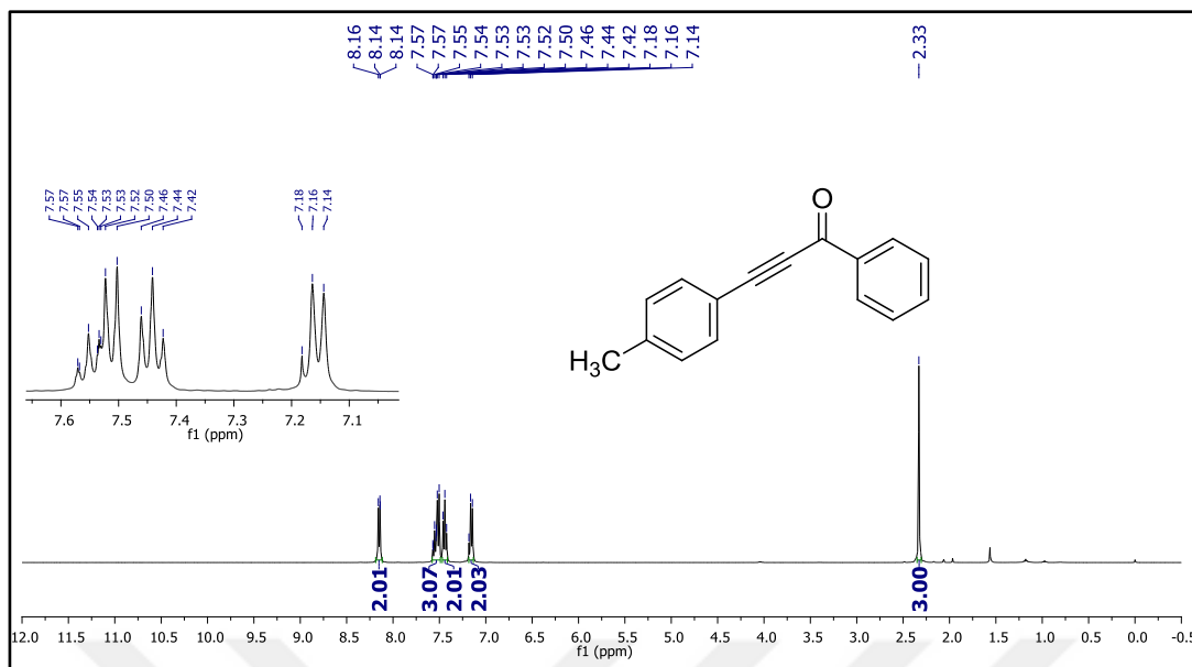
Figure 27. 1 H NMR spectrum of compound 49e.
