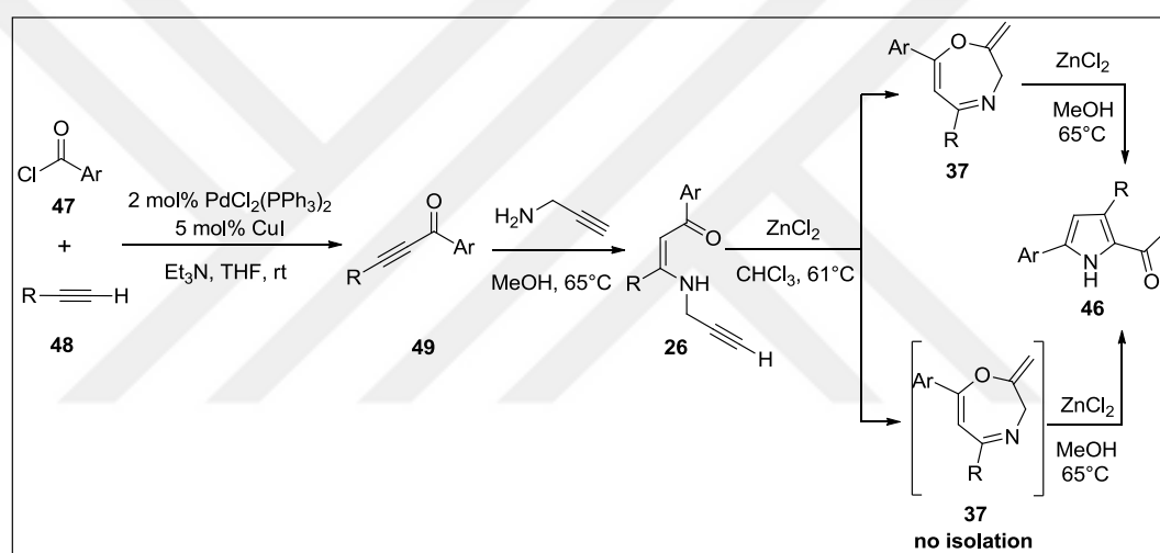
Scheme 27. General synthetic pathway for the synthesis of pyrroles 46 .
