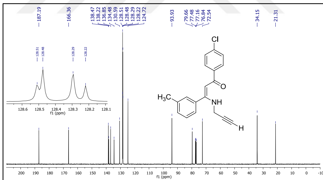
Figure 82. ^{13}\text{C} NMR spectrum of compound 26l.
