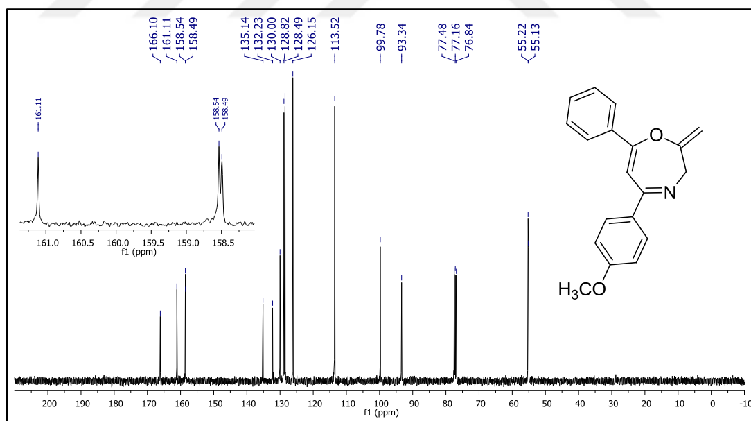
Figure 110. ^{13}\text{C} NMR spectrum of compound 37f.
