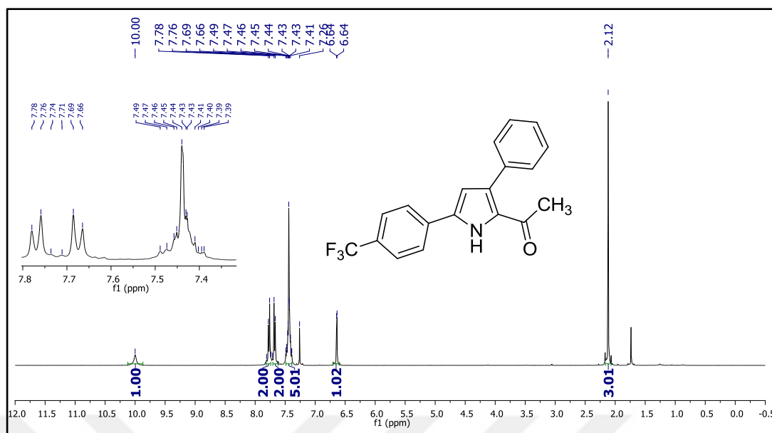
Figure 145. ^1\text{H} NMR spectrum of compound 46d.
