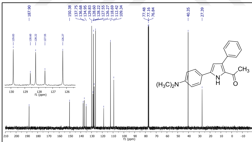
Figure 144. ^{13}\text{C} NMR spectrum of compound 46c.
