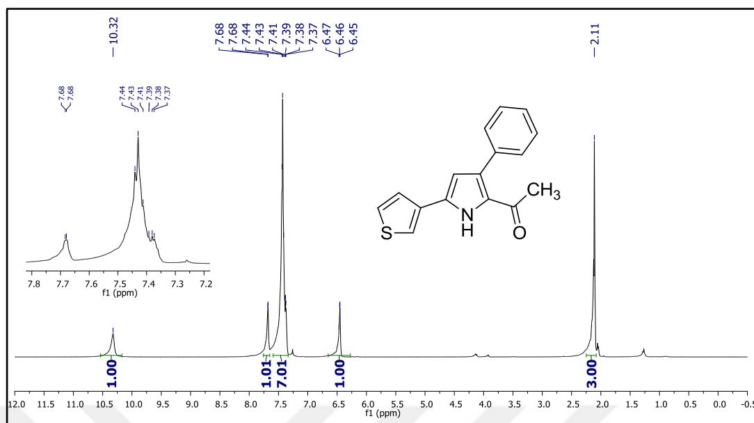
Figure 153. 1 H NMR spectrum of compound 46h.
