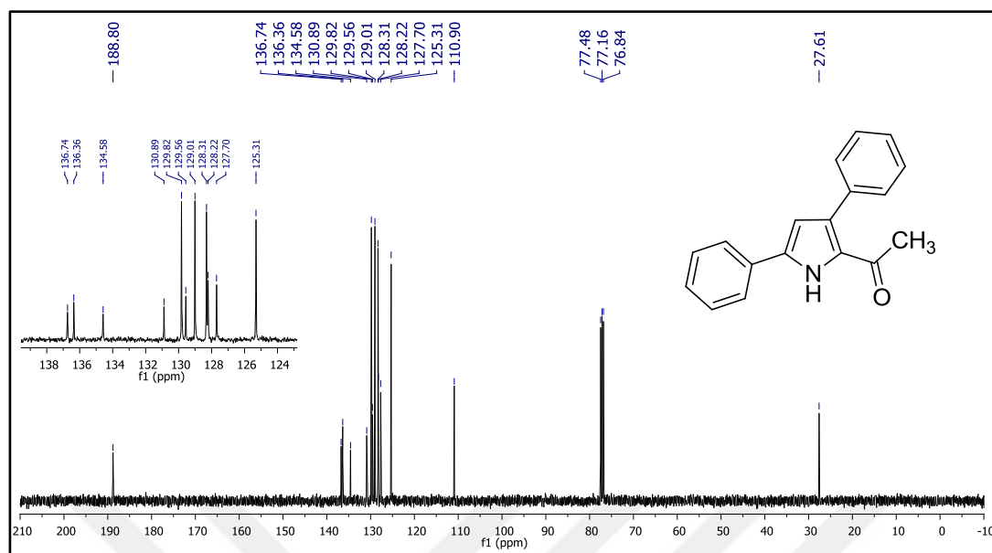
Figure 18. 13 C NMR spectra of 1-(3,5-diphenyl-1H-pyrrol-2-yl)ethanone ( 46a ).
