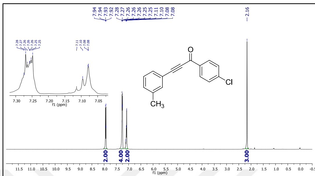
Figure 41. 1 H NMR spectrum of compound 49l.
