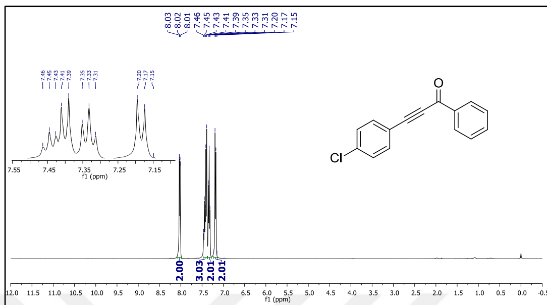
Figure 37. ^1\text{H} NMR spectrum of compound 49j.
