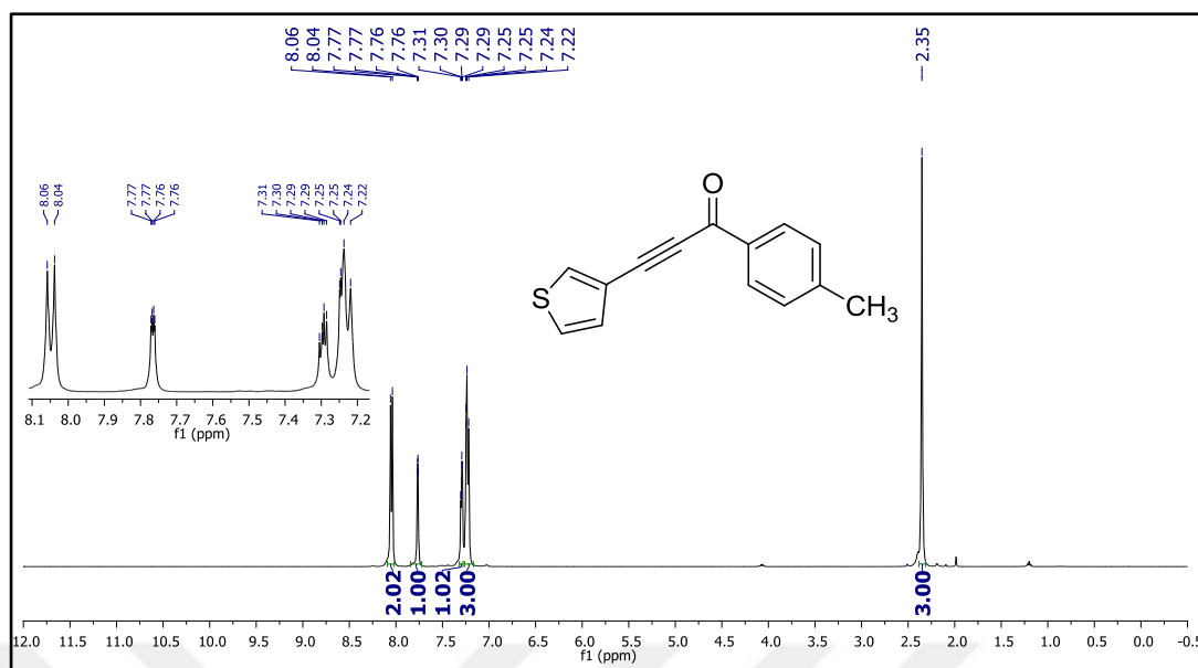
Figure 53. 1 H NMR spectrum of compound 49r.
