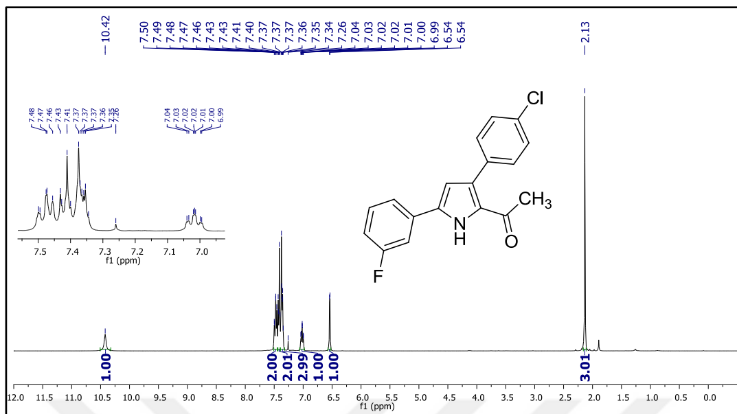
Figure 163. ^1\text{H} NMR spectrum of compound 46m.
