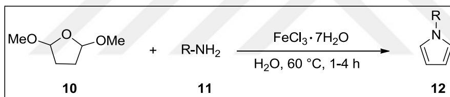
Scheme 4. Synthesis of iron catalyzed N -substituted pyrrole derivatives.
