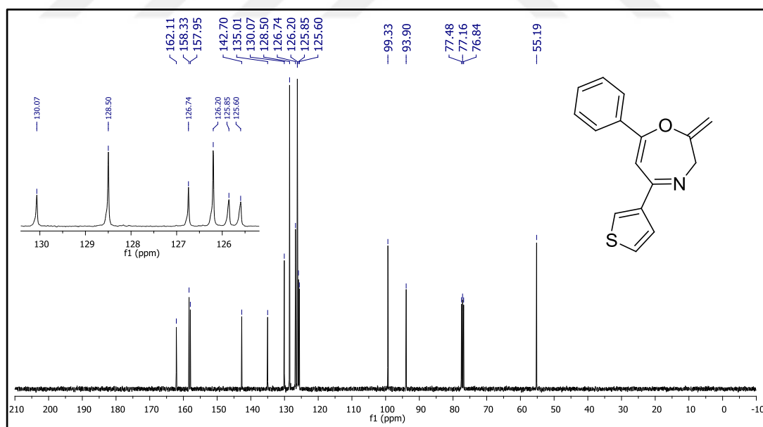
Figure 114. 13 C NMR spectrum of compound 37h.
