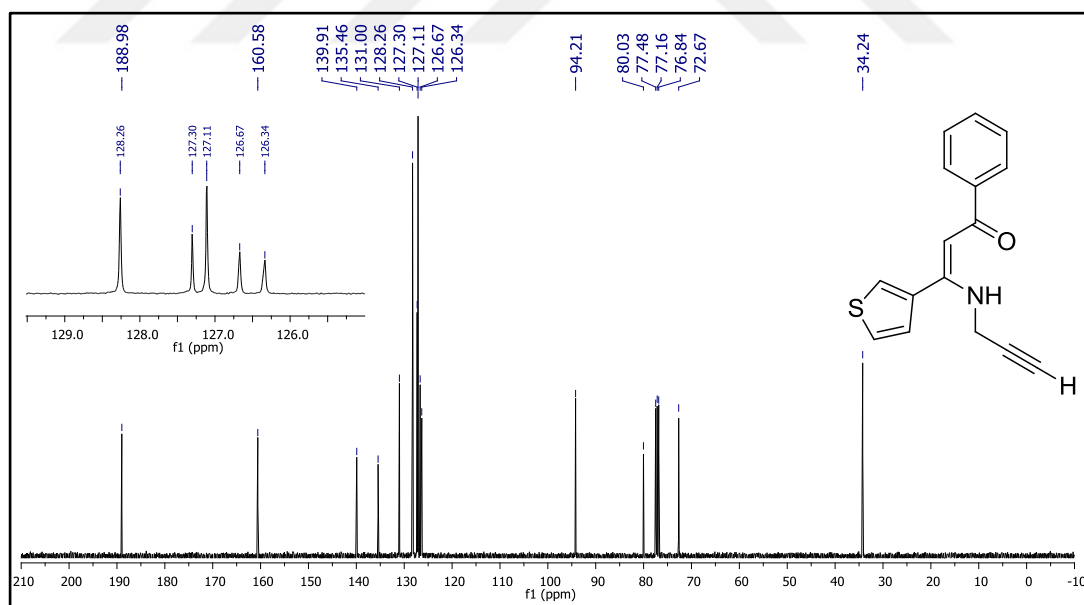
Figure 74. ^{13}\text{C} NMR spectrum of compound 26h.
