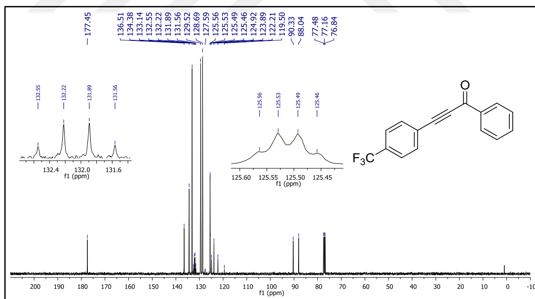
Figure 26. ^{13}\text{C} NMR spectrum of compound 49d .
