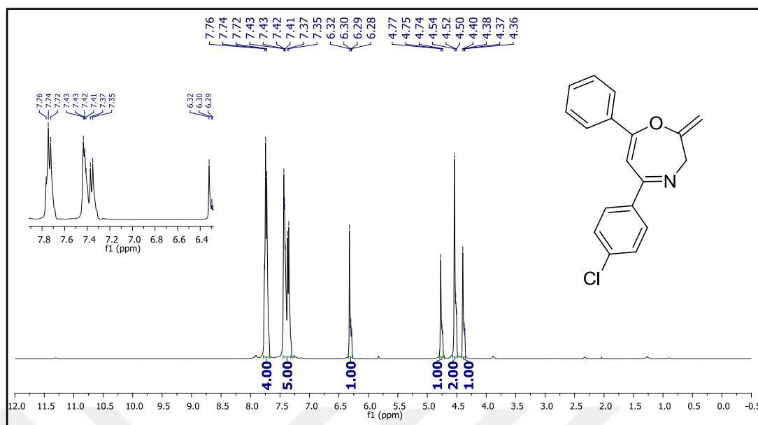
Figure 117. 1 H NMR spectrum of compound 37j.
