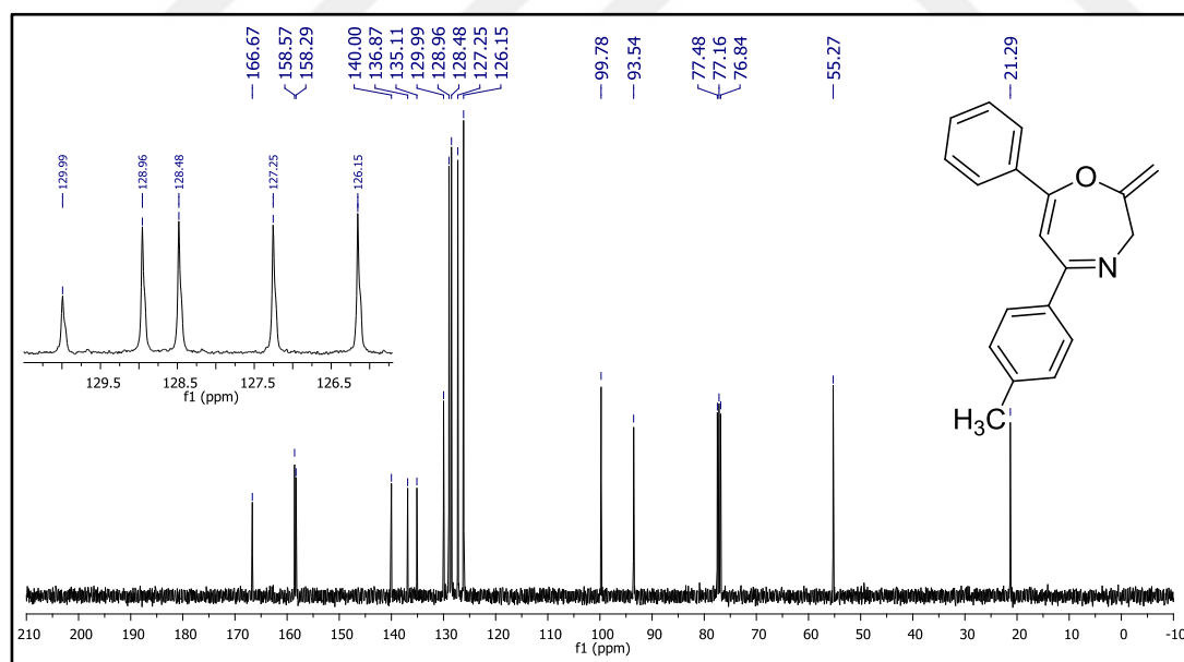
Figure 108. 13 C NMR spectrum of compound 37e.
