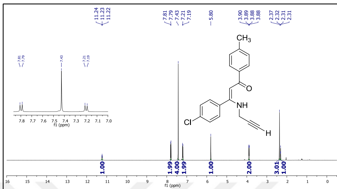
Figure 97. ^1\text{H} NMR spectrum of compound 26t.
