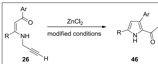
Scheme 25. Synthesis of pyrroles 46 in modified conditions.
