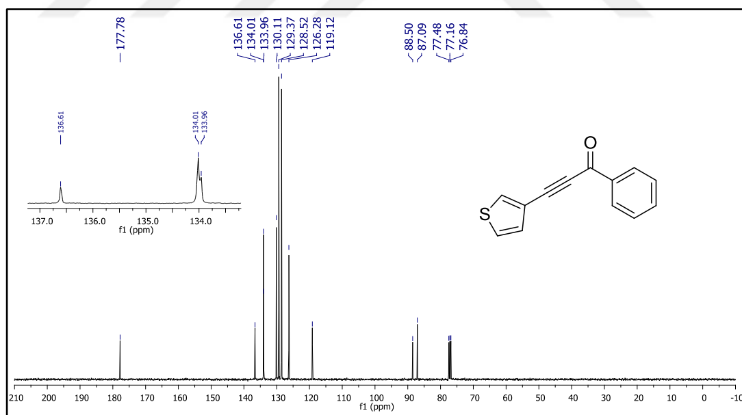
Figure 34. ^{13}\text{C} NMR spectrum of compound 49h.
