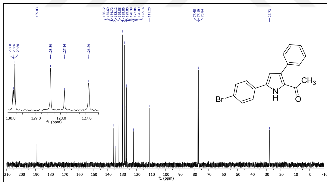
Figure 160. 13 C NMR spectrum of compound 46k.
