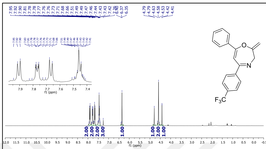
Figure 105. 1 H NMR spectrum of compound 37d.
