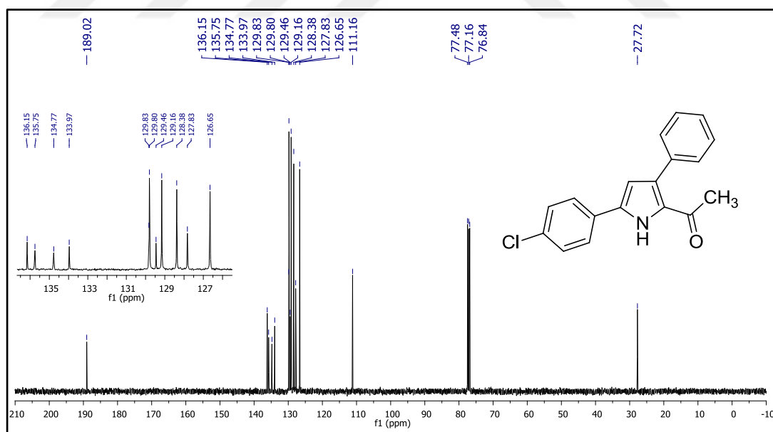
Figure 158. ^{13}\text{C} NMR spectrum of compound 46j.
