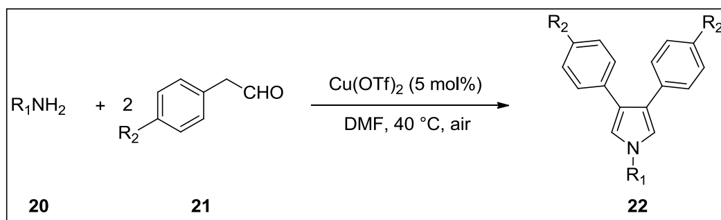
Scheme 7. Synthesis of 1,3,4-trisubstituted pyrrole derivatives.
