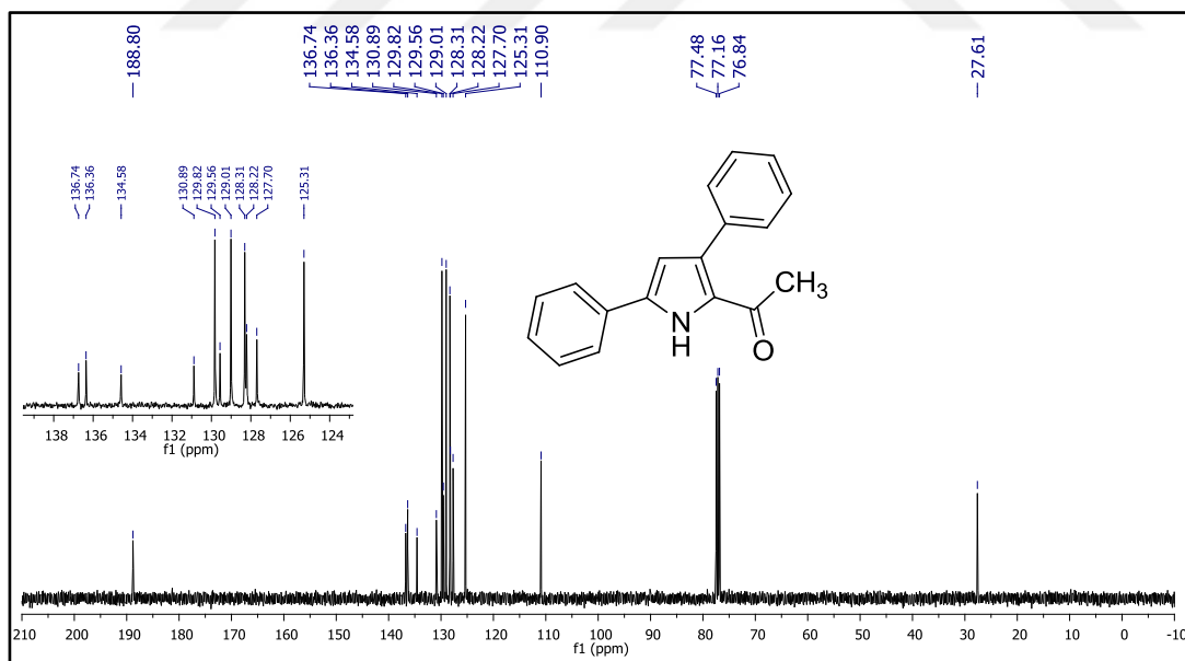
Figure 140. ^{13}\text{C} NMR spectrum of compound 46a .
