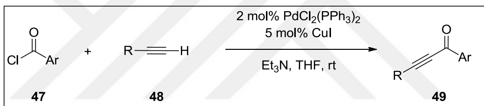
Scheme 22. Synthesis of \alpha,\beta -alkynic ketones 49 .
