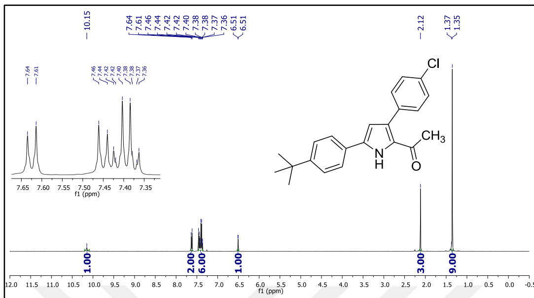
Figure 167. 1 H NMR spectrum of compound 46o .
