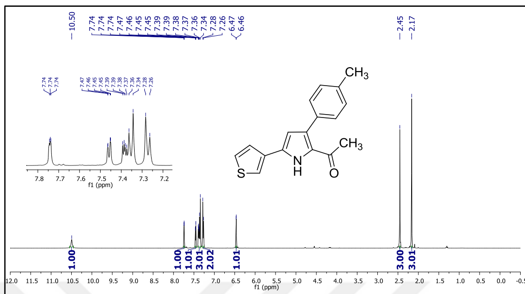
Figure 173. 1 H NMR spectrum of compound 46r.
