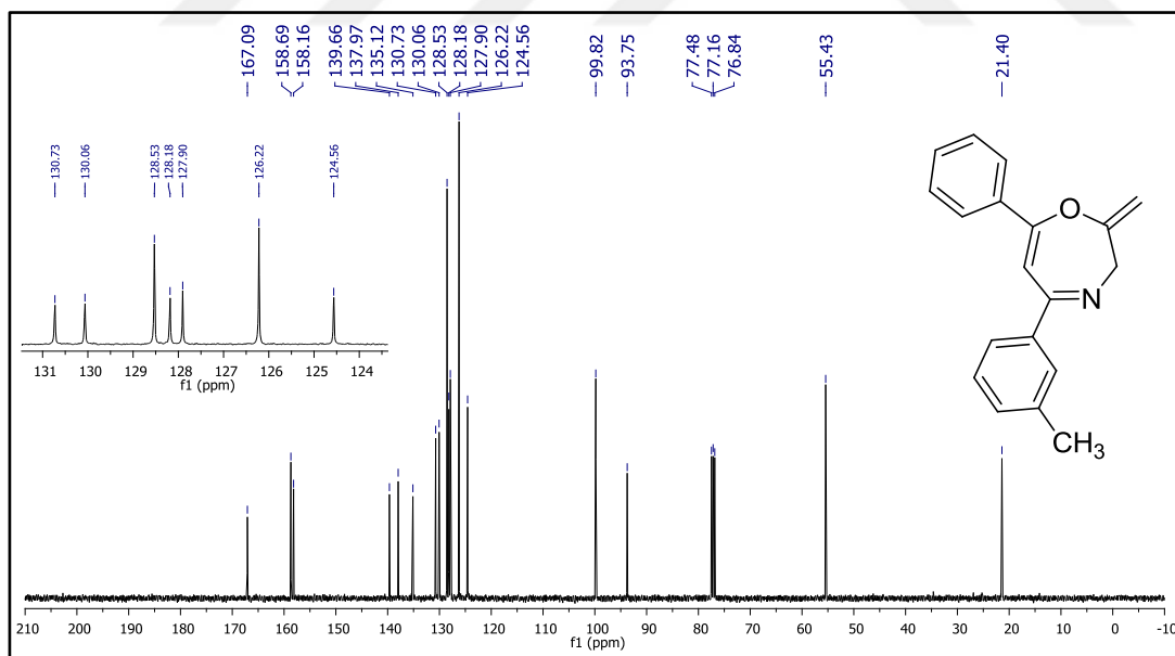
Figure 112. 13 C NMR spectrum of compound 37g.
