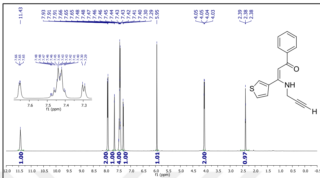
Figure 73. ^1\text{H} NMR spectrum of compound 26h.
