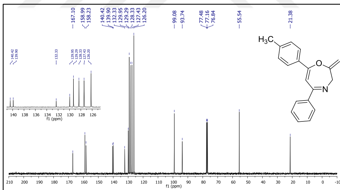
Figure 130. 13 C NMR spectrum of compound 37p.
