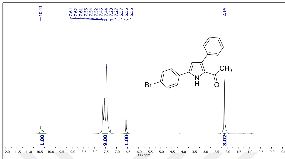
Figure 159. 1 H NMR spectrum of compound 46k.
