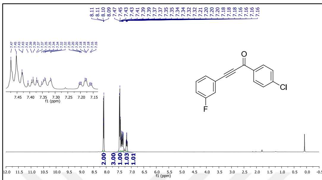
Figure 43. ^1\text{H} NMR spectrum of compound 49m .
