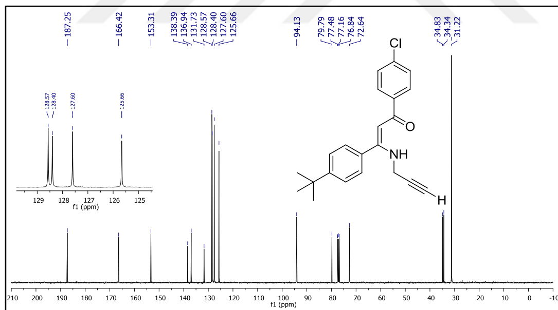
Figure 88. ^{13}\text{C} NMR spectrum of compound 26o.
