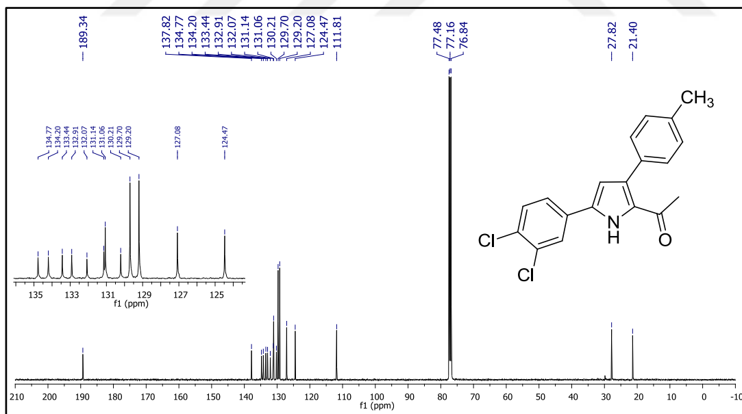
Figure 176. 13 C NMR spectrum of compound 46s.
