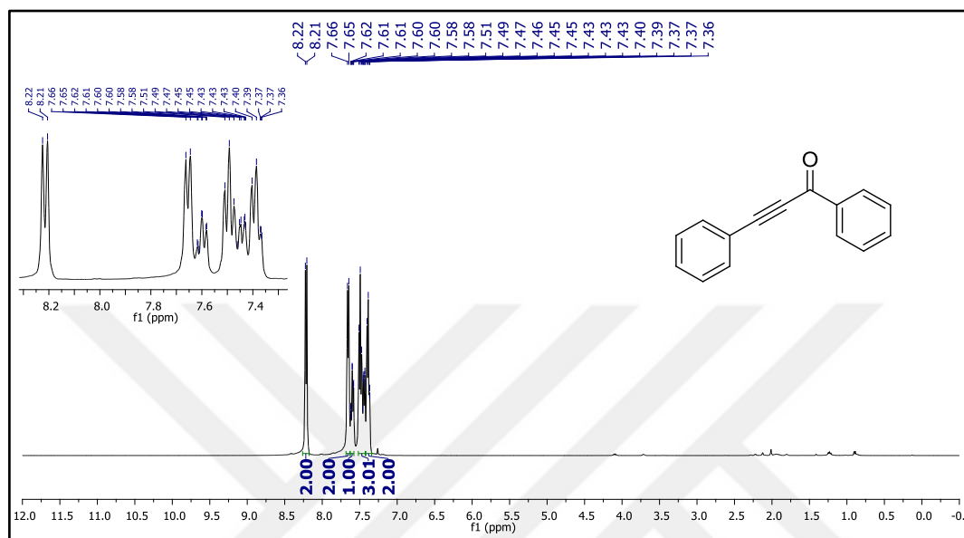
Figure 11. 1 H NMR spectrum of 1,3-diphenylprop-2-yn-1-one (49a).
