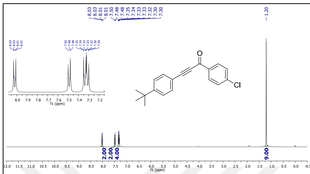
Figure 47. ^1\text{H} NMR spectrum of compound 49o .
