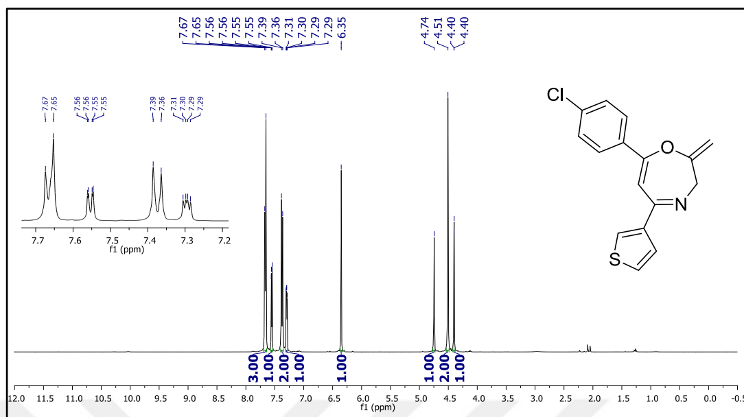
Figure 125. 1 H NMR spectrum of compound 37n.
