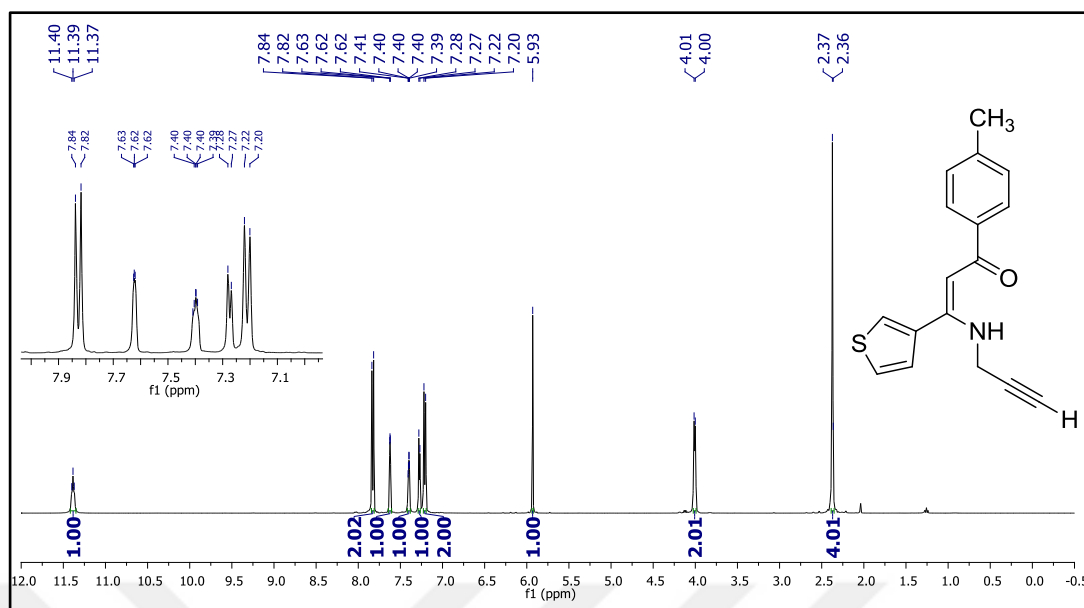
Figure 93. ^1\text{H} NMR spectrum of compound 26r.
