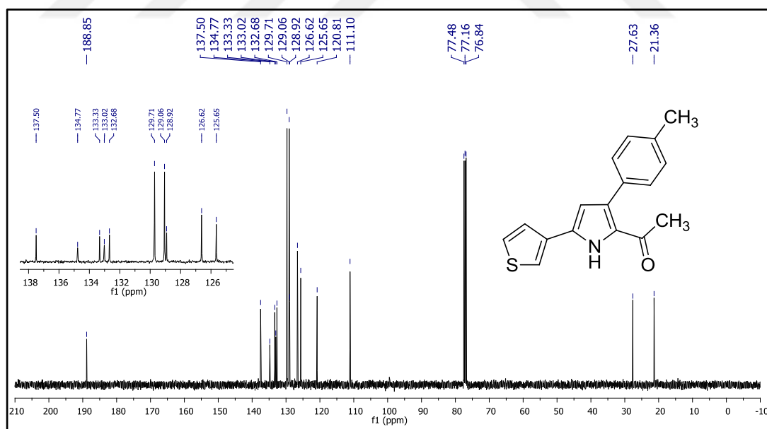
Figure 174. 13 C NMR spectrum of compound 46r.
