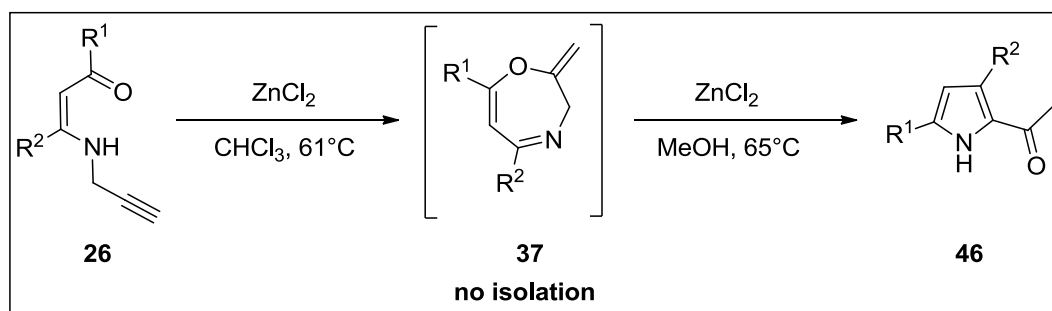
Scheme 21. Synthesis of pyrrole derivatives from N -propargylic \beta -enaminones 26 via one-pot two-step synthesis method.
