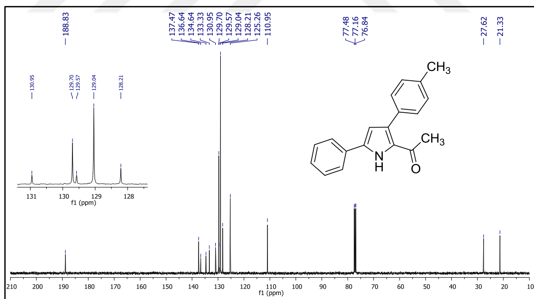
Figure 170. 13 C NMR spectrum of compound 46p.
