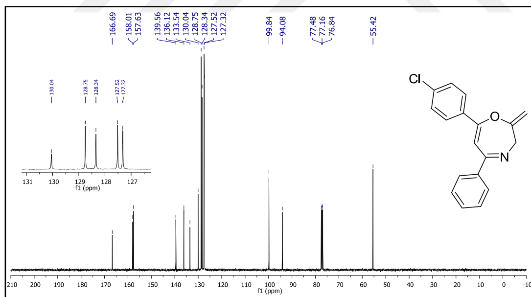
Figure 132. 13 C NMR spectrum of compound 37q .
