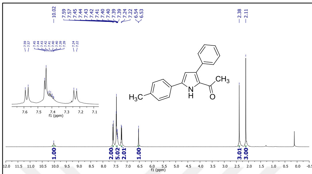
Figure 147. 1 H NMR spectrum of compound 46e.
