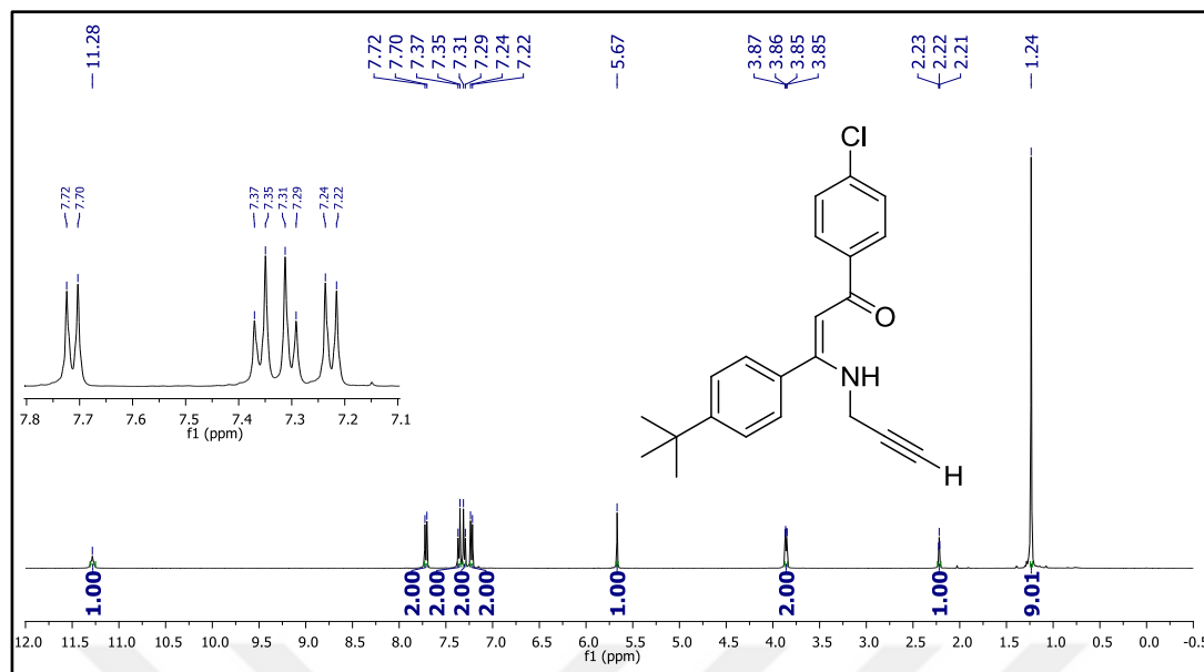
Figure 87. ^1\text{H} NMR spectrum of compound 26o.
