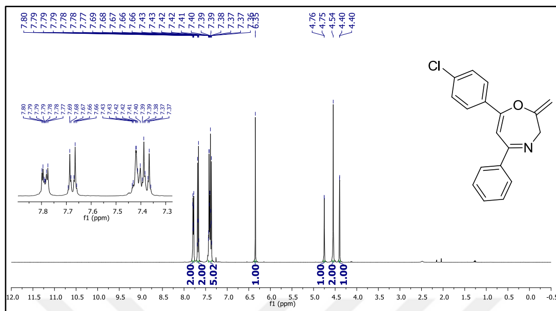
Figure 131. 1 H NMR spectrum of compound 37q .
