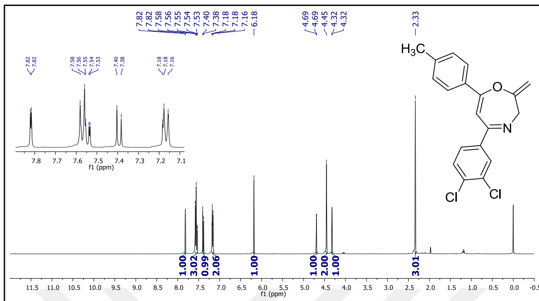
Figure 135. 1 H NMR spectrum of compound 37s.
