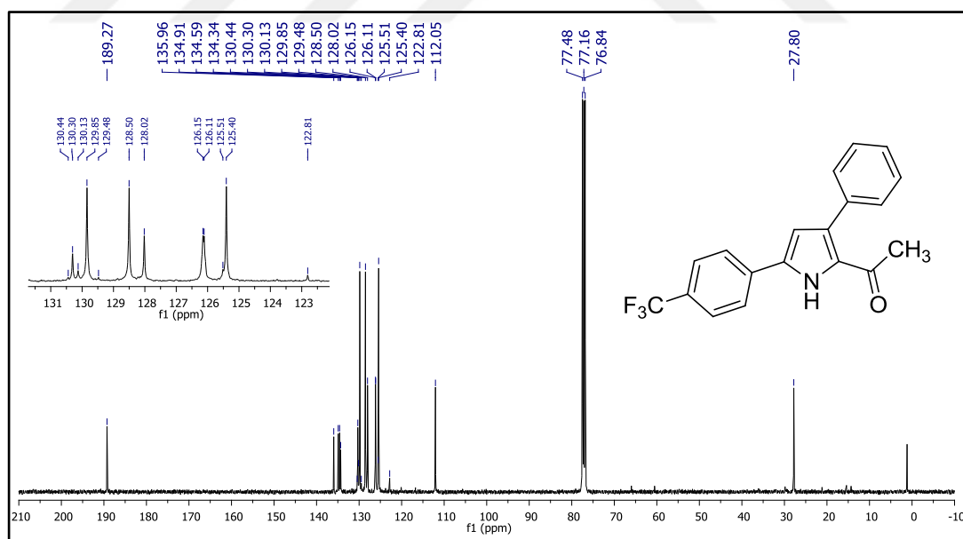
Figure 146. ^{13}\text{C} NMR spectrum of compound 46d.
