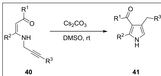
Scheme 14. Synthesis of polysubstituted pyrroles.
