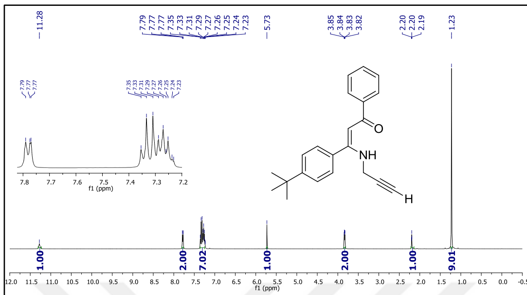
Figure 75. ^1\text{H} NMR spectrum of compound 26i.
