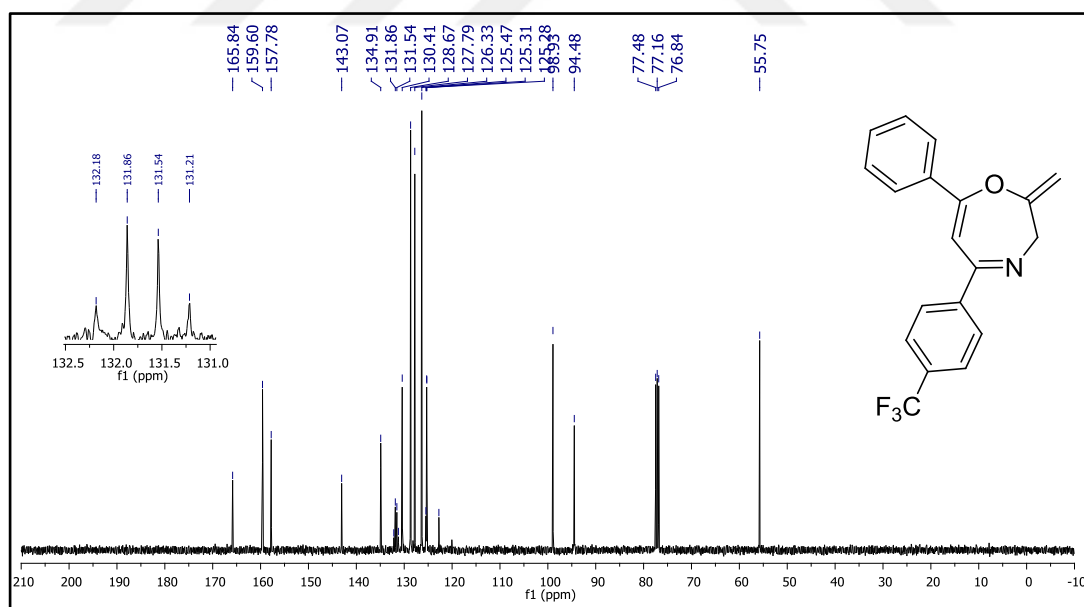
Figure 106. 13 C NMR spectrum of compound 37d.
