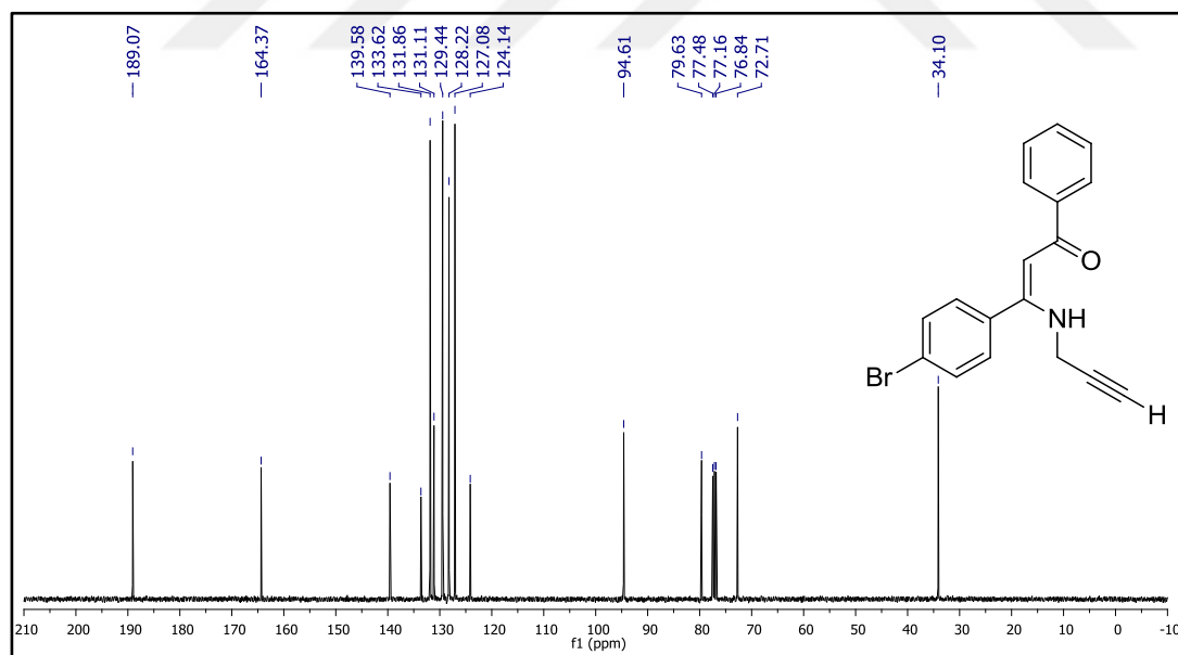
Figure 80. 13 C NMR spectrum of compound 26k.
