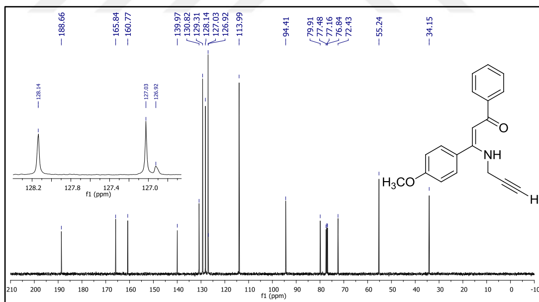
Figure 70. 13 C NMR spectrum of compound 26f.
