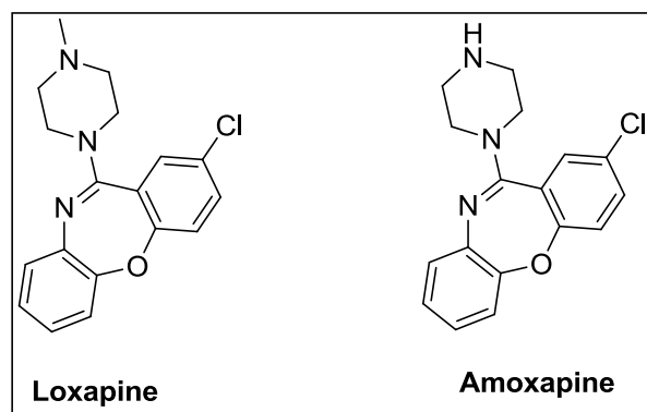
Figure 7. 1,4-Oxazepine containing drugs.
