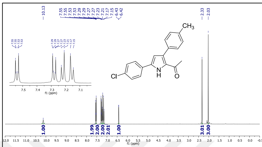
Figure 177. ^1\text{H} NMR spectrum of compound 46t.
