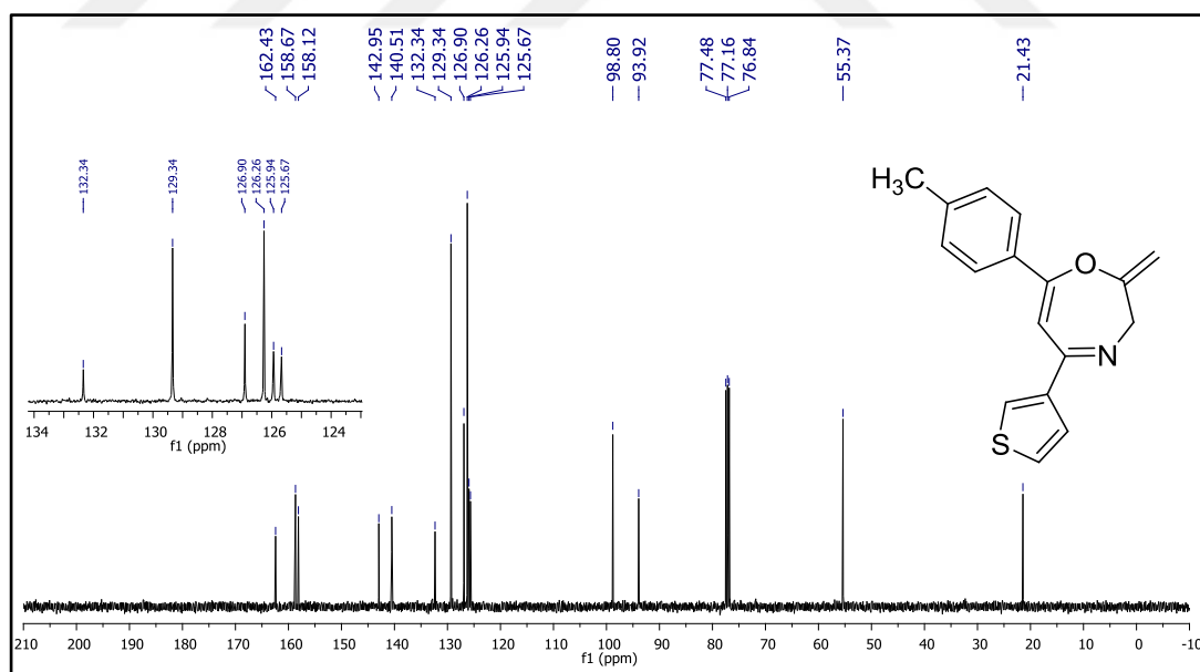
Figure 134. 13 C NMR spectrum of compound 37r.
