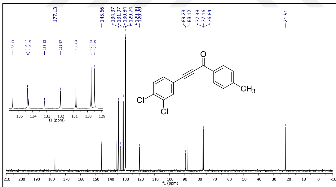
Figure 56. ^{13}\text{C} NMR spectrum of compound 49s.
