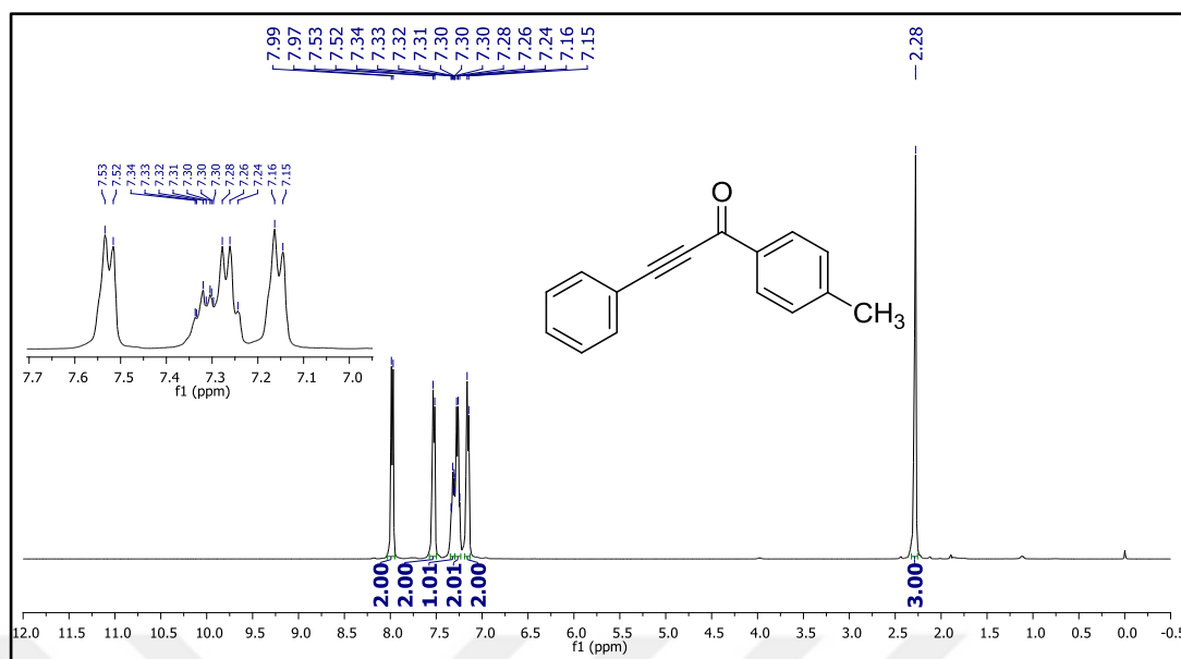
Figure 49. ^1\text{H} NMR spectrum of compound 49p.
