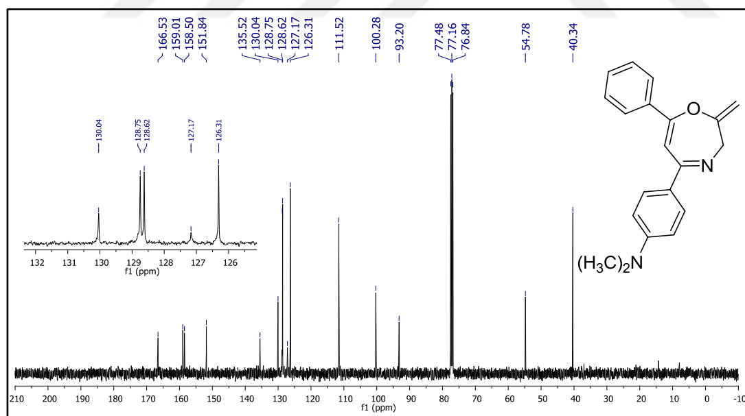
Figure 104. ^{13}\text{C} NMR spectrum of compound 37c.
