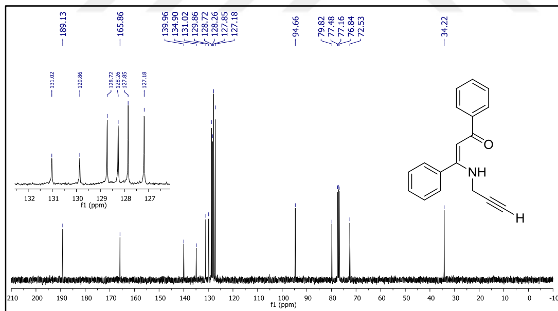
Figure 60. 13 C NMR spectrum of compound 26a.
