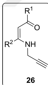
Figure 10. Structure of N -propargylic \beta -enaminones.
