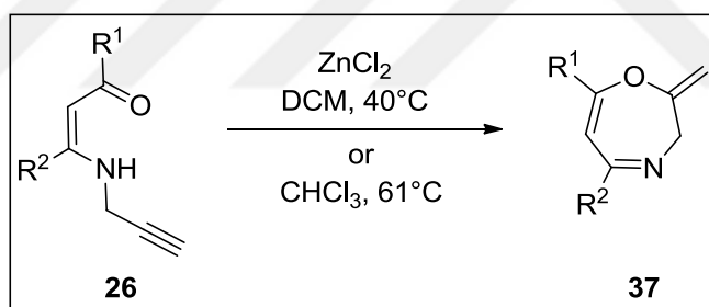
Scheme 18. Synthesis of 2-methylene-2,3-dihydro-1,4-oxaepines 37 .
