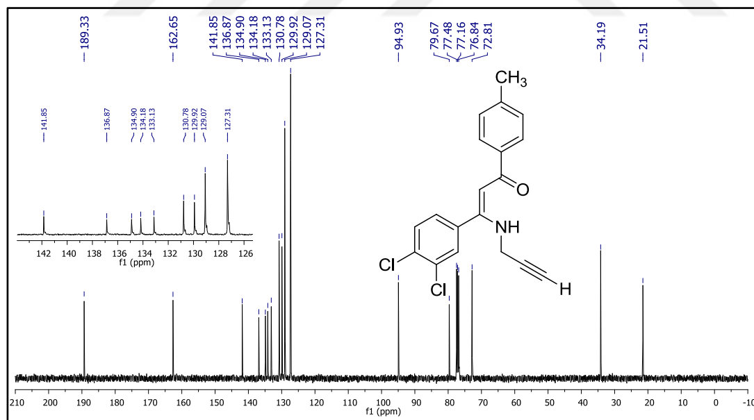
Figure 96. 13 C NMR spectrum of compound 26s.
