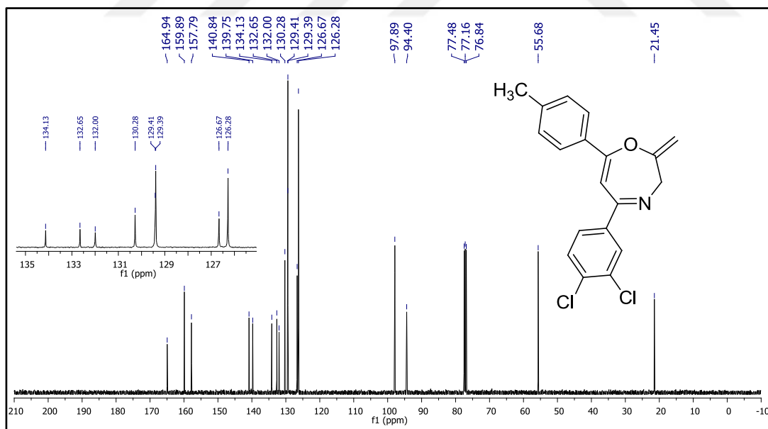
Figure 136. 13 C NMR spectrum of compound 37s.
