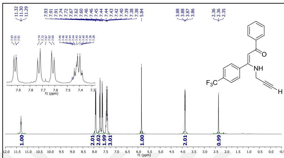
Figure 65. 1 H NMR spectrum of compound 26d.
