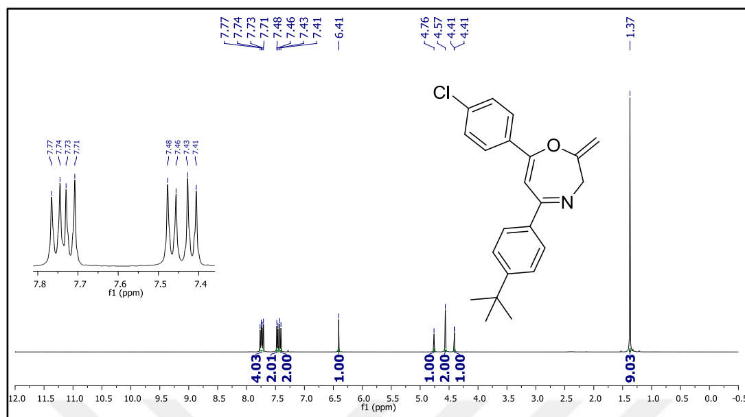
Figure 127. ^1\text{H} NMR spectrum of compound 37o.
