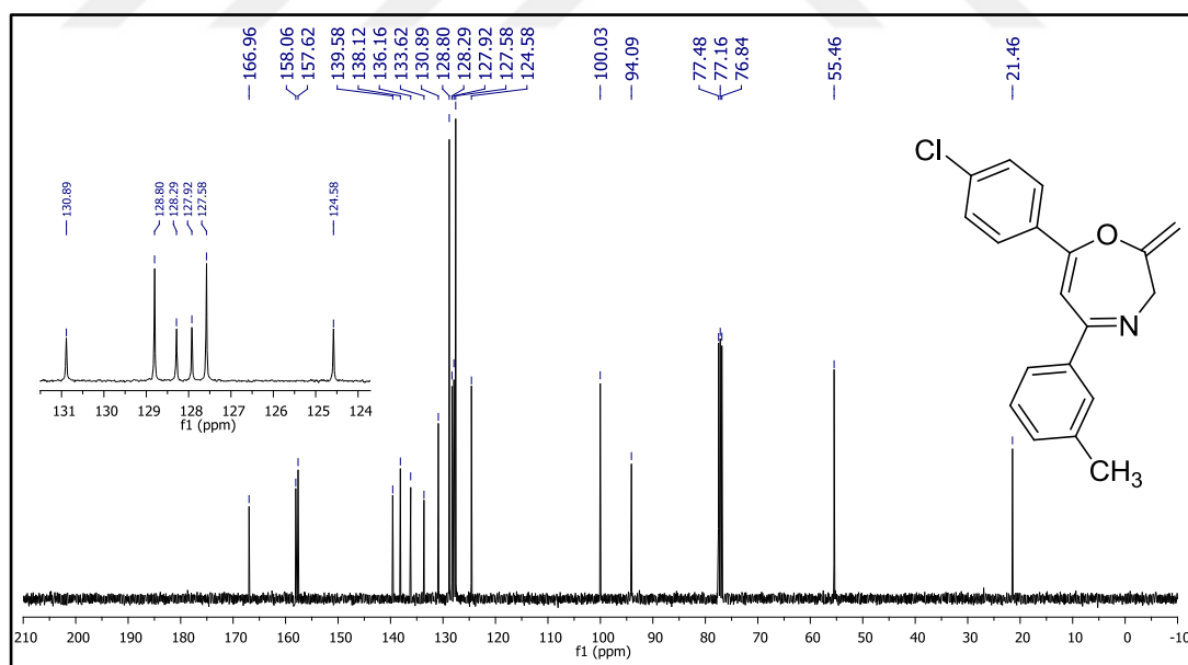
Figure 122. 13 C NMR spectrum of compound 37I.
