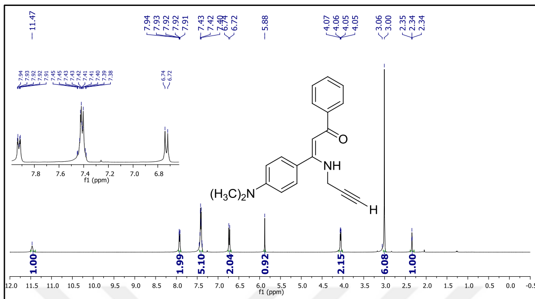
Figure 63. 1 H NMR spectrum of compound 26c.
