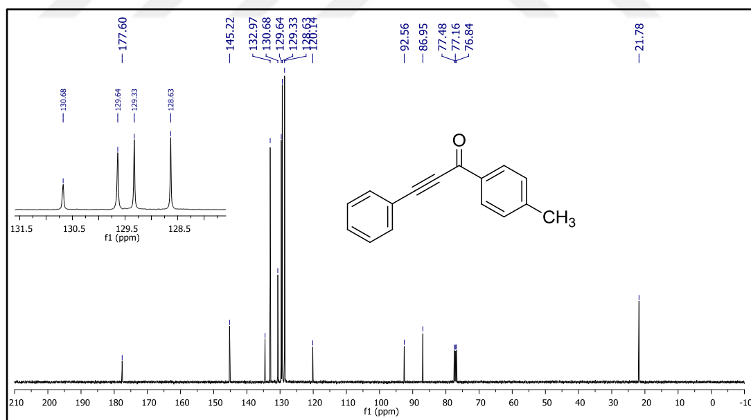
Figure 50. ^{13}\text{C} NMR spectrum of compound 49p.
