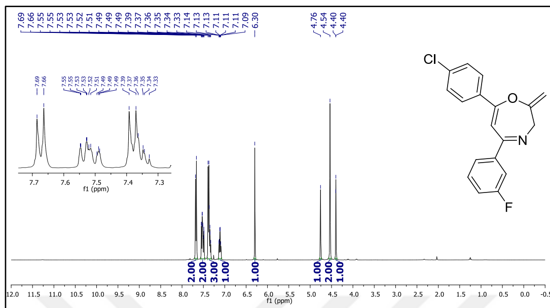
Figure 123. 1 H NMR spectrum of compound 37m.
