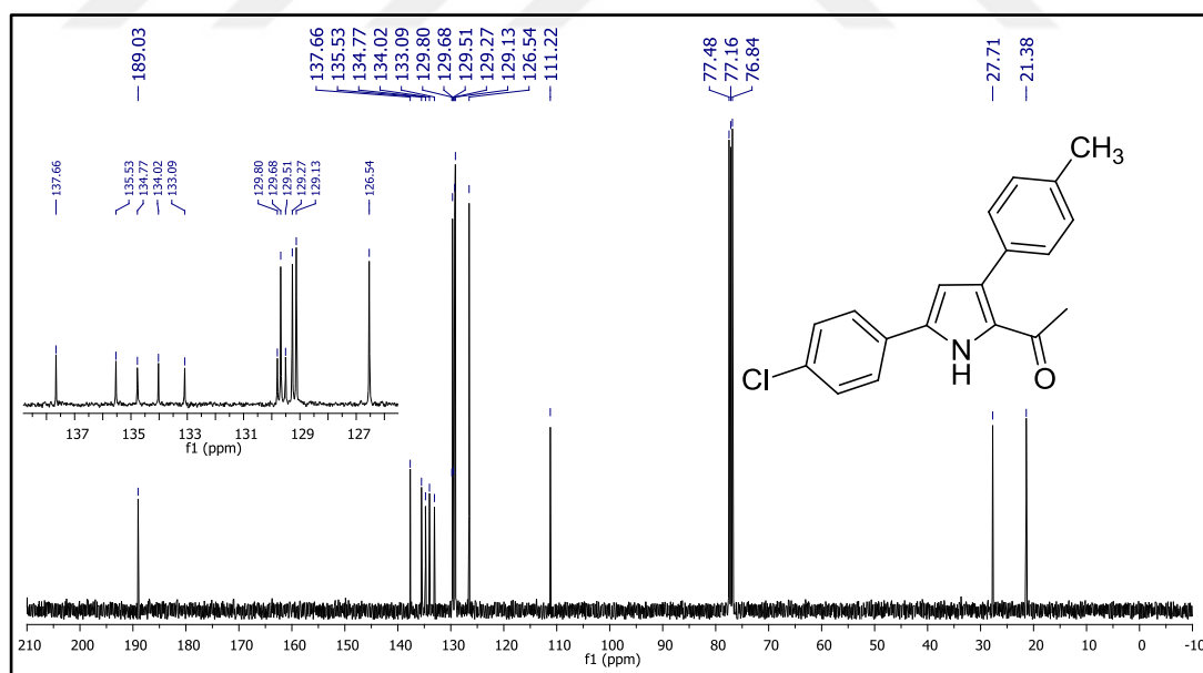
Figure 178. ^{13}\text{C} NMR spectrum of compound 46t.
