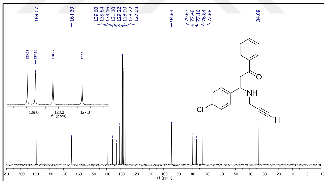
Figure 78. 13 C NMR spectrum of compound 26j.
