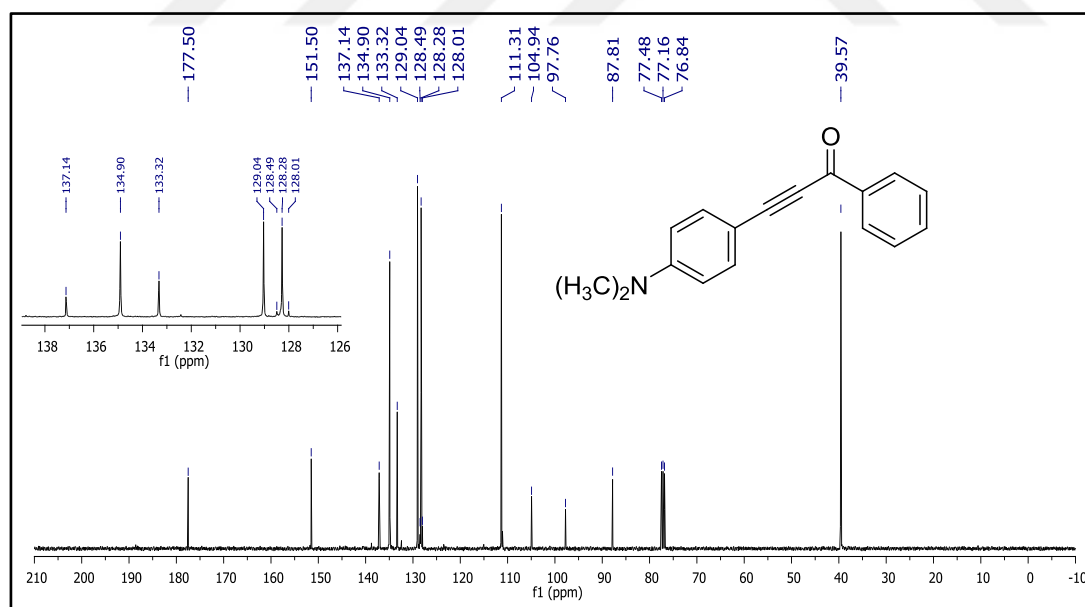
Figure 24. 13 C NMR spectrum of compound 49c.
