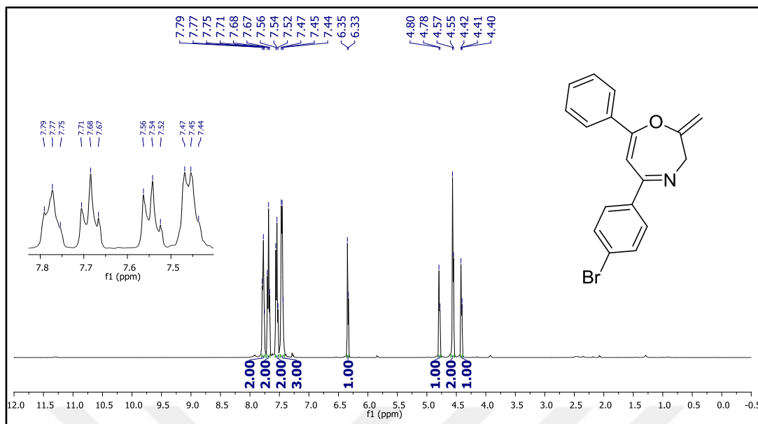
Figure 119. 1 H NMR spectrum of compound 37k.
