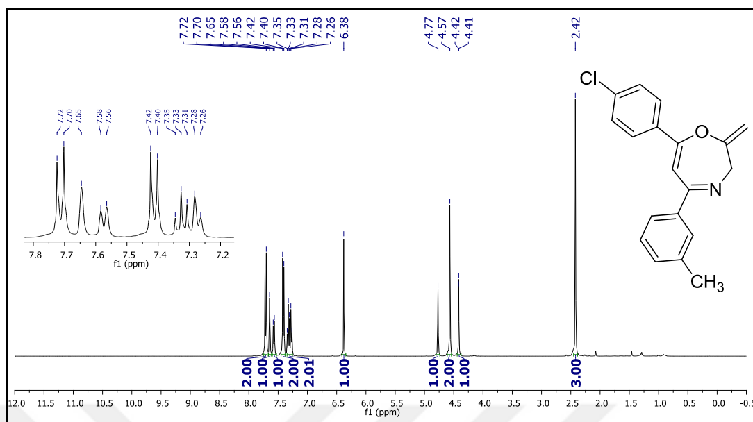
Figure 121. 1 H NMR spectrum of compound 37I.
