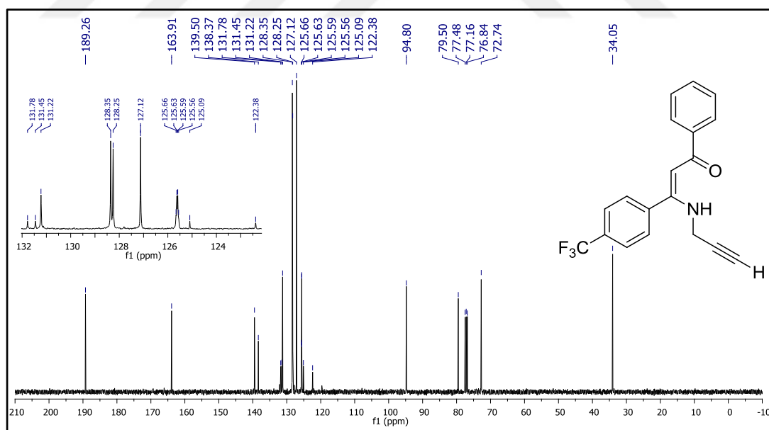
Figure 66. 13 C NMR spectrum of compound 26d.
