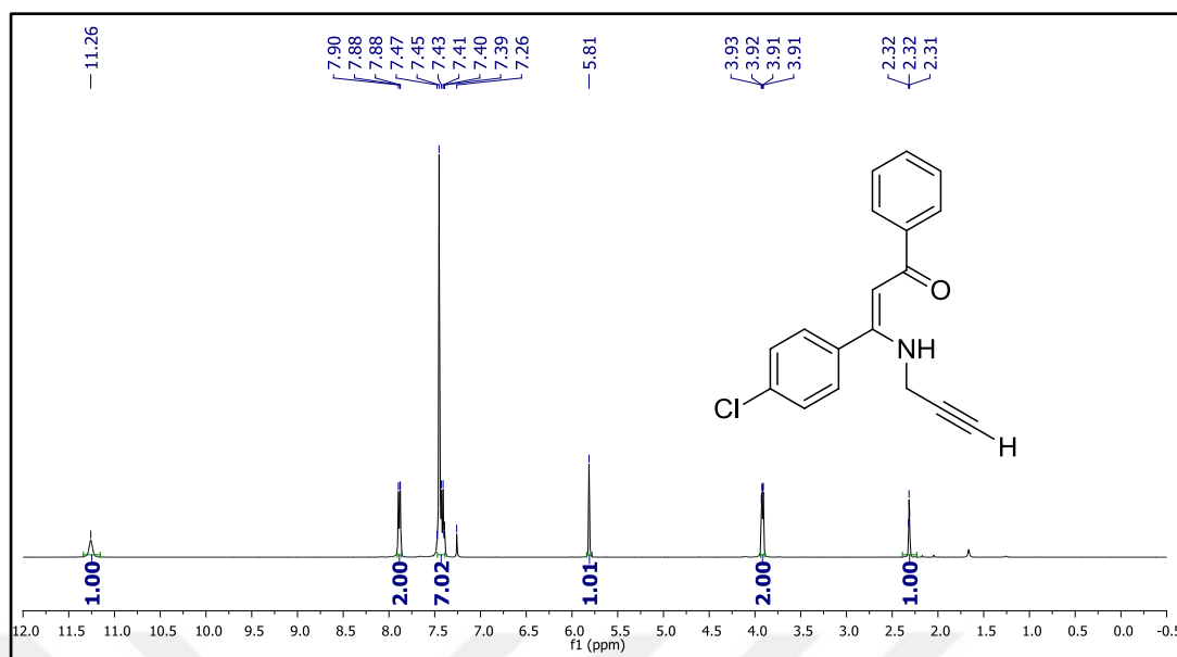
Figure 77. 1 H NMR spectrum of compound 26j.
