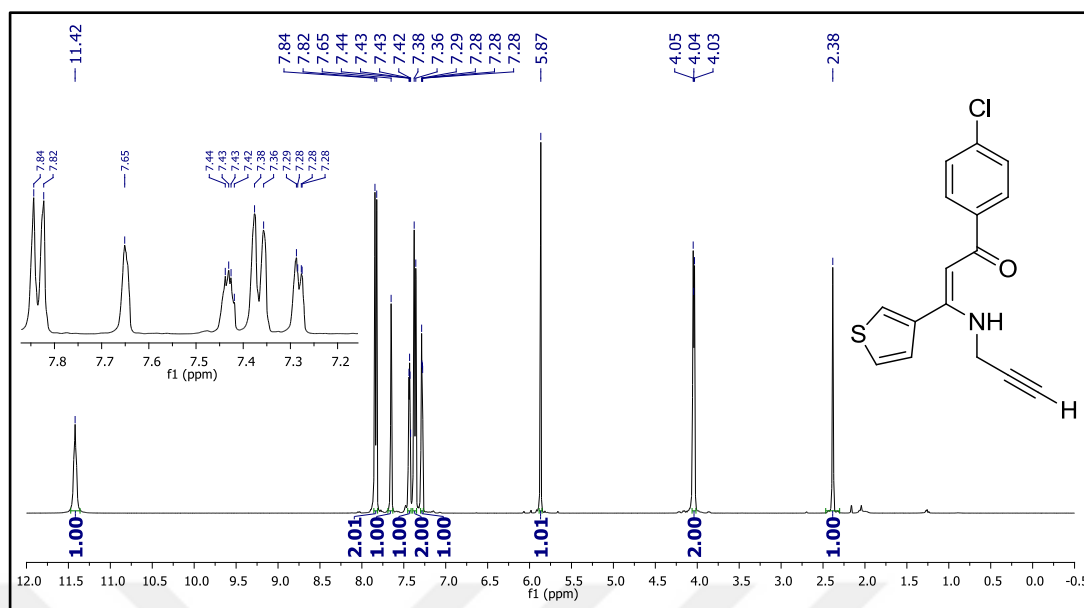
Figure 85. 1 H NMR spectrum of compound 26n.
