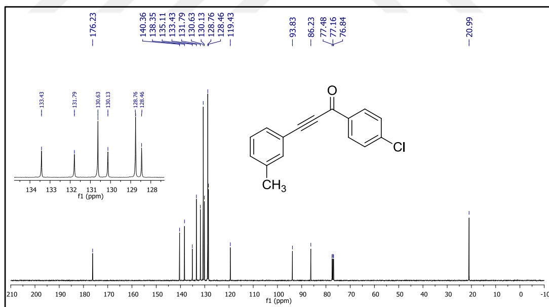
Figure 42. 13 C NMR spectrum of compound 49l.
