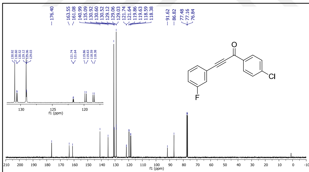
Figure 44. ^{13}\text{C} NMR spectrum of compound 49m .
