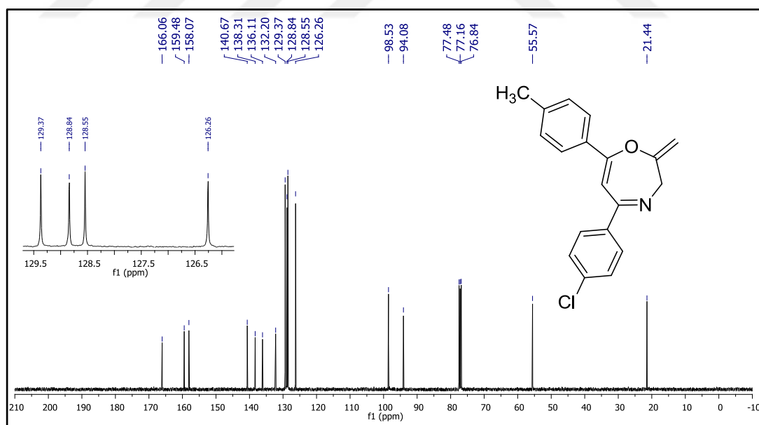
Figure 138. ^{13}\text{C} NMR spectrum of compound 37t .
