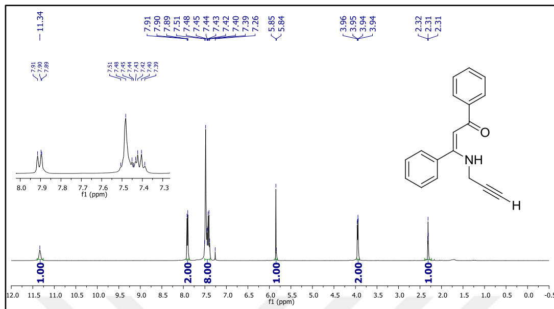
Figure 59. 1 H NMR spectrum of compound 26a.
