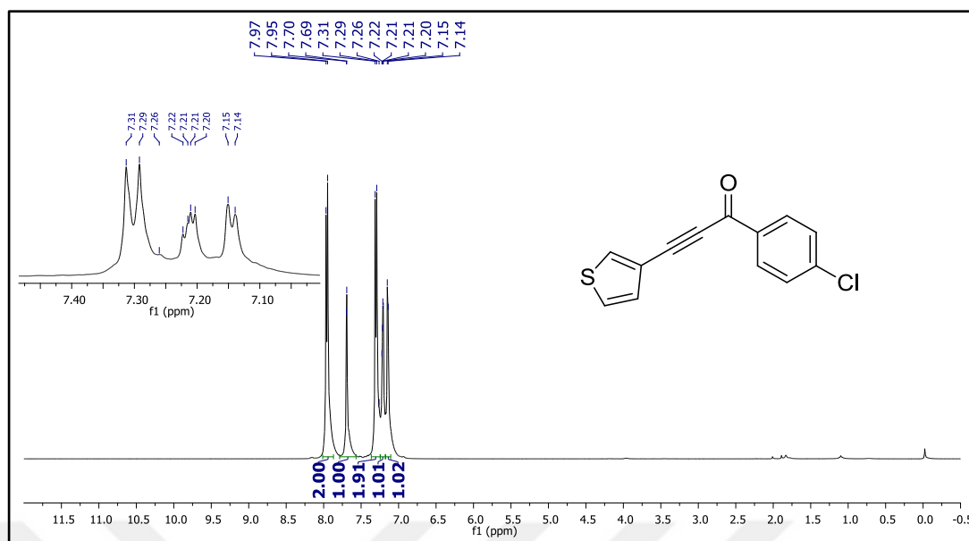
Figure 45. 1 H NMR spectrum of compound 49n .
