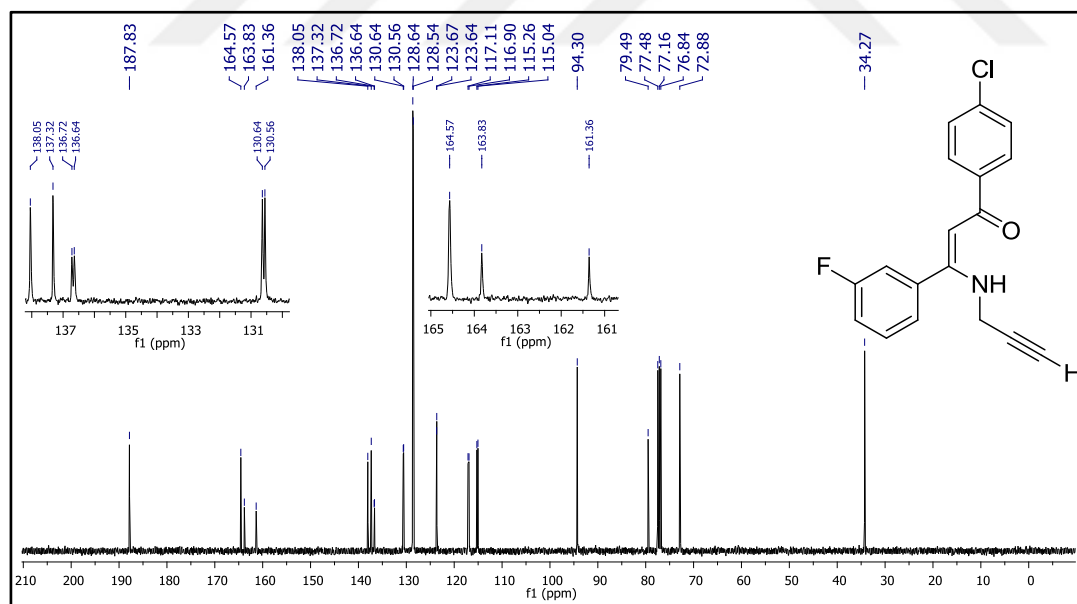
Figure 84. 13 C NMR spectrum of compound 26m.
