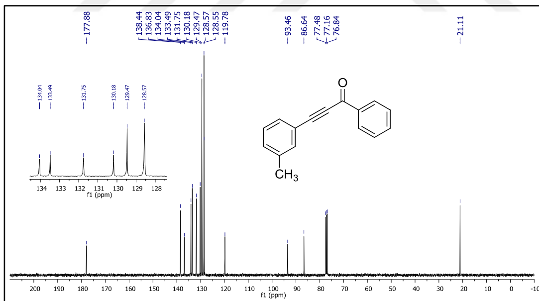
Figure 32. ^{13}\text{C} NMR spectrum of compound 49g.
