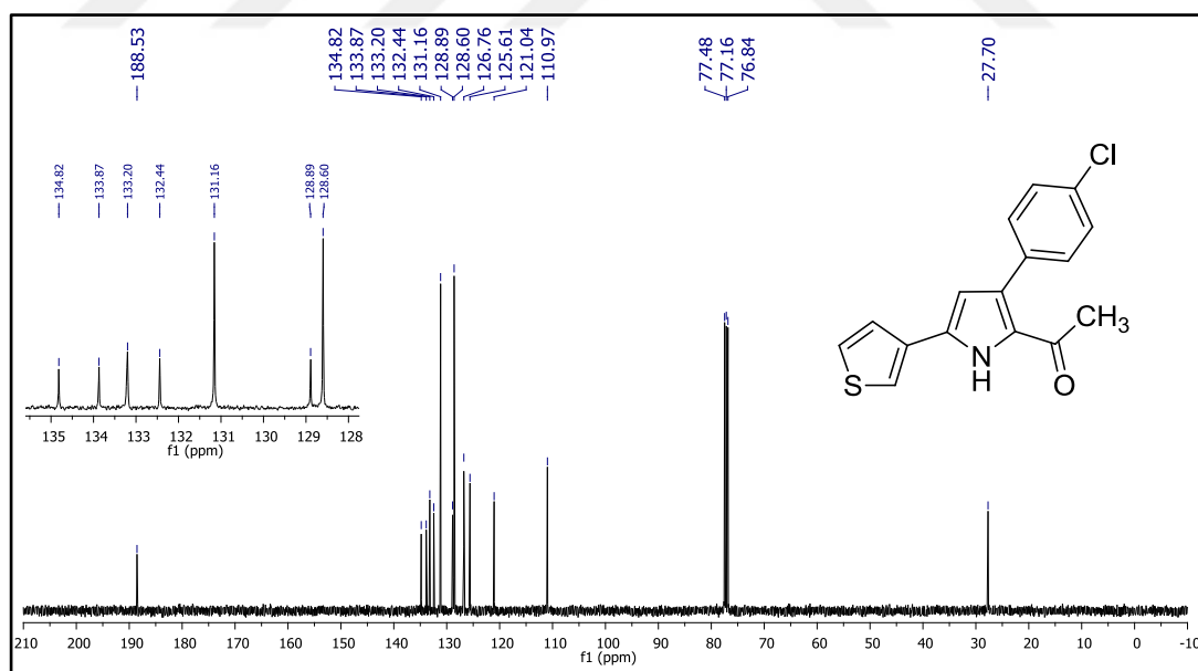
Figure 166. 13 C NMR spectrum of compound 46n.
