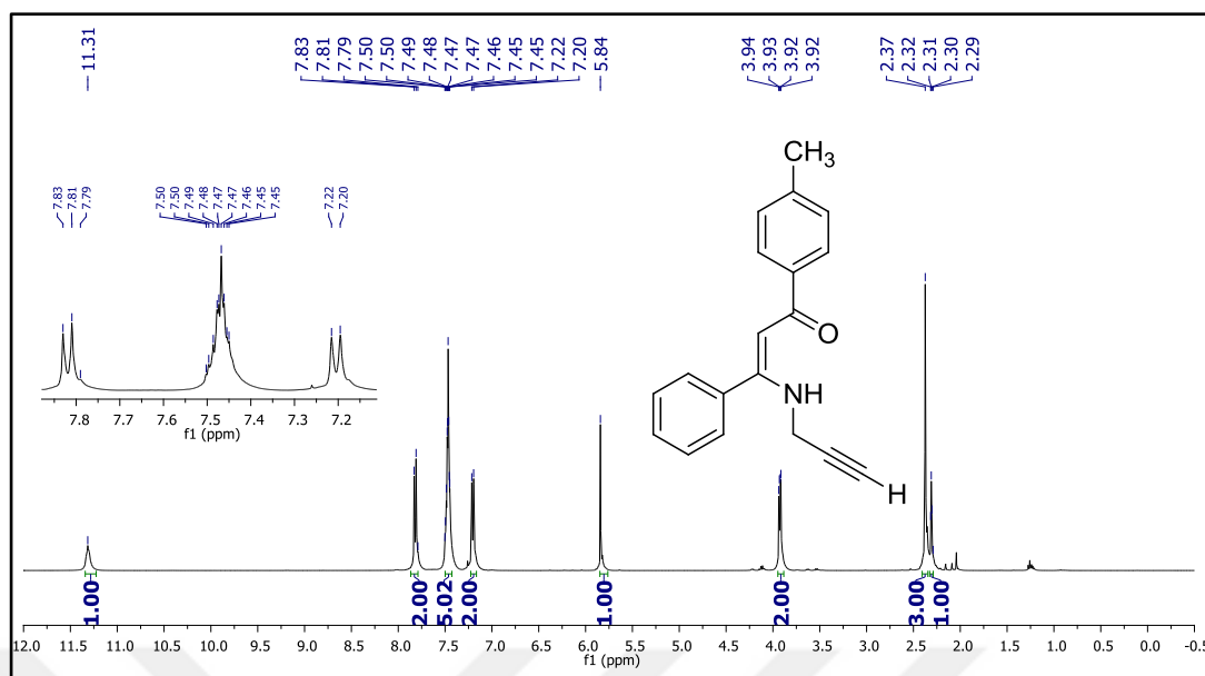
Figure 89. 1 H NMR spectrum of compound 26p.
