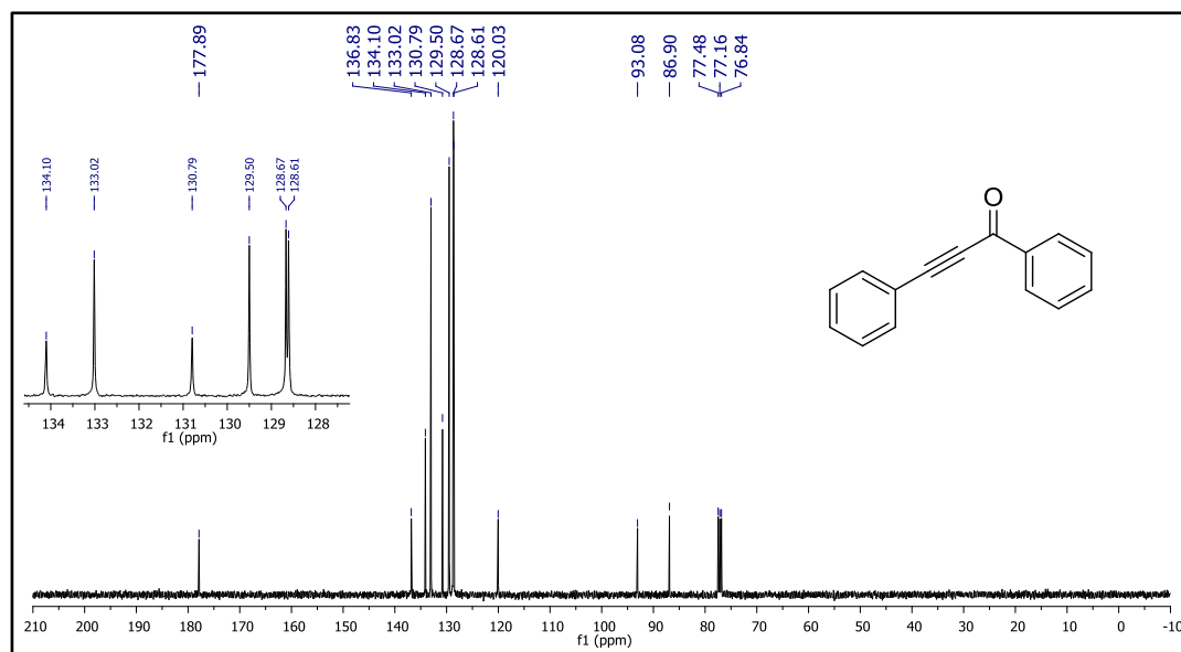
Figure 12. 13 C NMR spectrum of 1,3-diphenylprop-2-yn-1-one (49a).
