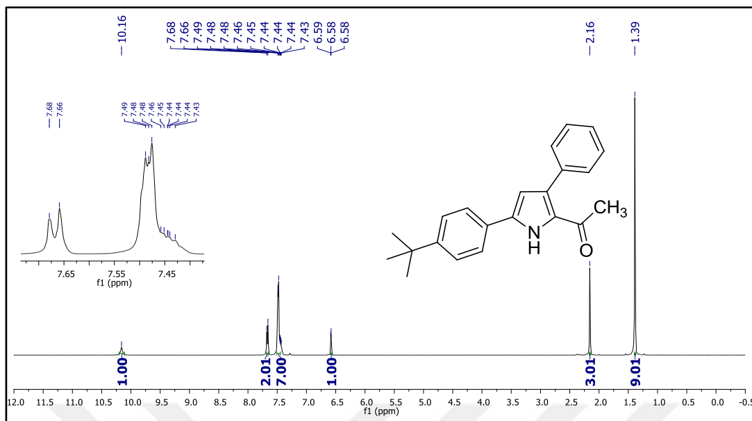
Figure 155. 1 H NMR spectrum of compound 46i .
