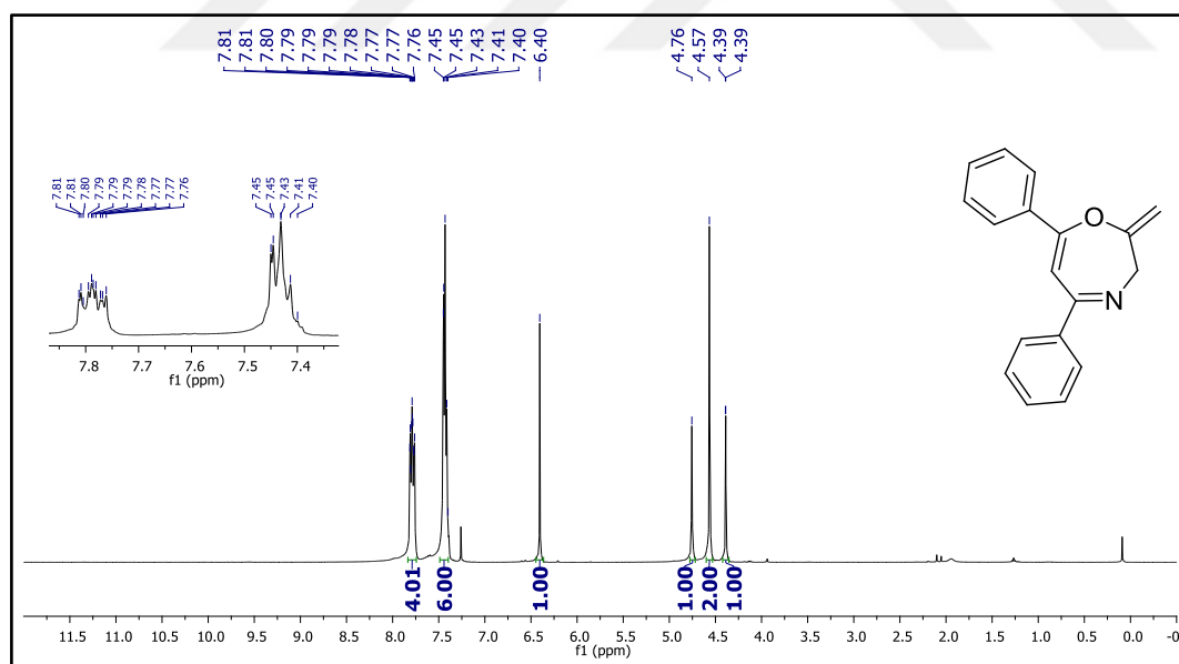
Figure 15. ^1\text{H} NMR spectrum of 2-methylene-5,7-diphenyl-2,3-dihydro-1,4-oxazepine ( 37a ).
