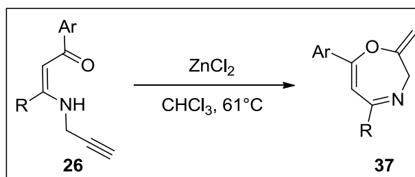
Scheme 24. Synthesis of 1,4-oxazepines 37 .
