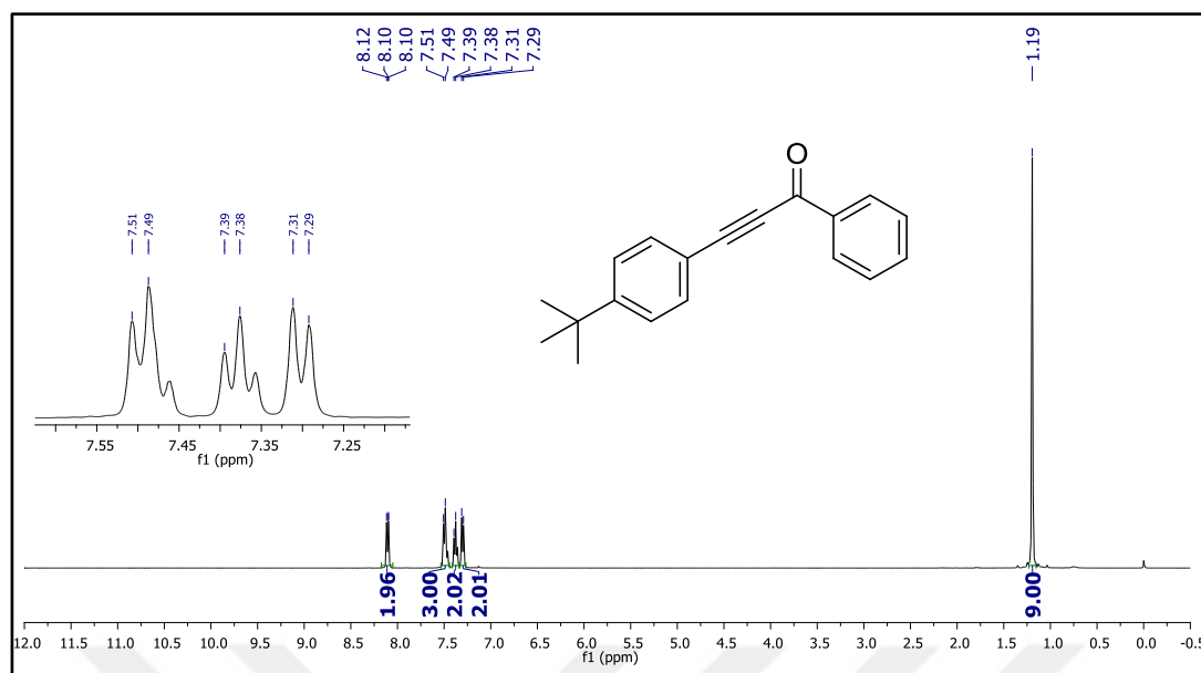
Figure 35. ^1\text{H} NMR spectrum of compound 49i.
