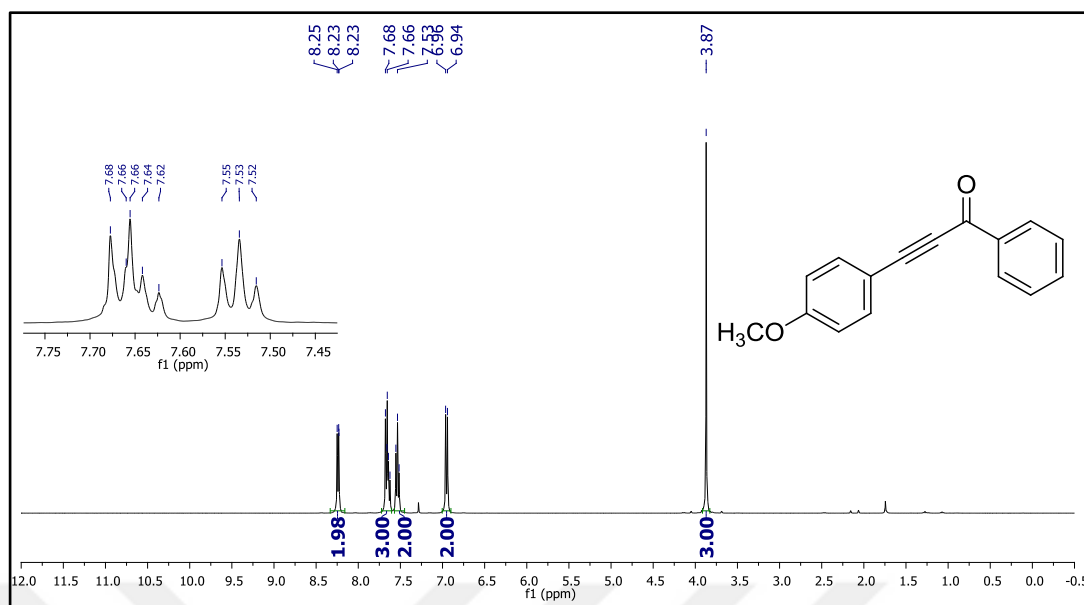
Figure 29. 1 H NMR spectrum of compound 49f.
