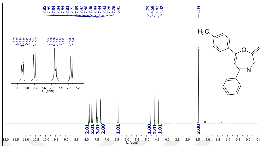
Figure 129. 1 H NMR spectrum of compound 37p.
