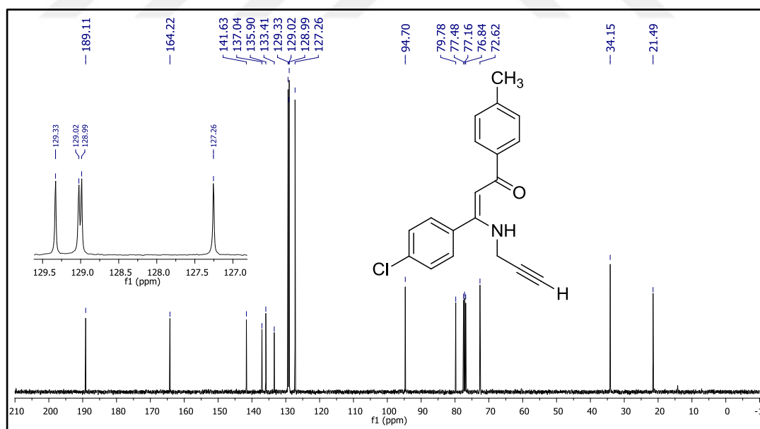
Figure 98. ^{13}\text{C} NMR spectrum of compound 26t.
