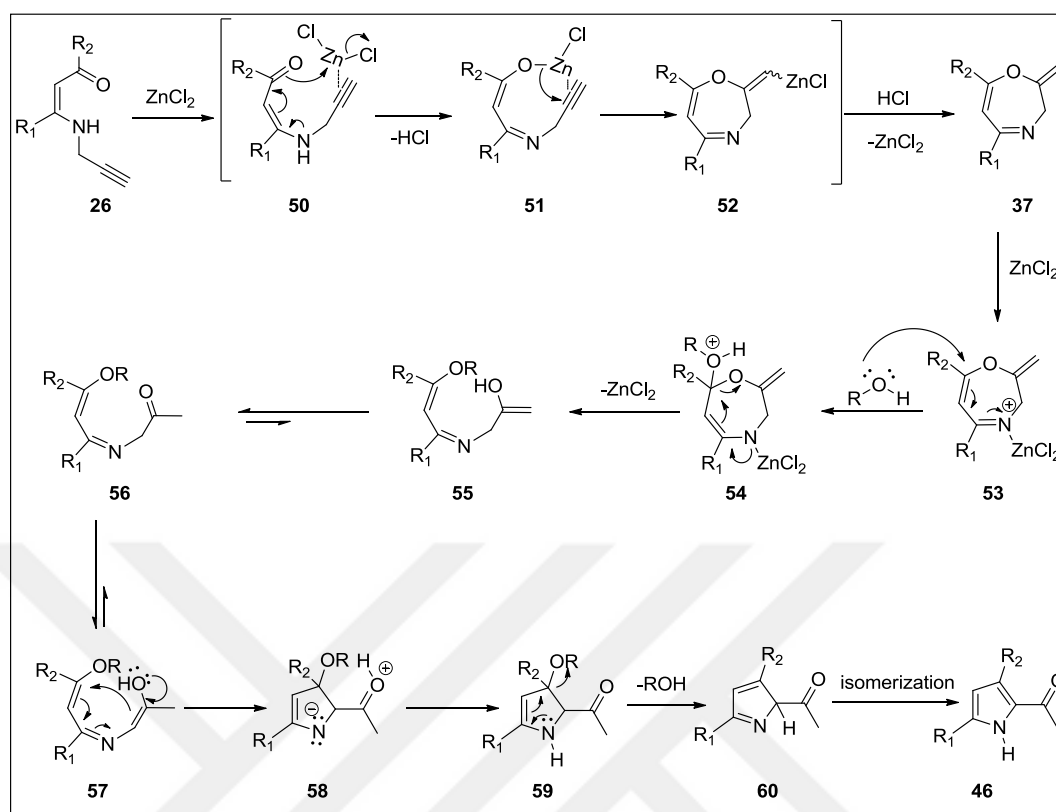
Scheme 26. Proposed mechanism for the desired pyrrole 46 .
