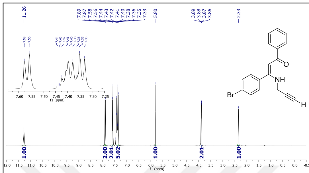
Figure 79. 1 H NMR spectrum of compound 26k.
