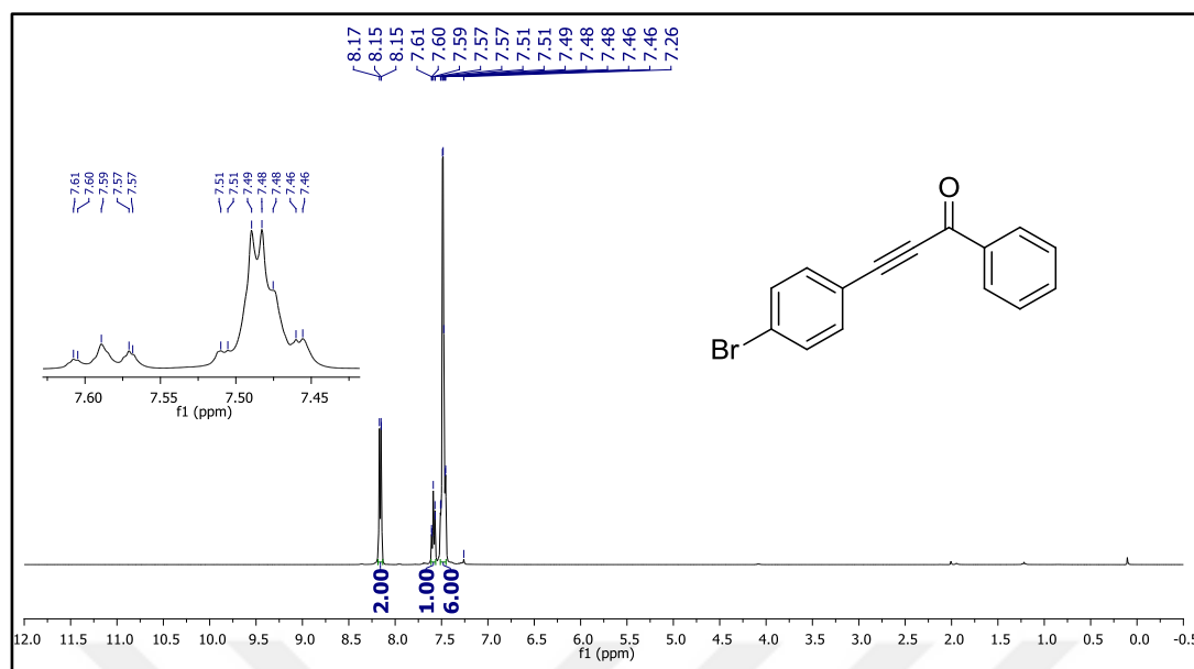
Figure 39. 1 H NMR spectrum of compound 49k .
