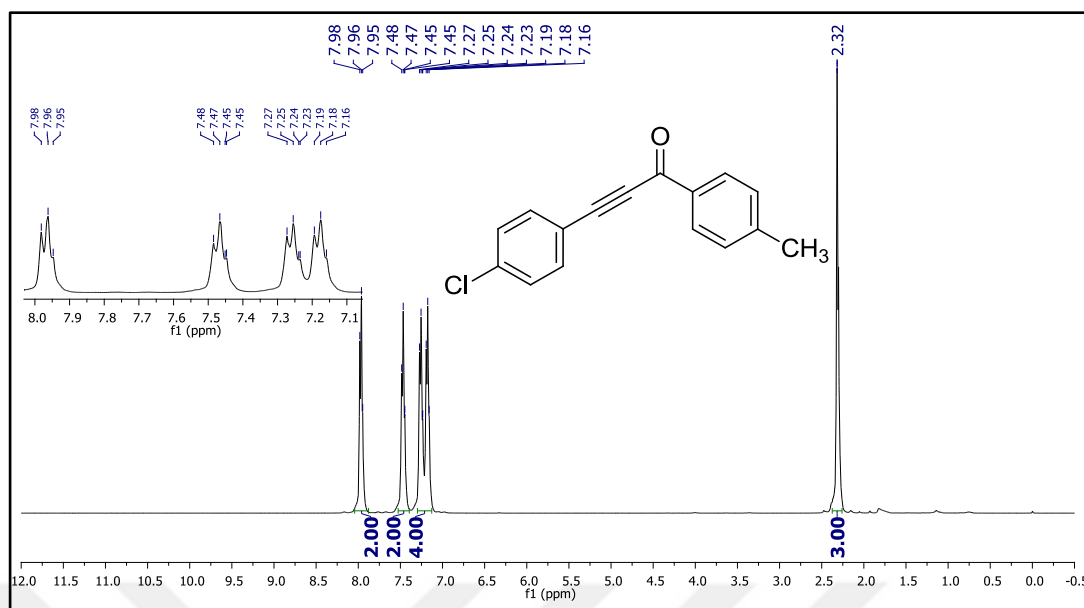
Figure 57. ^1\text{H} NMR spectrum of compound 49t.
