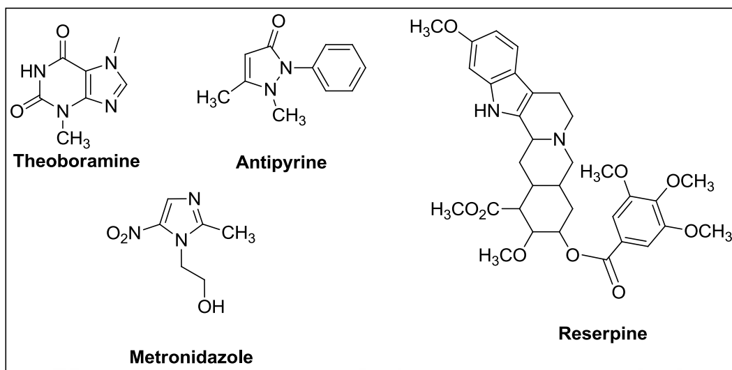
Figure 4. Some examples of natural and synthetic drugs.
