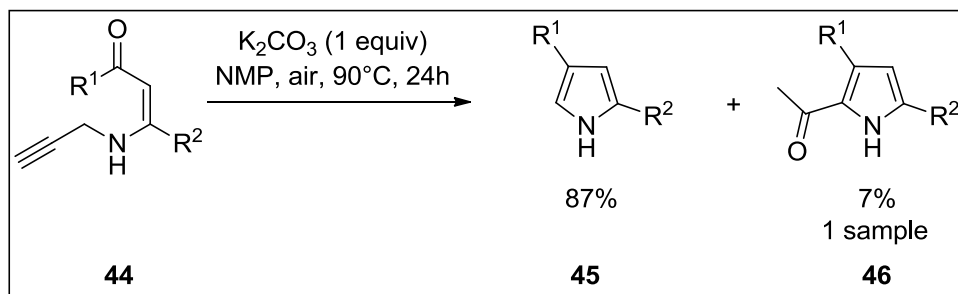
Scheme 16. Synthesis of 2,4-disubstituted pyrroles.
