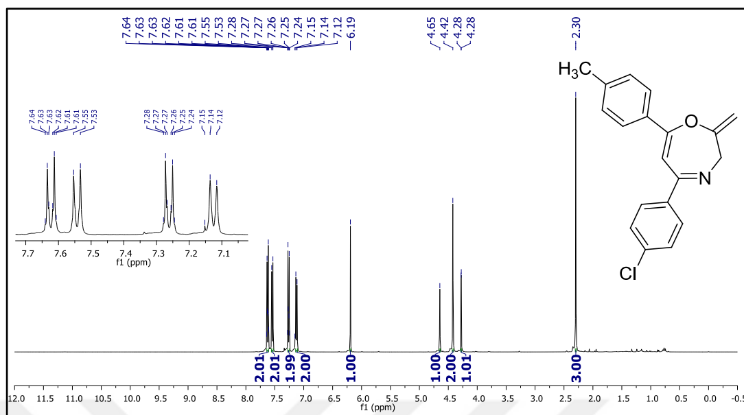
Figure 137. ^1\text{H} NMR spectrum of compound 37t .
