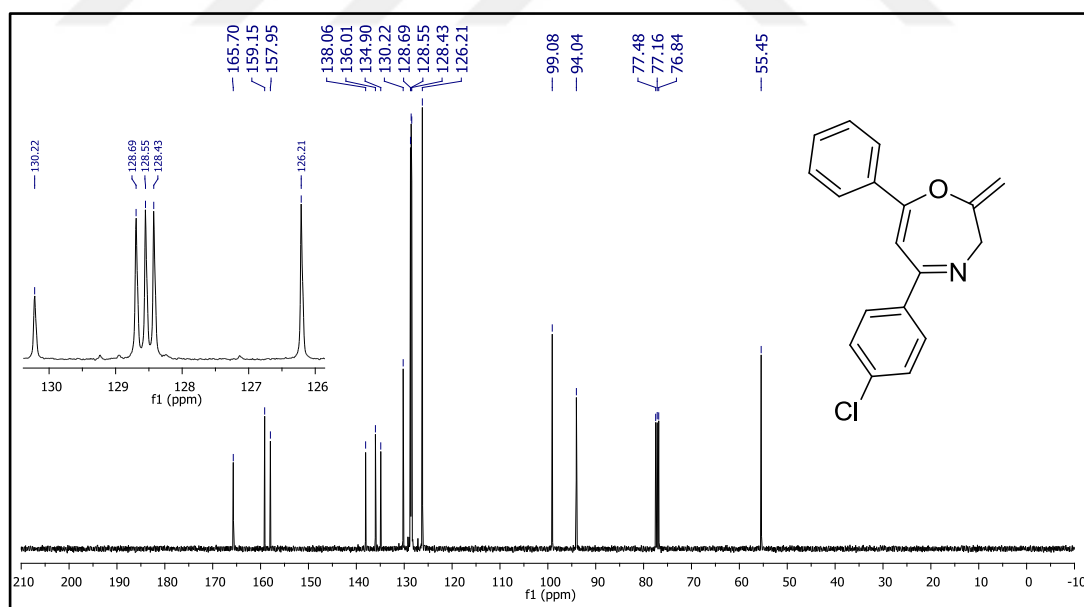
Figure 118. 13 C NMR spectrum of compound 37j.
