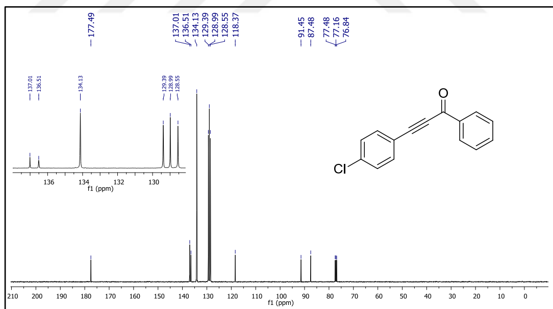
Figure 38. ^{13}\text{C} NMR spectrum of compound 49j.
