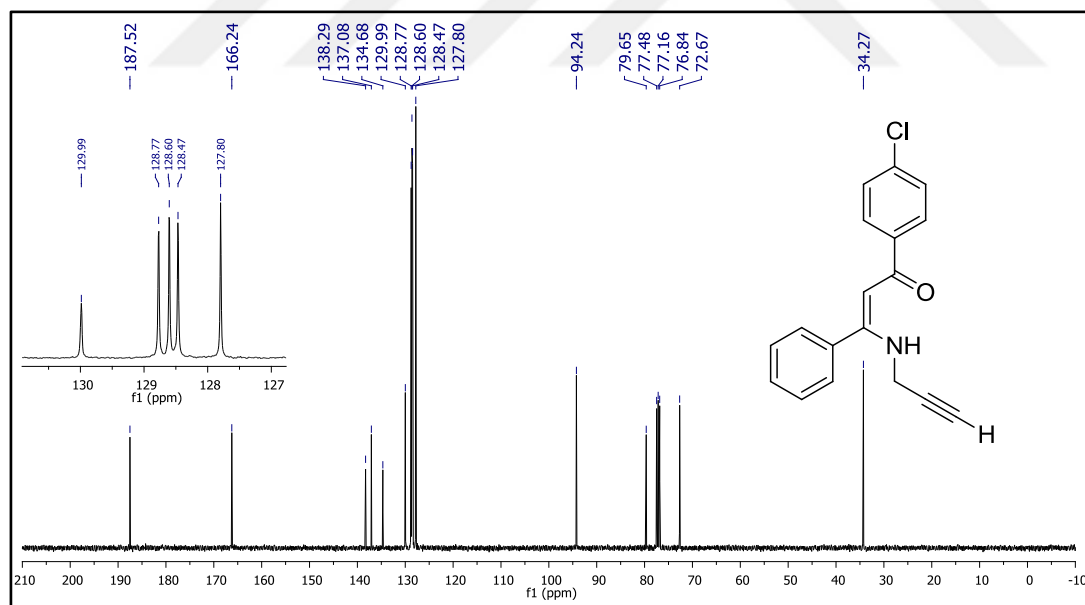
Figure 92. ^{13}\text{C} NMR spectrum of compound 26q.
