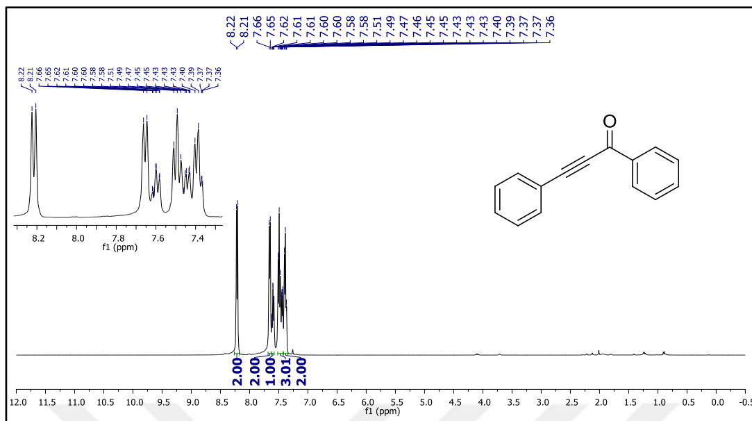
Figure 19. ^1\text{H} NMR spectrum of compound 49a.
