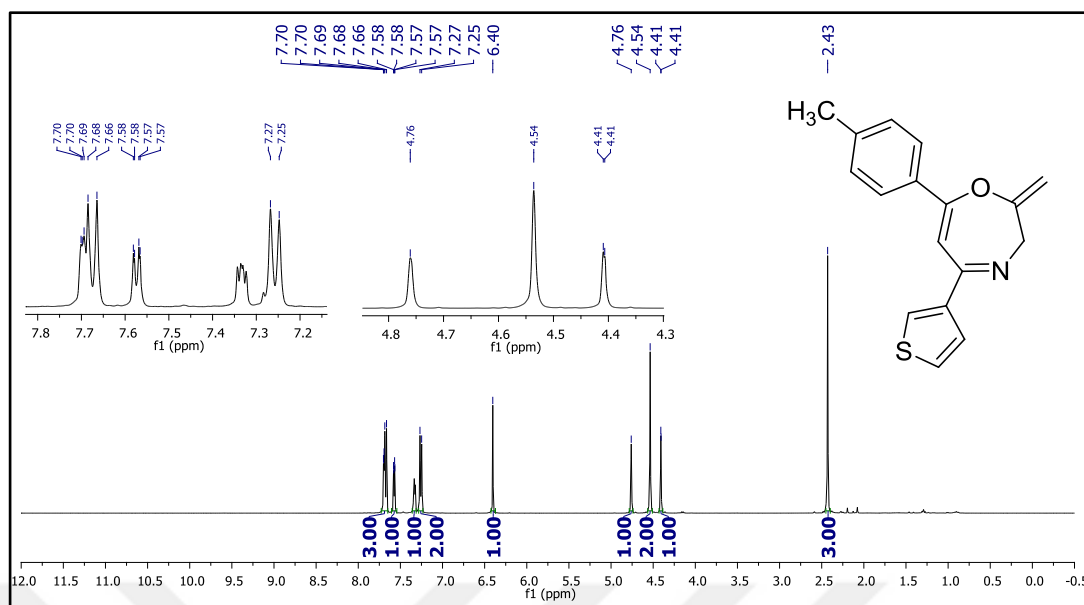
Figure 133. 1 H NMR spectrum of compound 37r.
