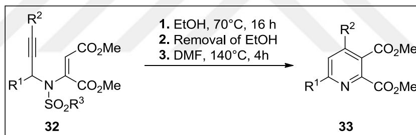
Scheme 11. Synthesis of pyridine derivatives.
