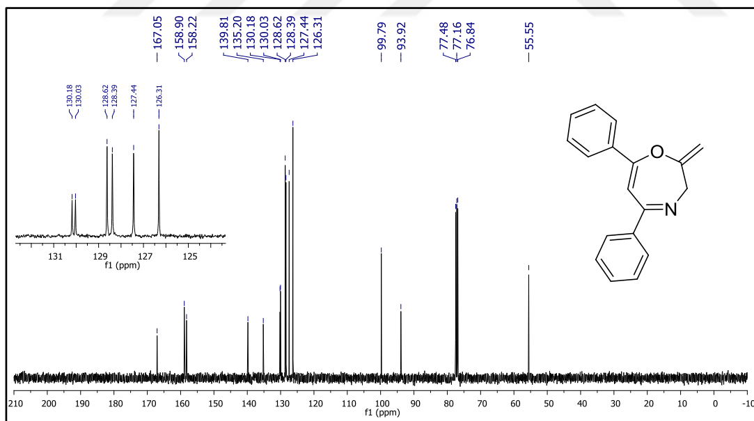
Figure 100. ^{13}\text{C} NMR spectrum of compound 37a.
