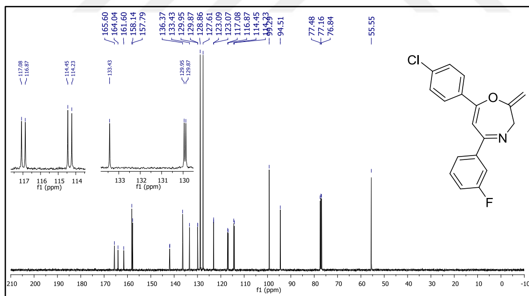
Figure 124. 13 C NMR spectrum of compound 37m.
