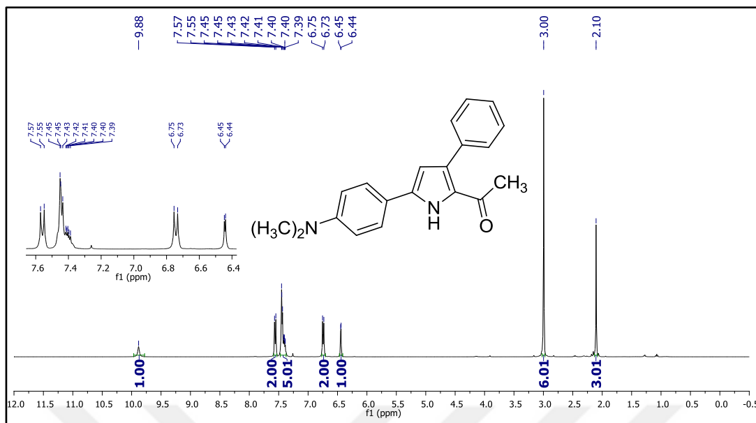
Figure 143. ^1\text{H} NMR spectrum of compound 46c.
