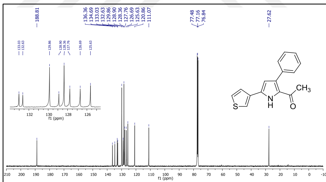
Figure 154. 13 C NMR spectrum of compound 46h.
