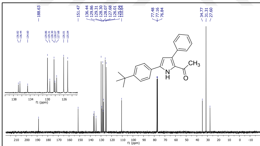
Figure 156. 13 C NMR spectrum of compound 46i .
