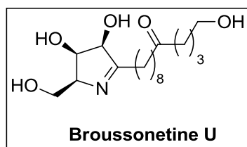
Figure 8. An example of 1-pyrroline containing natural product.
