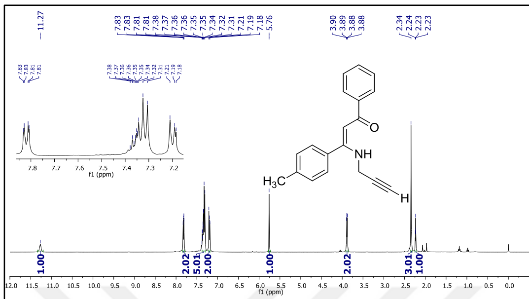
Figure 67. 1 H NMR spectrum of compound 26e.
