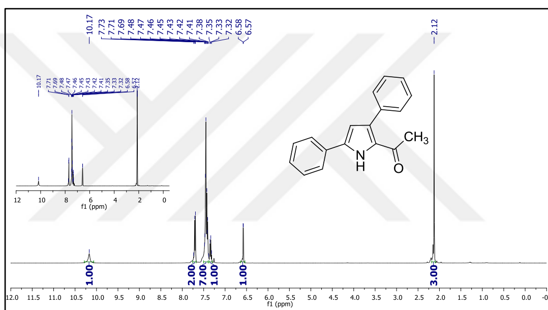
Figure 17. ^1\text{H} NMR spectra of 1-(3,5-diphenyl-1H-pyrrol-2-yl)ethanone (46a).
