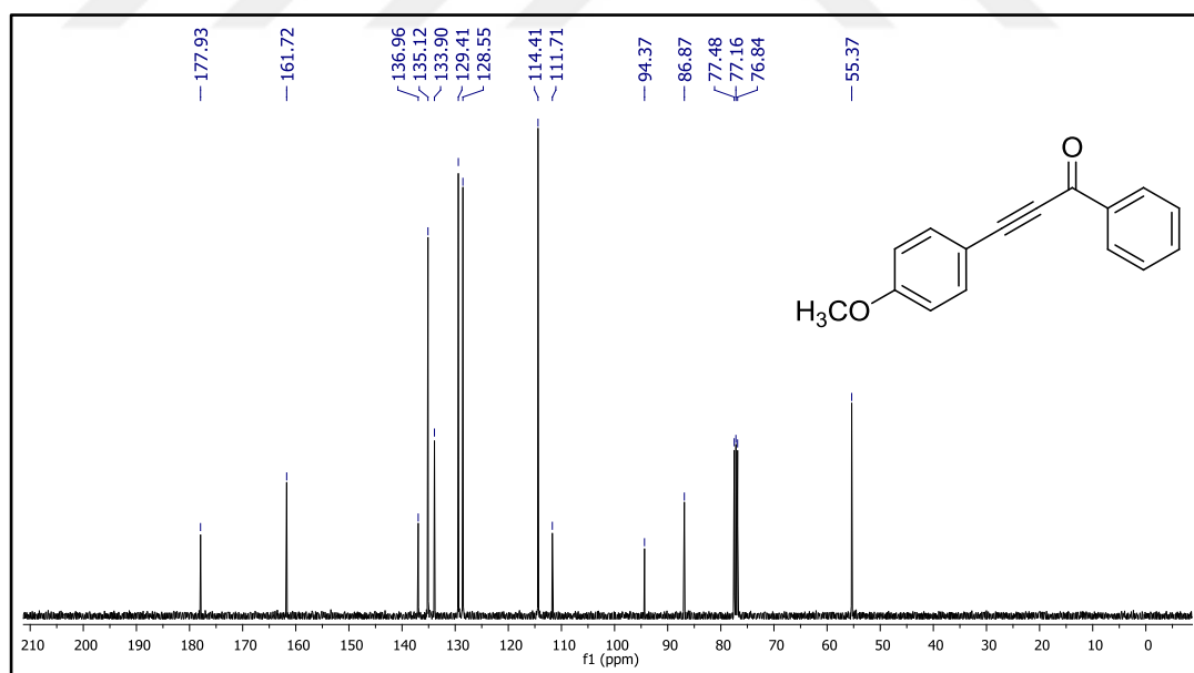
Figure 30. 13 C NMR spectrum of compound 49f.
