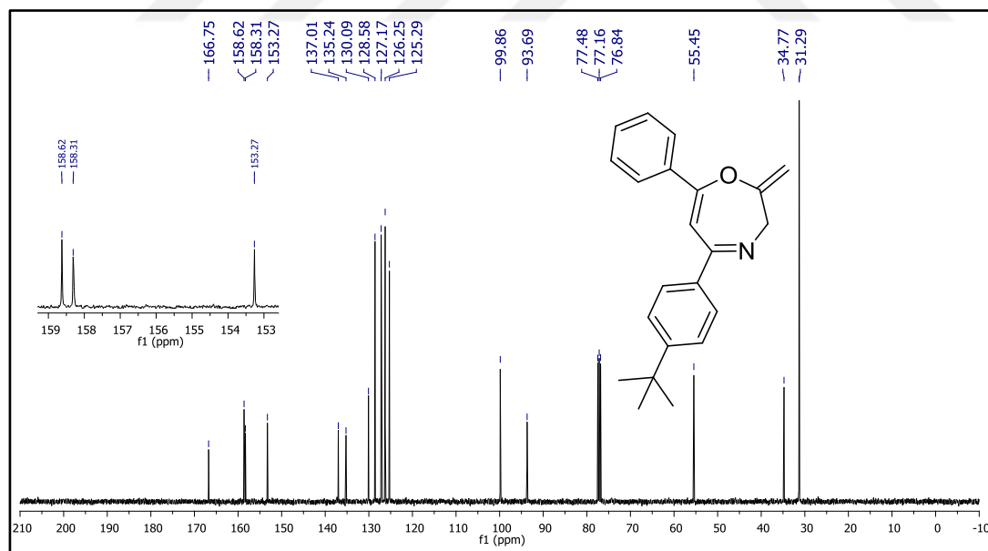
Figure 116. 13 C NMR spectrum of compound 37i.
