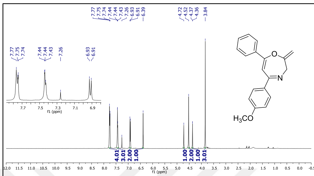
Figure 109. ^1\text{H} NMR spectrum of compound 37f.
