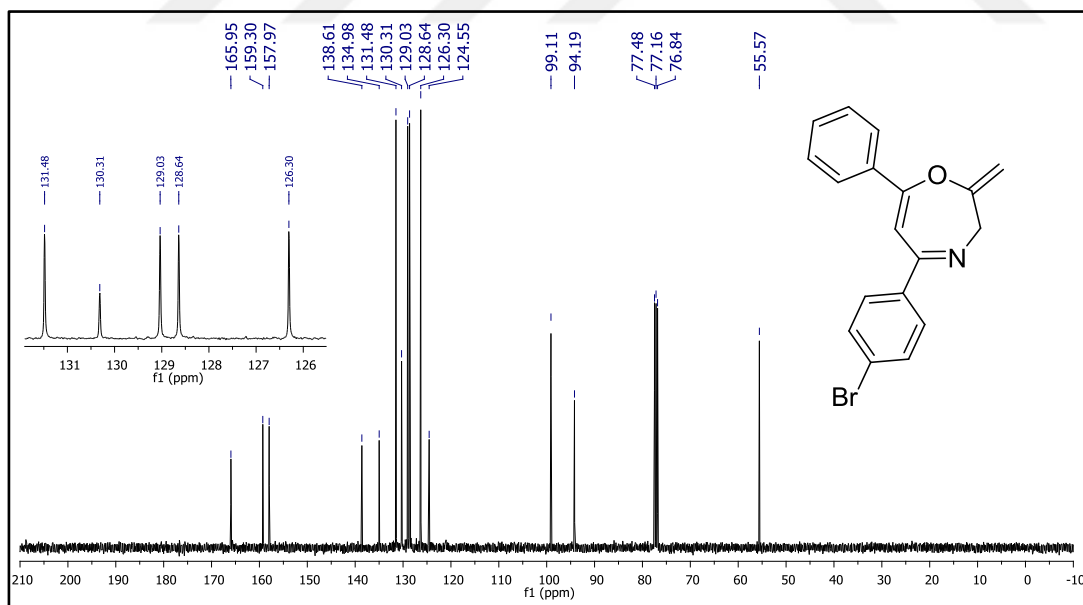
Figure 120. 13 C NMR spectrum of compound 37k.
