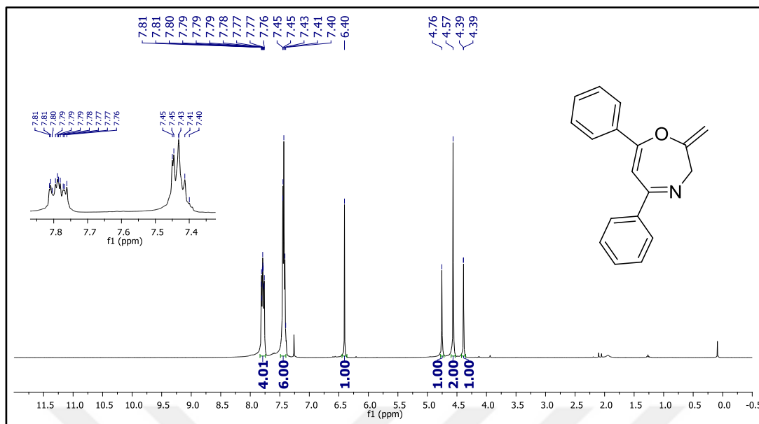
Figure 99. ^1\text{H} NMR spectrum of compound 37a.
