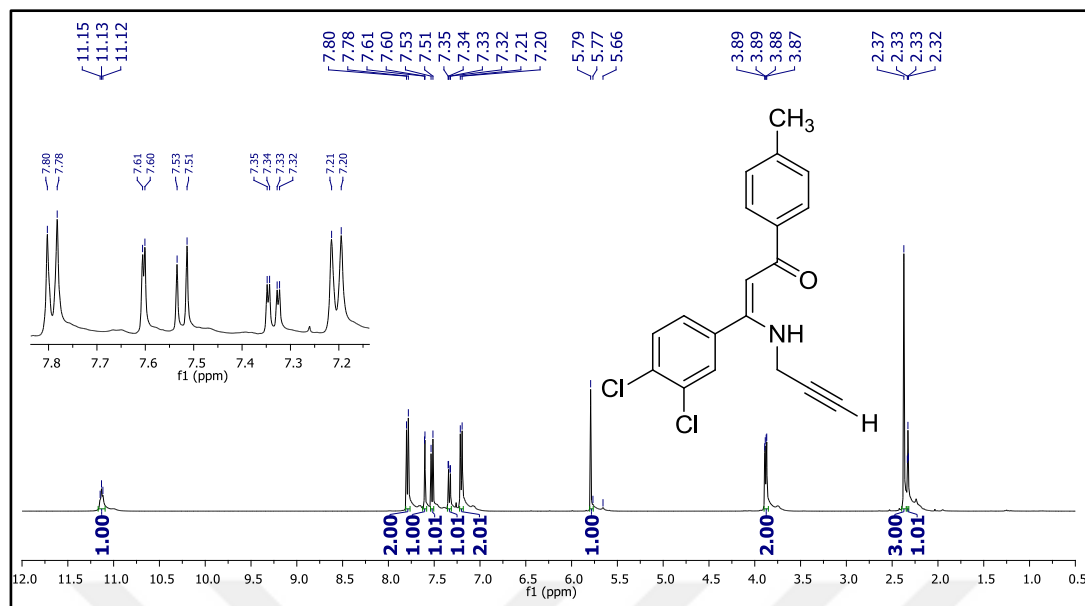
Figure 95. 1 H NMR spectrum of compound 26s.
