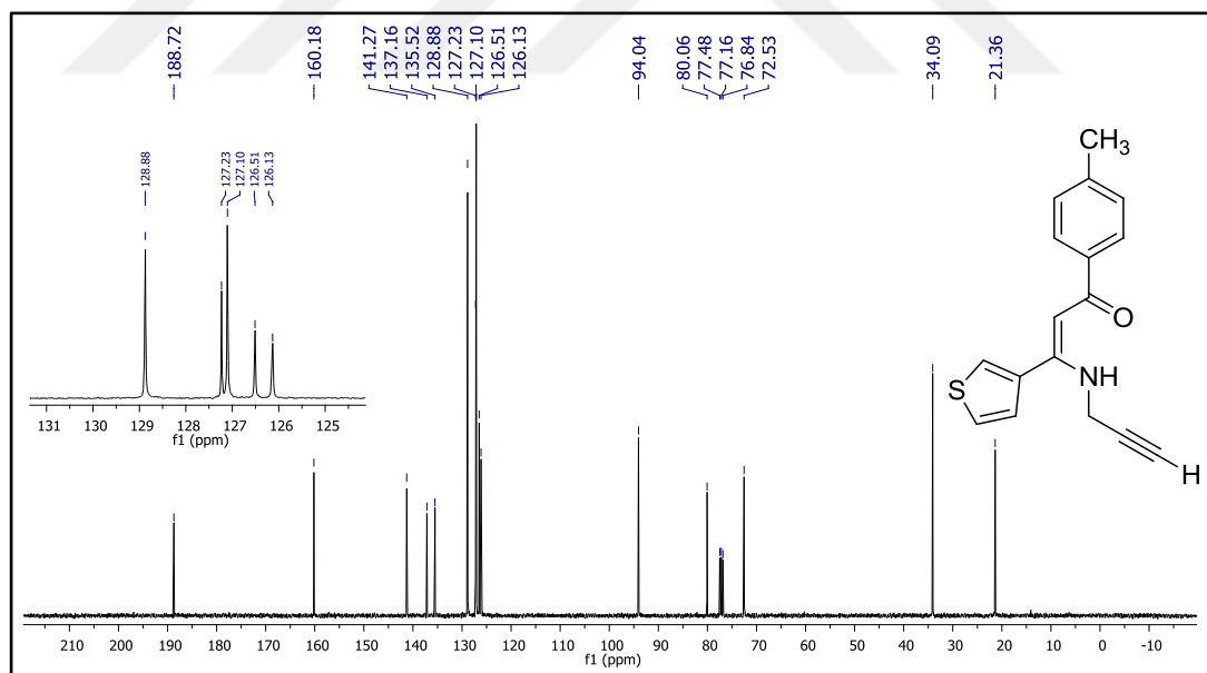
Figure 94. ^{13}\text{C} NMR spectrum of compound 26r.
