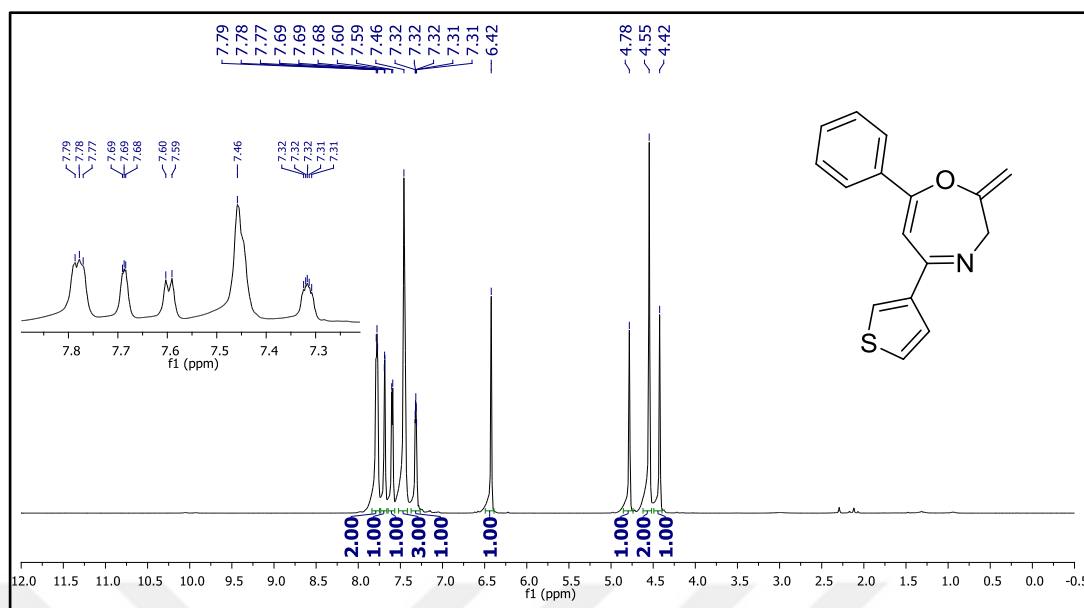
Figure 113. 1 H NMR spectrum of compound 37h.
