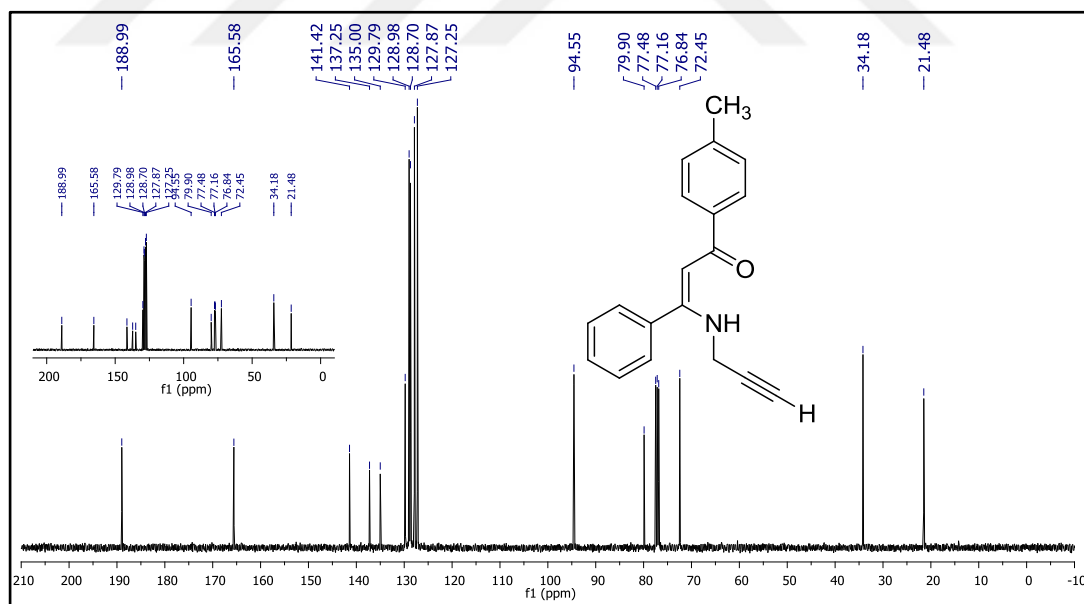
Figure 90. 13 C NMR spectrum of compound 26p.
