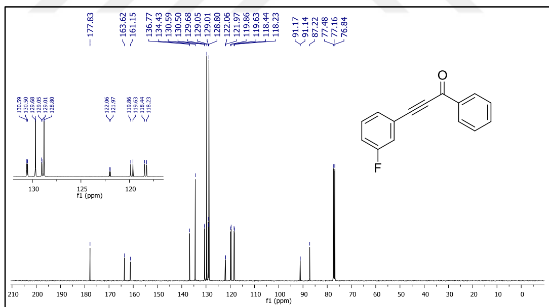
Figure 22. ^{13}\text{C} NMR spectrum of compound 49b.
