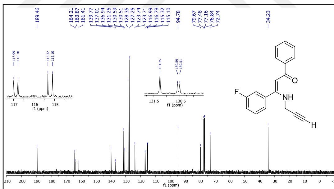
Figure 62. ^{13}\text{C} NMR spectrum of compound 26b.
