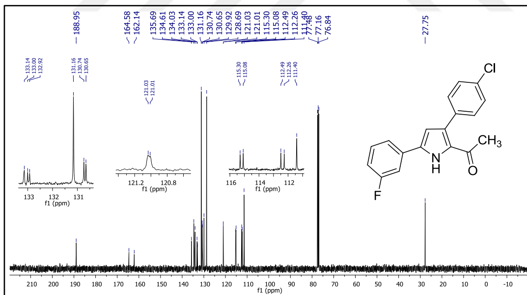
Figure 164. ^{13}\text{C} NMR spectrum of compound 46m.
