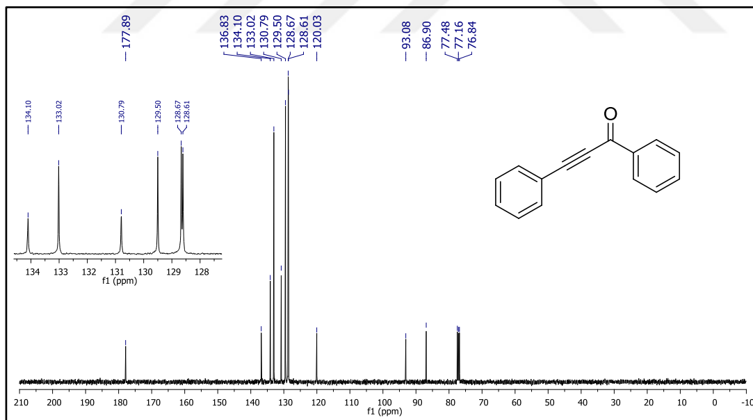
Figure 20. ^{13}\text{C} NMR spectrum of compound 49a.
