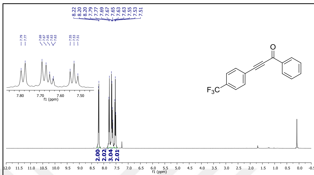
Figure 25. ^1\text{H} NMR spectrum of compound 49d .
