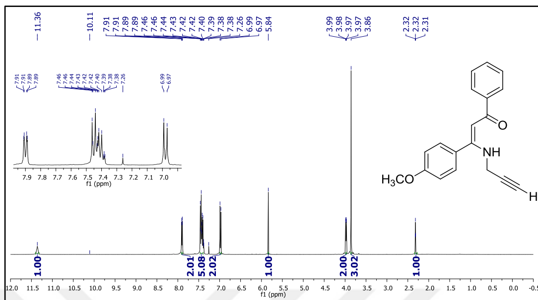
Figure 69. 1 H NMR spectrum of compound 26f.
