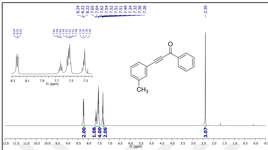
Figure 31. ^1\text{H} NMR spectrum of compound 49g.
