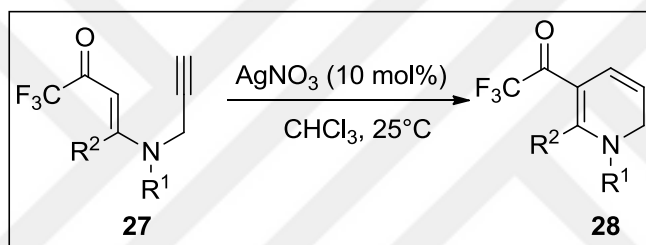
Scheme 9. Ag-catalyzed cyclization of trifluoromethylated N -propargylic \beta -enaminones.
