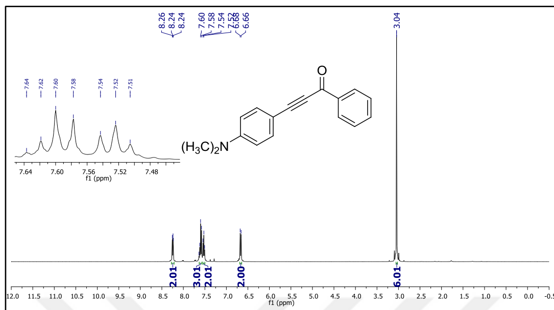
Figure 23. 1 H NMR spectrum of compound 49c.
