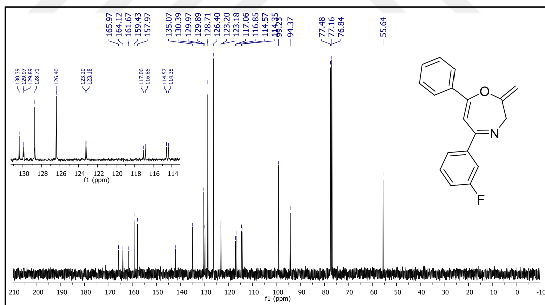
Figure 102. 13 C NMR spectrum of compound 37b.
