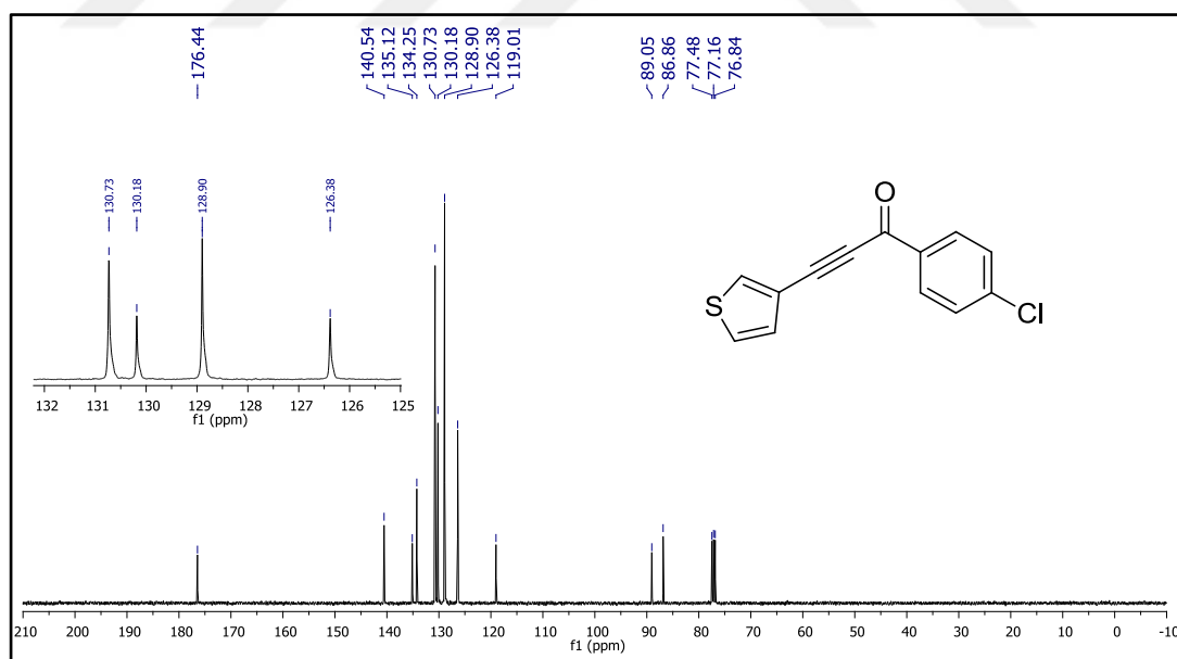
Figure 46. 13 C NMR spectrum of compound 49n .
