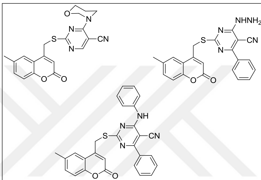
Figure 3. Some examples of coumarin containing anticancer compounds.
