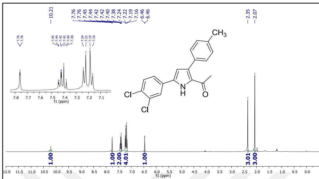
Figure 175. 1 H NMR spectrum of compound 46s.
