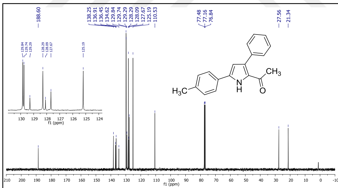
Figure 148. 13 C NMR spectrum of compound 46e.
