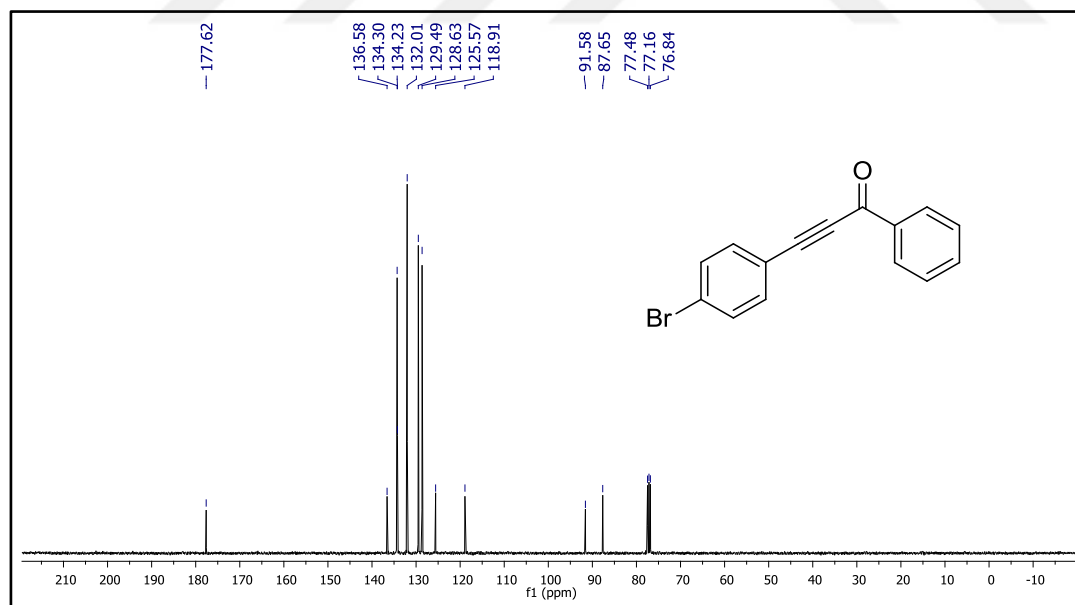
Figure 40. 13 C NMR spectrum of compound 49k .
