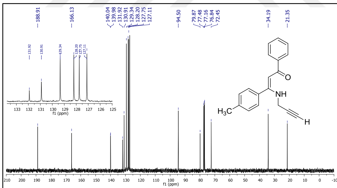
Figure 68. 13 C NMR spectrum of compound 26e.
