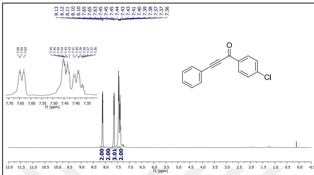
Figure 51. ^1\text{H} NMR spectrum of compound 49q .
