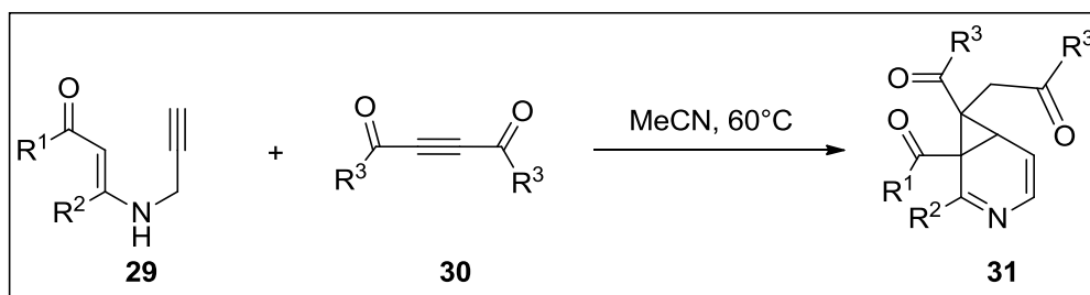
Scheme 10. Synthesis of fused pyridine ring systems.
