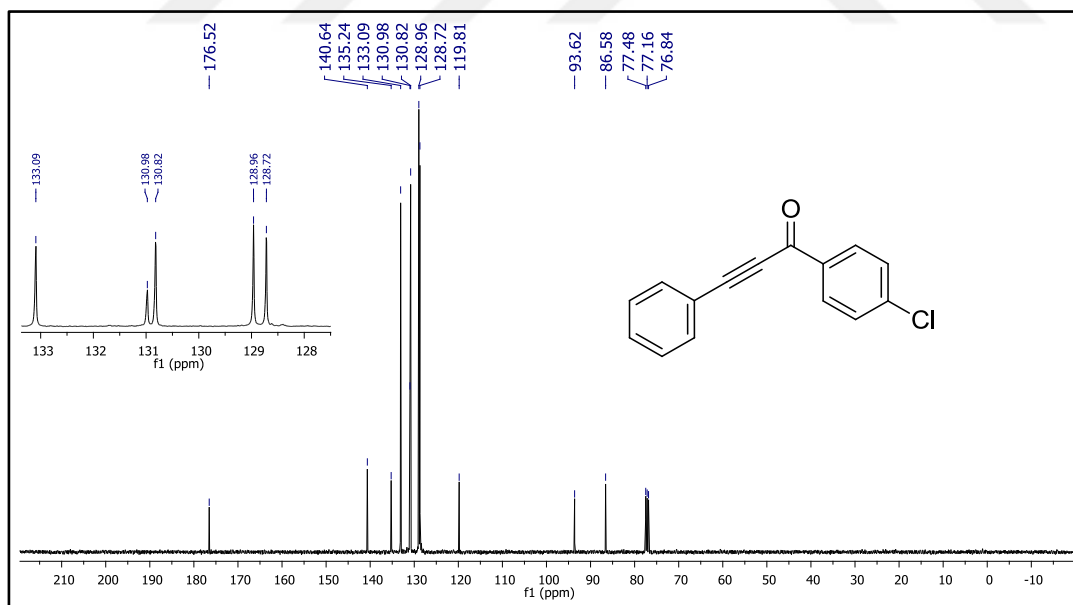
Figure 52. ^{13}\text{C} NMR spectrum of compound 49q .
