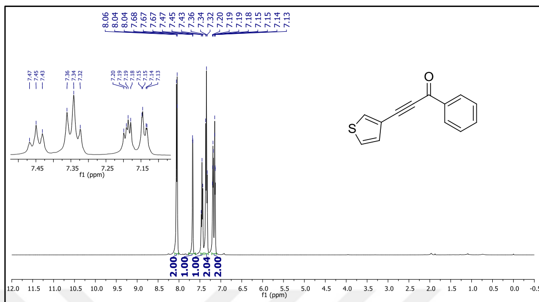
Figure 33. ^1\text{H} NMR spectrum of compound 49h.
