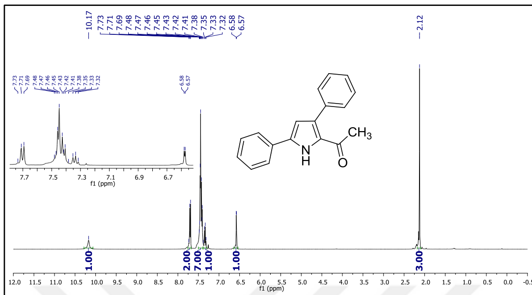
Figure 139. ^1\text{H} NMR spectrum of compound 46a .
