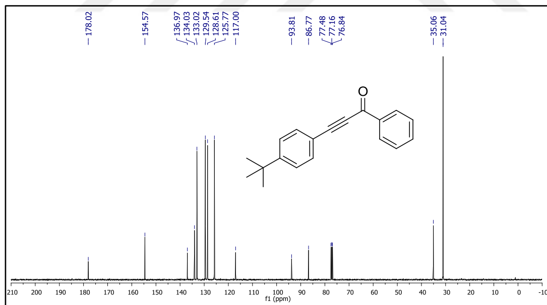
Figure 36. ^{13}\text{C} NMR spectrum of compound 49i.
