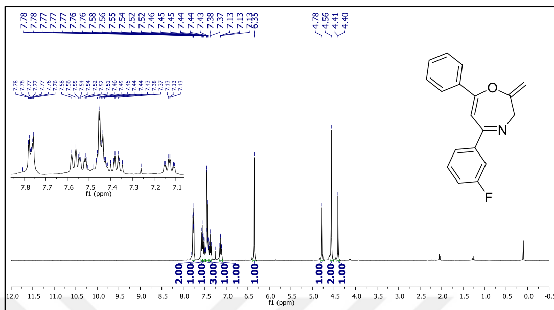
Figure 101. 1 H NMR spectrum of compound 37b.
