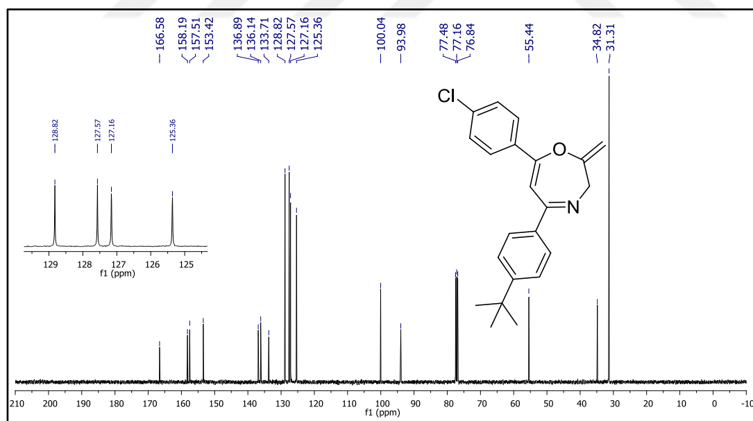
Figure 128. ^{13}\text{C} NMR spectrum of compound 37o.
