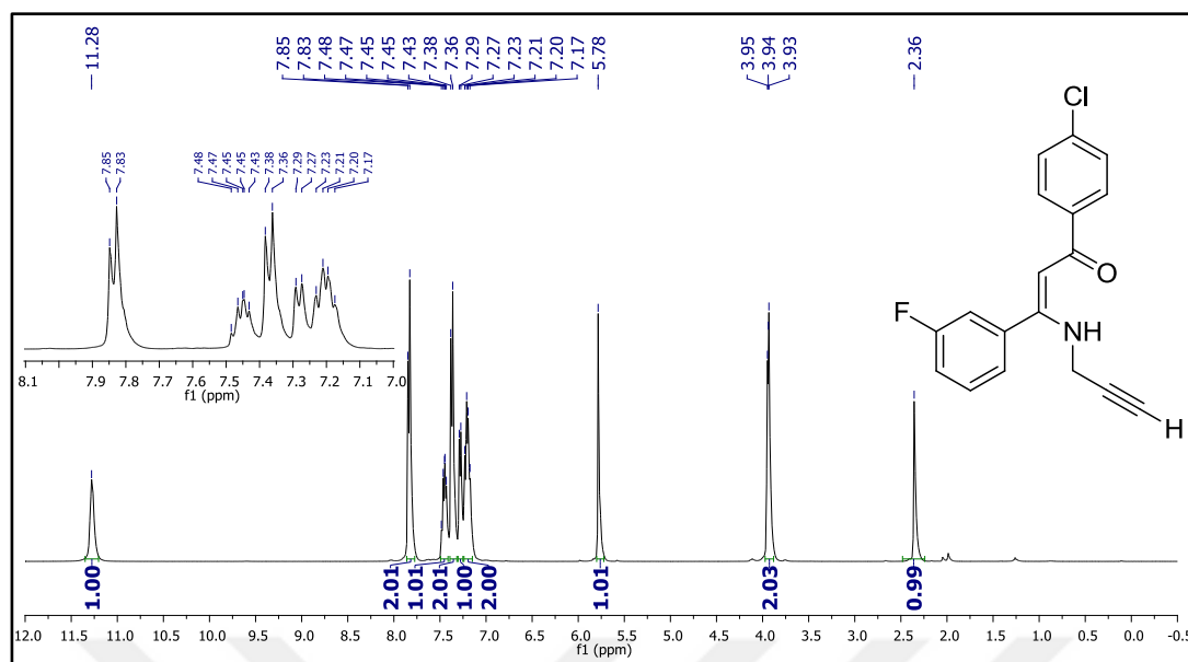
Figure 83. 1 H NMR spectrum of compound 26m.
