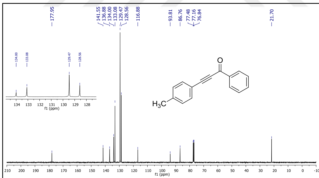
Figure 28. 13 C NMR spectrum of compound 49e.
