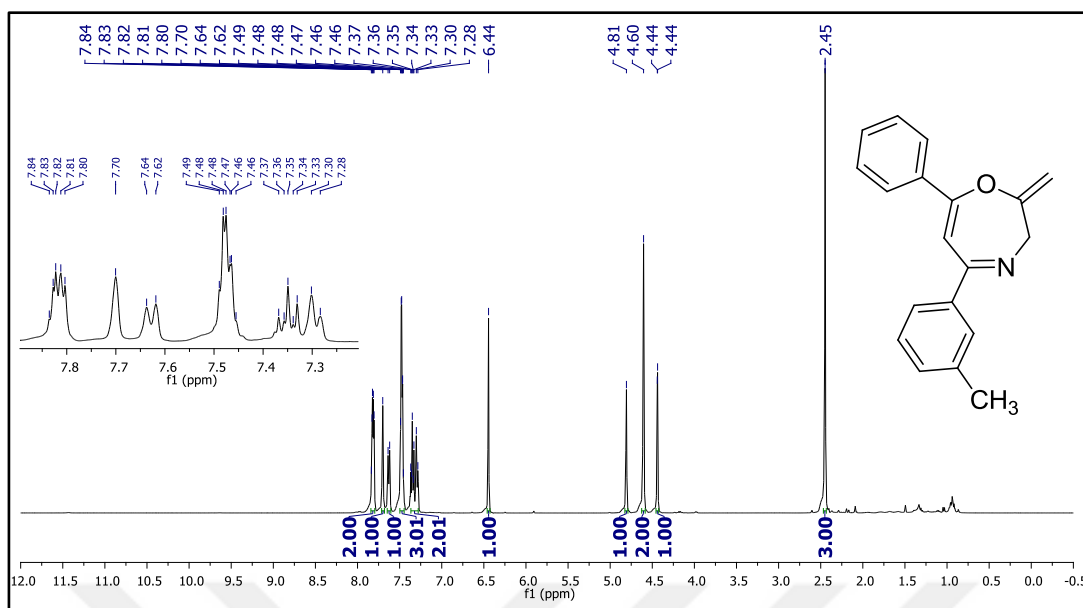
Figure 111. 1 H NMR spectrum of compound 37g.
