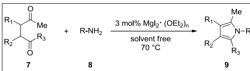
Scheme 3. Synthesis of N -substituted pyrrole derivatives.
