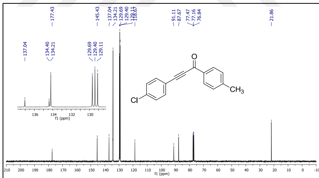
Figure 58. ^{13}\text{C} NMR spectrum of compound 49t.
