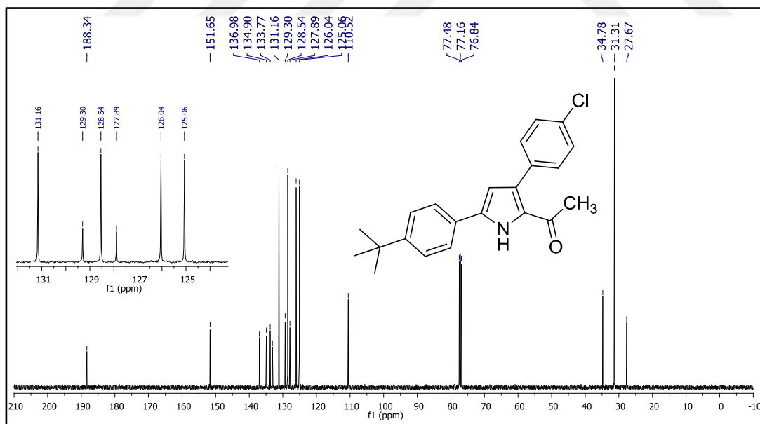
Figure 168. 13 C NMR spectrum of compound 46o .
