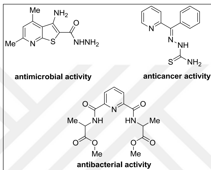
Figure 6. Pyridine containing molecules found in various drugs.
