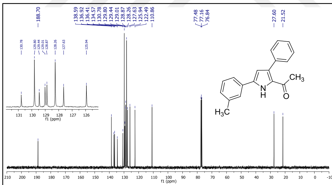
Figure 152. ^{13}\text{C} NMR spectrum of compound 46g .
