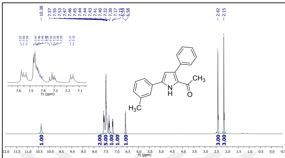
Figure 151. ^1\text{H} NMR spectrum of compound 46g .
