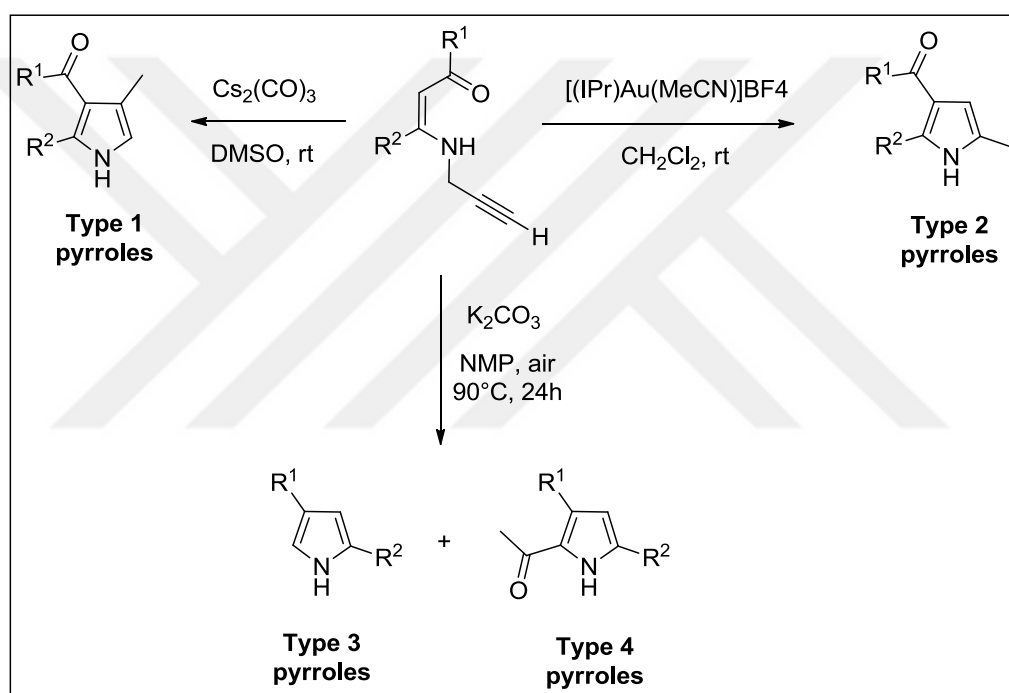
Scheme 17. Synthesis of types of pyrroles from N -propargylic \beta -enaminones.
