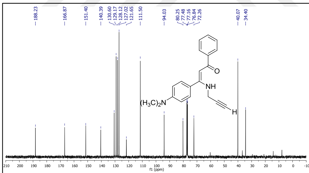
Figure 64. 13 C NMR spectrum of compound 26c.
