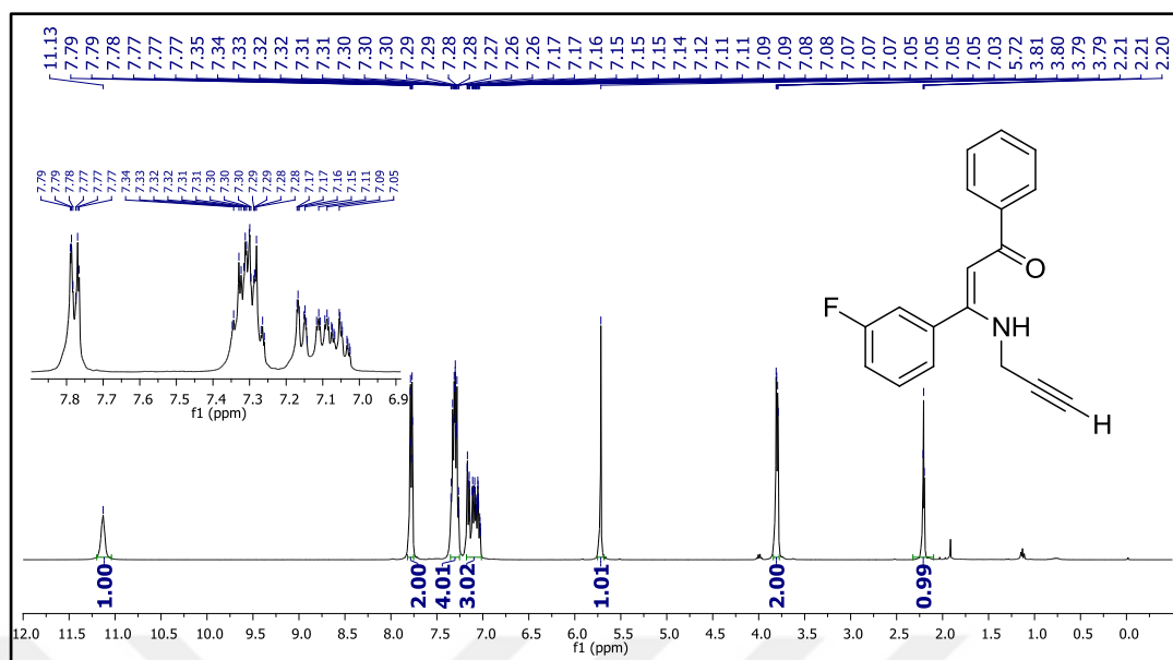
Figure 61. ^1\text{H} NMR spectrum of compound 26b.
