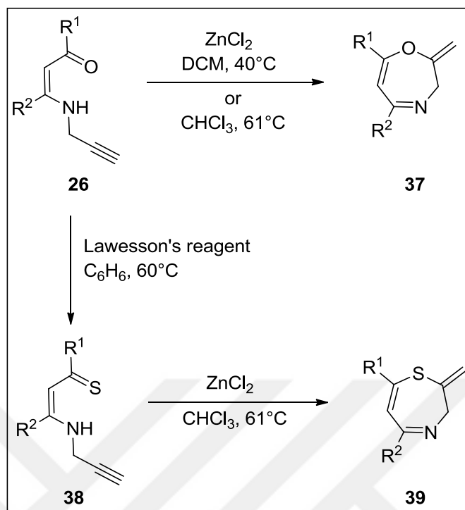
Scheme 13. Synthesis of 1,4-oxazepine and 1,4-thiazepine derivatives.
