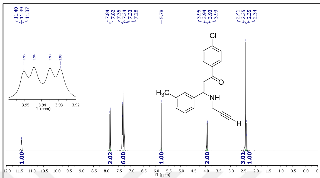
Figure 81. ^1\text{H} NMR spectrum of compound 26l.
