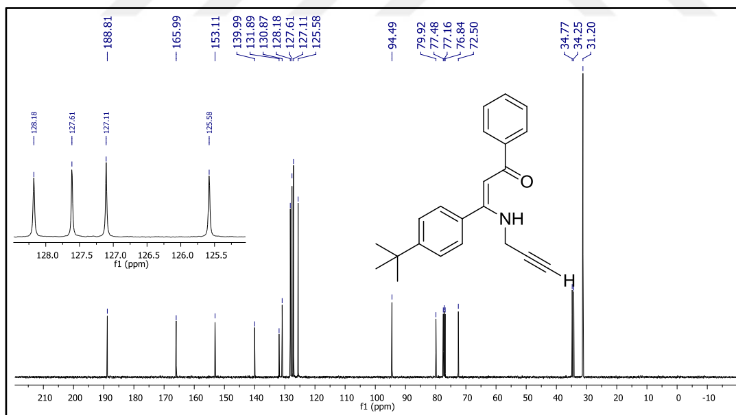
Figure 76. ^{13}\text{C} NMR spectrum of compound 26i.
