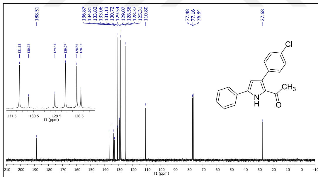
Figure 172. 13 C NMR spectrum of compound 46q .
