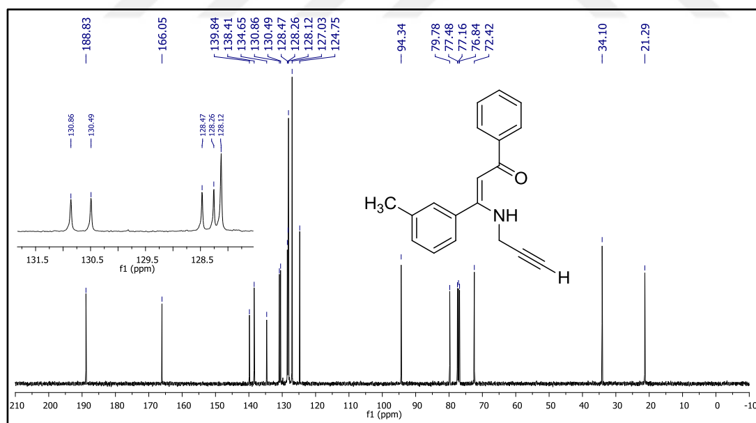
Figure 72. ^{13}\text{C} NMR spectrum of compound 26g .
