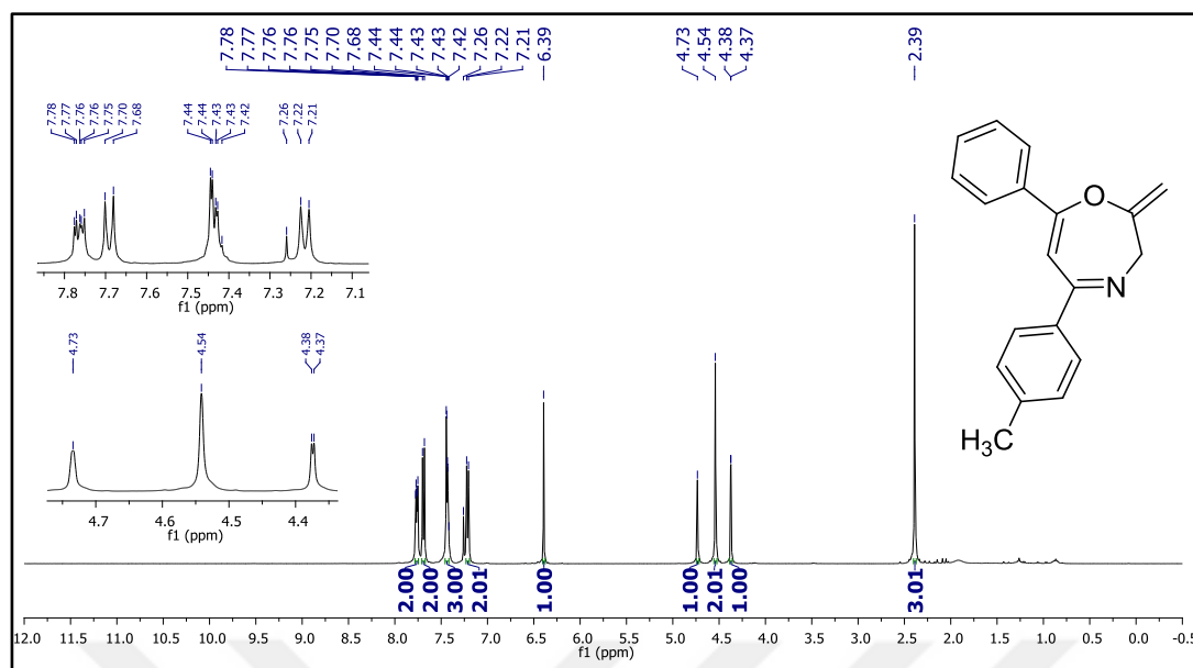
Figure 107. 1 H NMR spectrum of compound 37e.
