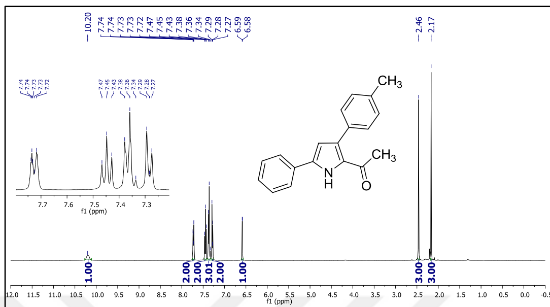
Figure 169. 1 H NMR spectrum of compound 46p.
