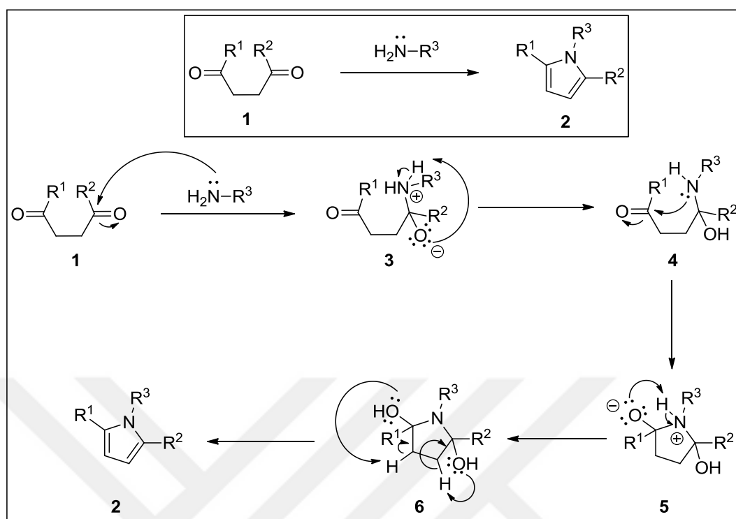
Scheme 2. Mechanism of Paal Knorr pyrrole synthesis.
