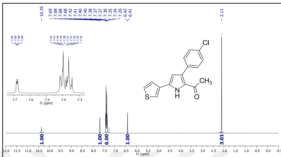
Figure 165. 1 H NMR spectrum of compound 46n.
