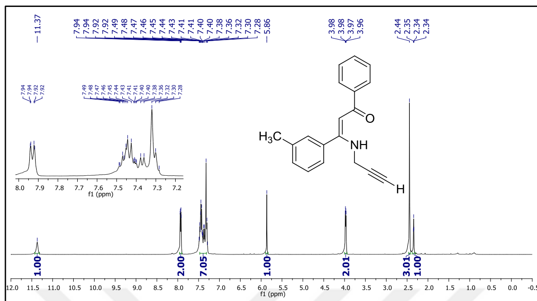
Figure 71. ^1\text{H} NMR spectrum of compound 26g .
