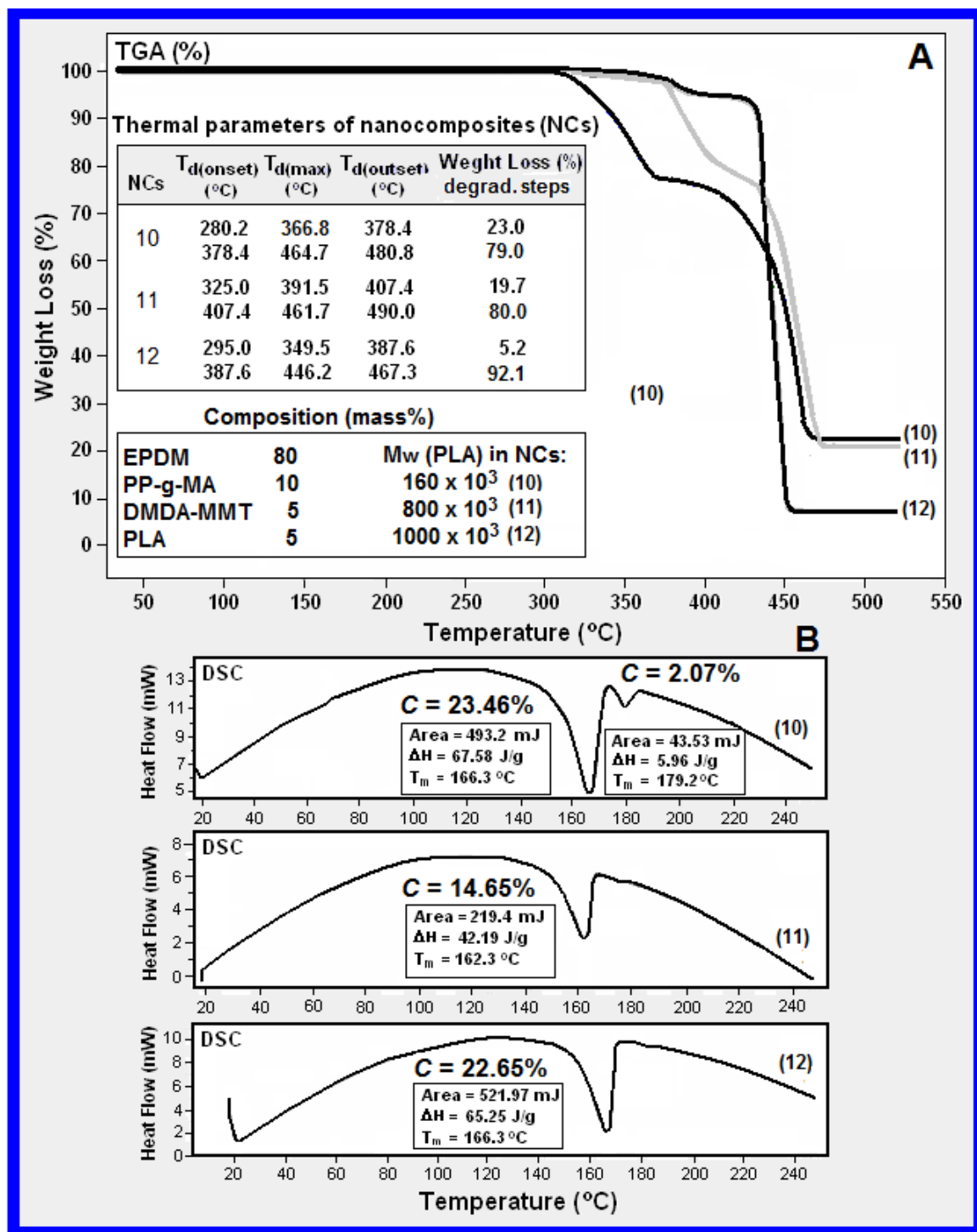
Figure 4.23. (A) TGA and (B) DSC curves of EPDM/PP-g-MA blend incorporated with PLA/DMDA (5 %) nanocomposite contained PLA with different Mw. Effect of PLA molecular mass on the thermal behaviors of NCs.
