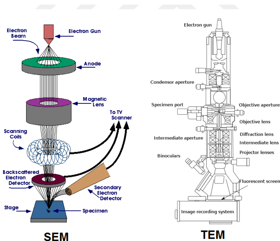
Figure 2.13. SEM and TEM working elements during analysis [41].
