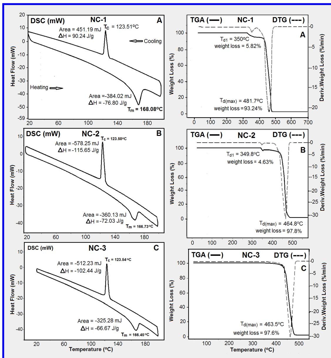
Figure 4.10. The DSC curves of melting (heating) and recrystallization (cooling) processing and TGA-DTG curves and thermal degradation parameters of NC-1 (A), NC-2 (B) and NC-3 (C) nanocomposites. Heating/cooling rate of 10 ^{\circ}\text{C}/\text{min} under nitrogen atmosphere.
