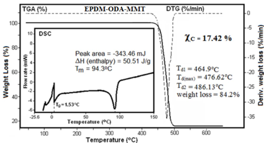
Figure 4.20. DSC and TGA-DTG curves of pristine EPDM/ODA-MMT rubber. Heating rate 10 ^\circ\text{C}/\text{min} under nitrogen flow.
