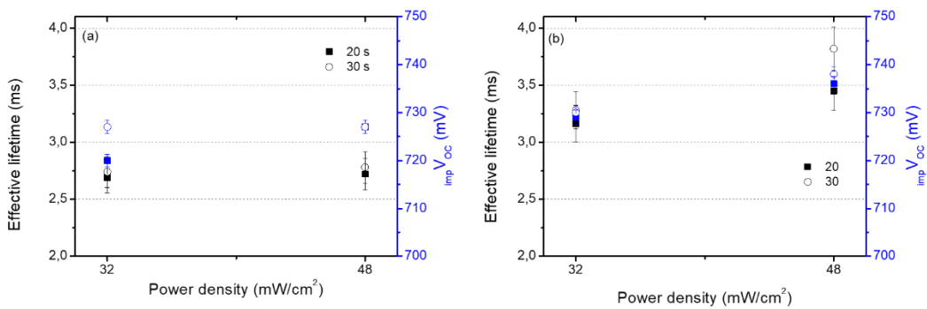
Figure 4. 5. Effective lifetime and _{imp}V_{OC} results after HPT at (a) 1.0 Torr and (b) 1.5 Torr pressures.
