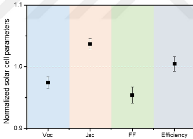
Figure 3. 15. Solar cell parameters fabricated on tetragonal-star-shaped IPs normalized for upright pyramids.
