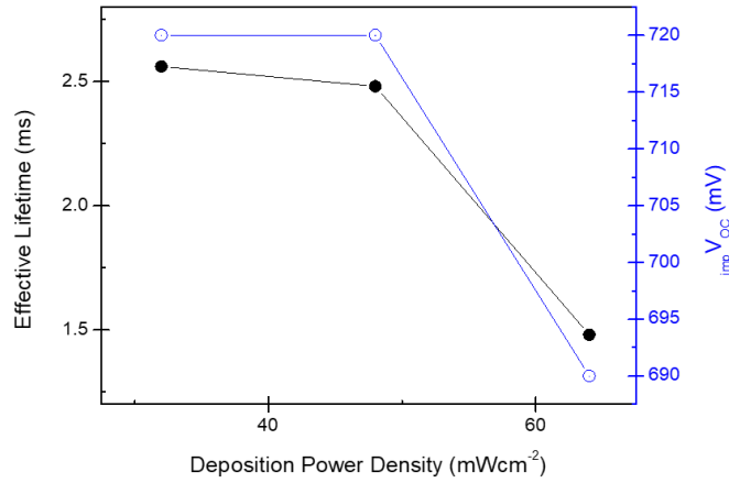
Figure 4. 3. Effective lifetime and \text{imp}V_{\text{OC}} results for various deposition power densities.
