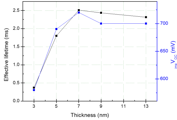
Figure 4. 4. Effective lifetime and _{imp}V_{OC} results for various thicknesses of (i) a-Si:H layer.
