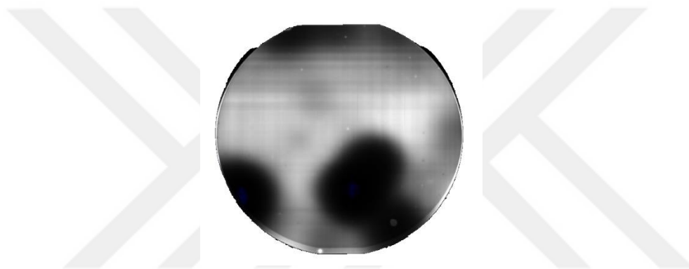
Figure 4. 12. PL images of the sample passivated with SiO 2 .
