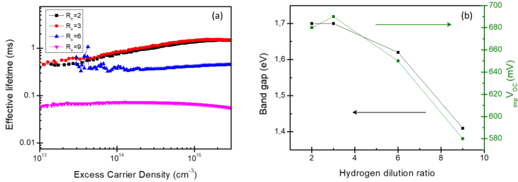
Figure 4. 2. (a) Effective lifetime vs. excess carrier density results and (b) band gap/ \text{imp}V_{\text{OC}} results for various hydrogen dilution ratios.
