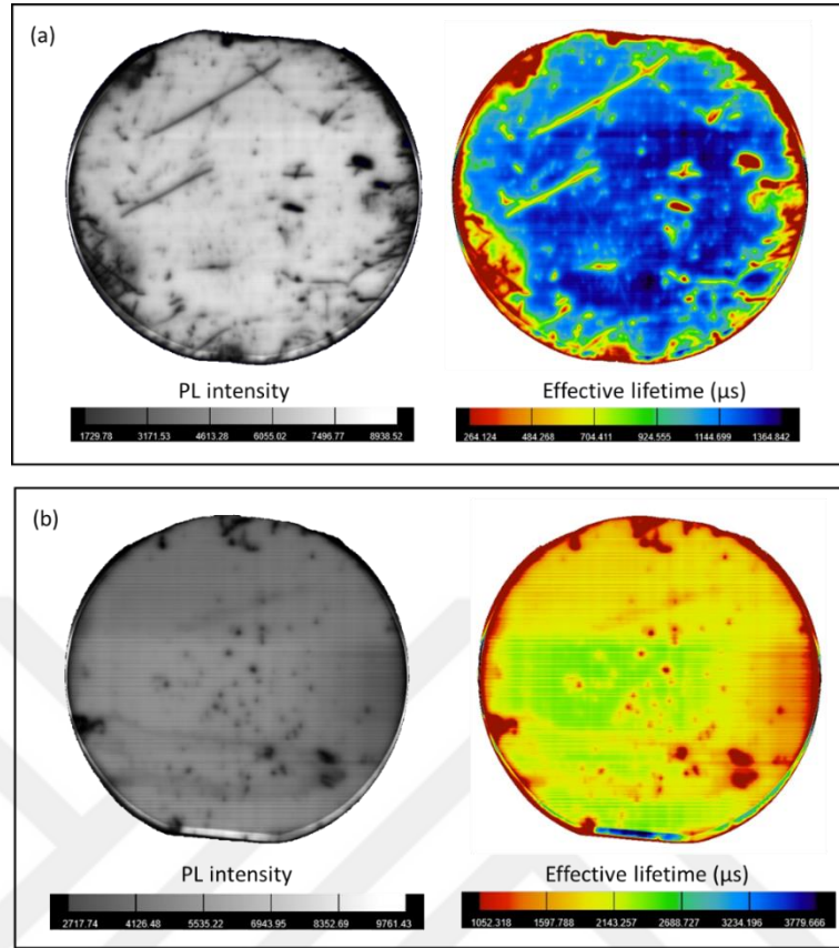
Figure 4. 11. Corrected (left) and calibrated (right) PL images of (i) a-Si:H passivated samples showing (a) scratches due to glass holder and (b) with new Al holder.
