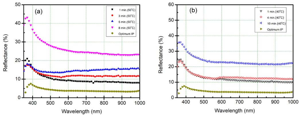
Figure 3. 16. Spectral reflectance results of Si surface after etching for various durations at (a) 50^\circ\text{C} and (b) 40^\circ\text{C} .
