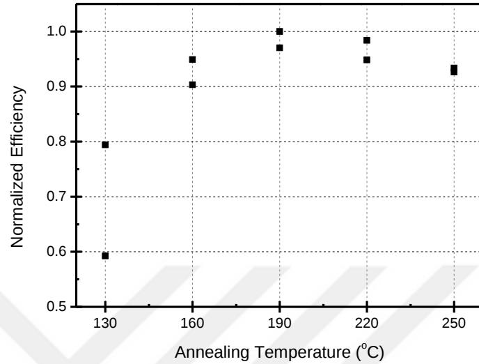
Figure 6. 26. The normalized efficiency values of ESH solar cells for different annealing temperatures.
