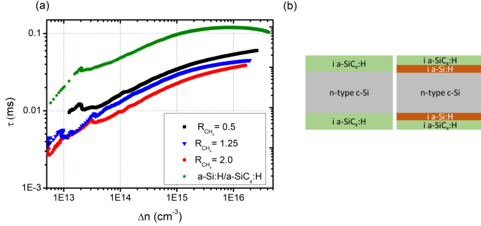
Figure 4.33. (a) Effective lifetime results of a-SiC x :H layers deposited at 80 mWcm -2 and R_{H_2} = 3 under various methane flow and stack layer passivation values, (b) cross-sectional view of the passivation structure.
