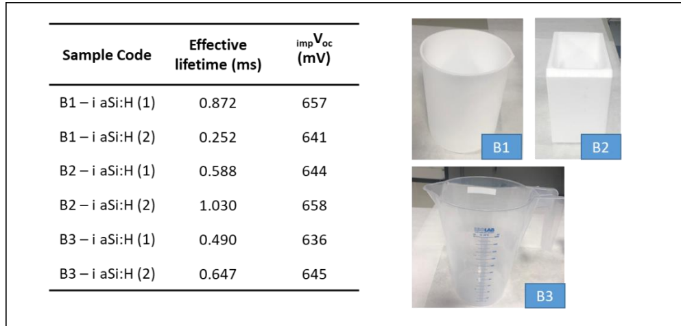
Figure 4. 16. Effective lifetime results of samples after cleaning in the new PFA (B1) and PVDF (B2) beakers, and only native-oxide cleaning by dipping into HF:HCl:H 2 O solution inside the PP beaker (B3).
