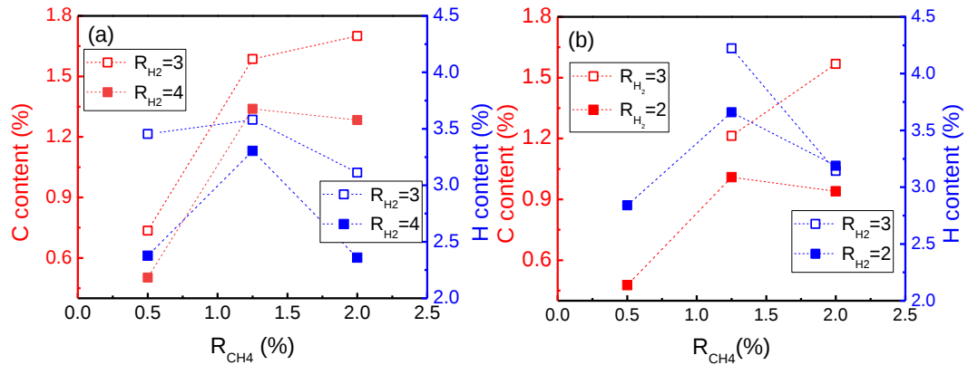
Figure 4. 27. Hydrogen and carbon content of a-SiC x :H layers for (a) 80 mWcm -2 and (b) 48 mWcm -2 deposition power densities.
