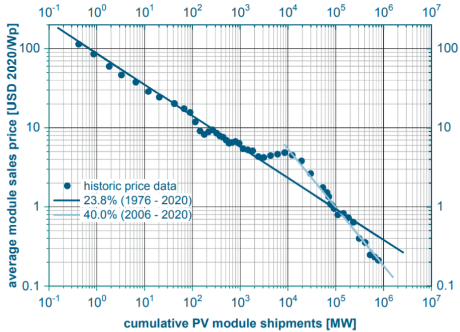
Figure 1. 6. The learning curve of module price as a function of cumulative shipments [14].
