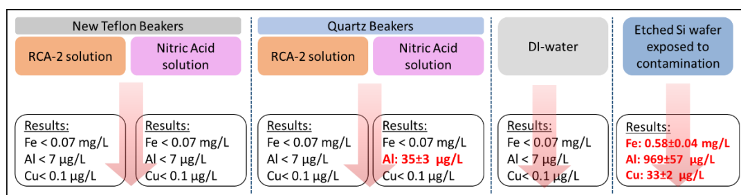
Figure 4. 18. ICP-MS results for various possibly contaminated samples.
