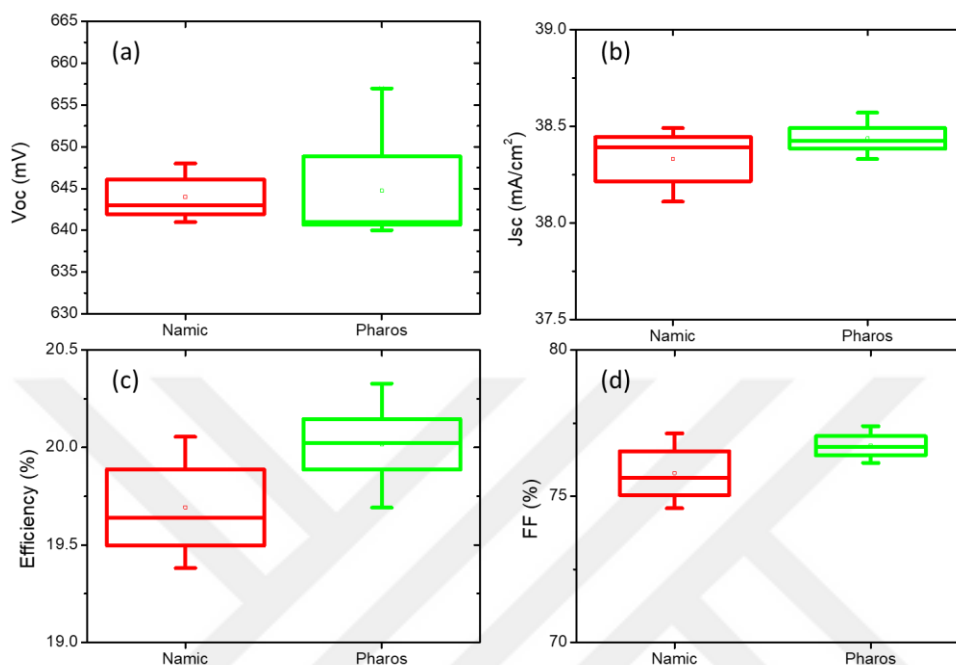
Figure 6. 18. Comparative results for SHJ solar cell parameters metalized by two different low-temperature Ag pastes.
