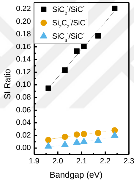
Figure 4. 31. Different corporations of C atoms with Si atoms in the matrix increase linearly with the optical band gap values as the mean SI ratio of the cluster combinations in \text{a-SiC}_x\text{:H} matrices.
