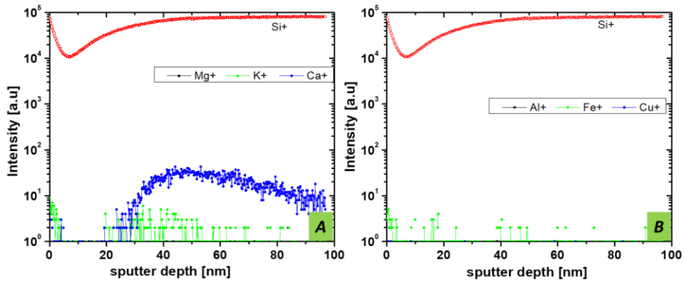
Figure 4. 19. ToF-SIMS measurement profiles for the samples cleaned in new quartz beakers and passivated with (i) a-Si:H layer.
