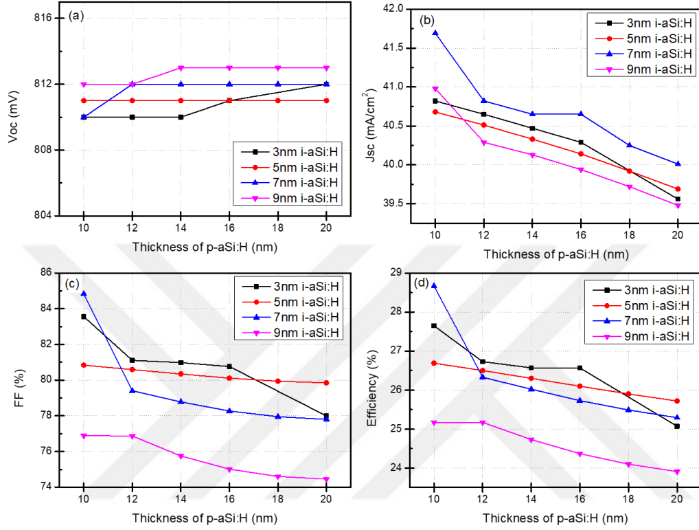
Figure 2. 8. The impact of (p) a-Si:H and (i) a-Si:H thickness on (a) V_{OC} , (b) J_{SC} , (c) FF and (d) \eta values.
