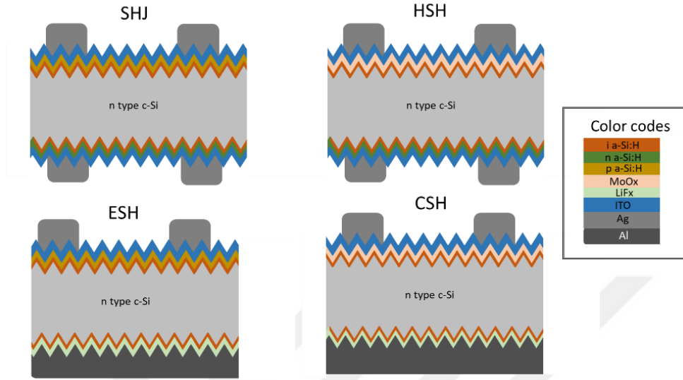
Figure 6. 23. Cross-sectional view of different CSH solar cell structures.
