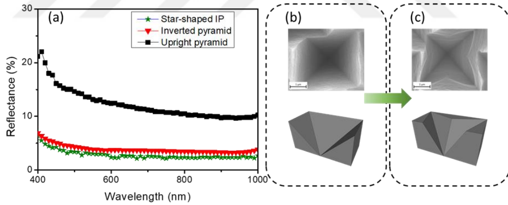
Figure 3. 14. (a) The comparison of spectral reflectance for random upright pyramid, IPs, and tetragonal-start-shaped IPs and (b) top SEM view and cross-sectional representative of standard and (c) tetragonal-star-shaped IPs.
