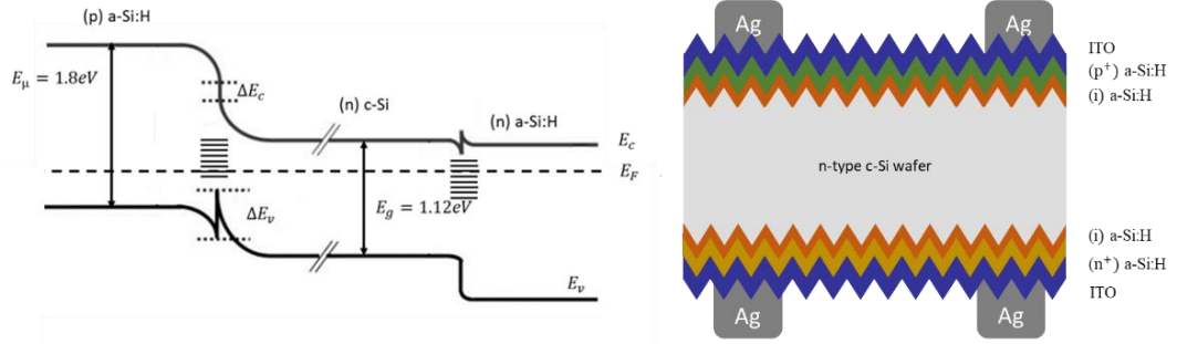
Figure 1. 7. The band gap diagram (left) and sectional view (right) of SHJ solar cell.
