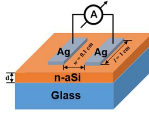
Figure 5. 2. Cross-sectional view of the sample prepared for I-V characterization.
