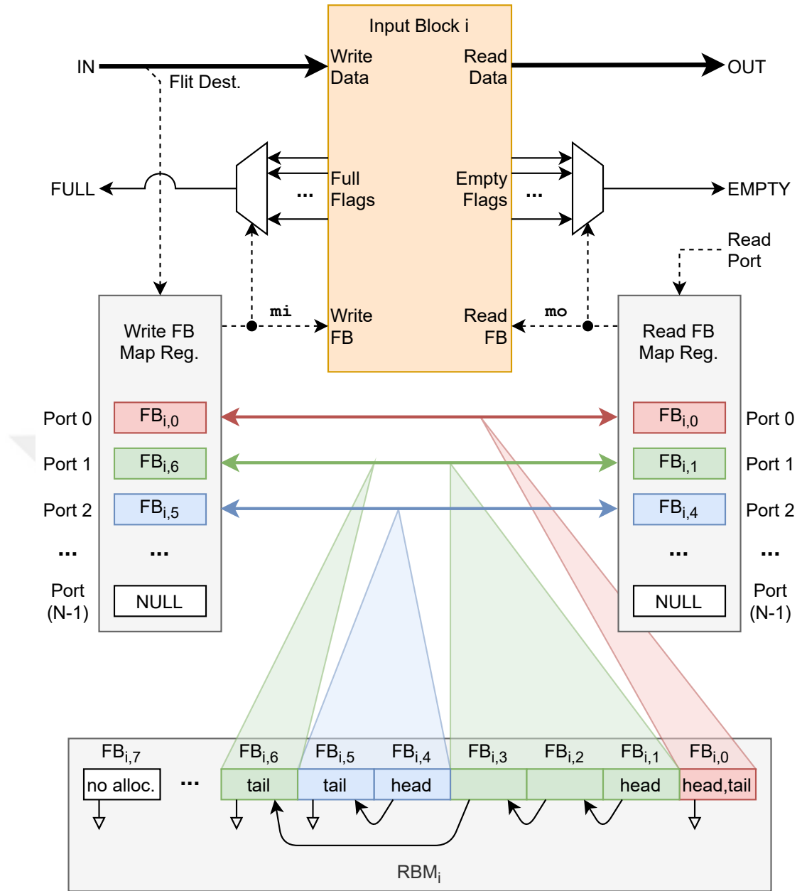
Figure 3.2: Flex Buffer Allocation for Resource Efficient FIFO Organization
