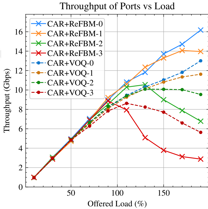
Figure 4.6: ReFlex Buffer Management with CAR (ports)
