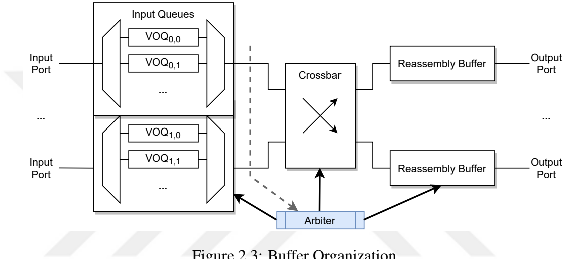
Figure 2.3: Buffer Organization
