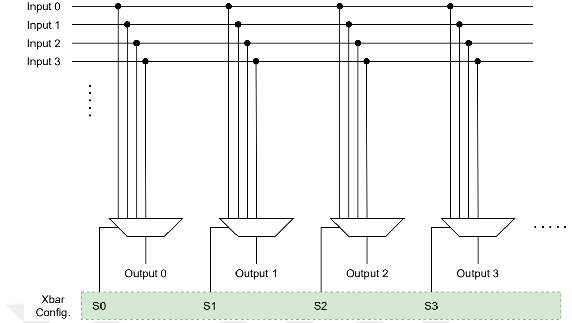
Figure 2.1: Crossbar Fabric
