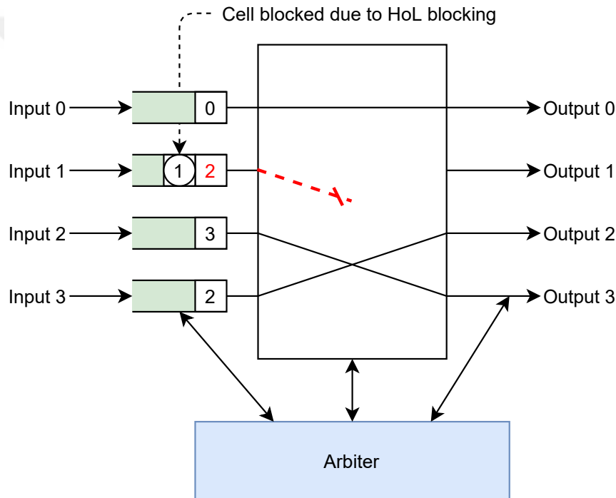
Figure 2.2: HoL Blocking Problem
