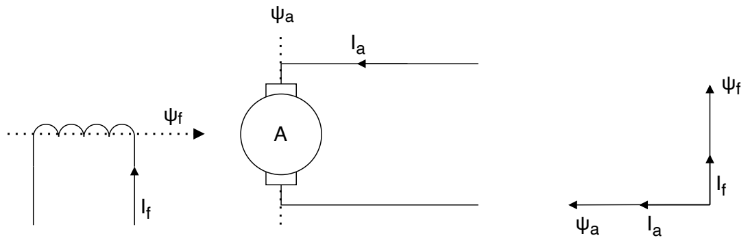
Figure 2.8: Separately excited DC motor with current [4]
