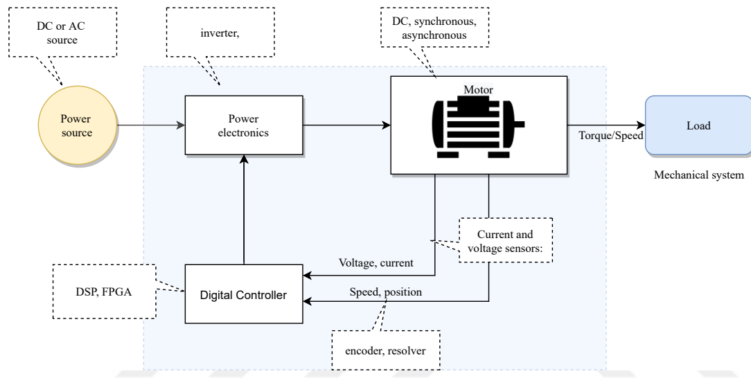
Figure 1.1: Block diagram of motor drives
