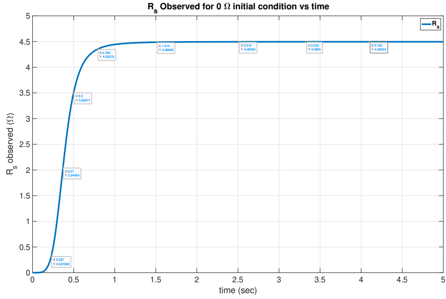
Figure 4.3: Convergence of the estimator when the initial condition for \hat{R}_s is 0 \Omega
