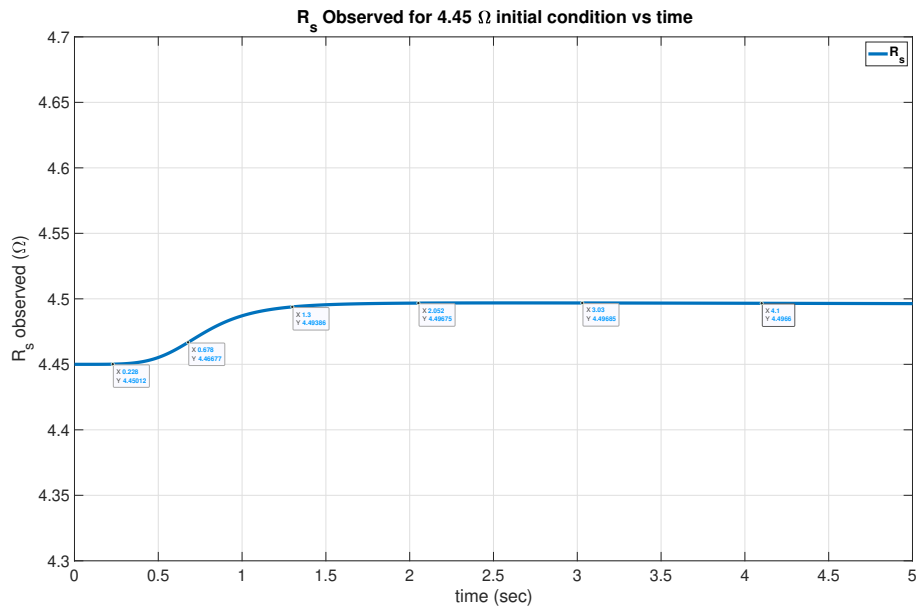
Figure 4.4: Convergence of the estimator when the initial condition for \hat{R}_s is 4.45 \Omega
