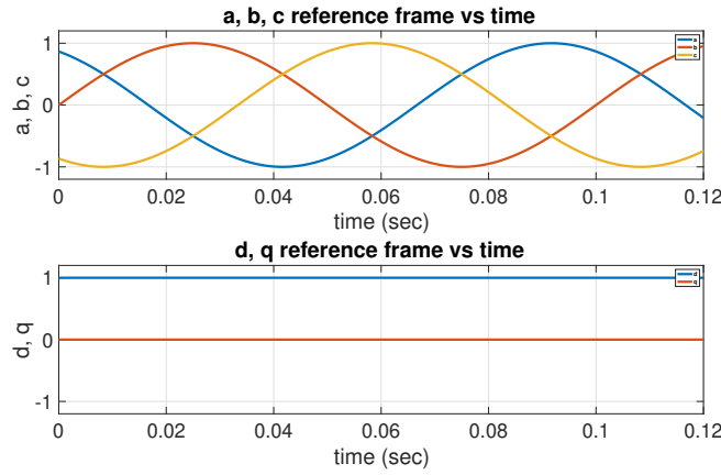
Figure 2.17: Stationary reference frame to synchronous reference frame transformation
