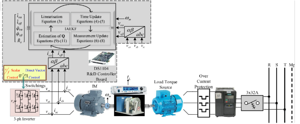
Figure 5.1: Block diagram of the experimental setup conducted with an Inverter
