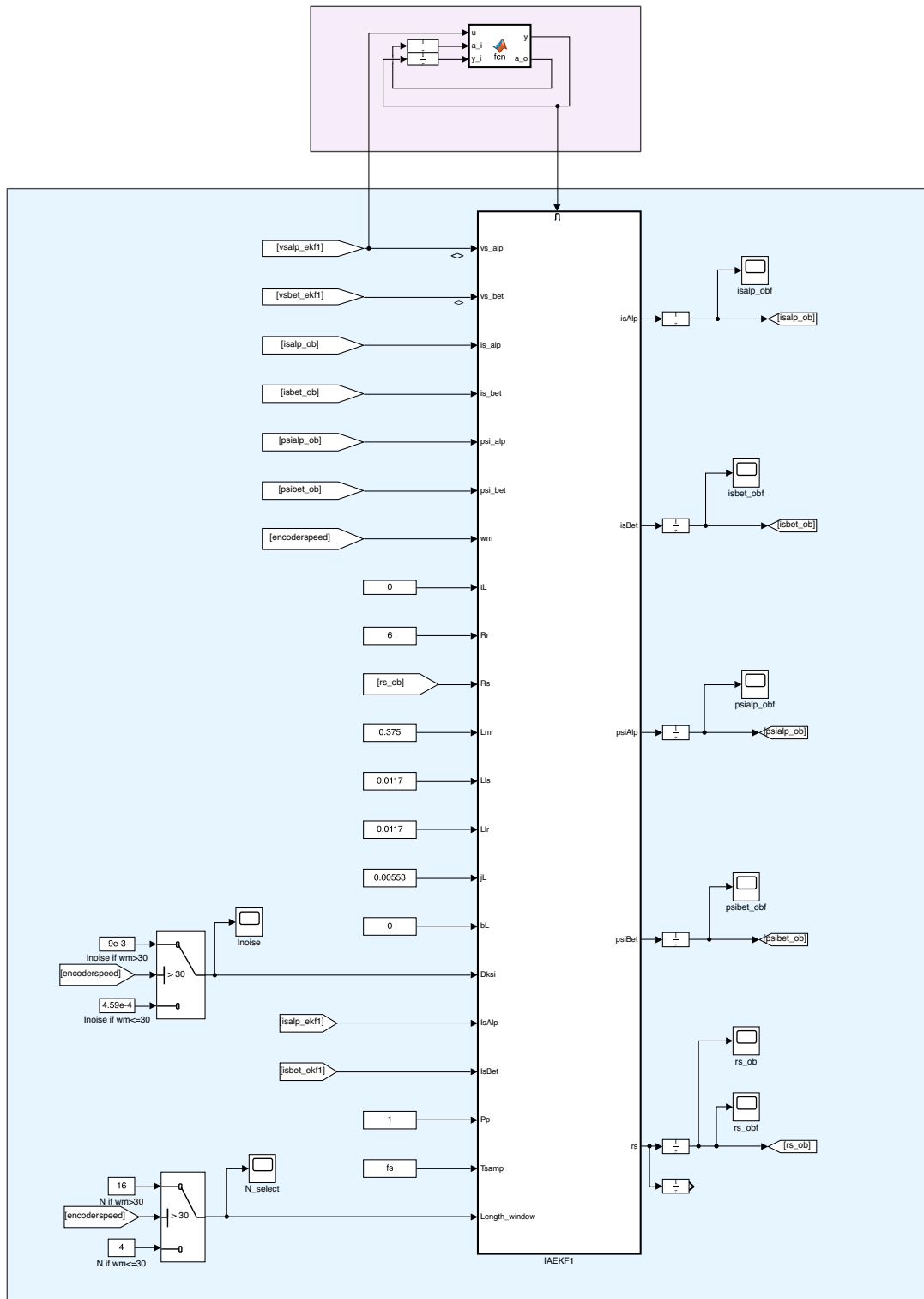
Figure 4.1: IAEKF algorithm's subsystem in Simulink
