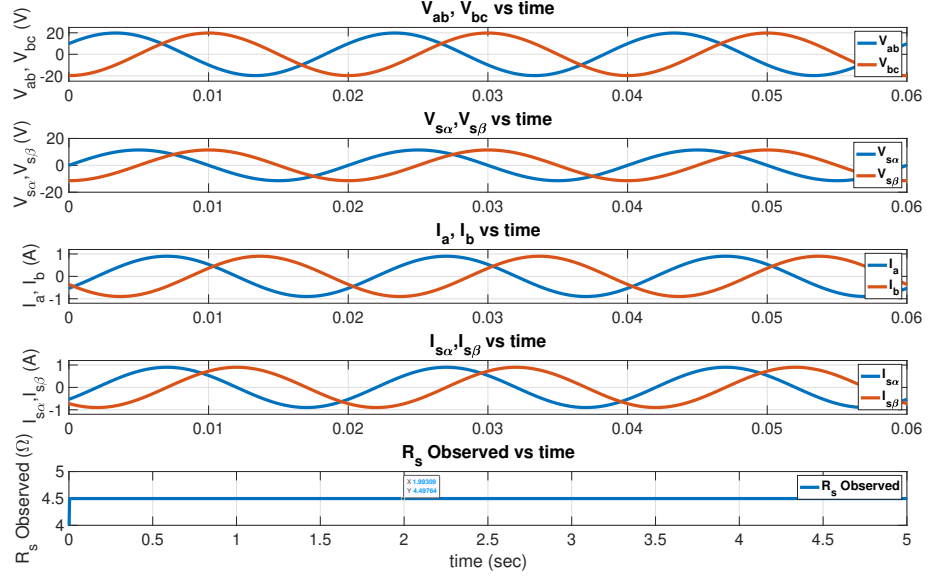
Figure 4.5: Standstill simulation result for test motor without any series resistance
