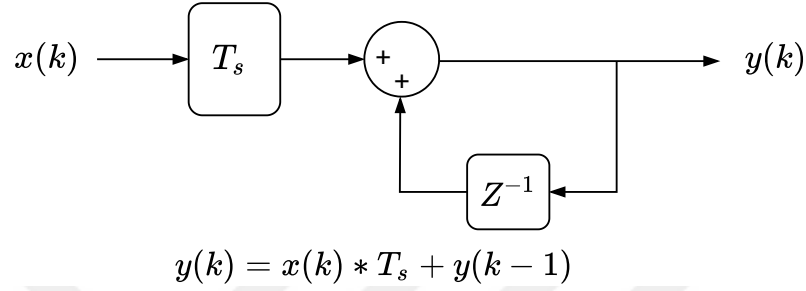
Figure 2.20: Discrete integrator implemented with backward Euler method
