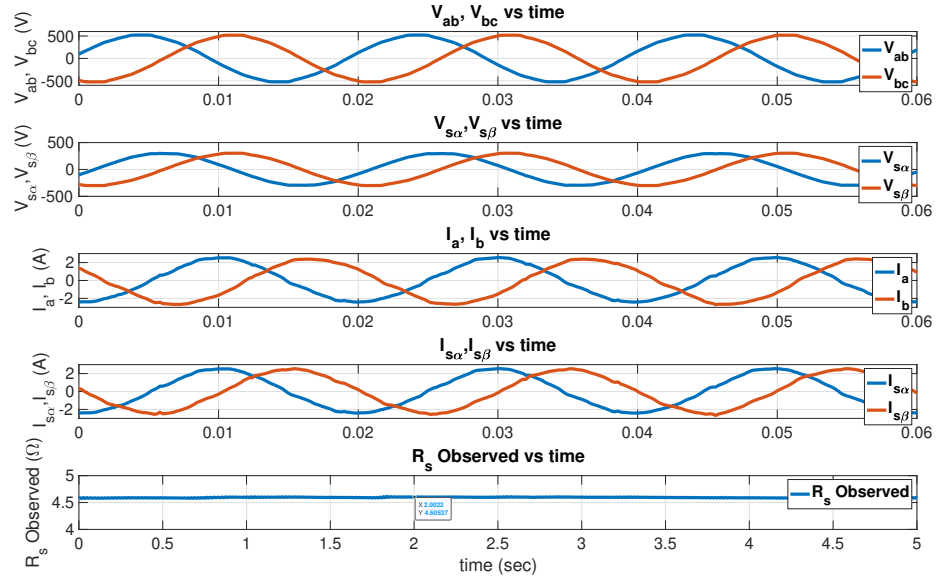
Figure 6.5: Variables used to estimate R_s at 3000 RPM without 1\ \Omega series resistance
