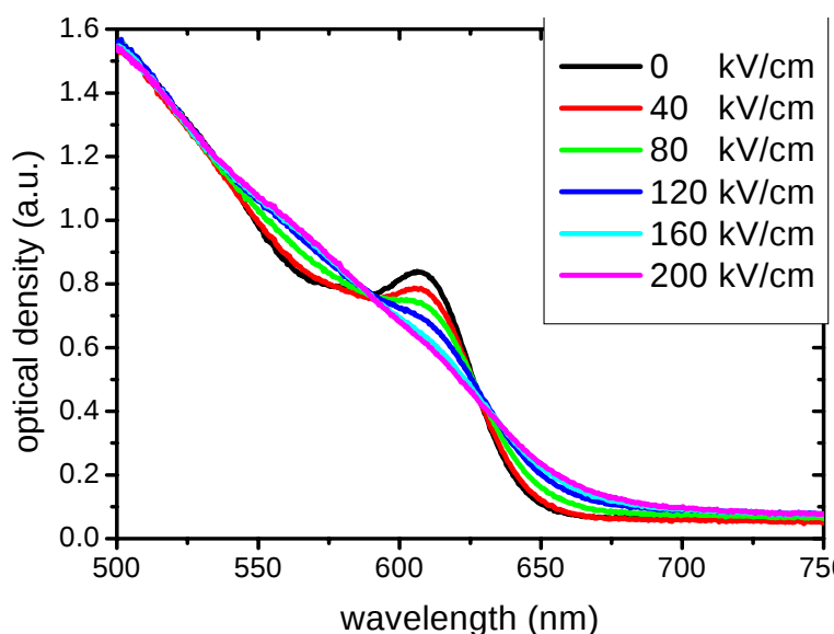
Figure 3.2.3.3 Optical density of CdSe nanodots for different electric field values.
