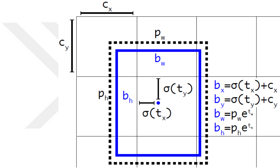
Figure 2.2.1. YOLOv3 Bounding Box Calculations.
