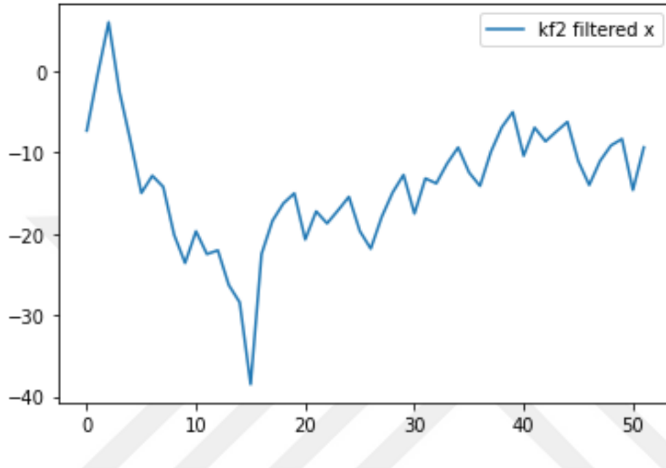
Figure 4.13. Kalman Filter 2 x- axis error graph.
