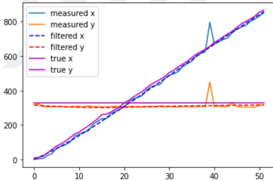
Figure 4.10. Star x, y Coordinate Values Higher Covariance Kalman Filter 2.
