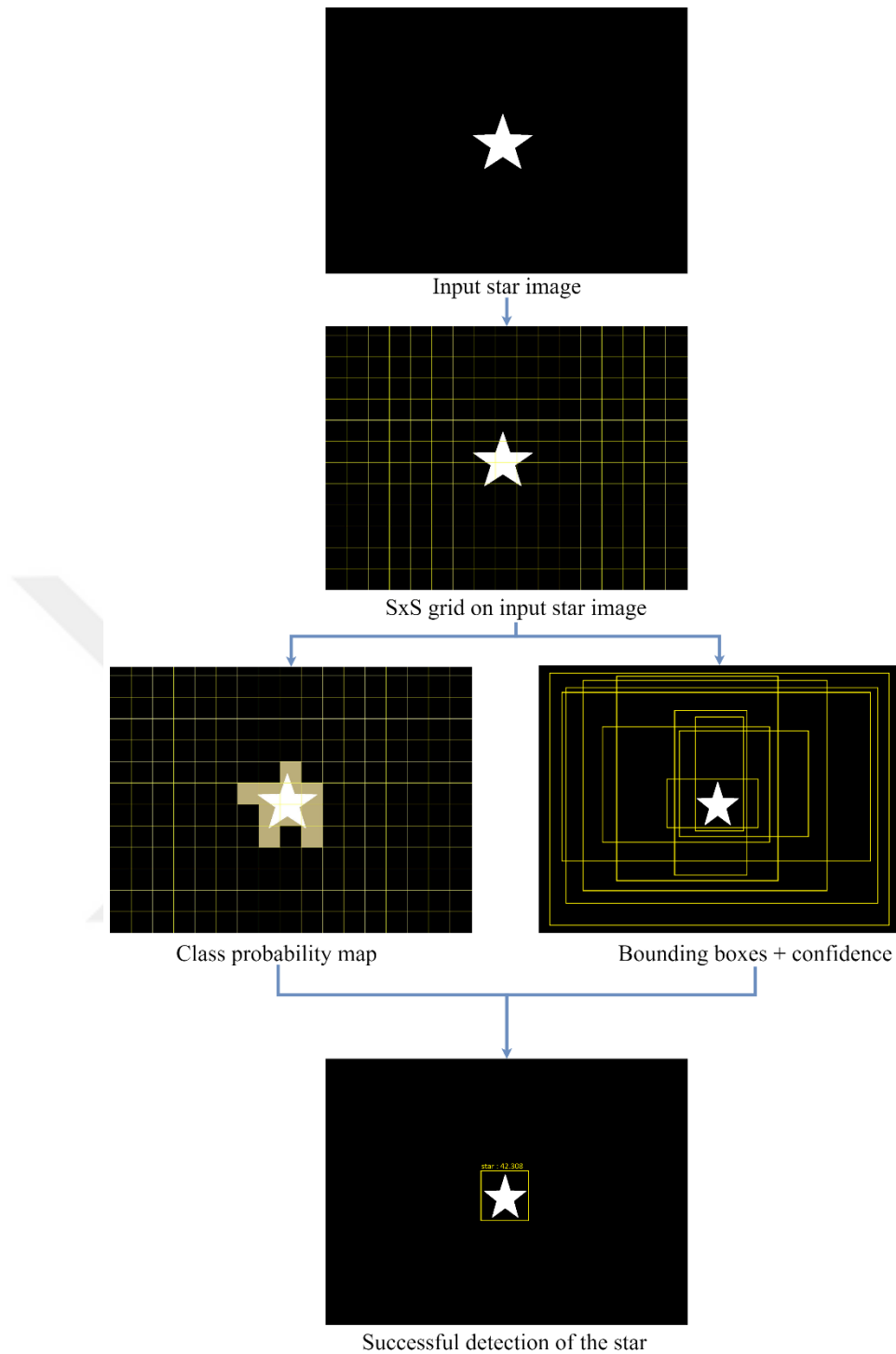
Figure 2.3.1. Star detection with YOLOv3 architecture.
