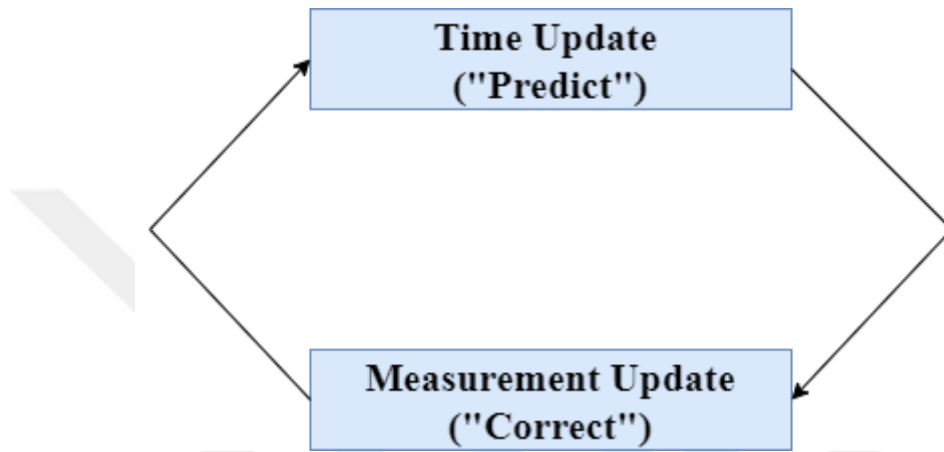
Figure 3.1.1. Continuing Discrete Kalman Filter Cycle.
