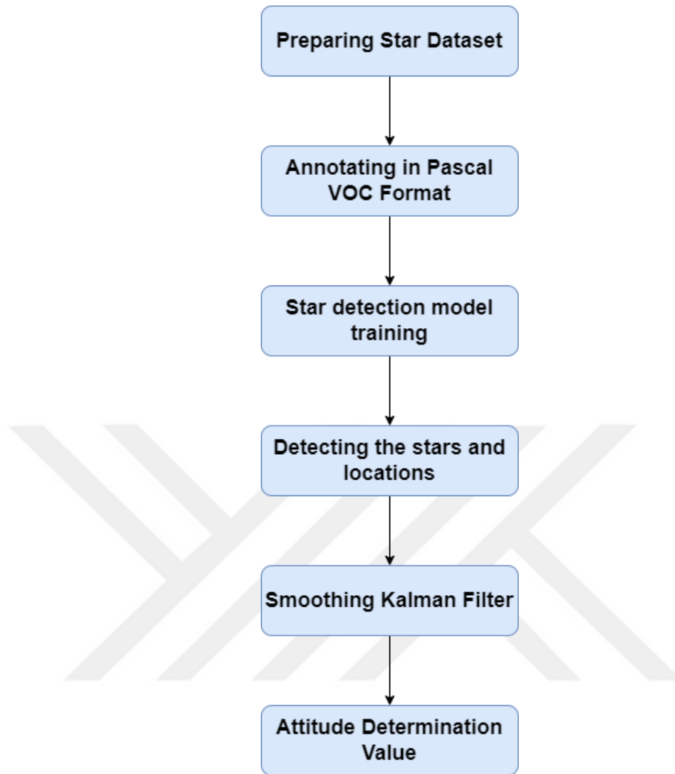
Figure 2.1. Block Diagram of Algorithm.
