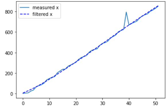
Figure 4.6. Kalman Filter 2 x-axis output.
