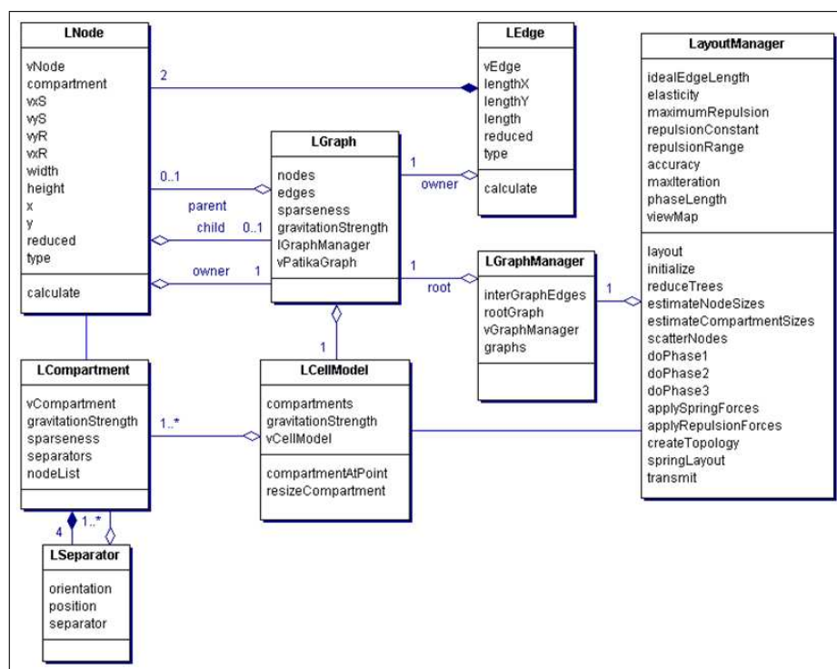
Figure 5.1: All information required to layout a view is stored as described here.
