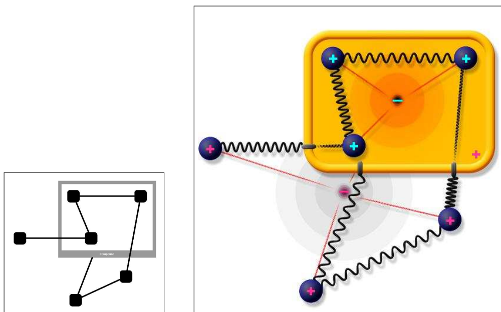
Figure 4.1: Part of a sample compound graph (left) and the corresponding physical model used by our algorithm (right).
