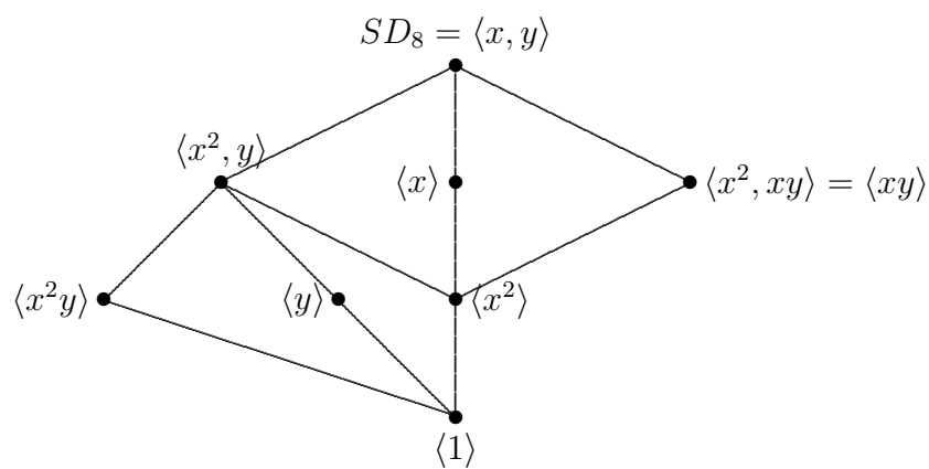
Figure 4.5: SD_8
