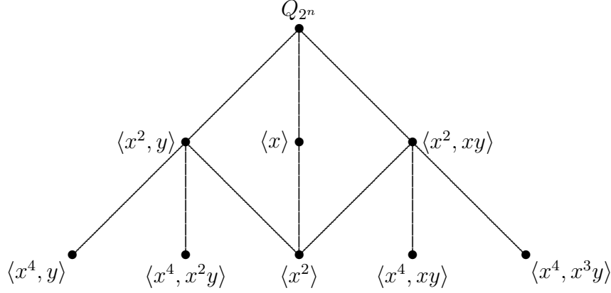
Figure 4.8: Q_{2^n}
