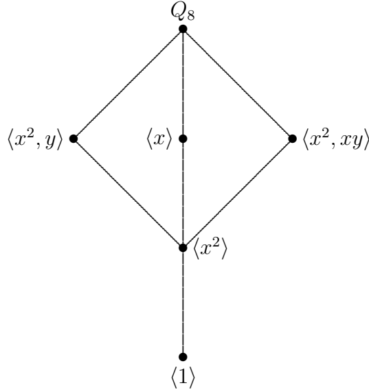
Figure 4.7: Q_8
