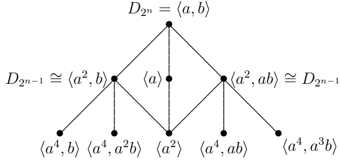
Figure 4.1: D_{2^n}
