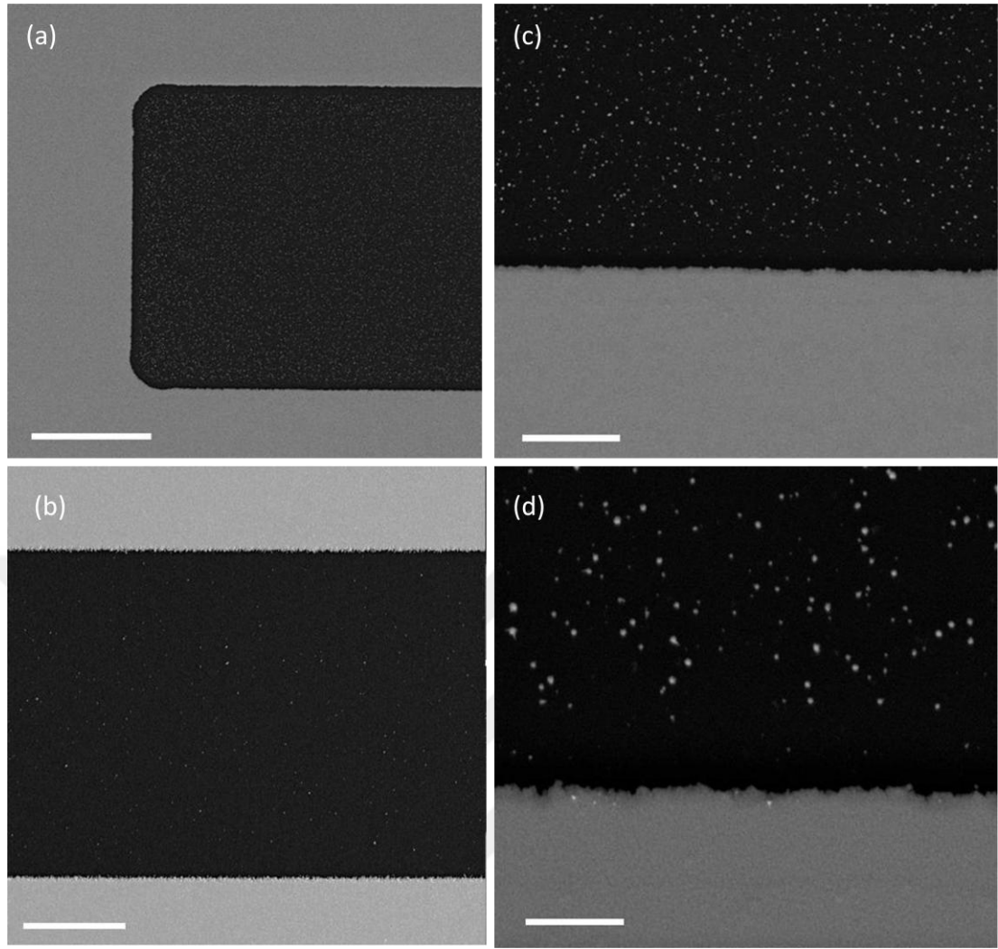
Figure 3.1. SEM micrographs of gold nanoparticles located in the gaps between the electrodes on the PMMA surface. Scale bars are 20, 15, 5 and 2\mu\text{m} for (a), (b), (c), (d) respectively.
