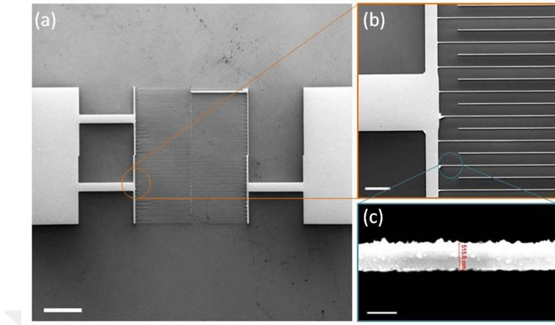
Figure 2.7. SEM images of 500nm comb-like electrode lines fabricated from EBL. Scale bars are 250, 25 and 0.5 \mu\text{m} for (a), (b) and (c) respectively.
