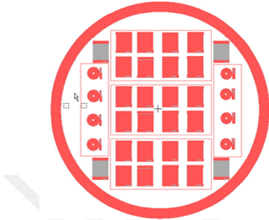
Figure 2. 1. L-Edit mask of the electrodes for fabrication in photolithography
