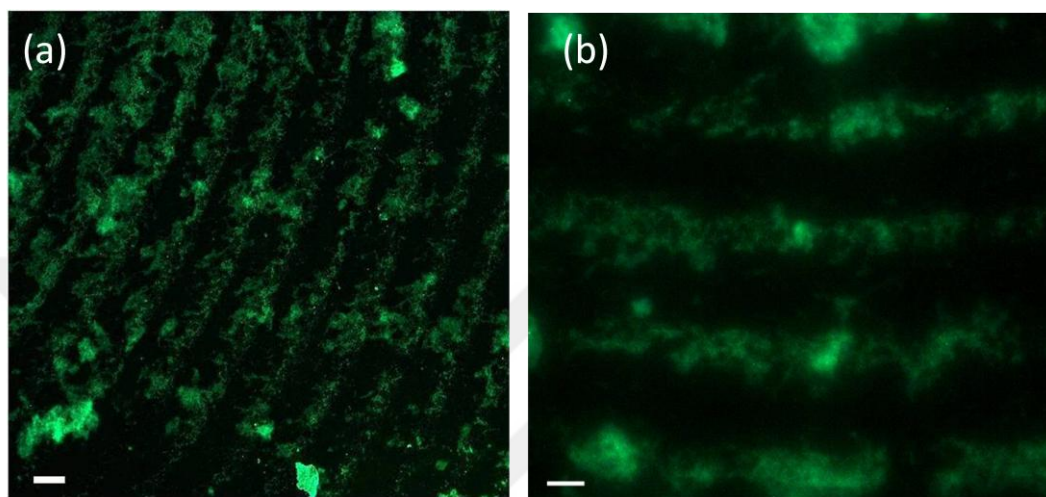
Figure 3.3. Fluorescent micrographs of latex nanoparticle assemblies on the tori-like electrode surface. Scale bars are 40 and 20 \mu\text{m} for (a) and (b) respectively.
