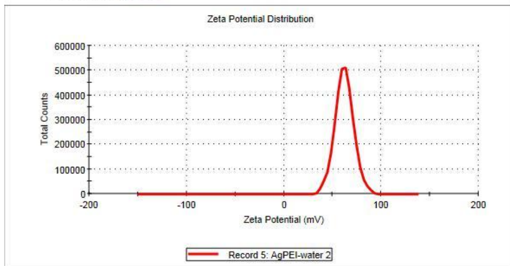
Figure A1. Zeta potential curve for positively charged silver nanoparticles.
