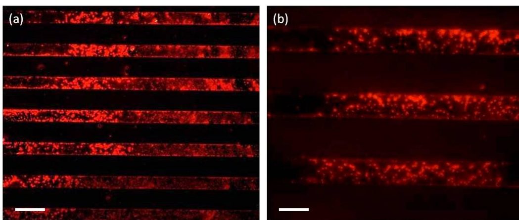
Figure 3.5. Fluorescent micrographs of silica nanoparticle patterns on rectangular electrodes. Scale bars indicate 50 and 20 \mu m for (a) and (b) respectively.
