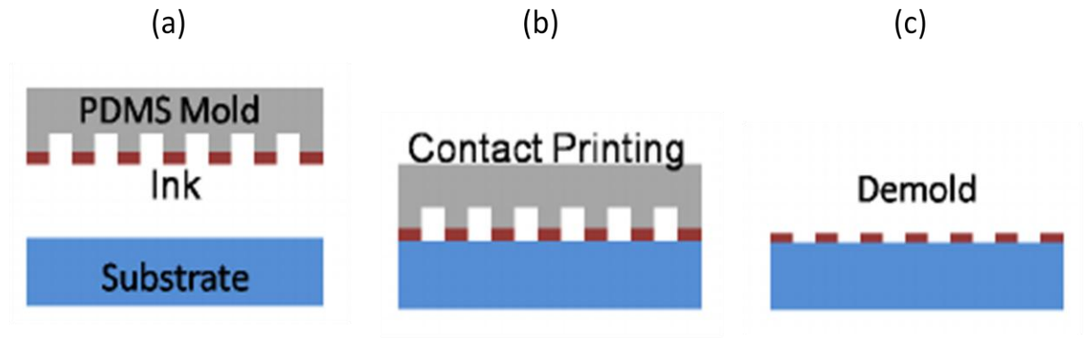
Figure 1.1. Nanoimprint Lithography steps (a) structured PDMS mold with target ink (nanoparticle) (b) pattern transfer onto substrate. (c) patterned substrate.
