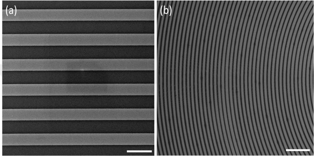
Figure 2.6. SEM micrographs of gold electrodes. a) Rectangular shape (electrode lines are parallel to each other) b) Tori-like shape. Scale bars are 50 and 250 \mu\text{m} for (a) and (b) respectively.
