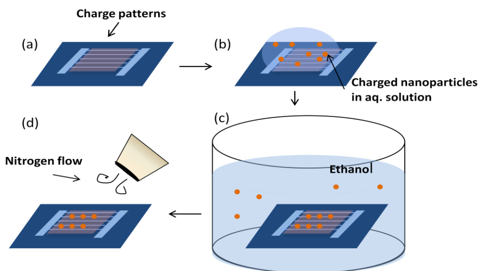
Figure 2.9. Schematics of the experimental procedure: (a) substrate with charge patterns; (b) dropping the nanoparticle solution to the surface for certain amount of time; (c) developing in ethanol to remove nanoparticles from undesired areas; (d) drying the surface.
