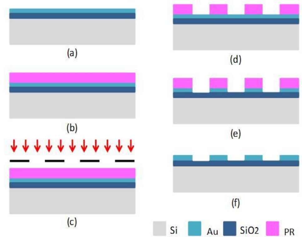
Figure 2.5. Schematics of fabrication steps of electrodes obtained with photolithography. (a) Thermal evaporation of 100 nm gold film on \text{SiO}_2 substrate. (b) Photoresist spin-coating (c) Transferring electrode patterns to PR surface by using UV exposure (red arrows) and photomask (black lines). (d) PR development
