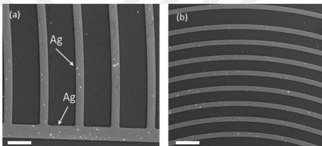
Figure 3.2. Silver nanoparticles accumulations on the tori-shape electrodes. Scale bars are 50 \mu for (a) and 100 \mu m for (b).
