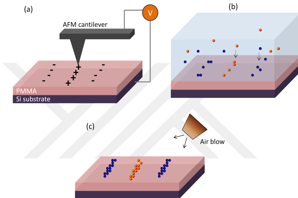
Figure 1.3. Schematics of AFM nanoxerography where the charged nanogels are electrostatically directed to the surface. (a) AFM charge writing on dielectric film (b) development in solvent after nanoparticles incubation (c) air blow drying.
