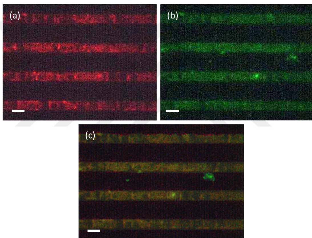
Figure 3. 8. Composite patterns containing silica (a) and latex (b) assembled on 20 \mu\text{m} wide electrodes ; (c) combination of (a) and (b) to show that both particles are on the same surface. Scale bar is 20 \mu\text{m} for all images.
