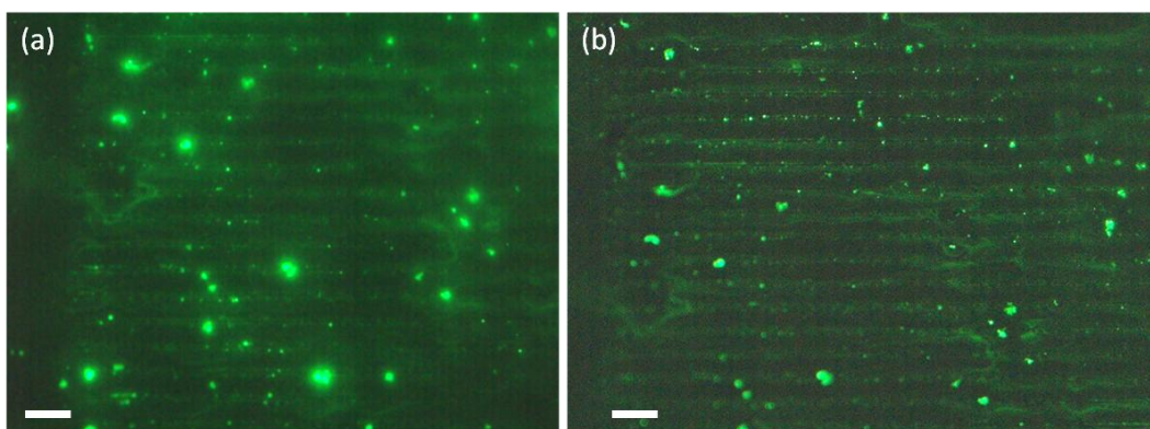
Figure 3.4. Latex nanoparticle patterns on 500 nm wide electrodes. Scale bar is 2 \mu m for both images.
