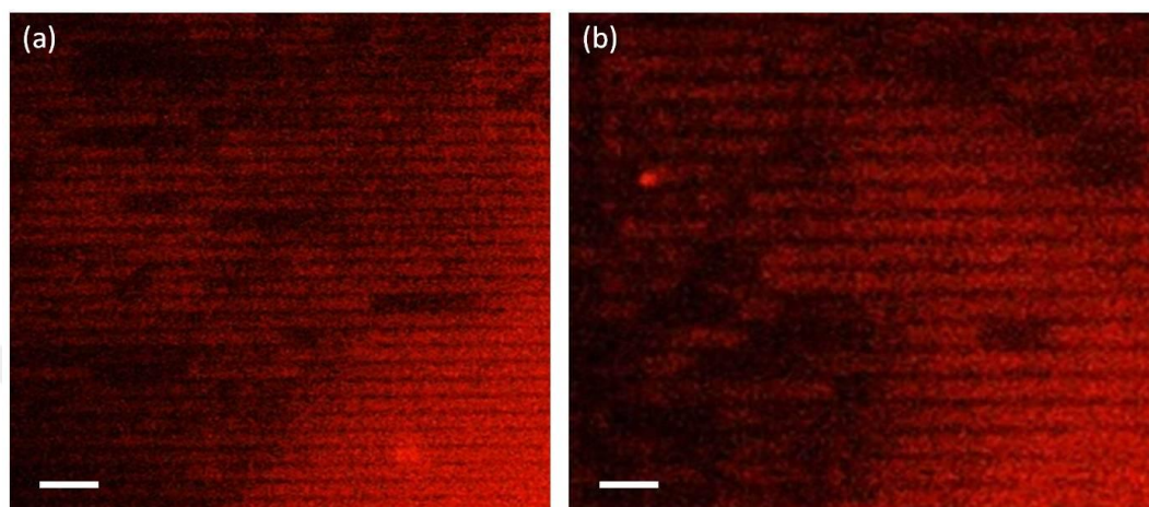
Figure 3.6. Silica nanoparticle deposition on 1 \mu\text{m} electrode lines. Scale bars are 4 and 2 \mu\text{m} for (a) and (b) respectively.
