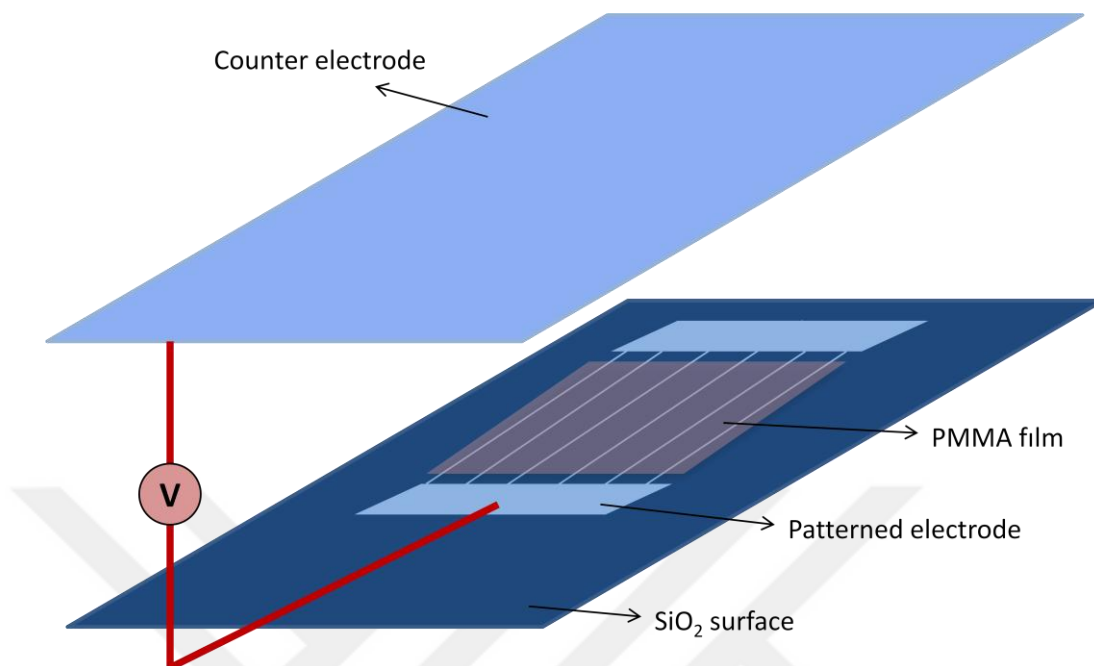
Figure 2. 8. Simple schematic view of the set-up for PMMA polarization
