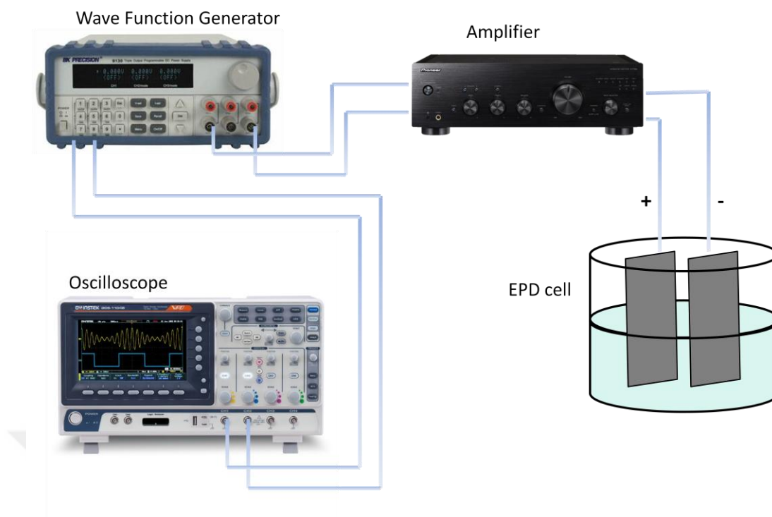
Figure 1.7. Experimental set-up for pulsed voltage electrophoretic deposition.
