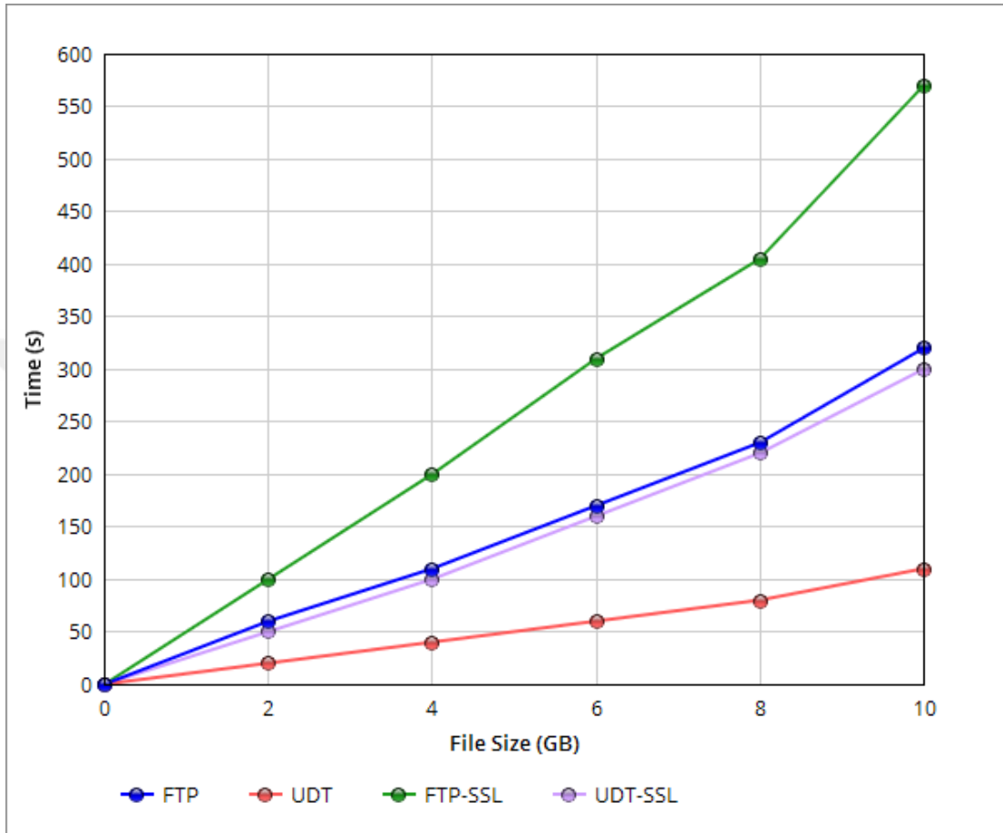
Figure 1.2: Performance Evaluation of FTP vs. UDT protocols with different file sizes. Adapted from [14].
