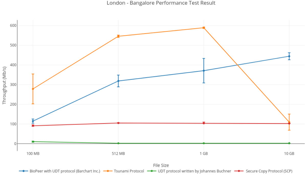
Figure 3.2: Performance test results in high latency network.
