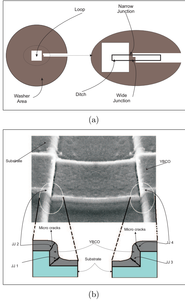
Figure 3.3: SEJ structure and the asymmetric grain boundary junctions shown for a rf-SQUID magnetometer.[2]
