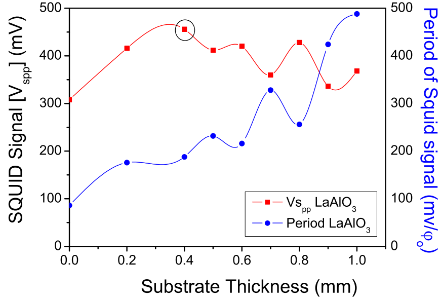
(a) LaAlO_3
