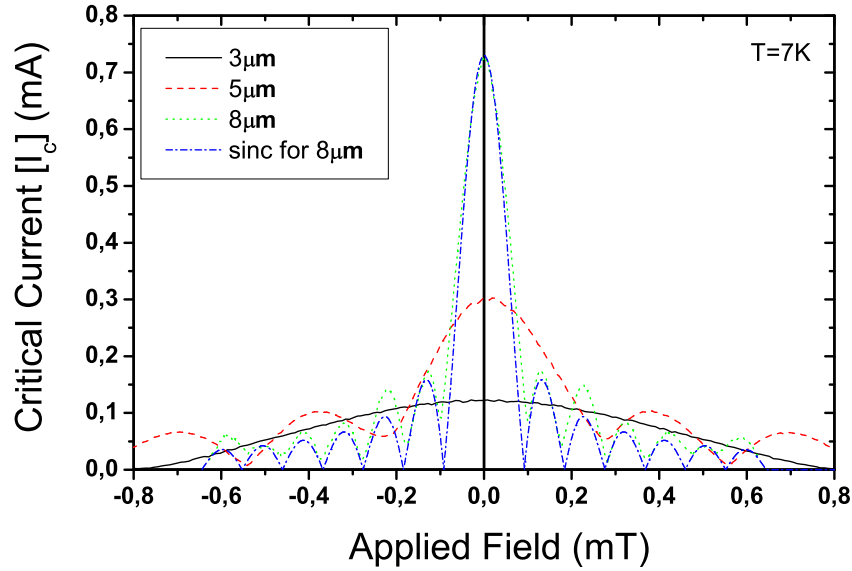
Figure 2.22: Magnetic field dependence of I_c of 3, 5, and 8 \mu\text{m} wide GB junctions on bi-crystal \text{SrTiO}_3 substrates. The calculated classical field dependence of the I_c is shown for the 8 \mu\text{m} wide junction.
