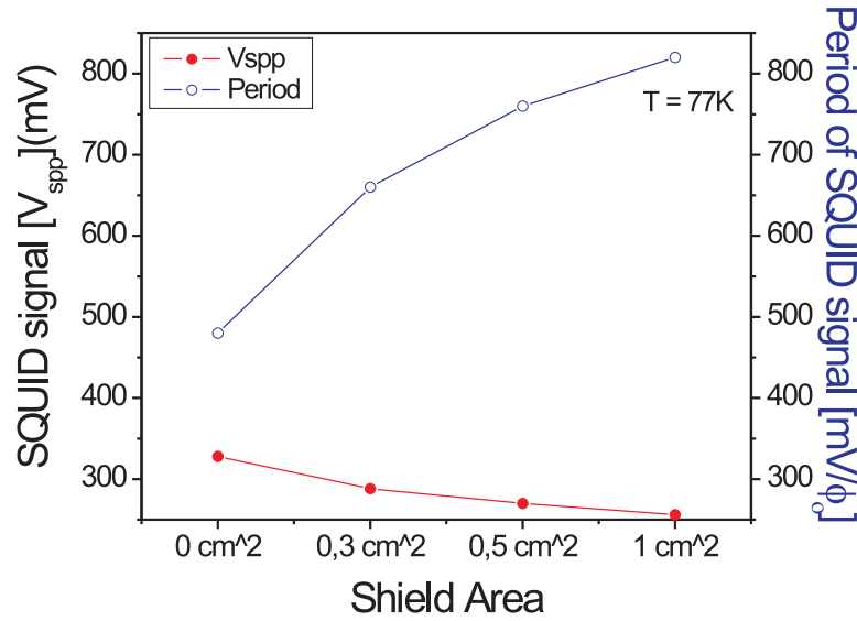
Figure 4.13: Effect of shield area on V_{spp} and period of the SQUID signal.
