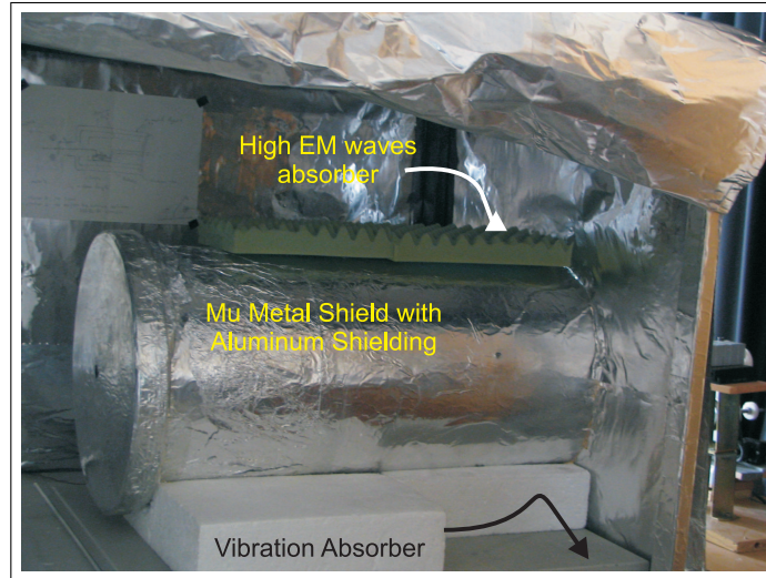
Figure 5.7: Three-layer \mu -metal shield with circular shape, used to shield against low frequency magnetic field.
