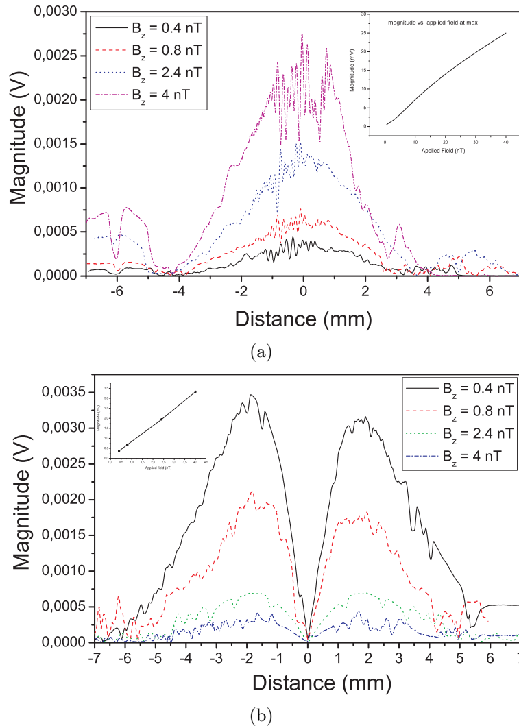
Figure 5.22: Finding the ultimate field resolution for wire scanning sample; (a) when the current through the wires are in the same direction, (b) when the current direction in the wires are apposite with respect to each other.
