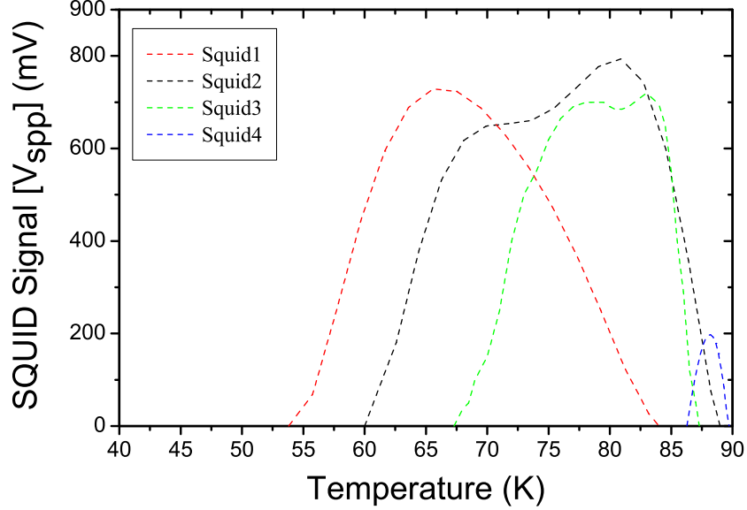
Figure 3.11: Flux to voltage transfer function signal, V_{spp} , versus temperature of rf-SQUID magnetometers with 100 \mu\text{m} \times 100 \mu\text{m} loops. “SQUID 2” has a 205nm deep ditch and SQUIDS 3 and 4 have 135nm deep ditches, made using the optimized CIBE process. “SQUID 1” has a 275nm deep ditch, made using un-optimized CIBE process. The junction width of “SQUID 3” is 2 \mu\text{m} , and the other devices have 3 \mu\text{m} wide junctions [5].
