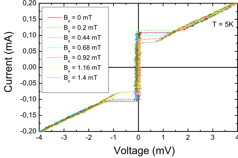
Figure 2.19: Magnetic field dependence of the I - V curves of a low field-sensitive 3\mu\text{m} wide junction made on 260nm deep CIBE steps.
