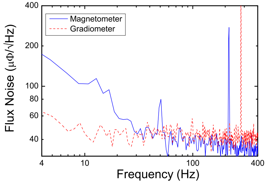
Figure 4.8: Noise spectra of bicrystal GB magnetometer and gradiometer designs on bicrystal SrTiO_3 substrate at their optimal operating temperatures.
