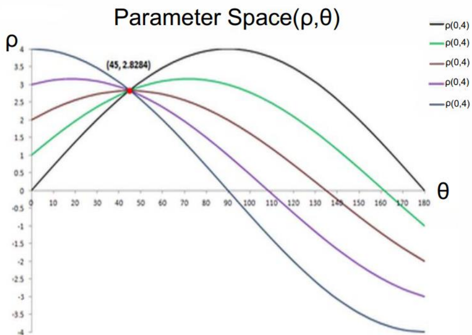
Figure 20: Line representation in (\rho, \theta) parameter space (Chandrasekar & Durga, 2014) © 2014 IEEE
