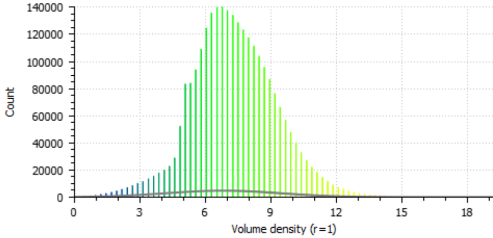
Figure 45: Histogram of spherical volume density ( r = 1 m) in Cadastre voxelized data (Gaussian Mean = 6.972, Standard Deviation = 2.593)
