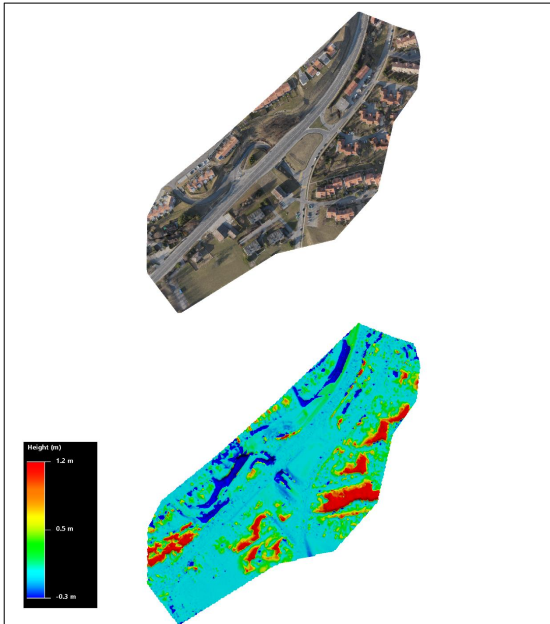
Figure 84: The RGB colored Cadastre dataset (top) and difference map between ground truth and CSF output
