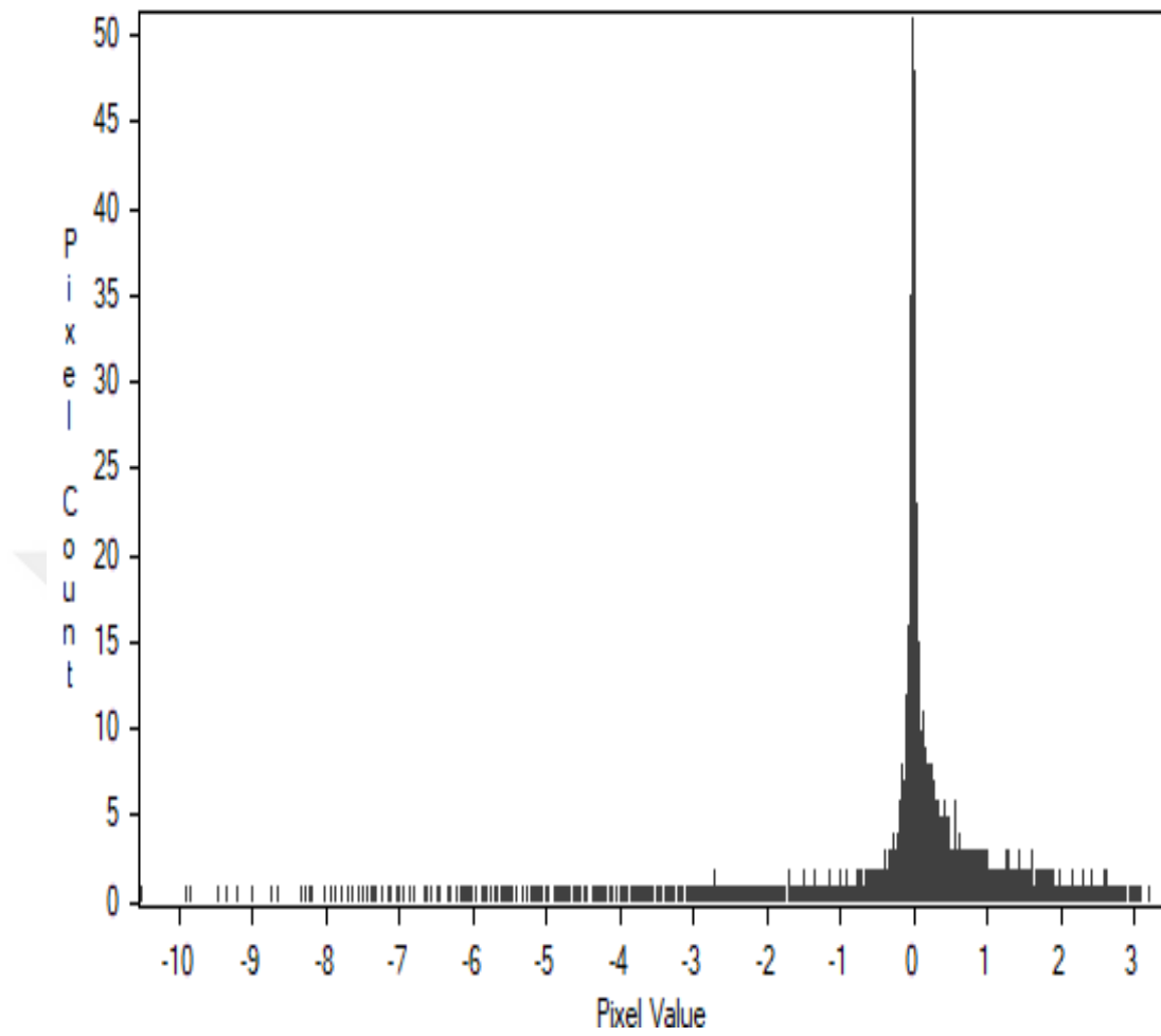
Figure 85: The histogram of the CSF output height difference in Cadastre dataset
