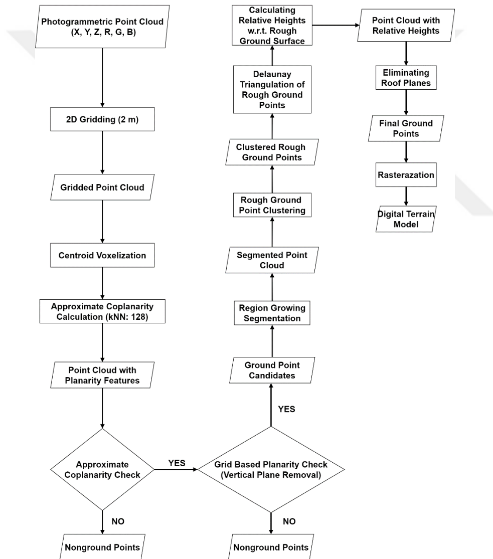
Figure 37: The flowchart of the proposed algorithm
