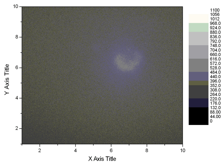
Figure 6.9a Acceptor emission in a cell both transfected with RFP-Mel and GFP-Cry
