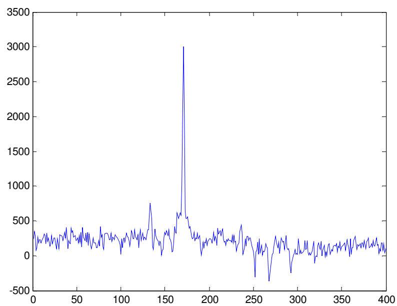
Figure 5.31 FRET signal
