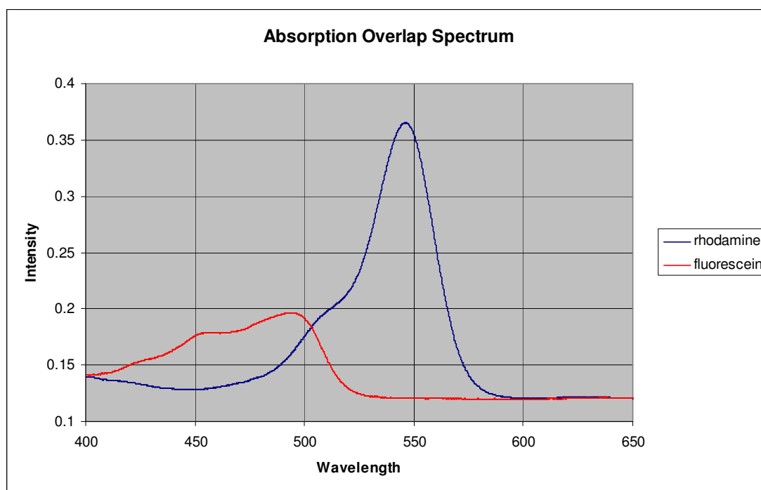
Figure 5.15 The overlap of absorption spectra of Rhodamine B 2 \mu\text{M} and Fluorescein Na 8 \mu\text{M}
