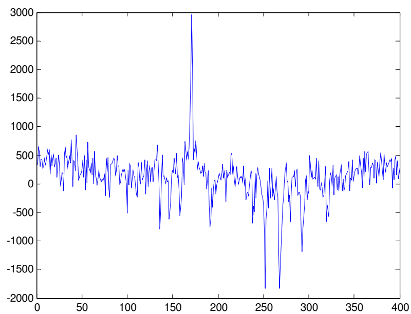
Figure 5.33 FRET signal
