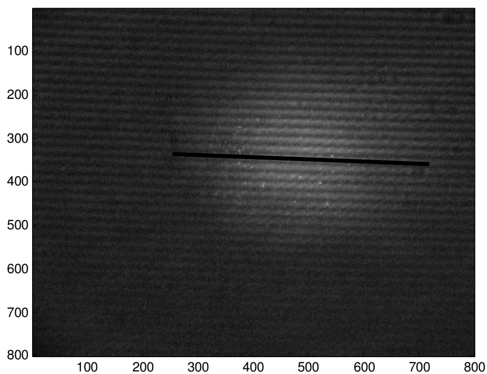
Figure 5.18 Profile line draw on donor acceptor sample
