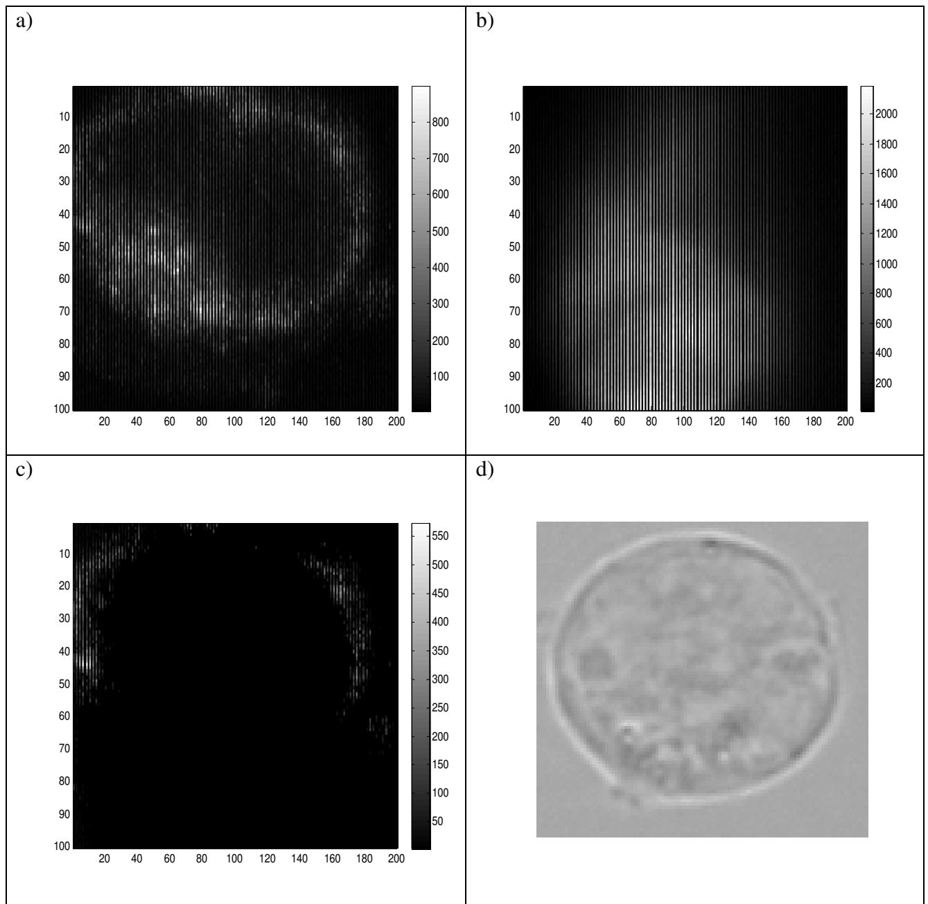
Figure 6.6 a) The confocal image of Melanopsin labeled with RFP b) Untransfected cell c) RFP tagged Melanopsin containing cell free of background light d) The transmission image of the cell.
