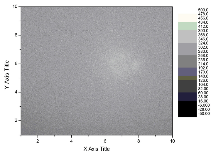
Figure 6.8b Donor Emission in a cell both transfected with both RFP-Mel and GFP-Cry
