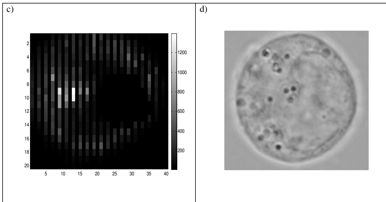
Figure 6.7 a) Cryptochrome labeled with GFP. b) Control cell. c) GFP tagged Cry cell free of background light. d) Transmission image of a cell with Cry labeled GFP
