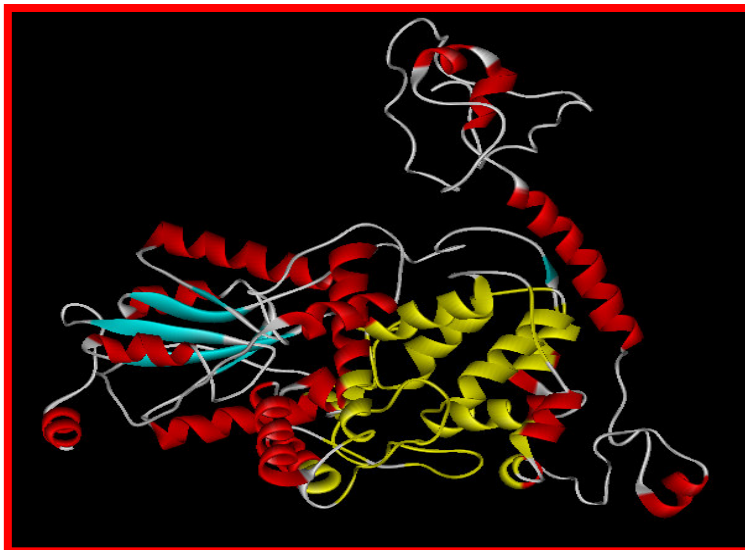
Figure 6.4 The binding of Melanopsin to the part of human Cry2 that is indicated by yellow color (by Evrim Besray Ünal, Koç University Computational Sciences and Eng. Department)
