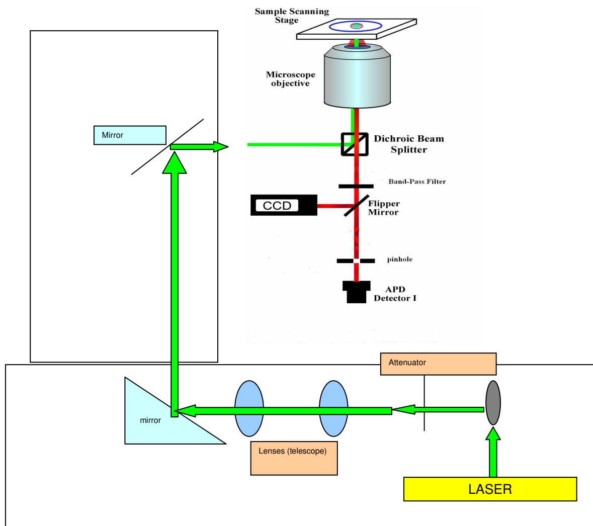
Figure 4.4 The set up of confocal microscopy
