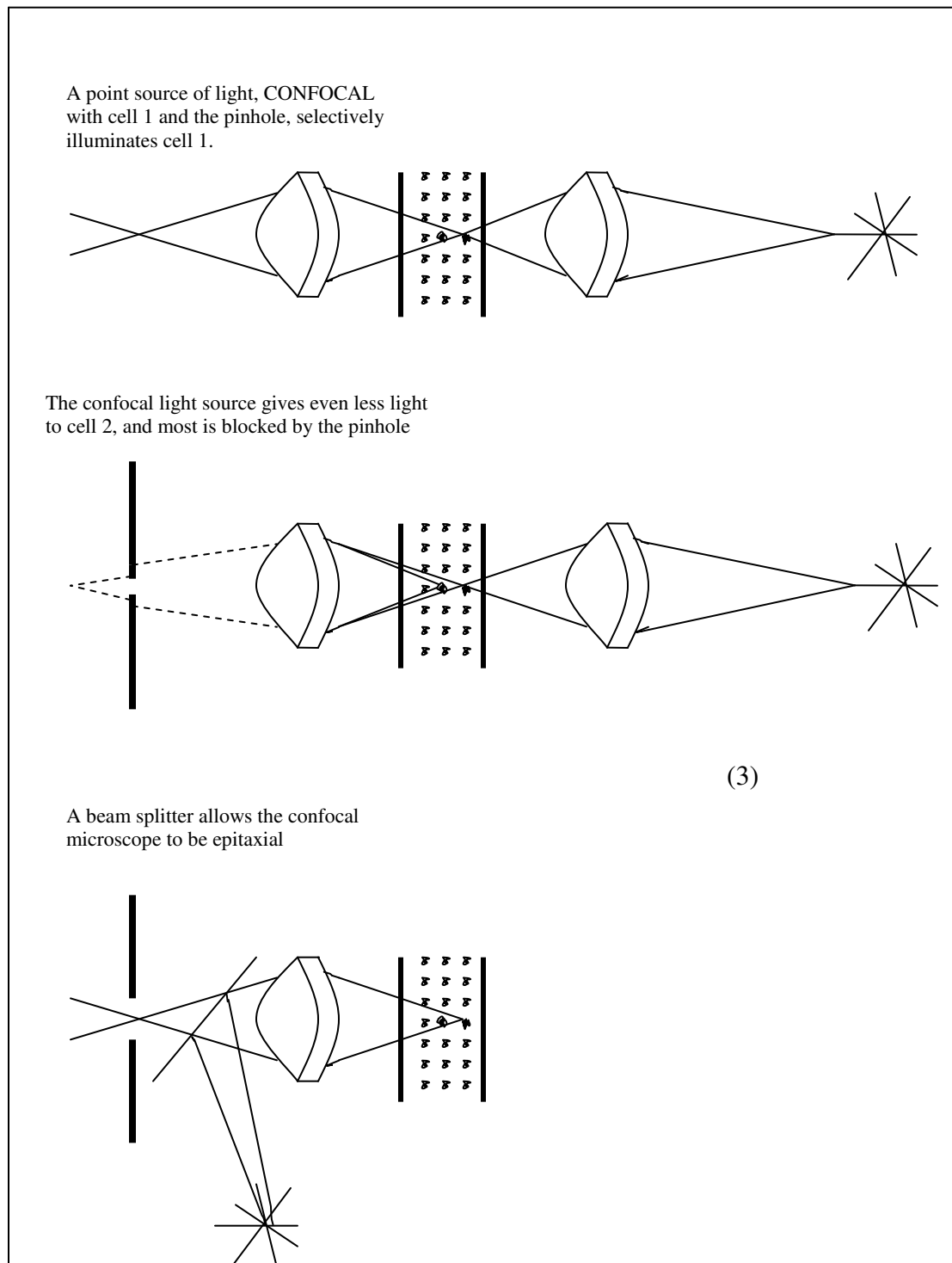
Figure. 3.2. A simple view of confocal microscope
