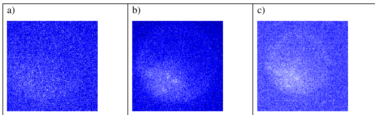
Figure 6.10 a) The image of donor and acceptor tagged molecules obtained with donor filter b) The image of donor and acceptor tagged molecules obtained with FRET filter c) The subtraction of donor emission from acceptor emission
