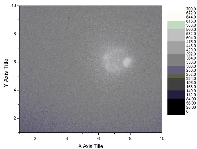
Figure 6.8a Acceptor emission in a cell both transfected with RFP-Mel and GFP-Cry
