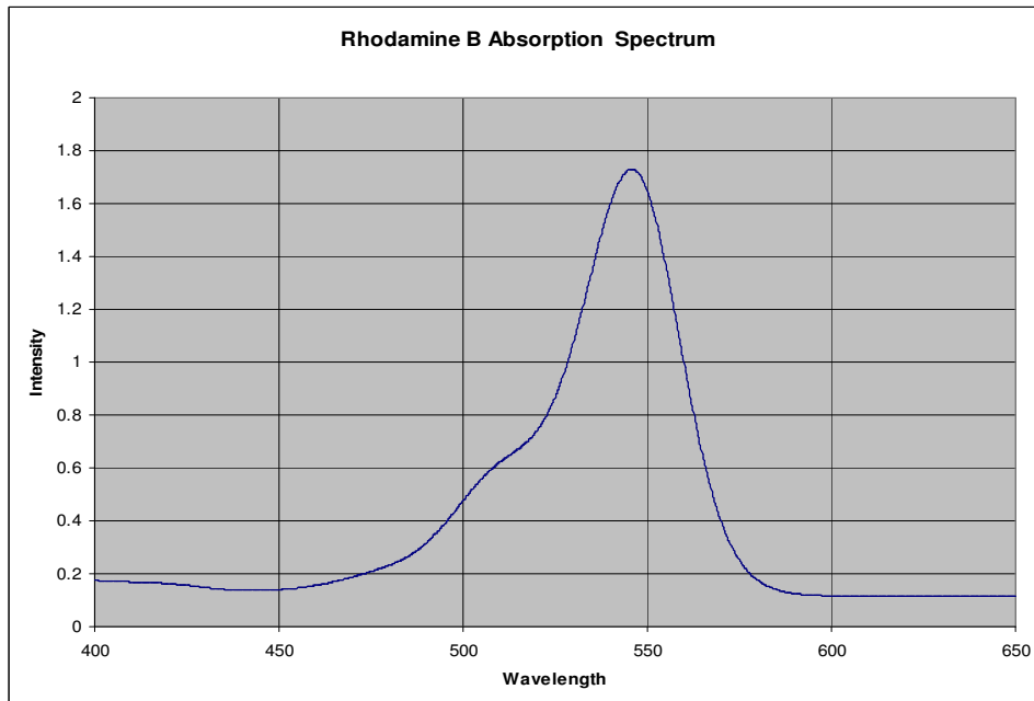
Figure 5.5 The absorption spectrum of Rhodamine B 20 μM in methanol
