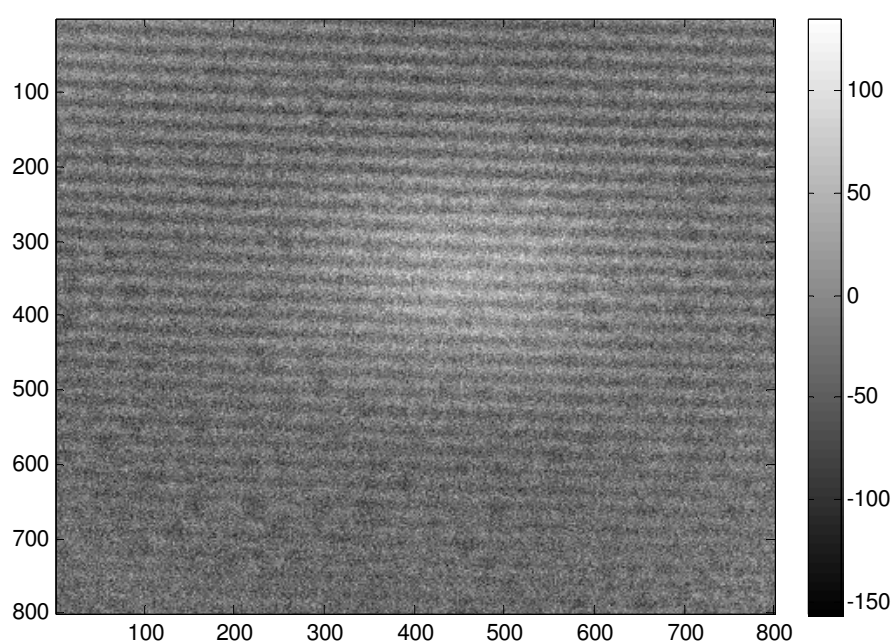
Figure 5.20 Donor bleed through in to FRET channel
