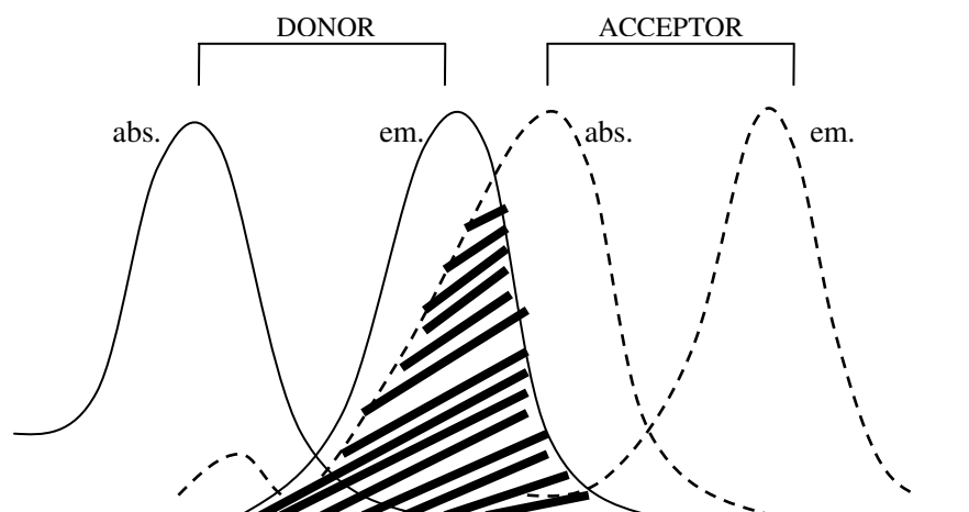
Figure 2.3. The spectral overlap between emission spectrum of the donor and the absorption spectrum of the acceptor
