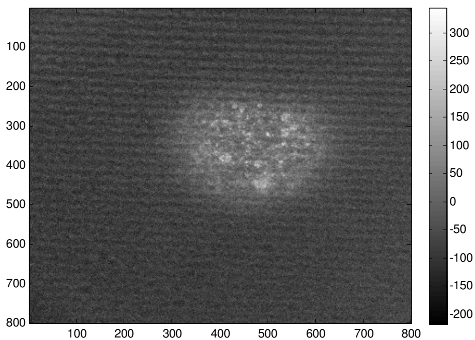
Figure 5.25 Acceptor emission with FRET filter
