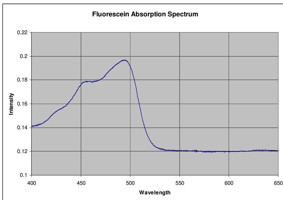
Figure 5.2 The absorption spectrum of Fluorescein 8 \mu\text{M} concentration in methanol
