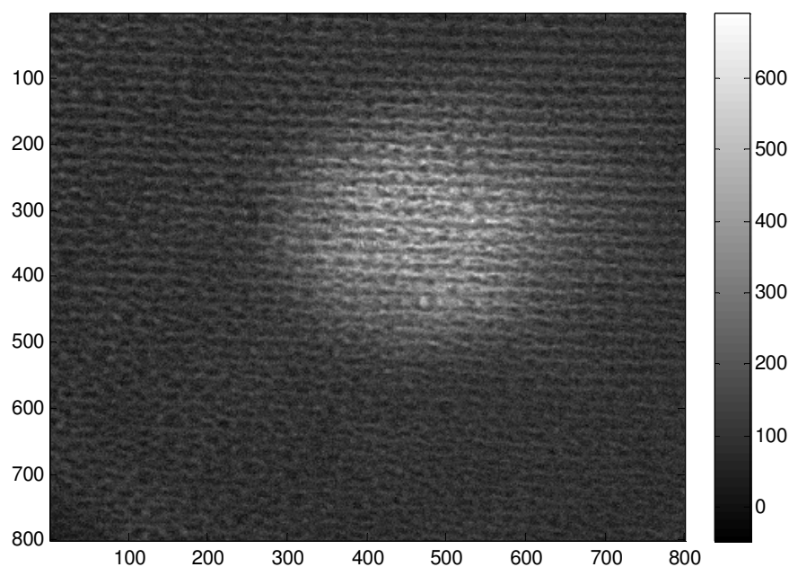
Figure 5.24 Acceptor emission with donor filter
