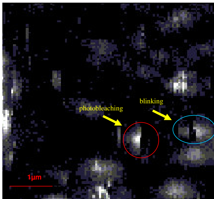
Figure 4.6. Photobleaching and blinking phenomena by confocal microscopy
