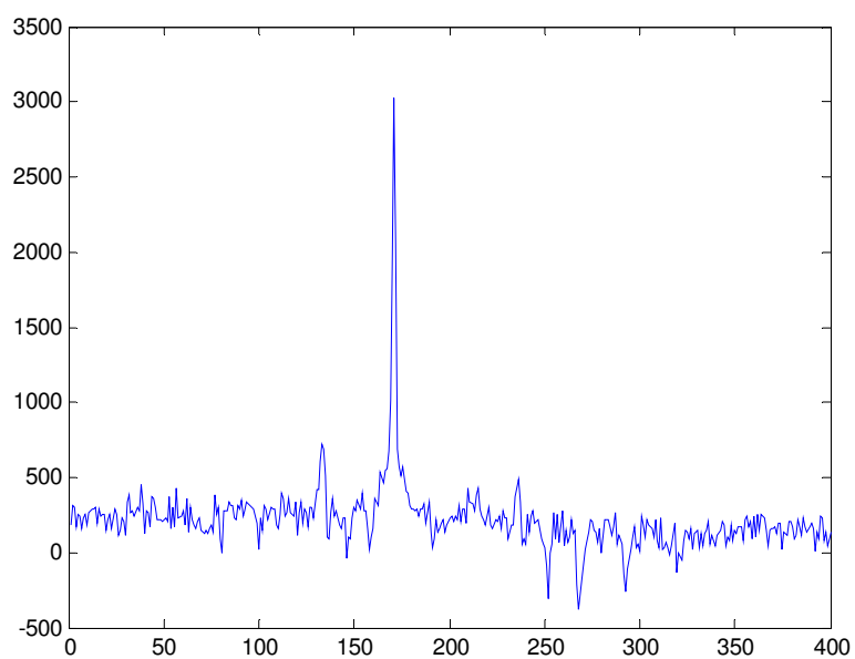
Figure 5.32 FRET signal
