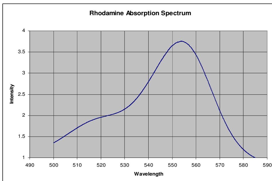
Figure 5.6 The absorption spectrum of Rhodamine B 25 \mu\text{M} in water
