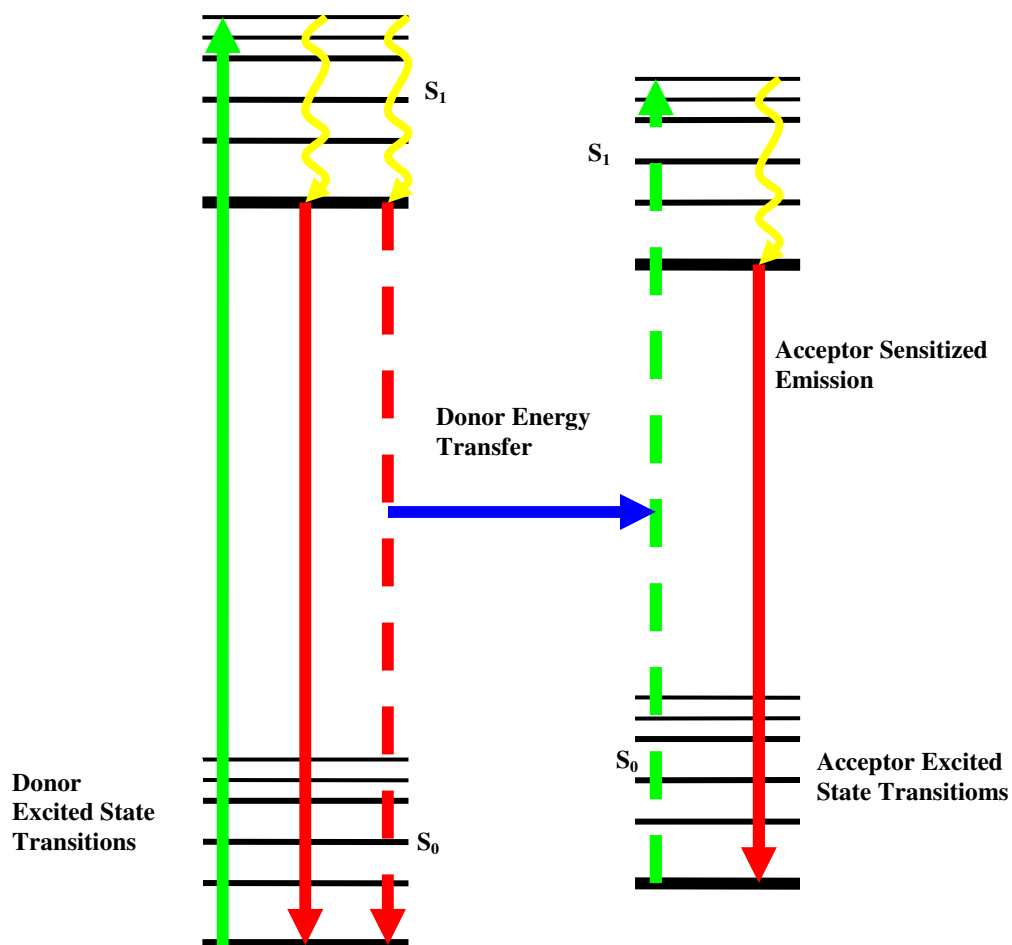
Figure 2.5 : Jablonski diagram illustrating the coupled transitions involved between the donor emission and acceptor absorbance in fluorescence resonance energy transfer
