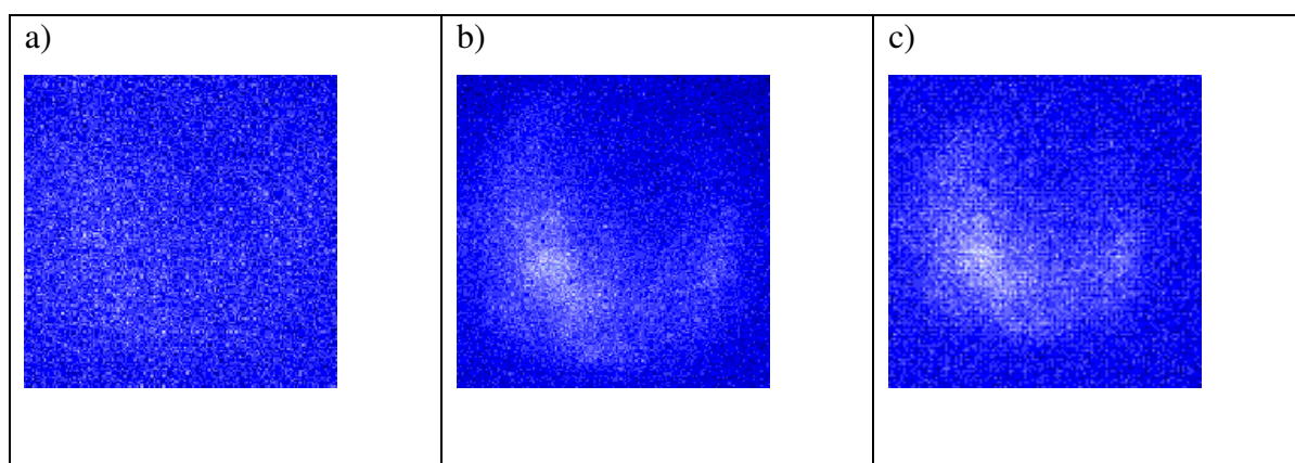
Figure 6.11 a) The image of donor and acceptor tagged molecules obtained with donor filter b) The image of donor and acceptor tagged molecules obtained with FRET filter c) The subtraction of donor emission from acceptor emission
