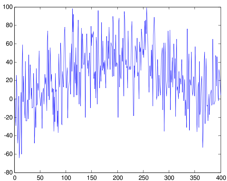
Figure 5.22 The intensity profile of donor emission in the range of acceptor
