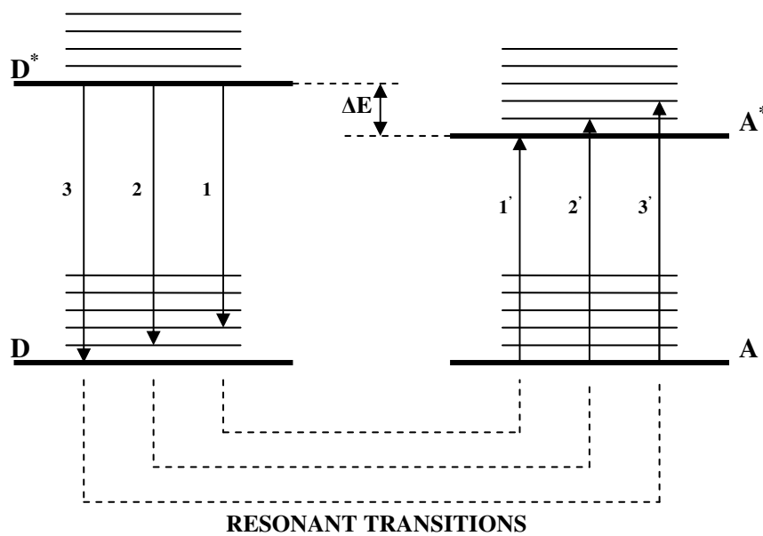
Figure 2.4. Coupled transitions in energy levels of donor and acceptor molecules
