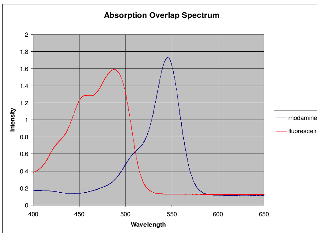
Figure 5.14 The overlap of the absorption spectra of Rhodamine B 20 \mu\text{M} and Fluorescein Na 80 \mu\text{M}
