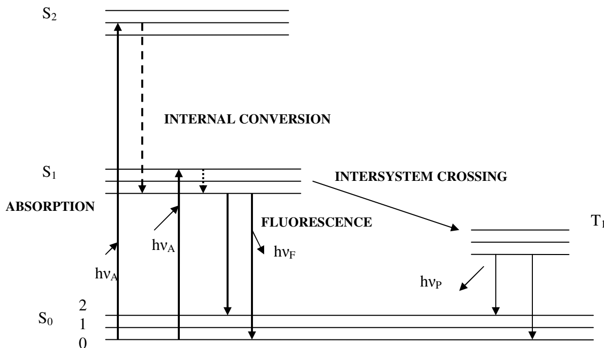
Figure 2.2. Jablonski Diagram
