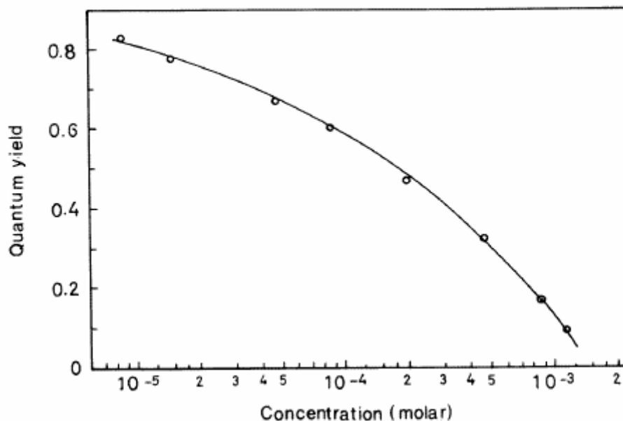
Figure 5.1 The variation in quantum yield of rhodamine B in methanol with concentration [29]
