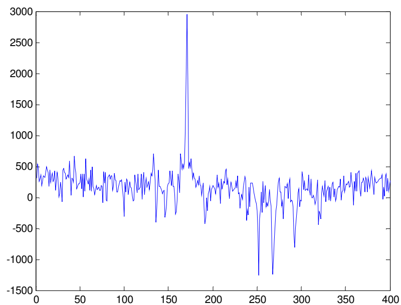
Figure 5.35 FRET signal
