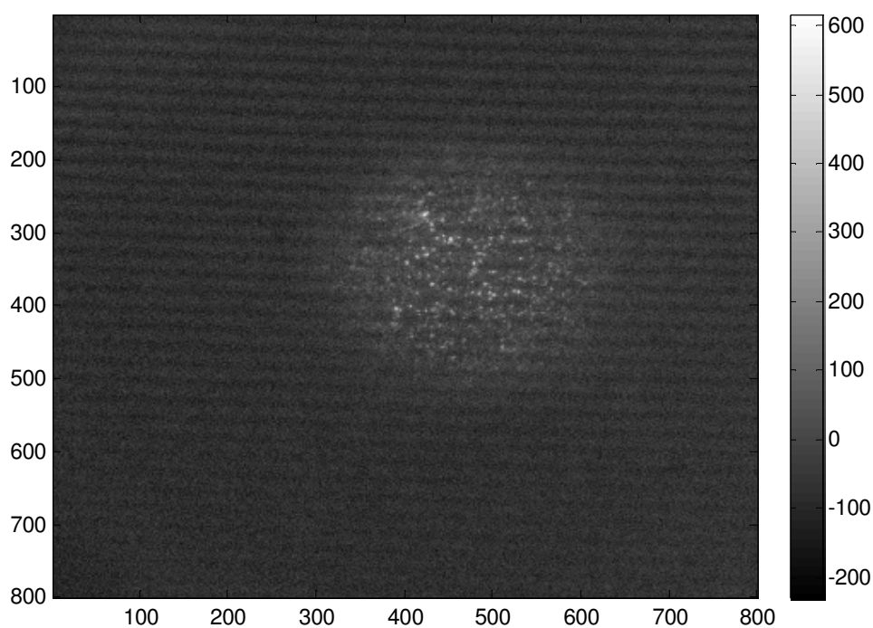
Figure 5.26 Acceptor emission from donor and acceptor sample
