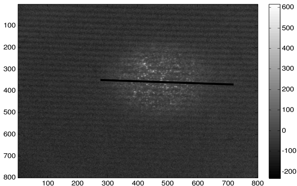
Figure 5.27 Profile line on sample containing donor and acceptor
