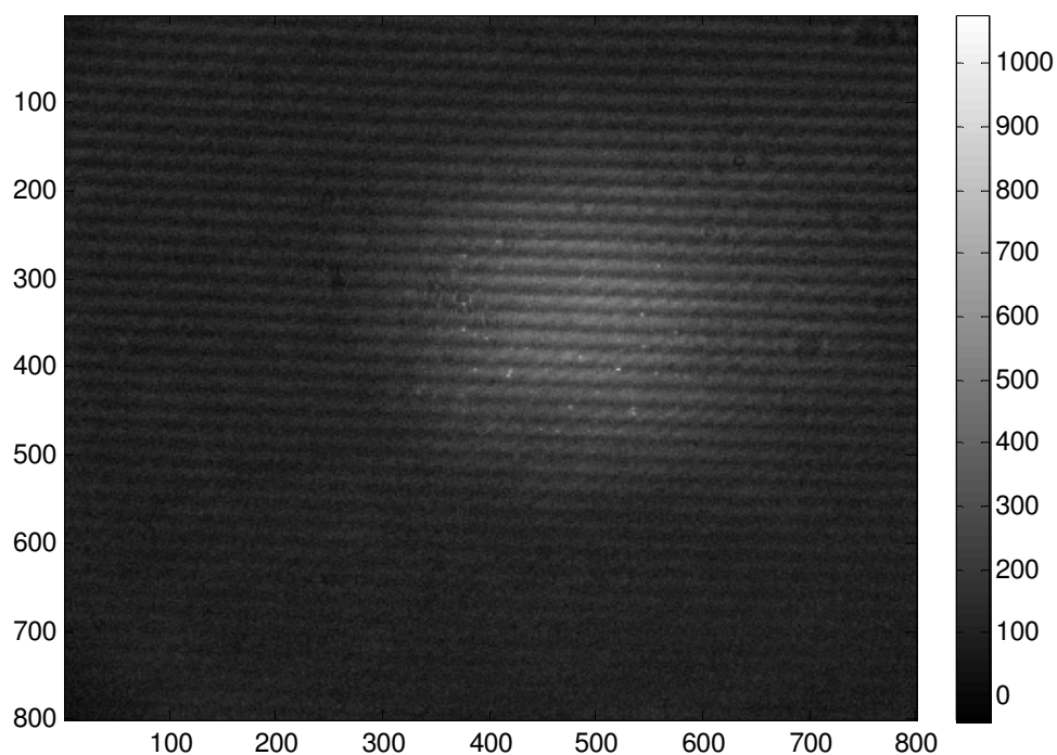
Figure 5.17 Donor emission from sample containing donor and acceptor
