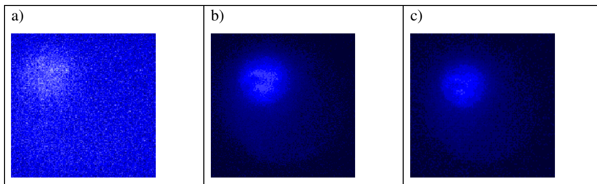
Figure 6.12 a) The image of donor and acceptor tagged molecules obtained with donor filter b) The image of donor and acceptor tagged molecules obtained with FRET filter c) The subtraction of donor emission from acceptor emission
