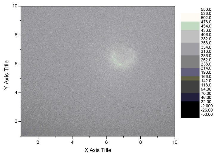
Figure 6.9b Donor Emission in a cell both transfected with both RFP-Mel and GFP-Cry
