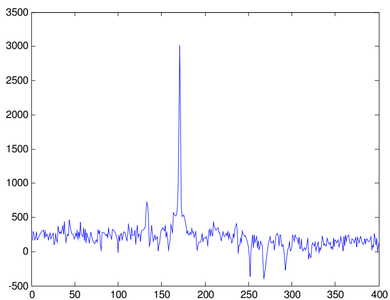
Figure 5.30 FRET signal
