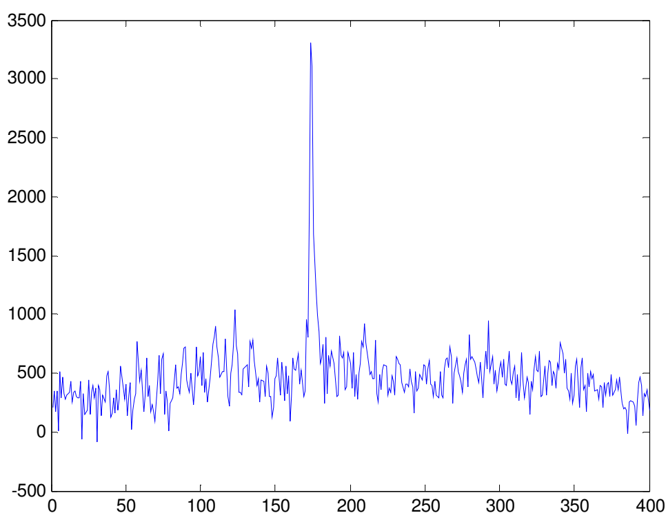
Figure 5.23 Extracted acceptor profile
