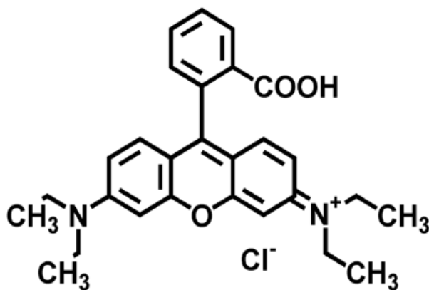
Figure 5.13 Rhodamine B
