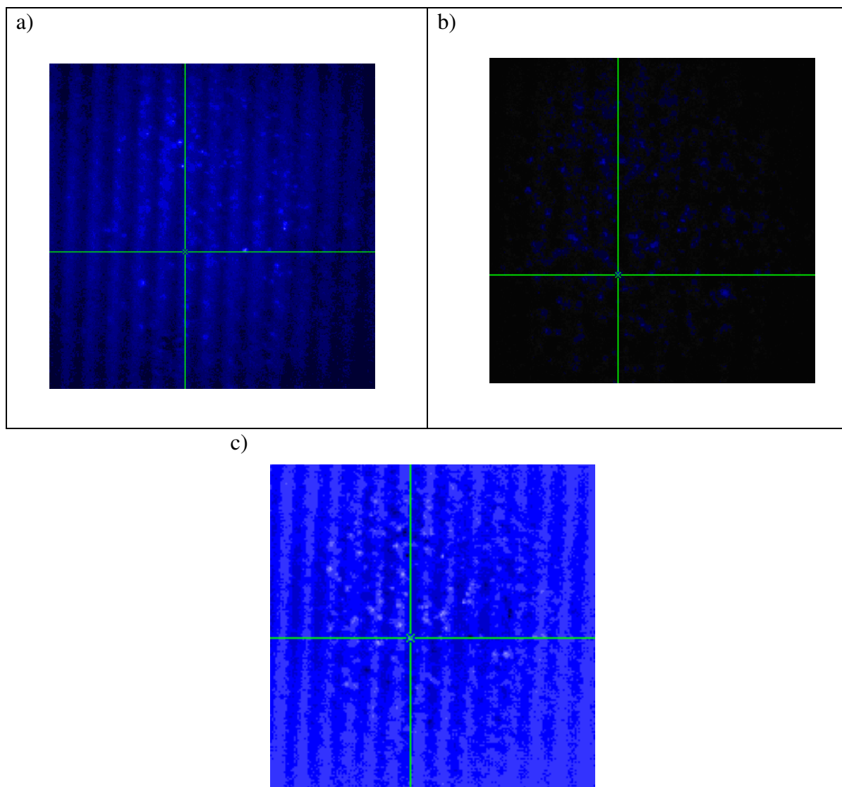
Figure 5.16 a) Fluorescence intensity image of a sample containing donor and acceptor molecules obtained by donor filter b) Fluorescence intensity image of the sample containing the mixture of donor and acceptor fluorophores obtained by fret filter c) The subtraction of donor fluorescence from acceptor fluorescence.
