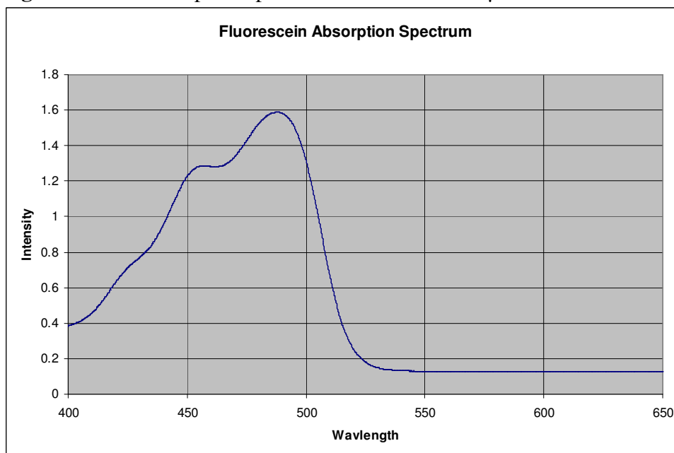
Figure 5.3 The absorption spectrum of Fluorescein 80 \mu\text{M} concentration in methanol
