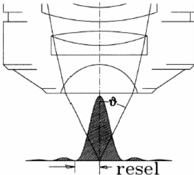
Figure 3.3. The resolution element due to a lens of NA = n \sin \theta is called a resel: the radius of the first dark fringe in the diffraction pattern, or half the diameter of the Airy disc [13]
