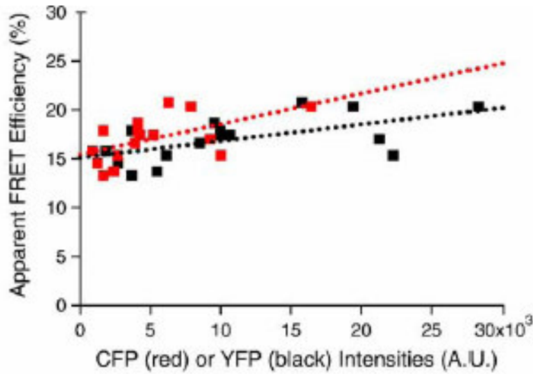
Figure 5.8 Non-Specific FRET CFP(donor) and YFP(acceptor)[32]
