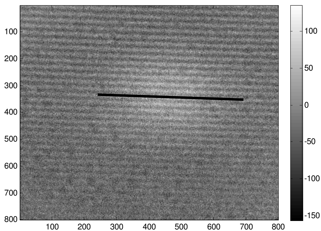
Figure 5.21 Profile line on donor sample
