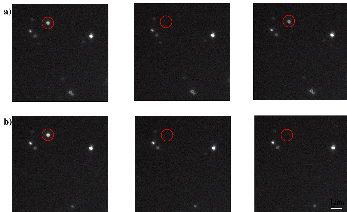
Figure 4.7. a) Blinking phenomenon b) photobleaching phenomenon by wide field microscopy
