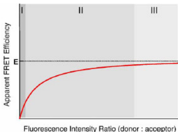
Figure 5.9 FRET efficiency versus donor:acceptor concentration ratio [32]
