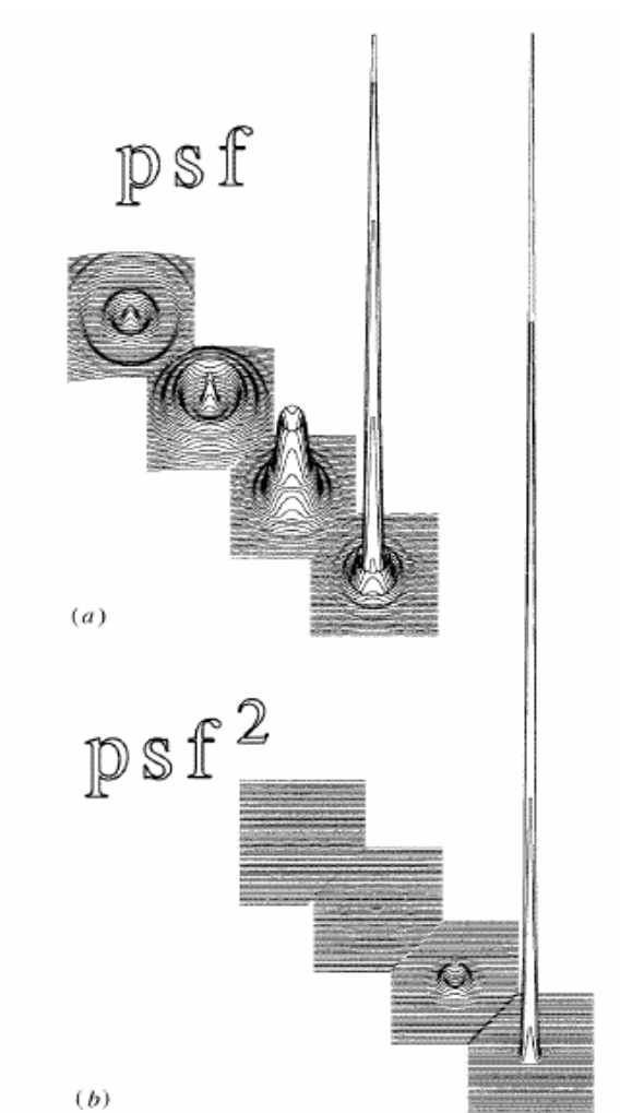
Figure 3.4. (a) conventional diffraction pattern, and in (b) it is for the confocal case [13].
