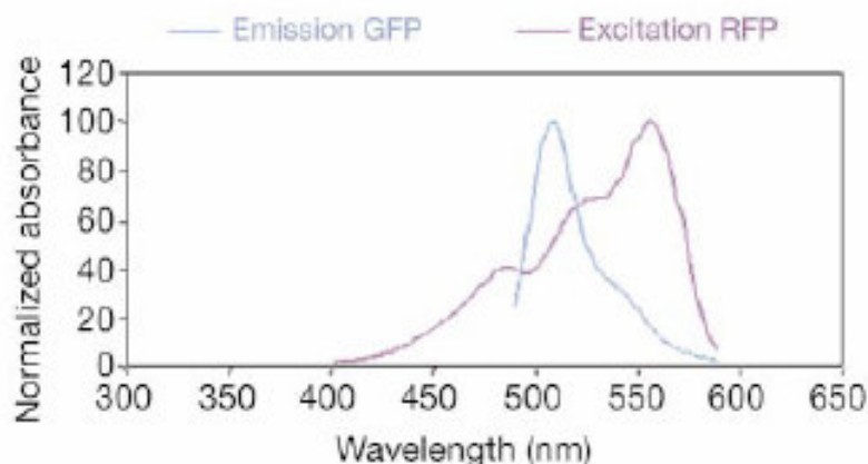
Figure 6.5 The spectral overlap of donor emission and acceptor absorption
