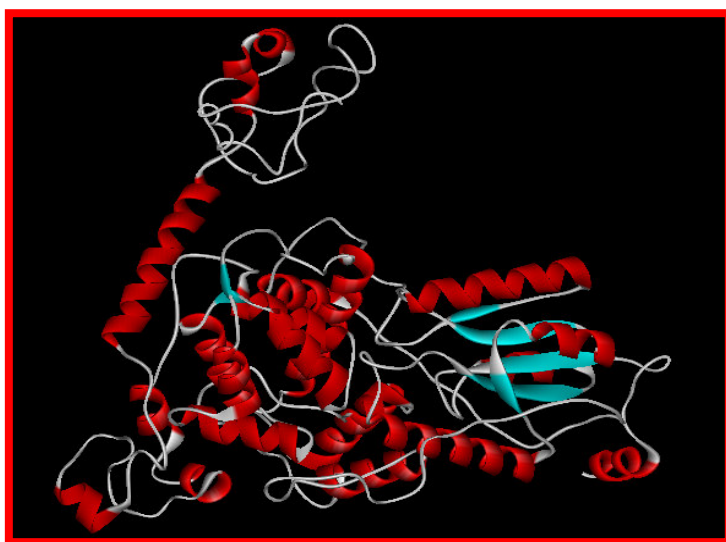
Figure 6.2 The computational modelling of human cryptochrome2 (by Evrim Besray Ünal Koç University Computational Sciences and Eng. Department)
