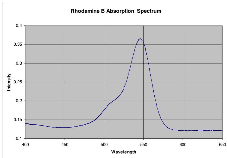
Figure 5.4 The absorption spectrum of Rhodamine B 2 μM in methanol
