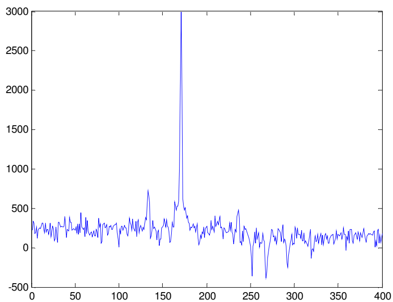
Figure 5.34 FRET signal
