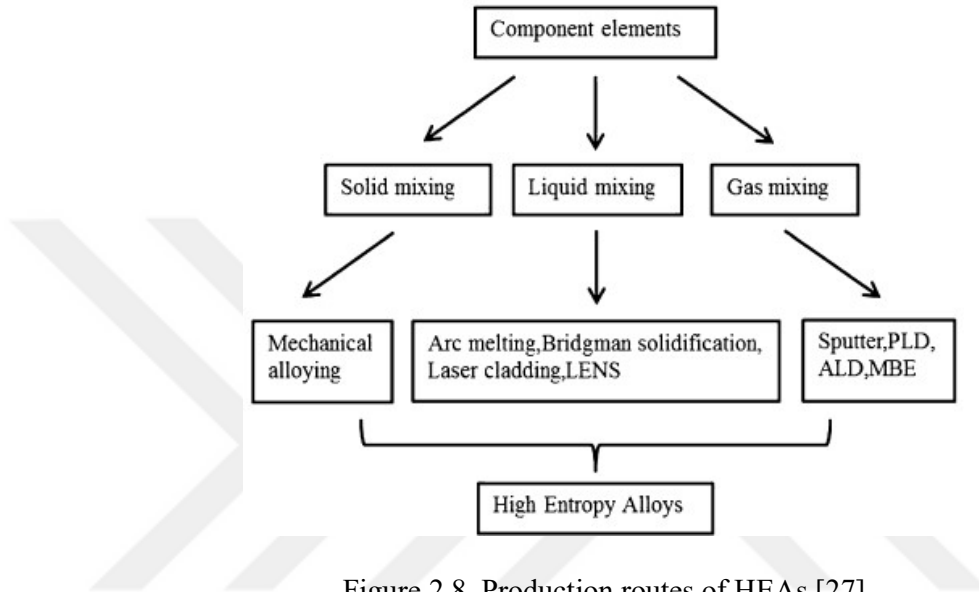
Figure 2.8. Production routes of HEAs [27]
