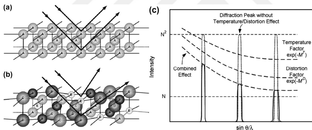
Figure 2.4. Effect of lattice distortion on XRD intensities a) perfect lattice consist of the same atoms, b) distorted lattice due to the different atoms with various radii, c) effect of temperature and lattice distortion on XRD intensities [20]
