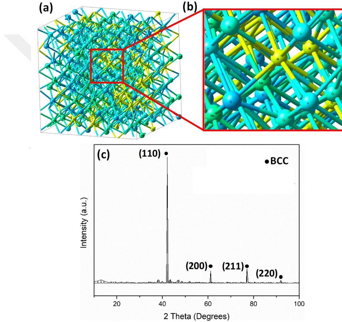
Figure 4.7. VASP simulation of AlTiVCrMn LWHEA; a) 4x4x4 simulation box, b) Zoom-in view of BCC crystal structure, c) Simulated XRD pattern based on atom positions obtained from VASP simulation
