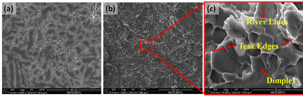
Figure 5.7. SEM images of \text{Cu}_{35}\text{Ni}_{25}\text{Al}_{20}\text{Ti}_{20} MEA a) annealed at 600 °C for 90 min. (4000x), b) fracture surface after compression test (1000x), c) Zoom-in view of the fracture surface (15000x)
