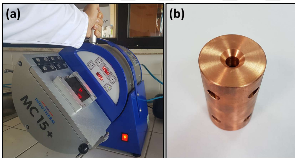
Figure 3.5. a) MC 15 Induction melter, molds adapted to the melter, b) copper mold
