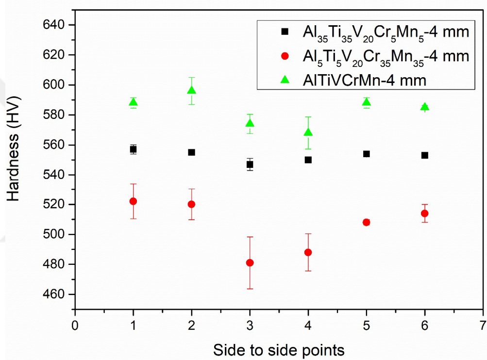
Figure 4.13. Hardness values of 4 mm AlTiVCrMn, Al 35 Ti 35 V 20 Cr 5 Mn 5 , and Al 5 Ti 5 V 20 Cr 35 Mn 35 cylindrical LWHEAs
