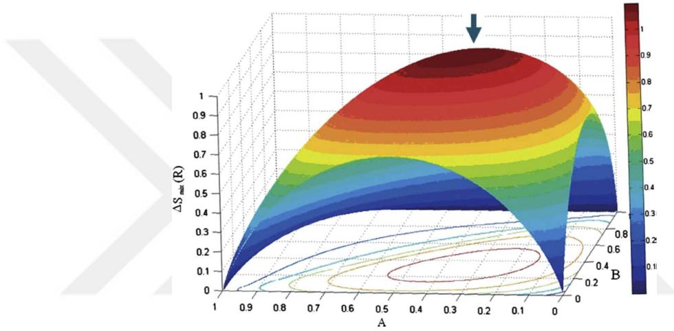
Figure 2.2. The change of \Delta S_{\text{mix}} with changing composition for a ternary system [16]
