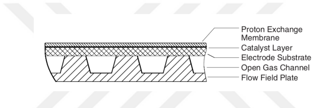
Figure 1.9. Cross-section of MEA in contact with the electrode substrate and open gas channels [16] .
