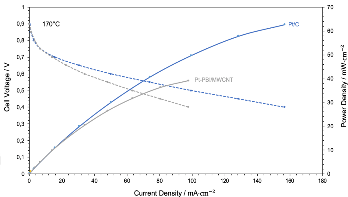
Figure 5.14. Voltage, current & power density curves of Pt-PBI/MWCNT and reference Pt/C at 170 °C.
