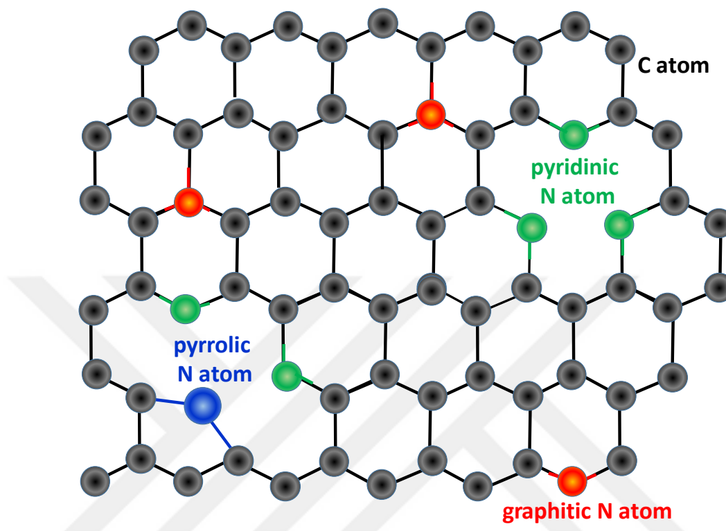
Figure 2.2. Schematic demonstration of graphitic-N, pyridinic-N, and pyrrolic N.
