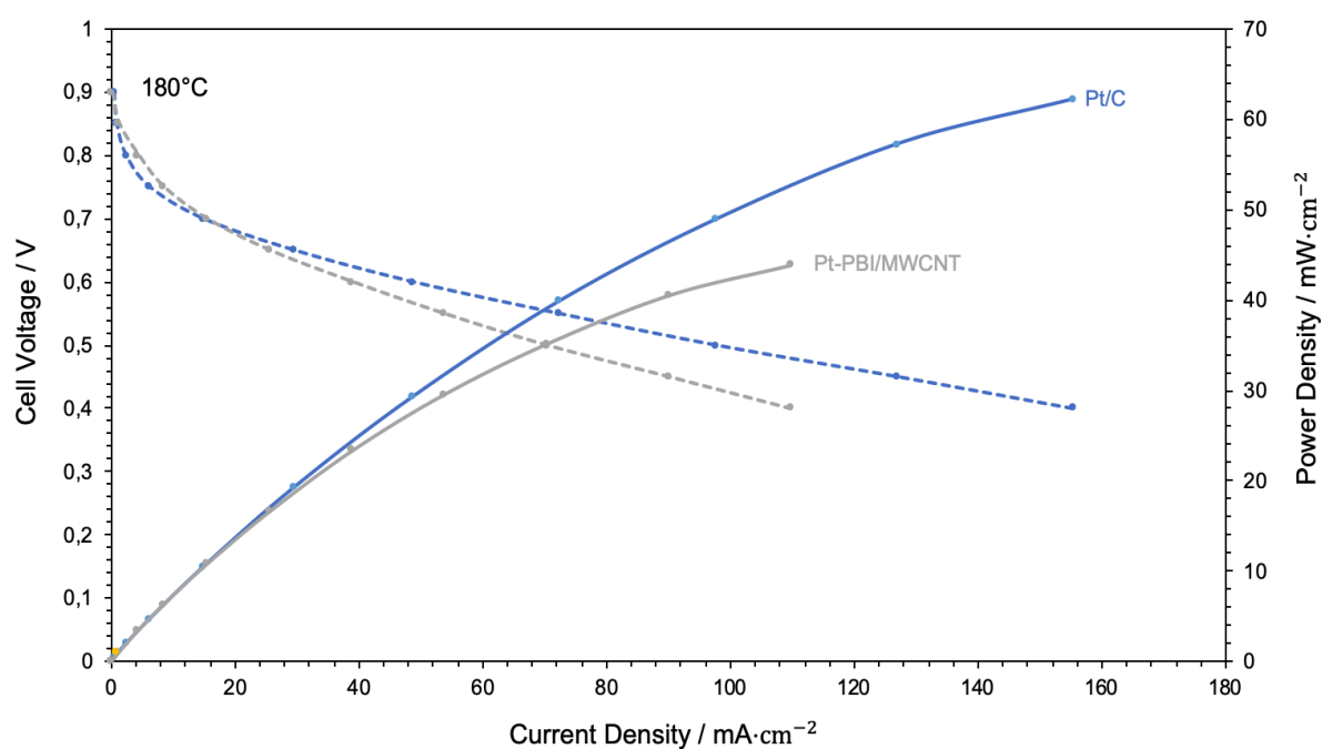
Figure 5.15. Voltage, current & power density curves of Pt-PBI/MWCNT and reference Pt/C at 180 °C.
