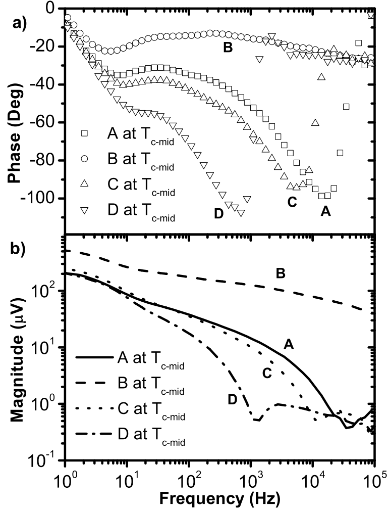
Figure 3.1: Phase (a) and magnitude (b) of the IR response vs. frequency of bolometers A, B, C, and D on 1 mm thick SrTiO 3 substrate at T_{c-mid} . The effect of the separation distance on the response is clearly observed.
