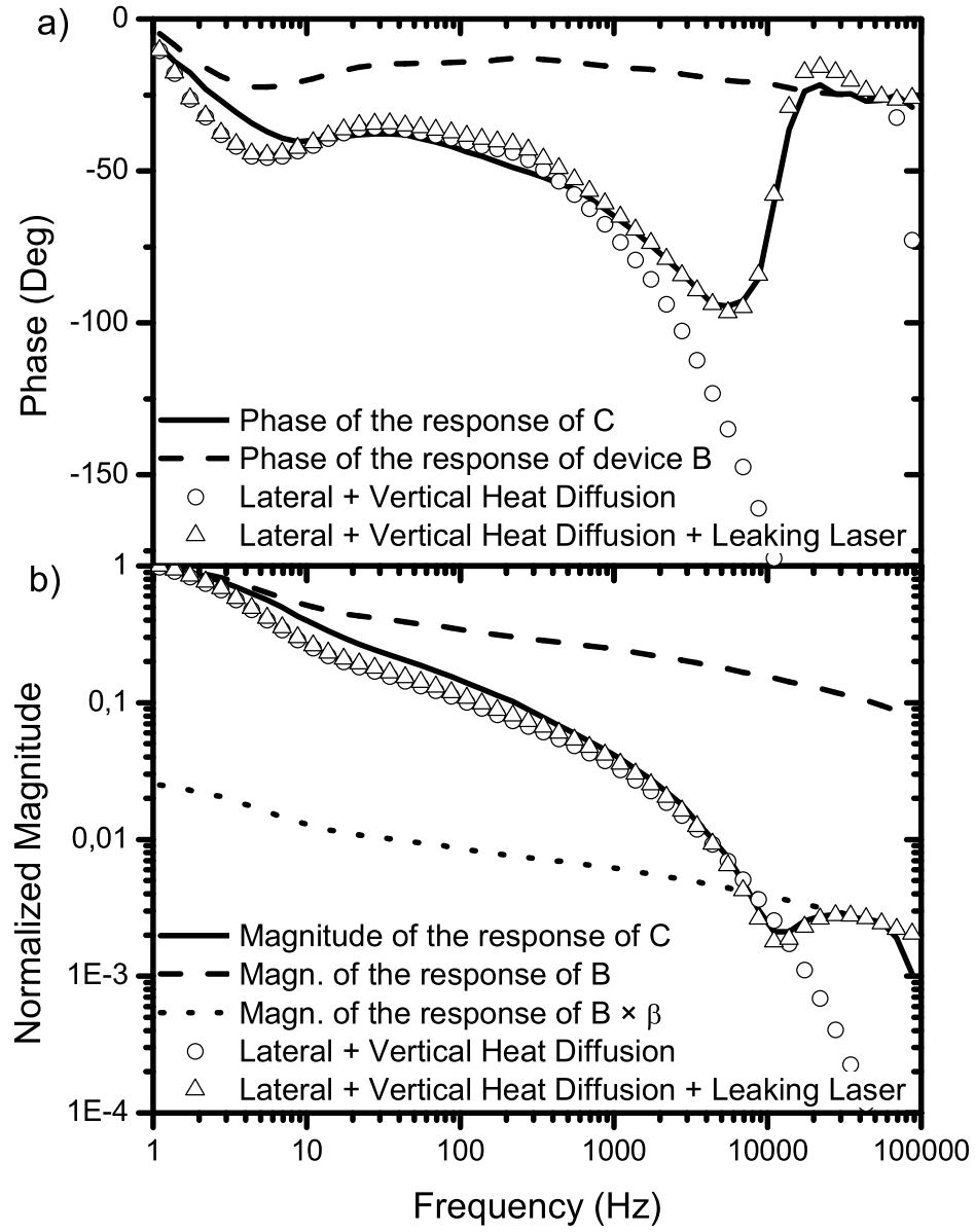
Figure 4.4: Measurement results of the response of device B (---) and C (—) and analytical model without (○) and with (△) leaking laser effect. (· · ·) shows the magnitude of device B multiplied by the transparency ( \beta ) of the mask.
