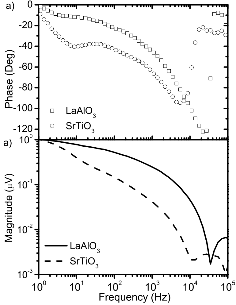
Figure 3.7: a) Phases and b) magnitudes of devices C on \text{LaAlO}_3 and \text{SrTiO}_3 substrates and their fitting curves.
