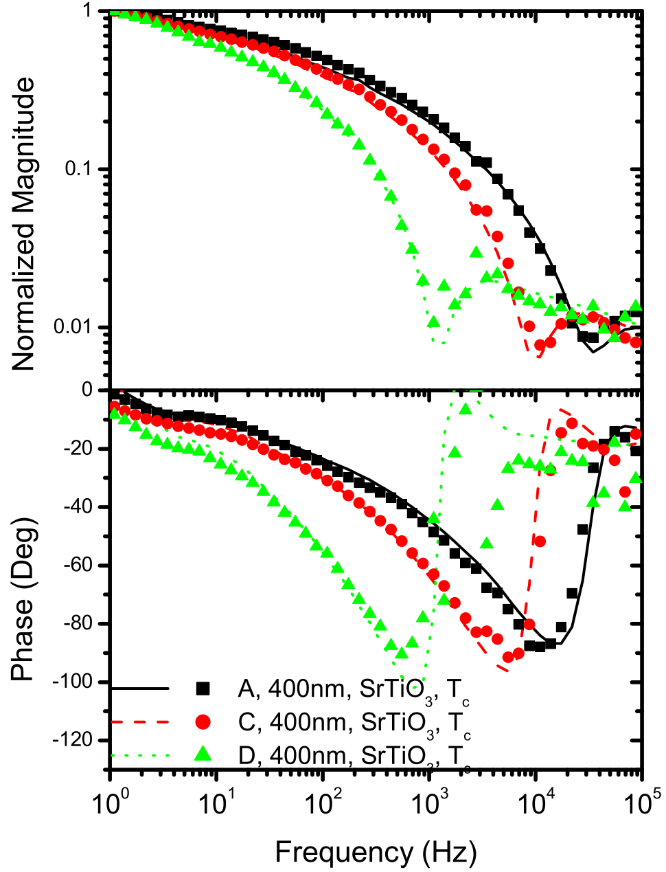
Figure 4.5: Verification of the model with the sense devices of different distances from the source device. (Table I rows 7, 8, 9) Scatter plots show the experimental data, line plots show the results of analytical model
