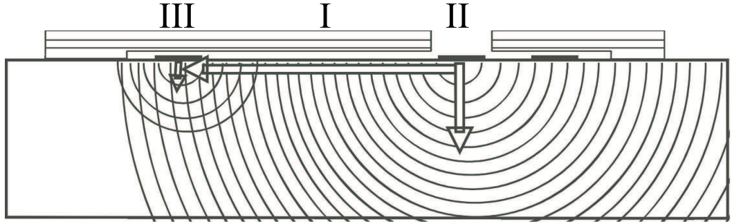
Figure 4.2: Three main parts of the analytical model: i) effect of the lateral heat diffusion, ii) effect of the vertical heat diffusion iii) effect of the leaking input laser
