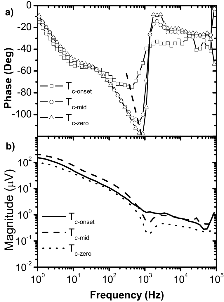
Figure 3.3: Phase (a) and magnitude (b) of the IR response vs. frequency of the sense bolometer, D on 1 mm thick \text{SrTiO}_3 substrate. The data is taken at three different temperatures: T_{c-zero} , T_{c-mid} , and T_{c-onset} .
