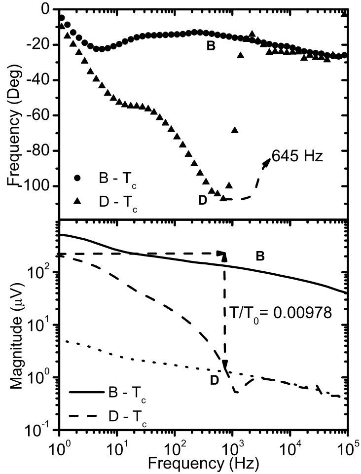
Figure 4.1: Obtaining the numeric values for the simple model from experimental data.
