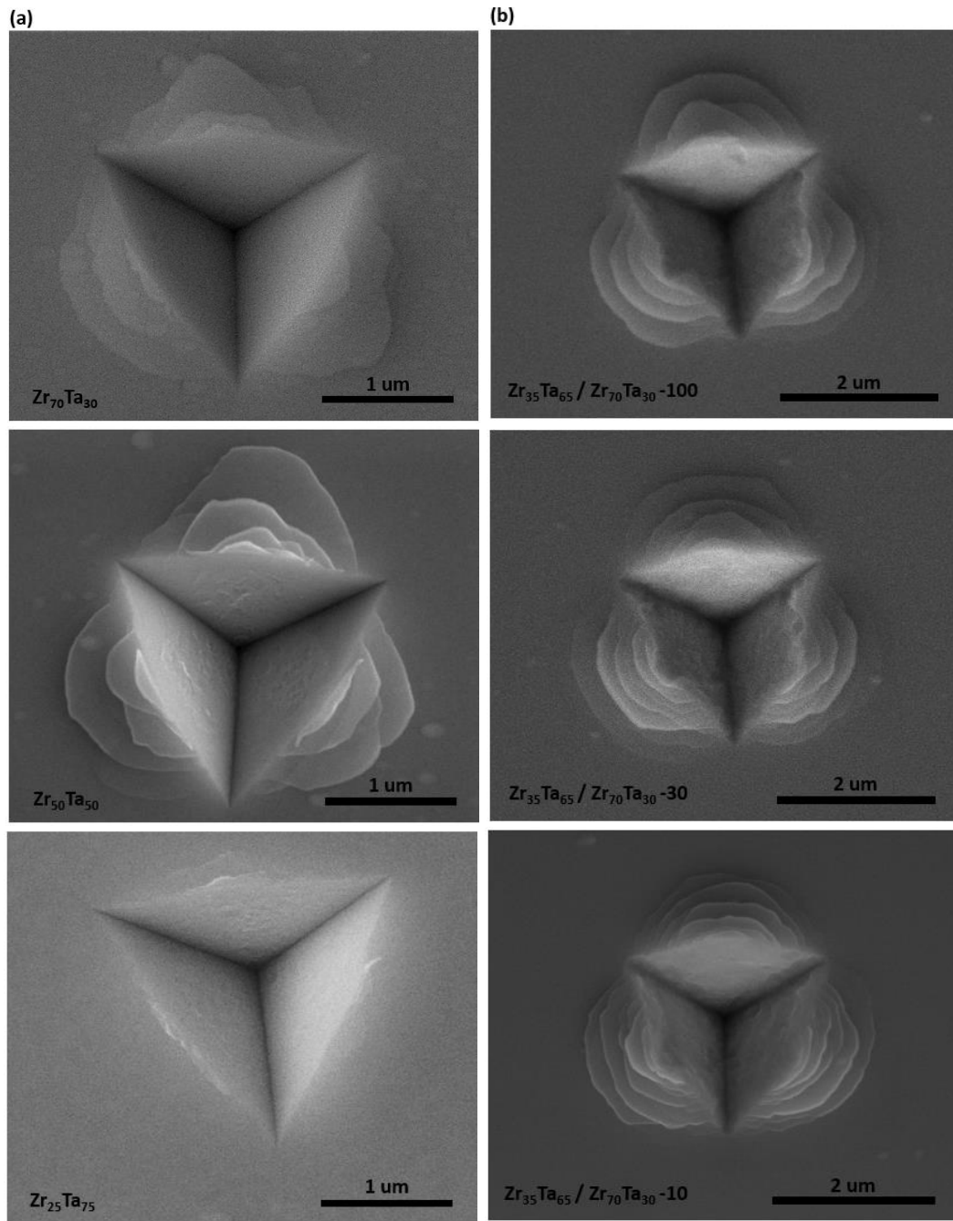
Figure 30. (a) SEM images of cube corner indentations on \text{Zr}_{25}\text{Ta}_{75} , \text{Zr}_{50}\text{Ta}_{50} , and \text{Zr}_{70}\text{Ta}_{30} monolithic samples. (b) SEM images of cube corner indentation on \text{Zr}_{35}\text{Ta}_{65}/\text{Zr}_{70}\text{Ta}_{30} nanolayers with different layer thicknesses.
