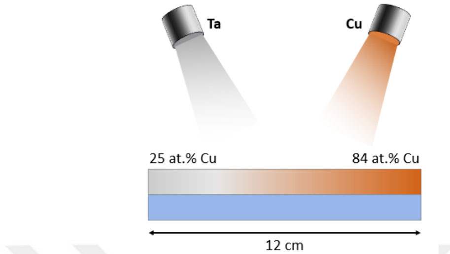
Figure 32. Schematic view of combinatorial sputtering for the CuTa study.
