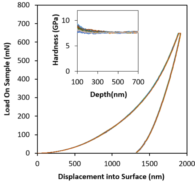
Figure 24. Load-displacement data of \text{Zr}_{50}\text{Ta}_{50} at 15 different locations. The inset indicates the hardness as a function of indentation depth for the same.
