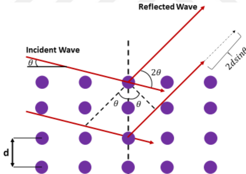
Figure 9. Illustration of Bragg's Law [79].
