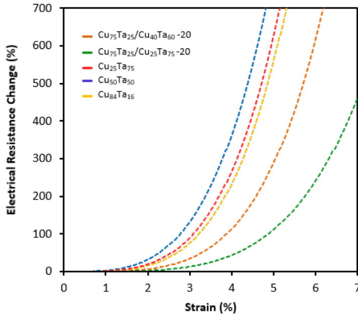
Figure 42. Electrical resistance versus strain for \text{Cu}_{84}\text{Ta}_{16} , \text{Cu}_{50}\text{Ta}_{50} , \text{Cu}_{25}\text{Ta}_{75} , \text{Cu}_{75}\text{Ta}_{25}/\text{Cu}_{40}\text{Ta}_{60} -20 and \text{Cu}_{75}\text{Ta}_{25}/\text{Cu}_{25}\text{Ta}_{75} -20 samples.
