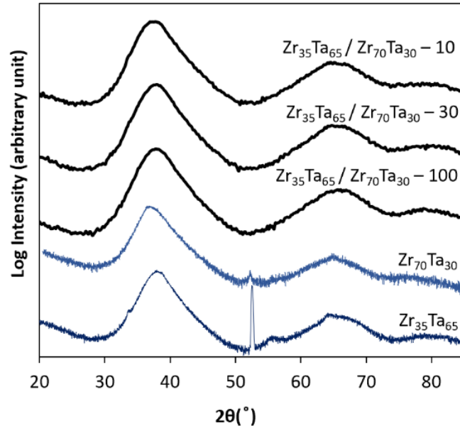
Figure 21. XRD patterns of ZrTa nanolayers and monolithic ZrTa.
