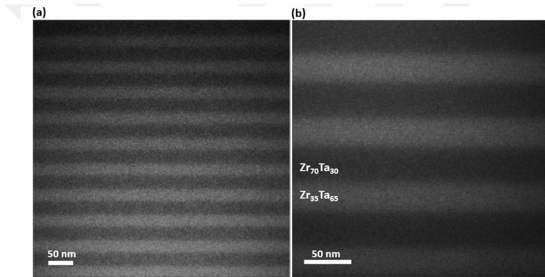
Figure 23. Cross-sectional bright-field TEM images of the nanolayered sample \text{Zr}_{35}\text{Ta}_{65}/\text{Zr}_{70}\text{Ta}_{30} – 30.
