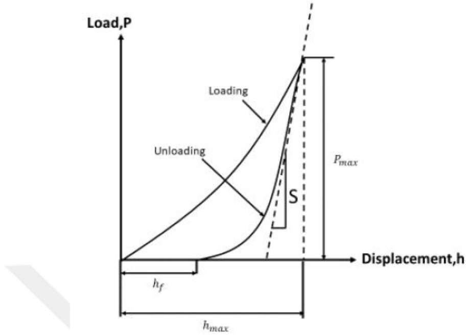
Figure 12. The schematic of a load-displacement curve for indentation [46].
