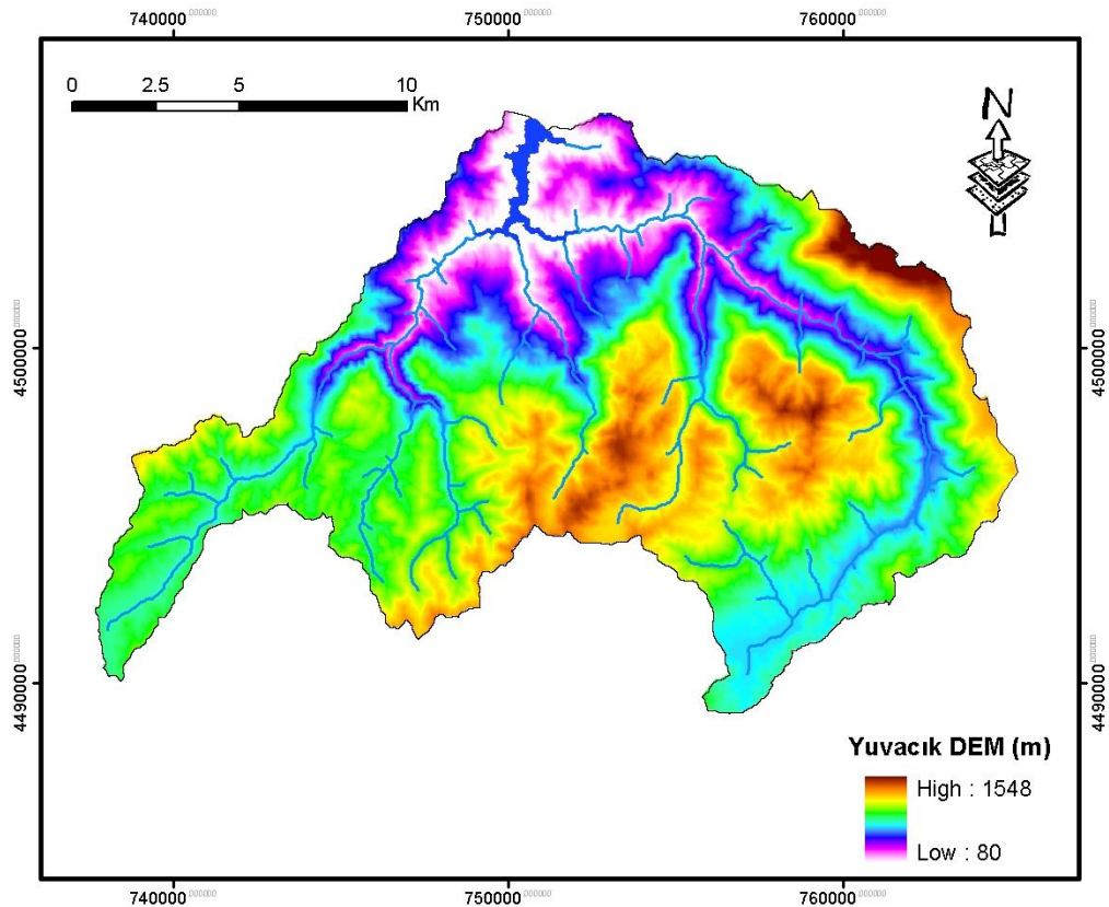
Figure 3.3 Digital Elevation Model (DEM) of Yuvacık Basin
