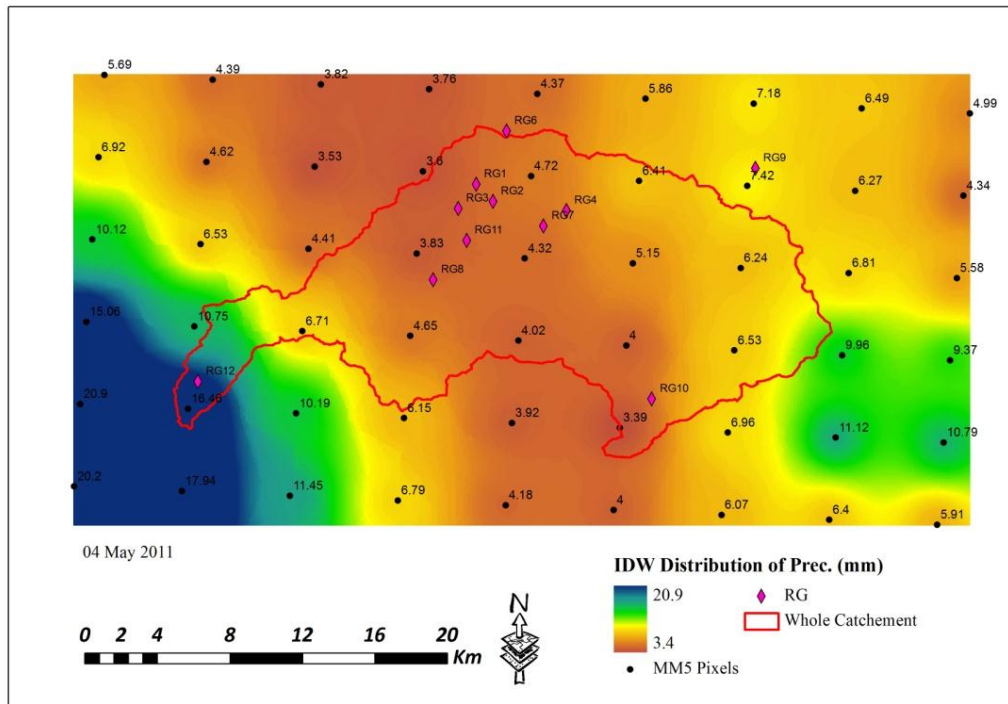
Figure 5.14 MM5 total precipitation distribution for 04 May 2011
