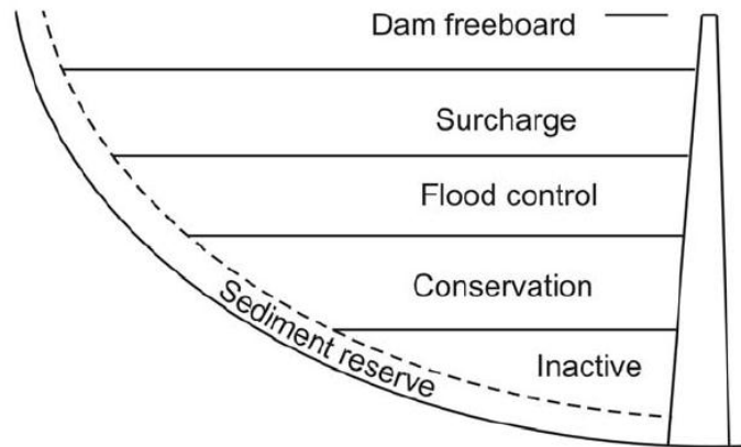
Figure 4.1 Reservoir pools (Wurbs 2005)
