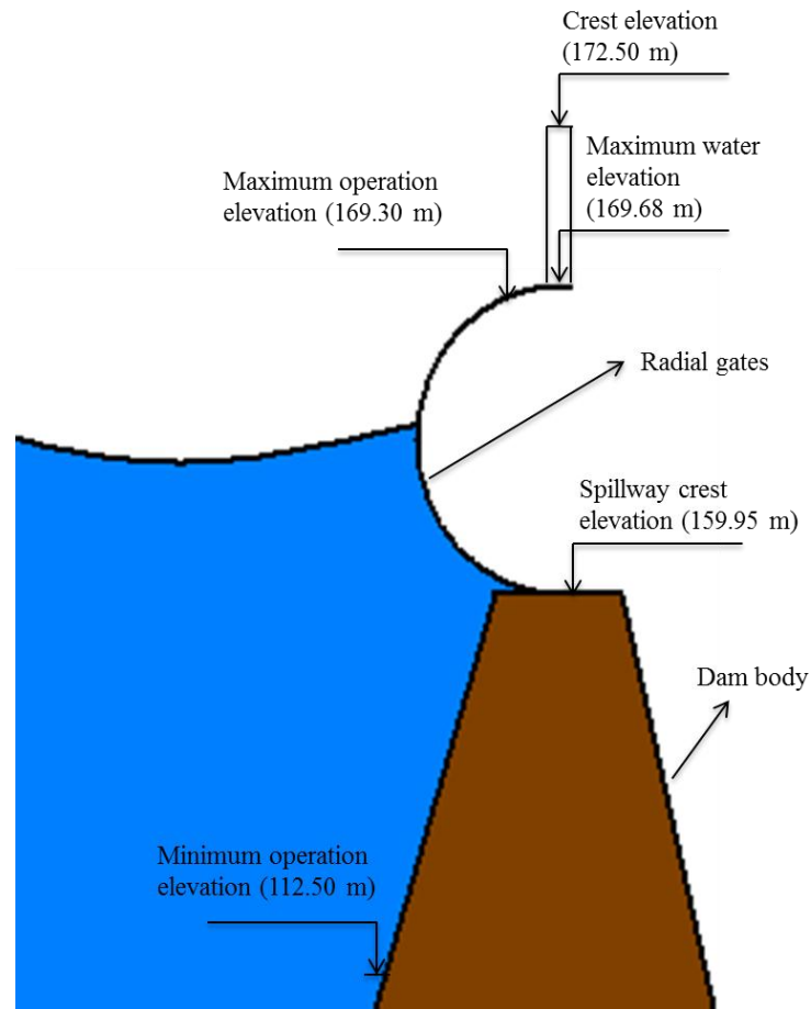
Figure 6.2 Critical elevations for reservoir operation
