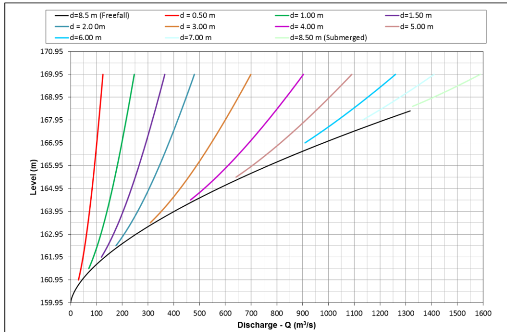
Figure 5.4 Spillway discharge curve for four gates with respect to different gate openings (DSI 1983)
