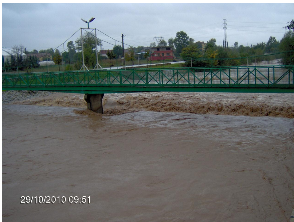
Figure 3.16 Downstream channel section at 7+800 km
