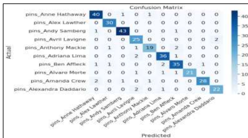
Figure 4.24: CM of LR.
