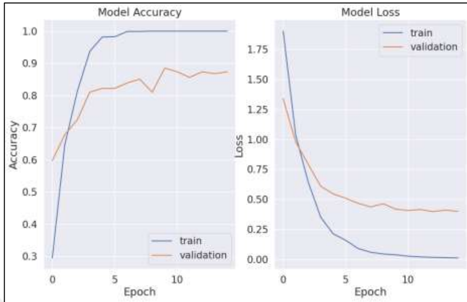
Figure 4.1: Accuracy and Loss Of ANN Model.
