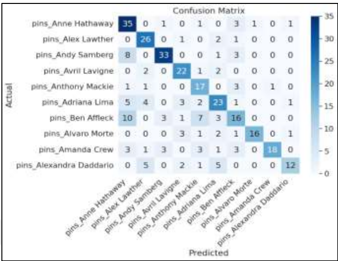
Figure 4.20: CM of KNN.
