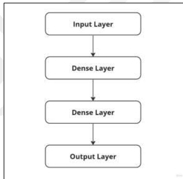
Figure 3.3: ANN Architecture.
