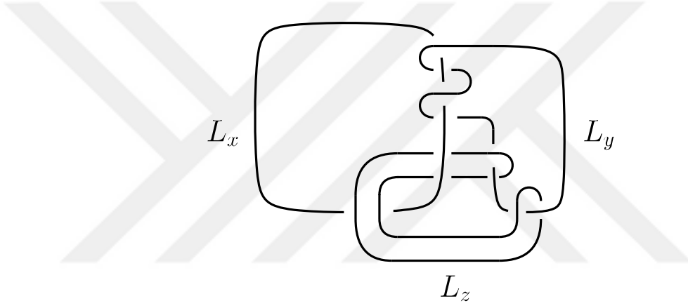
Figure 4.6. The link U_{022} , with linking numbers 0, 2, and 2. The difference from Figure 3.3 is at the lower right crossing.
