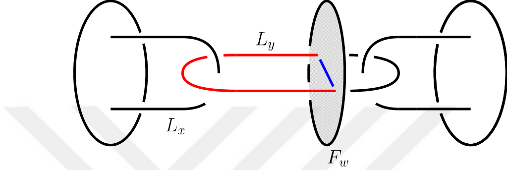
Figure 4.4. The core of the handle is shown in red while blue is the arc connecting the feet.
