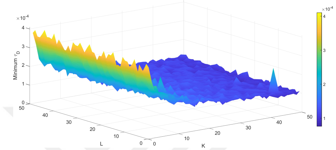
Figure 2.14: The minimum dwell time for different K and L values.
