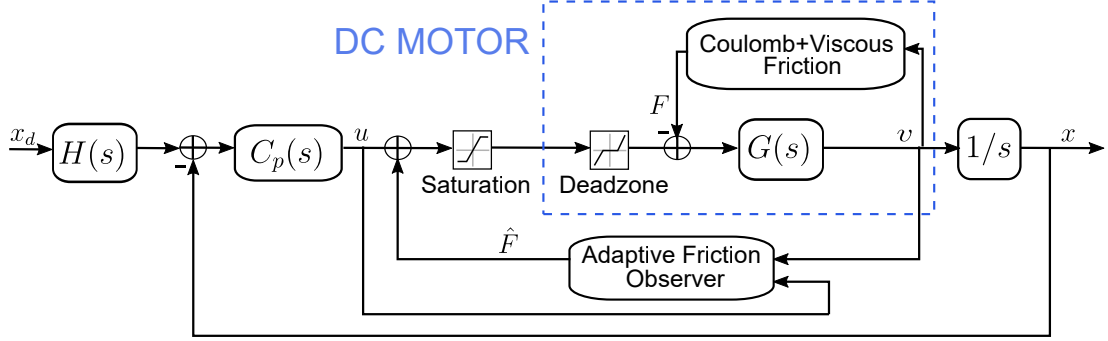
Figure 5.3: The block diagram of the DC motor position control system driven by Arduino Uno.
