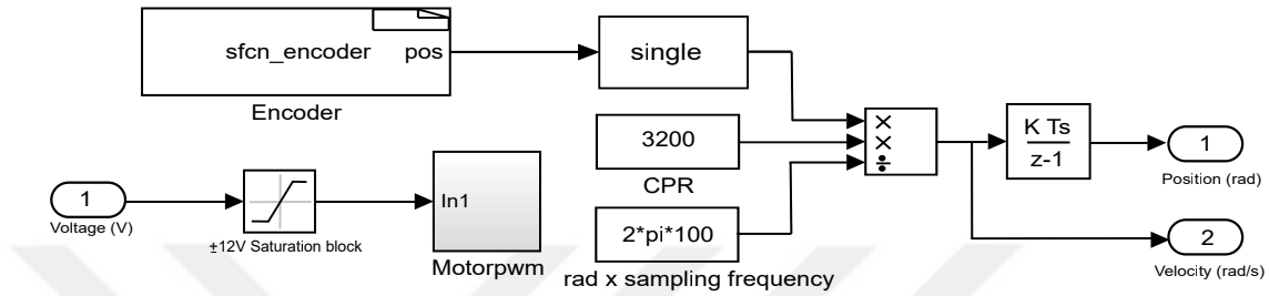
Figure B.2: Subblock diagram of DC Motor Plant
