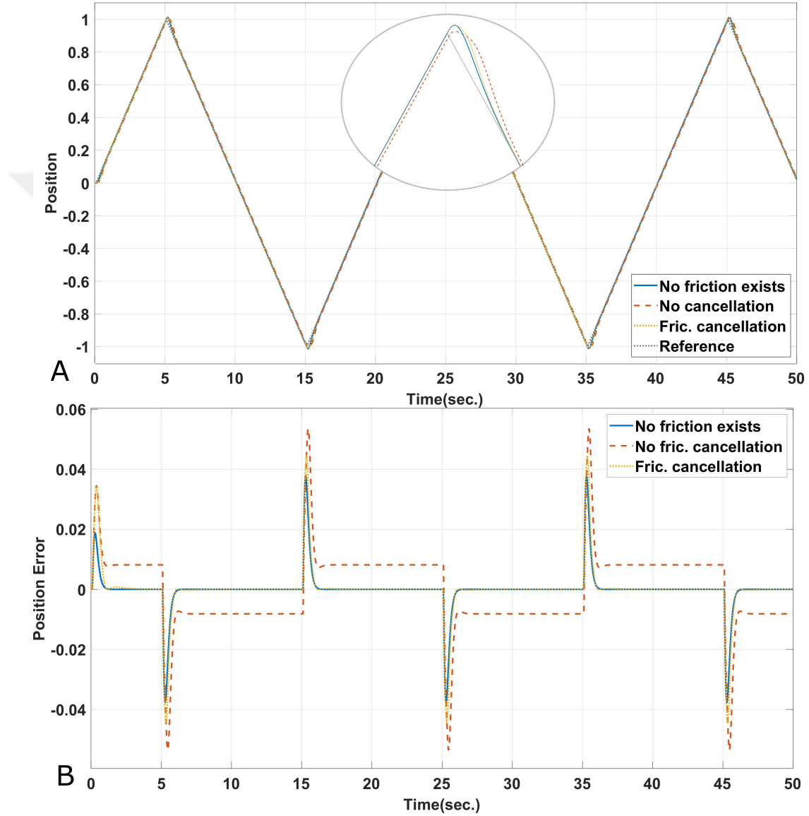
Figure 4.10: The System response for unit triangular wave input is applied to position control system including a 1 st order inverse Pade approximant based velocity predictor and a Friedland-Park type observer with k = 5 for T_d = 0.1 . Without Coulomb friction compensation, steady state errors for positive and negative position response are e_{ss}^+ = 0.8\% and e_{ss}^- = -0.8\% respectively. (A) Position tracking performance. (B) Position tracking error.
