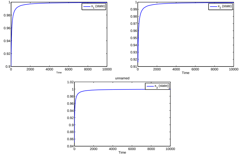
Figure 3.8: x_1(t) , x_2(t) and x_3(t) , \tau = 0 vs t graph for the homogenous gene regulatory network under positive feedback
