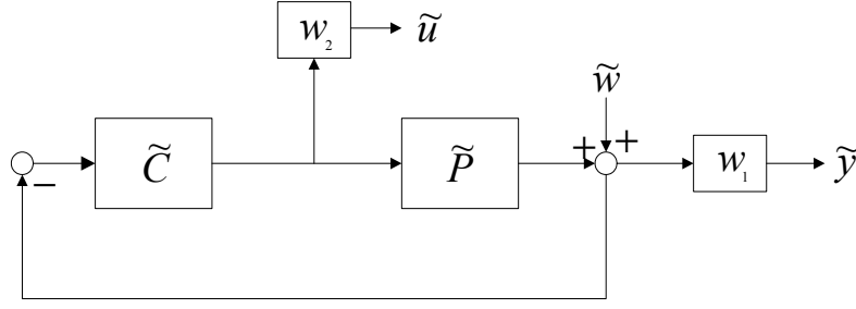
Figure 2.2: Feedback Control System
