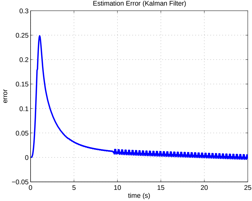
Figure 3.22: Estimation Error ( z(t) - \hat{z}(t) ) for the Kalman Filter with initial state with process noise information
