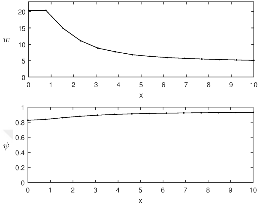
Figure 4.15: Vorticity (at y = 1 ) and stream function (at y = 0.9 ) by DBEM: Re = 10 .
