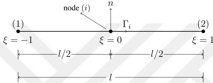
Figure 2.5: Constant element coordinate system [1]
