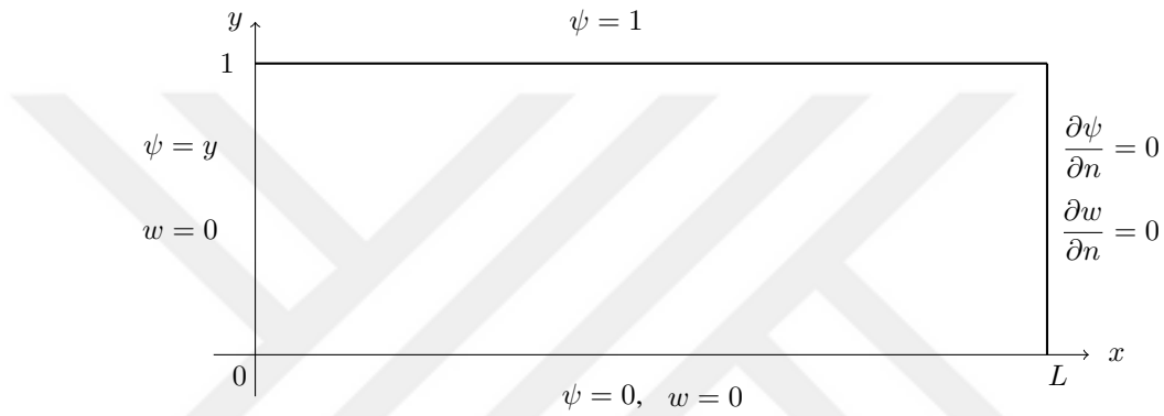
Figure 4.14: Geometry and the boundary conditions for the channel flow.
