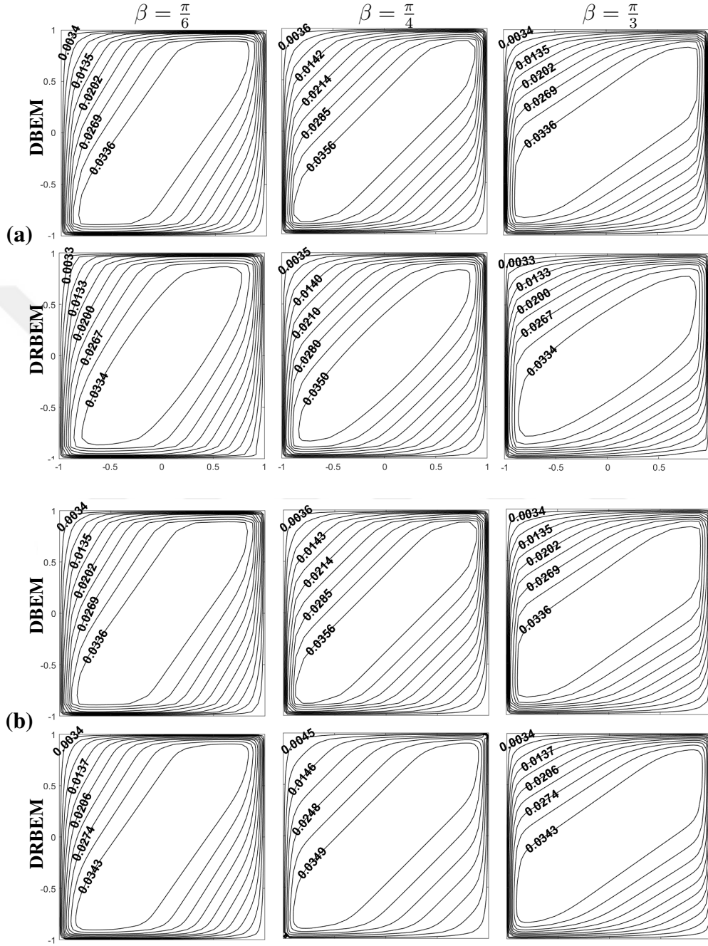
Figure 3.10: Effect of \beta on the velocity obtained by DBEM and DRBEM with the fundamental solution of (a) CD and (b) mH equations: \beta = \frac{\pi}{6}, \frac{\pi}{4}, \frac{\pi}{3} , M = 30 , T = 1 .
