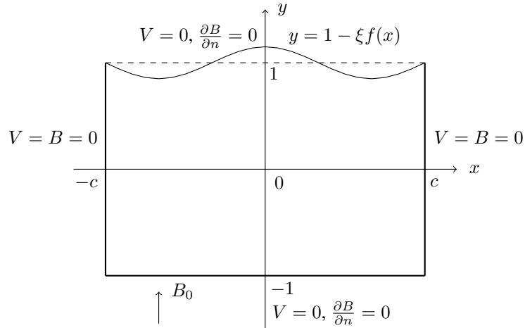
Figure 3.20: Cross-section of a perturbed duct with boundary conditions
