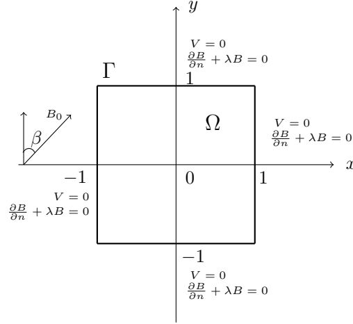
Figure 3.5: Geometry of MHD duct flow with straight walls and boundary conditions.
