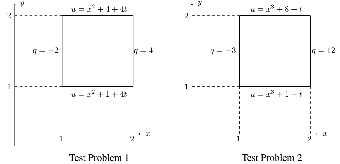
Figure 4.1: Geometries of the time-dependent heat conduction problems
