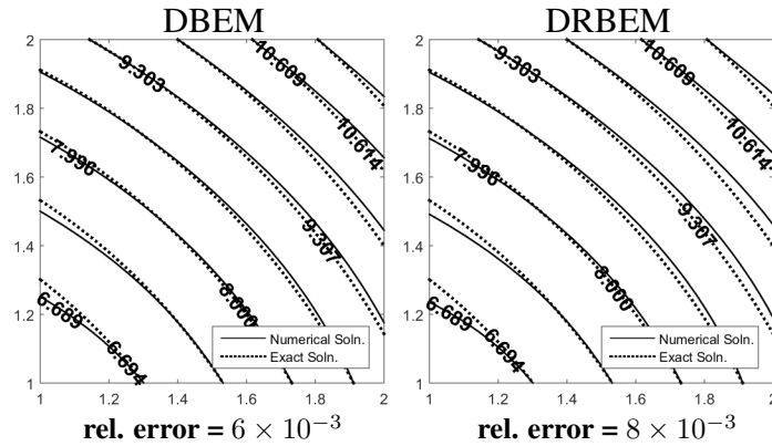
Figure 4.2: Comparison of the exact solution with the results of DBEM and DRBEM in terms of isotherms.
