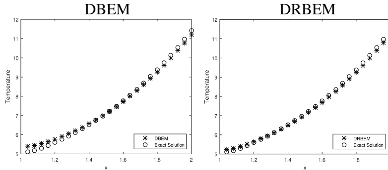
Figure 4.5: Temperature distribution along the line y = 1.5 by DBEM and DRBEM.
