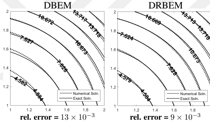
Figure 4.4: Comparison of the exact solution with the results of DBEM and DRBEM in terms of isotherms.
