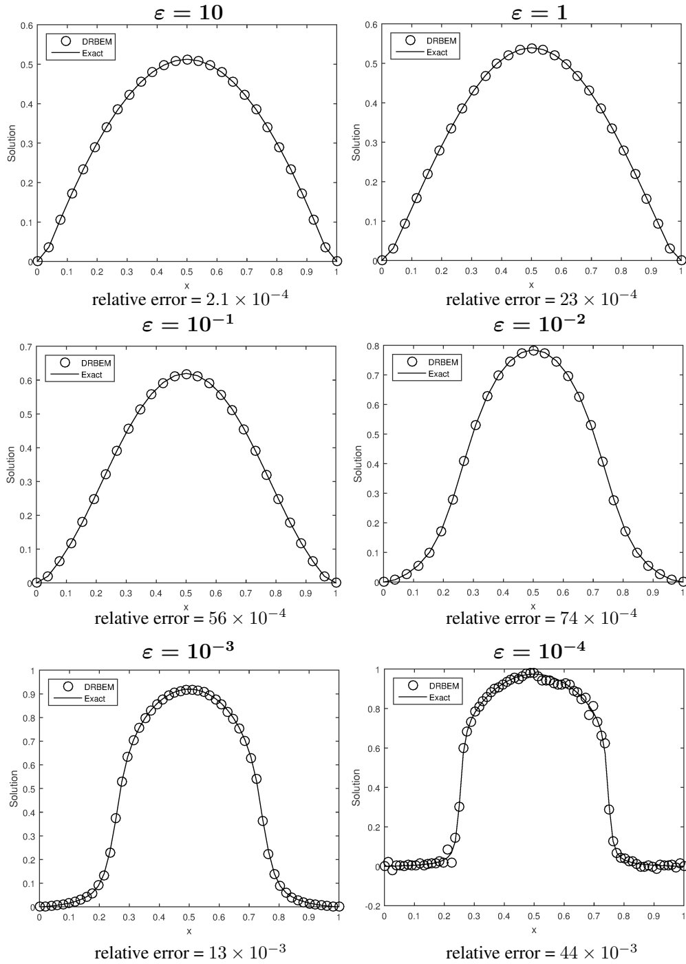
Figure 3.2: Effect of \varepsilon on the DRBEM solution with the fundamental solution of Laplace equation along horizontal centerline y = 0.5 at T = 0.5 .
