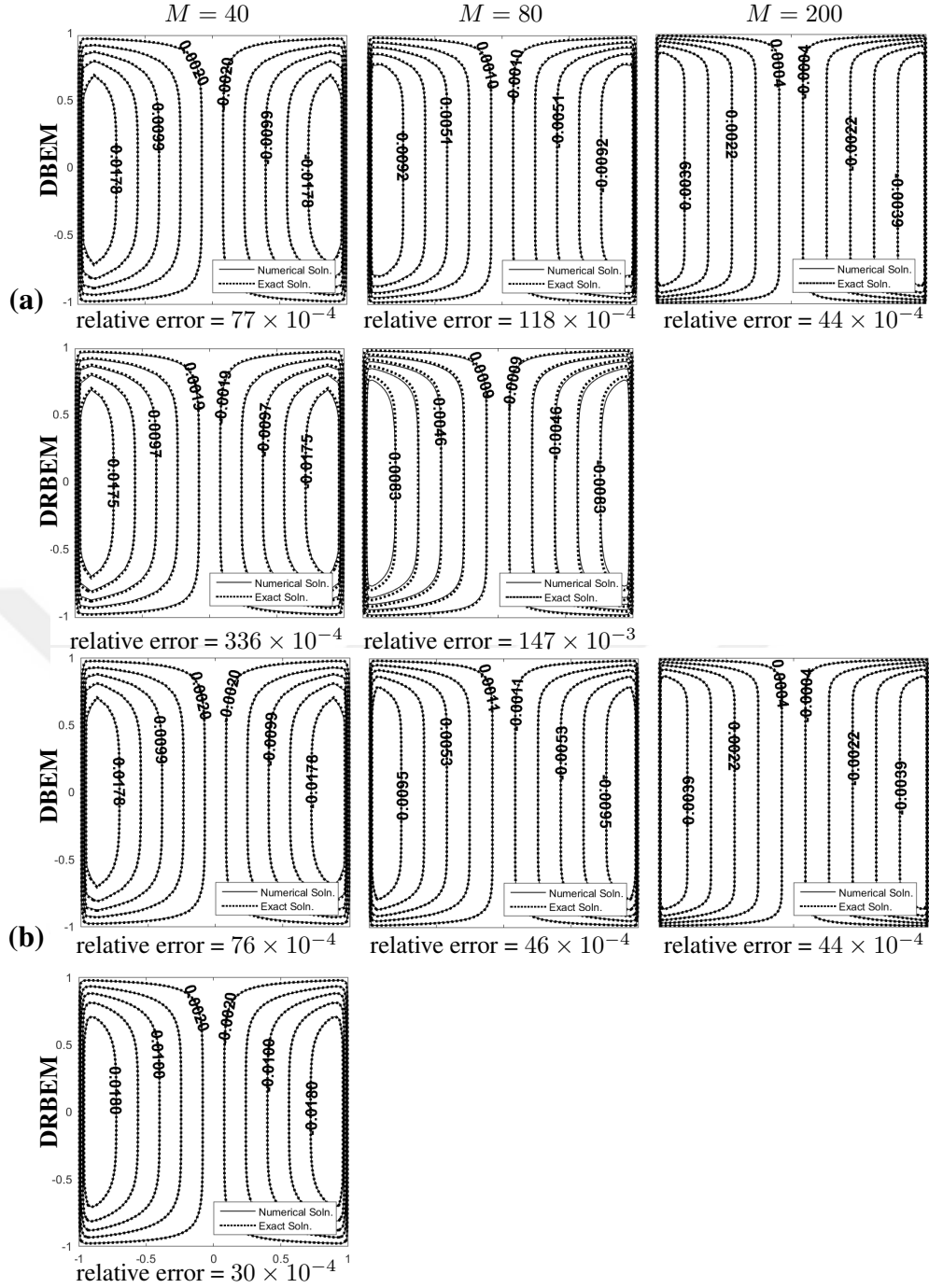
Figure 3.9: Effect of M on the induced current obtained by DBEM and DRBEM with the fundamental solution of (a) CD and (b) mH equations: M = 40, 80, 200 , \beta = \frac{\pi}{2} , T = 1 .
