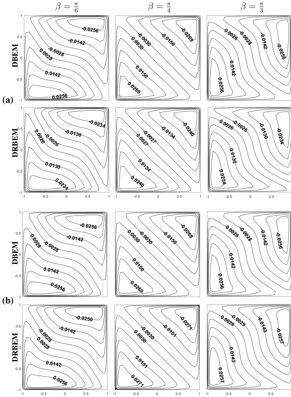
Figure 3.11: Effect of \beta on the induced current obtained by DBEM and DRBEM with the fundamental solution of (a) CD and (b) mH equations: \beta = \frac{\pi}{6}, \frac{\pi}{4}, \frac{\pi}{3} , M = 30 , T = 1 .
