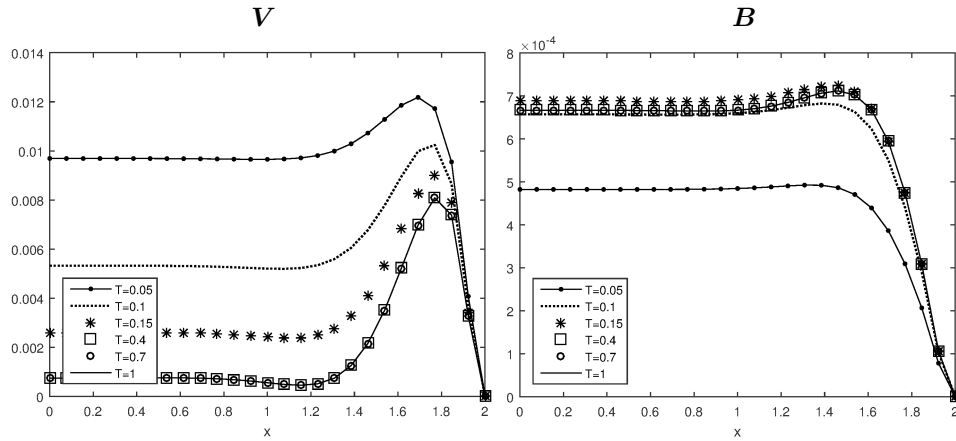
Figure 3.24: Velocity and induced magnetic field along horizontal centerline y = 0 at transient levels by DBEM with the fundamental solution of CD equation: M = 30 , \xi = 0 .
