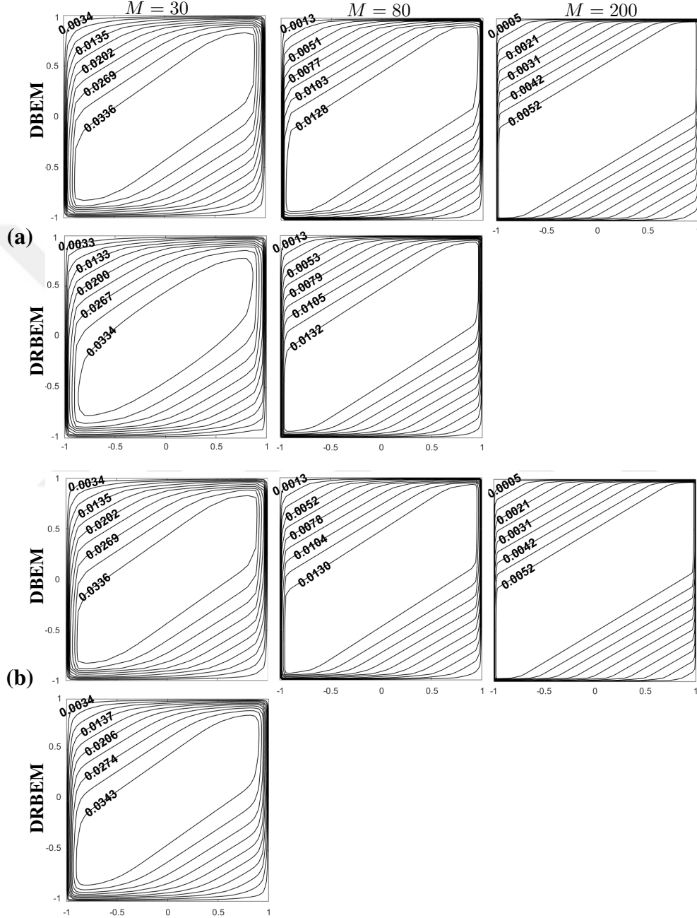
Figure 3.12: Effect of M on the velocity obtained by DBEM and DRBEM with the fundamental solution of (a) CD and (b) mH equations: M = 30, 80, 200 , \beta = \frac{\pi}{3} , T = 1 .
