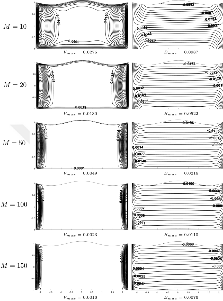
Figure 3.30: Effect of M on the velocity and induced current in a rectangular duct with perturbed upper wall obtained by DBEM with the fundamental solution of CD equation: M = 10, 20, 50, 100, 150 , f = -\cos(\frac{2\pi x}{3}) , \xi = 0.1 , T = 1 .
