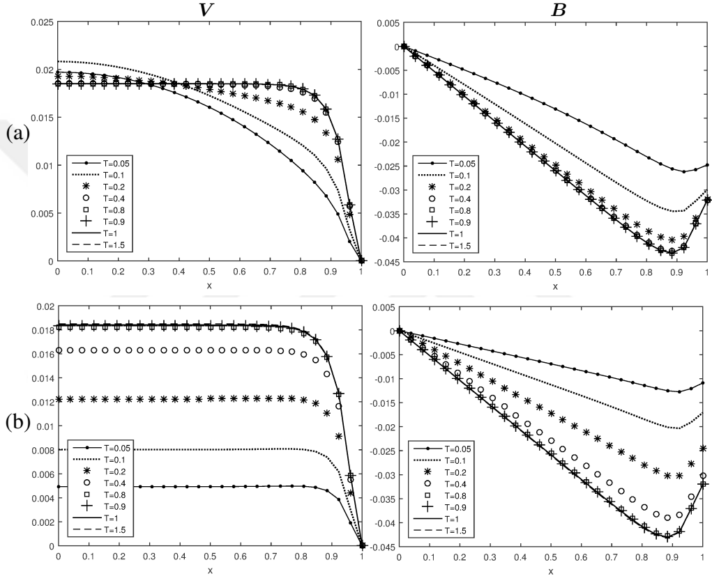
Figure 3.14: Velocity and induced magnetic field along horizontal centerline y = 0 at increasing time levels by DBEM with the fundamental solution of (a) CD and (b) mH equations: M = 20 , \lambda = 10 , \beta = \frac{\pi}{2} .
