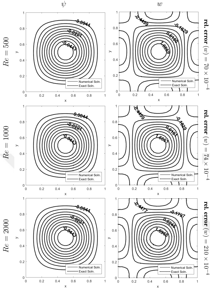
Figure 4.7: Effect of Re on the stream function and vorticity by DRBEM: Re = 500, 1000, 2000, T = 0.05 .
