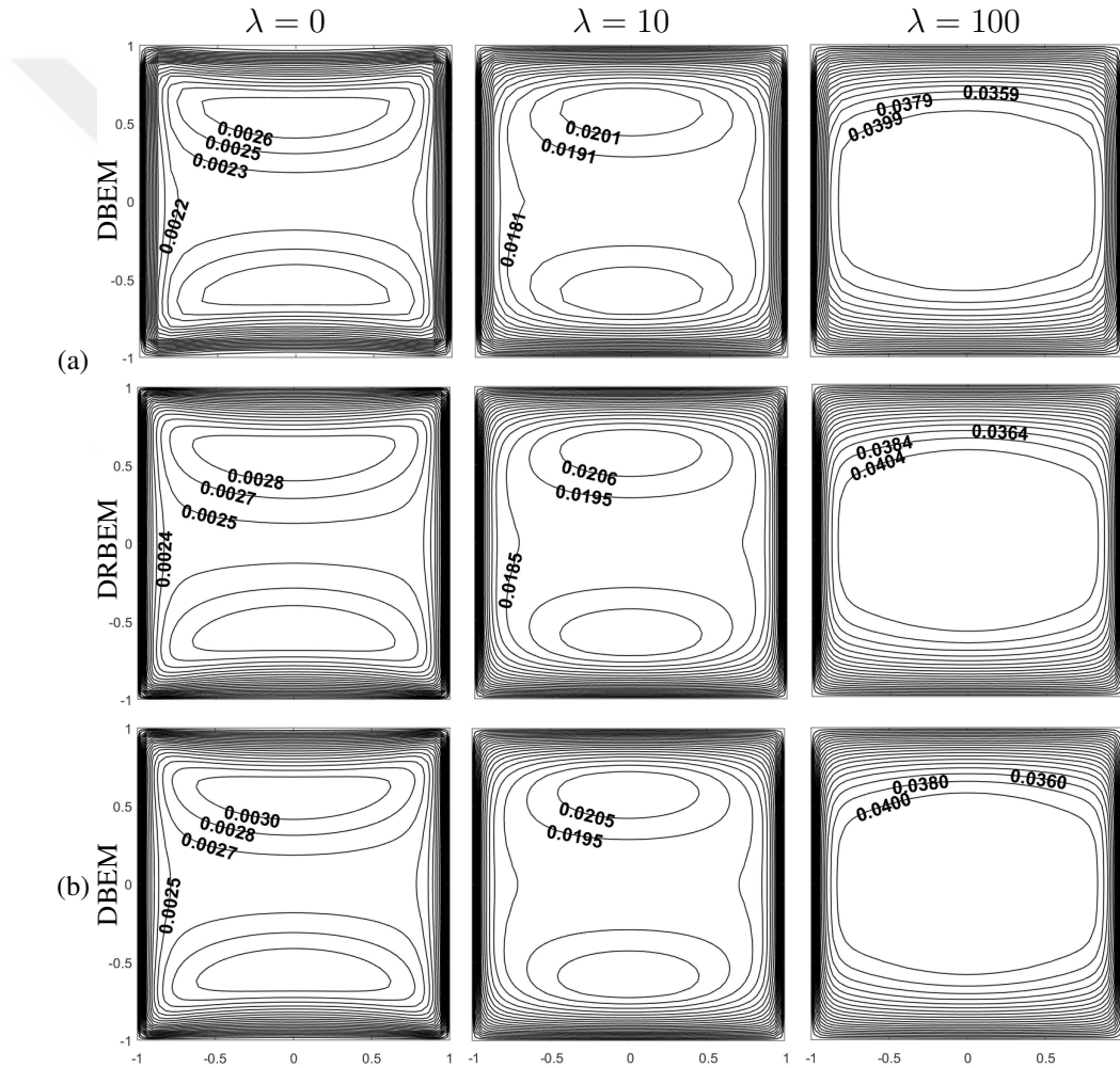
Figure 3.16: Effect of \lambda on the velocity obtained by DBEM and DRBEM with the fundamental solution of (a) CD and (b) mH equations: \lambda = 0, 10, 100 , M = 20 , \beta = \frac{\pi}{2} , T = 1 .
