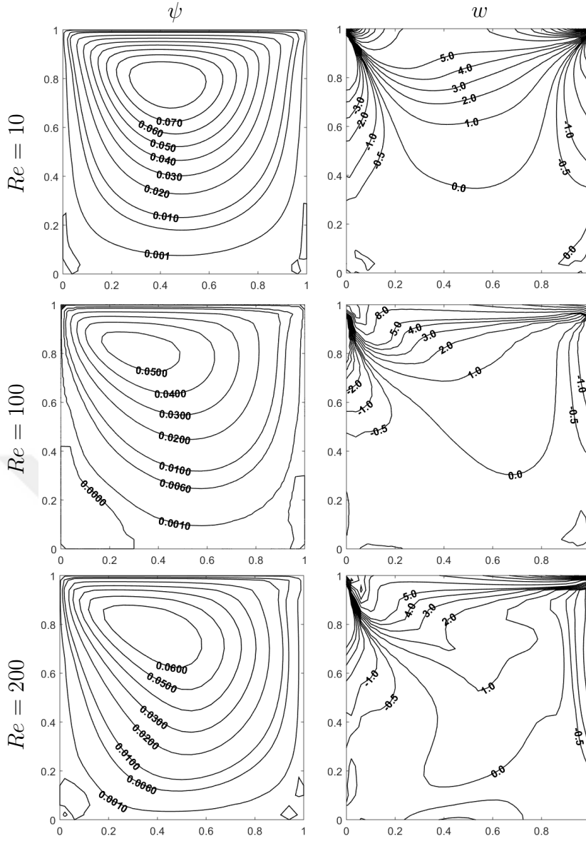
Figure 4.10: Effect of Re on the stream function and vorticity by DBEM: Re = 10, 100, 200 .
