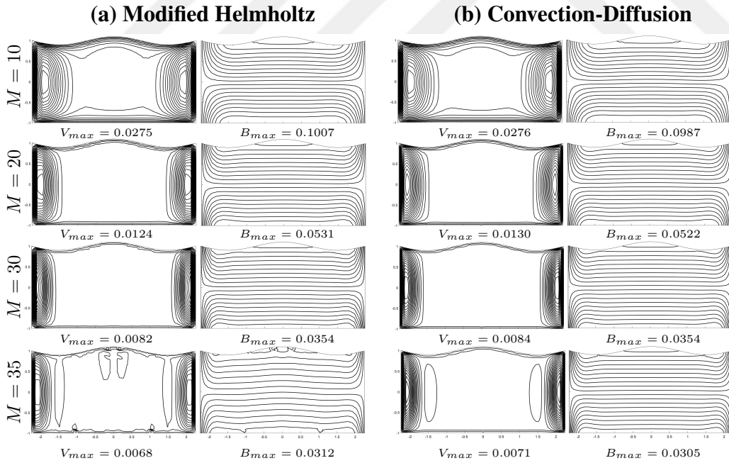
Figure 3.26: Effect of M on the velocity and induced current obtained by DBEM with the fundamental solution of (a) mH and (b) CD equations: M = 10, 20, 30, 35 , f = -\cos(\frac{2\pi x}{3}) , \xi = 0.1 , T = 1 .
