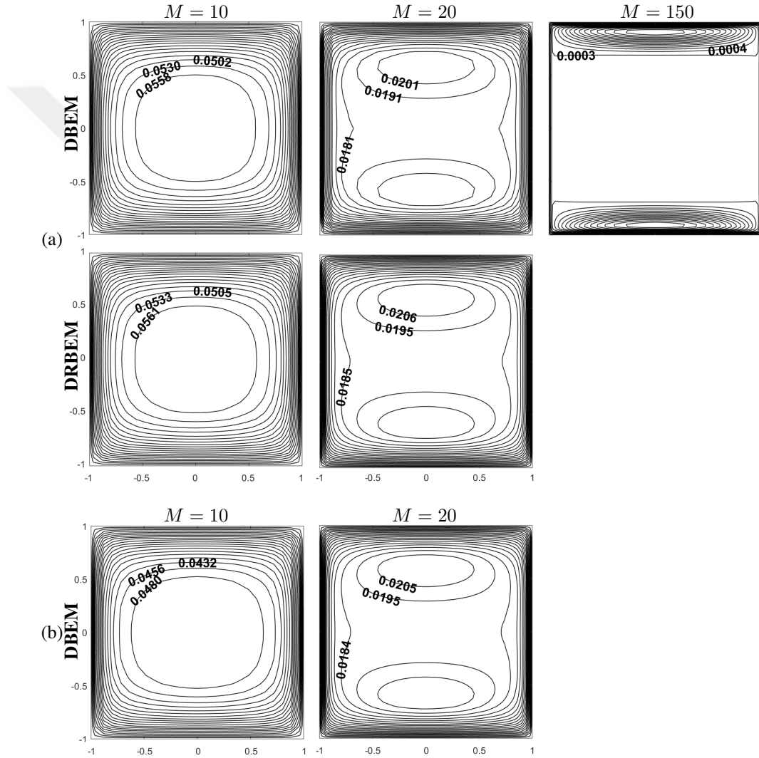
Figure 3.18: Effect of M on the velocity obtained by DBEM and DRBEM with the fundamental solution of (a) CD and (b) mH equations: M = 10, 20, 150 , \lambda = 10 , \beta = \frac{\pi}{2} , T = 1 .
