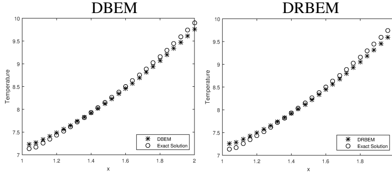
Figure 4.3: Temperature distribution along the line y = 1.5 by DBEM and DRBEM.
