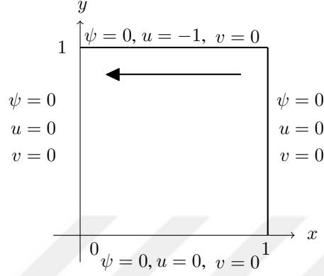
Figure 4.8: Geometry and the boundary conditions for the lid-driven cavity flow.
