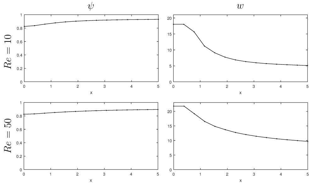
Figure 4.16: Stream function (at y = 0.9 ) and vorticity (at y = 1 ) by DBEM: Re = 10, 50 .
