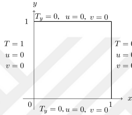
Figure 4.12: Geometry and the boundary conditions for the natural convection flow.
