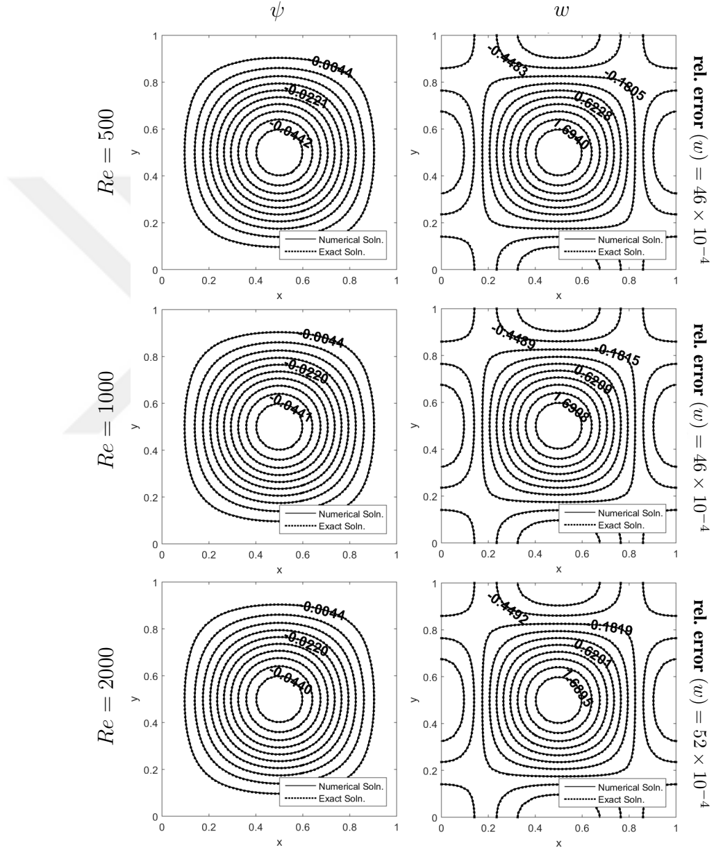
Figure 4.6: Effect of Re on the stream function and vorticity by DBEM: Re = 500, 1000, 2000, T = 0.05 .
