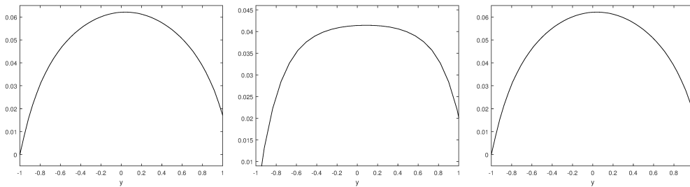
Figure 3.22: Velocity profile along the vertical lines x = -1.0 (left), x = 0 (middle) and x = 1.0 (right).
