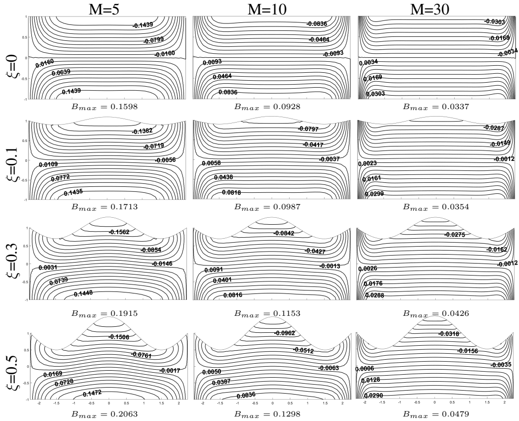
Figure 3.28: Effect of \xi on the induced current obtained by DBEM with the fundamental solution of CD equation: \xi = 0, 0.1, 0.3, 0.5 , M = 5, 10, 30 , f = -\cos(\frac{2\pi x}{3}) , T = 1 .
