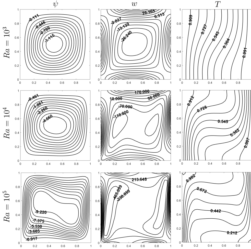
Figure 4.13: Effect of Ra on the stream function, vorticity and isotherms by DBEM: Ra = 10^3, 10^4, 10^5 .
