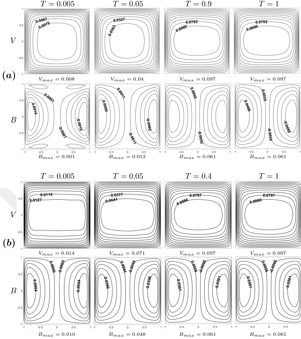
Figure 3.7: Time evolutions of the velocity and induced current by DBEM with the fundamental solutions of (a) CD and (b) mH equations: M = 10 , \beta = \frac{\pi}{2} .
