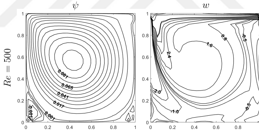
Figure 4.11: The streamlines and vorticity lines by DBEM when Re = 500 .
