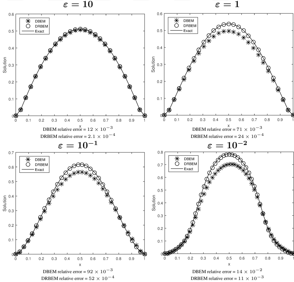
Figure 3.3: Effect of \varepsilon on the DBEM and DRBEM solutions with the fundamental solution of CDR equation along horizontal centerline y = 0.5 at T = 0.5 .
