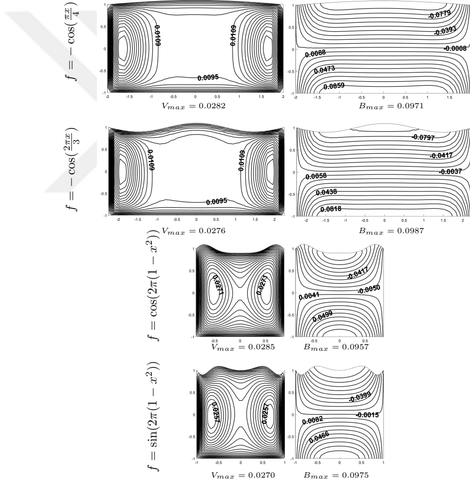
Figure 3.33: Effect of perturbation function f on the velocity and induced current in a rectangular duct with perturbed upper wall obtained by DBEM with the fundamental solution of CD equation: M = 10 , \xi = 0.1 , T = 1 .
