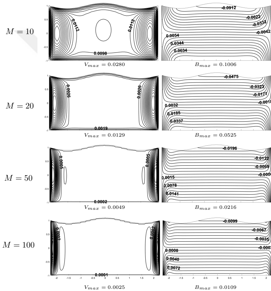
Figure 3.32: Effect of M on the velocity and induced current in a rectangular duct with perturbed upper wall obtained by DRBEM with the fundamental solution of CD equation: M = 10, 20, 50, 100 , f = -\cos(\frac{2\pi x}{3}) , \xi = 0.1 , T = 1 .
