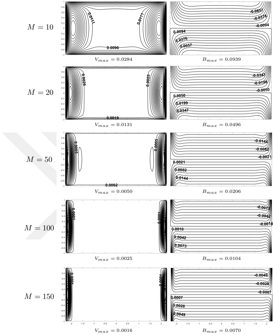
Figure 3.31: Effect of M on the velocity and induced current in a rectangular duct with straight walls obtained by DRBEM with the fundamental solution of CD equation: M = 10, 20, 50, 100, 150, T = 1 .
