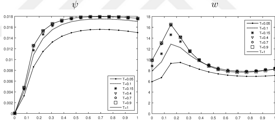
Figure 4.9: The stream function and vorticity along y = 0.9 at increasing time levels by DBEM with the fundamental solution of CD equation at Re = 10 .
