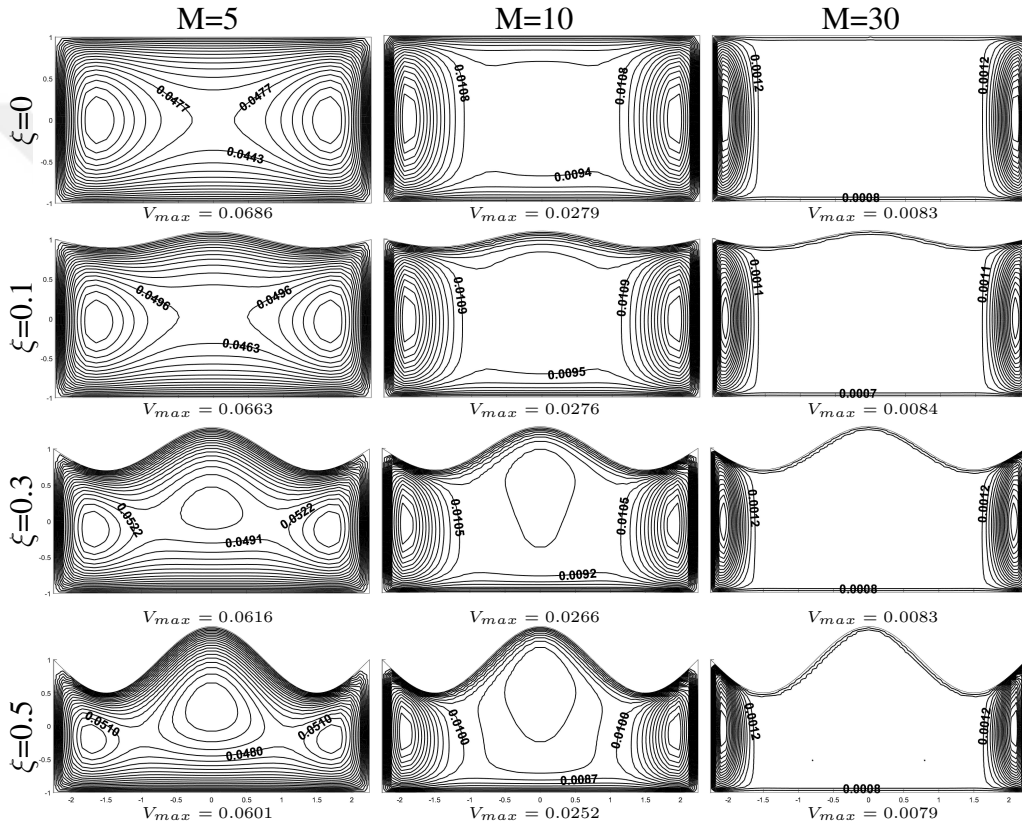
Figure 3.27: Effect of \xi on the velocity obtained by DBEM with the fundamental solution of CD equation: \xi = 0, 0.1, 0.3, 0.5 , M = 5, 10, 30 , f = -\cos(\frac{2\pi x}{3}) , T = 1 .
