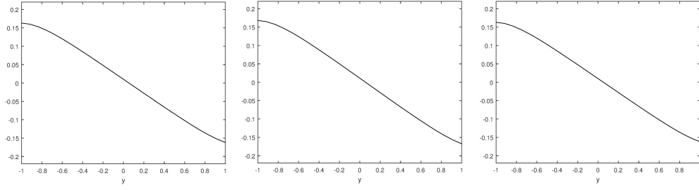
Figure 3.23: Induced magnetic field profile along the vertical lines x = -1.0 (left), x = 0 (middle) and x = 1.0 (right).
