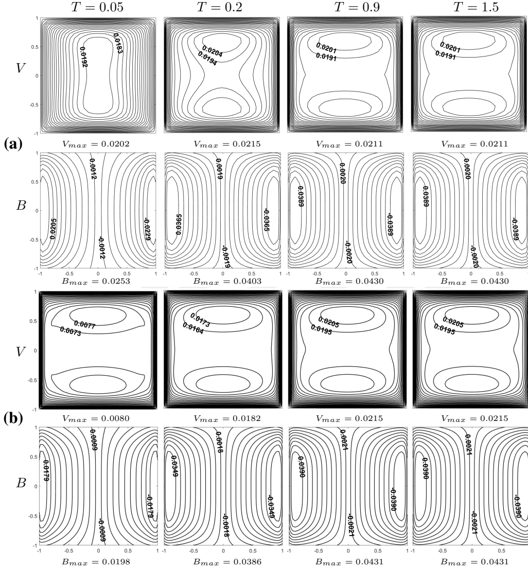
Figure 3.15: Time evolutions of velocity and induced current by DBEM with the fundamental solution of (a) CD and (b) mH equations: M = 20 , \lambda = 10 , \beta = \frac{\pi}{2} .
