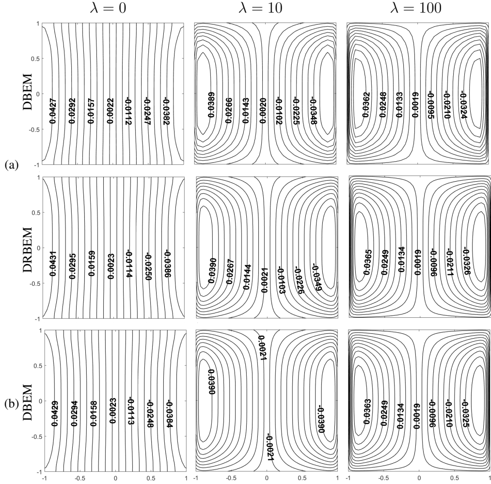
Figure 3.17: Effect of \lambda on the induced current obtained by DBEM and DRBEM with the fundamental solution of (a) CD and (b) mH equations: \lambda = 0, 10, 100 , M = 20 , \beta = \frac{\pi}{2} , T = 1 .
