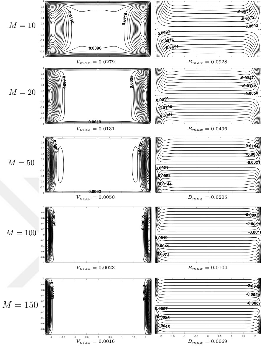
Figure 3.29: Effect of M on the velocity and induced current in a rectangular duct with straight walls obtained by DBEM with the fundamental solution of CD equation: M = 10, 20, 50, 100, 150, T = 1 .
