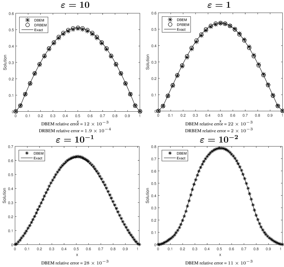
Figure 3.4: Effect of \varepsilon on the DBEM and DRBEM solutions with the fundamental solution of mH equation along horizontal centerline y = 0.5 at T = 0.5 .
