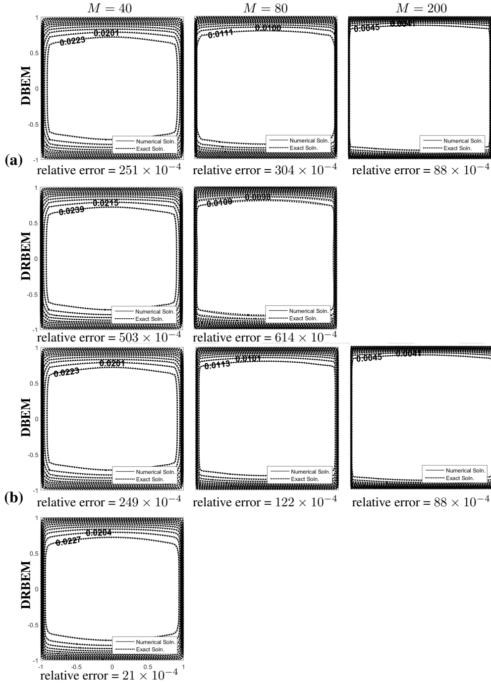
Figure 3.8: Effect of M on the velocity obtained by DBEM and DRBEM with the fundamental solution of (a) CD and (b) mH equations: M = 40, 80, 200 , \beta = \frac{\pi}{2} , T = 1 .
