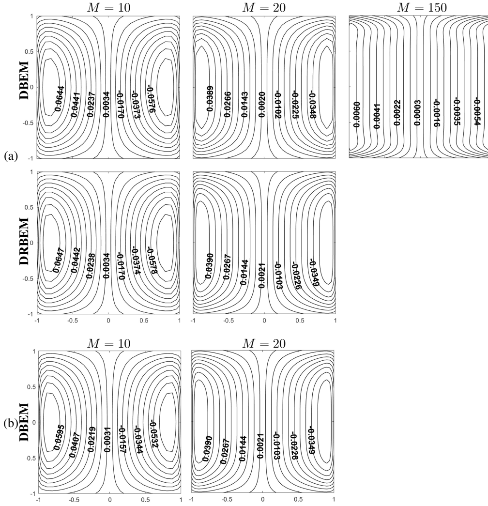
Figure 3.19: Effect of M on the induced current obtained by DBEM and DRBEM with the fundamental solution of (a) CD and (b) mH equations: M = 10, 20, 150 , \lambda = 10 , \beta = \frac{\pi}{2} , T = 1 .
