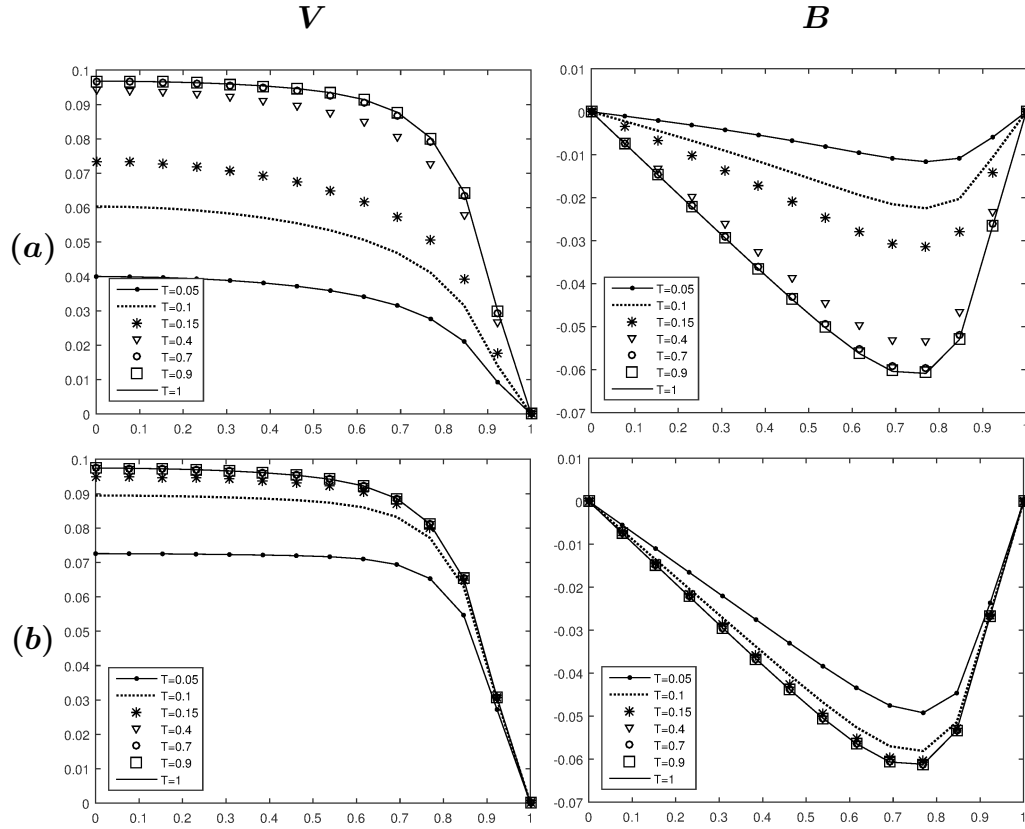
Figure 3.6: Velocity and induced magnetic field along horizontal centerline y = 0 at increasing time levels by DBEM with the fundamental solutions of (a) CD and (b) mH equations: M = 10 , \beta = \frac{\pi}{2} .
