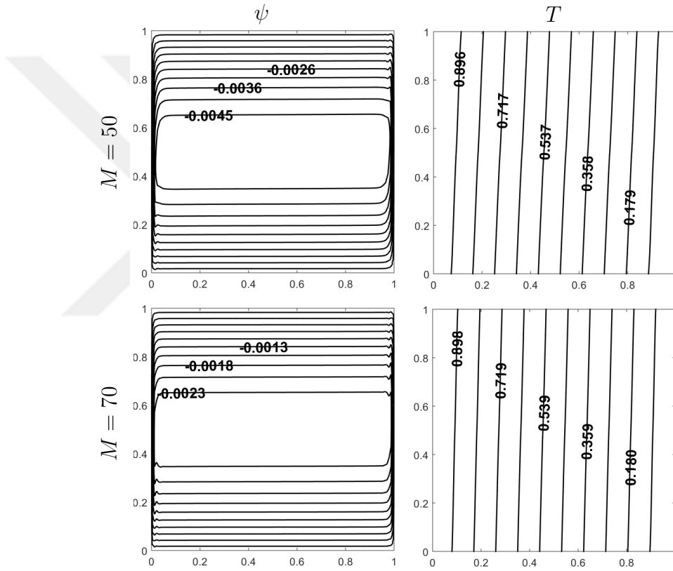
Figure 4.18: Effect of M on the stream function and temperature by DBEM: M = 50, 70, Ra = 100 .
