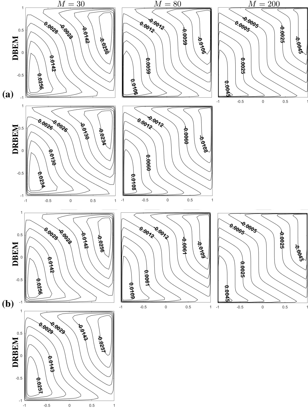
Figure 3.13: Effect of M on the induced current obtained by DBEM and DRBEM with the fundamental solution of (a) CD and (b) mH equations: M = 30, 80, 200 , \beta = \frac{\pi}{3} , T = 1 .
