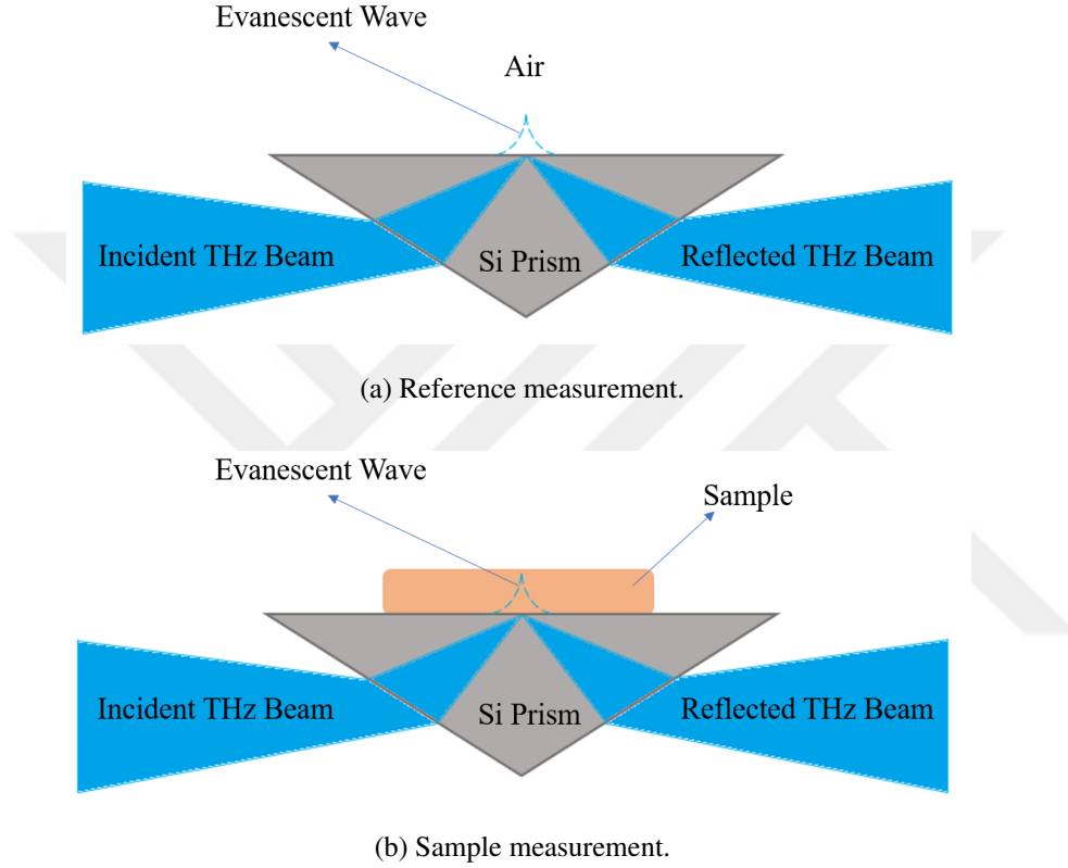
Figure 2.8: An illustration of reference and sample measurements.
