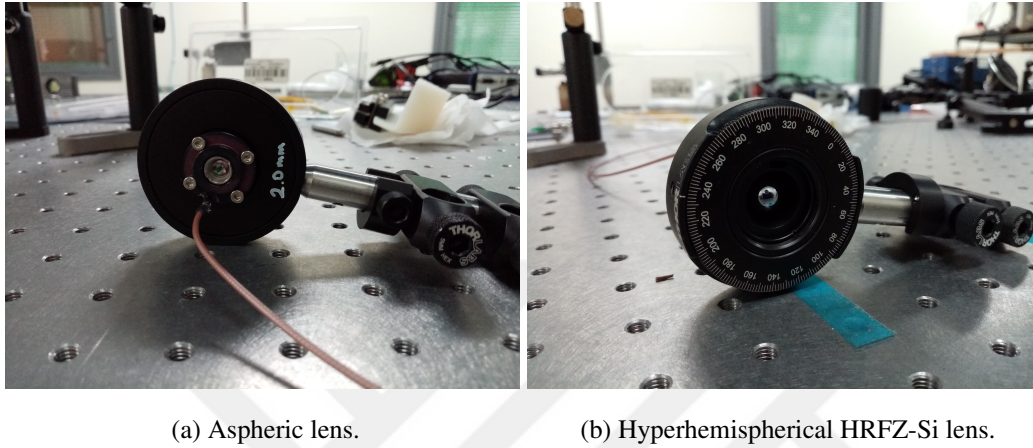
Figure 3.6: PCA with lenses and rotation mount.
