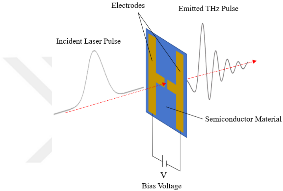
Figure 1.3: Schematic of THz generation with PCAs.
