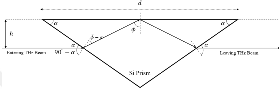
Figure 3.9: Cross Section of the ATR prism where \alpha = 38.4^\circ .
