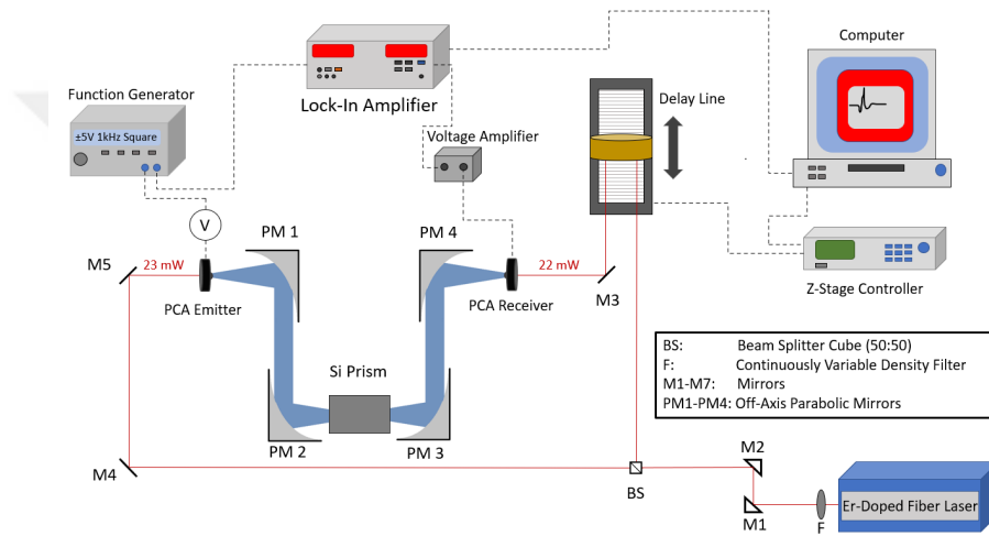
Figure 3.2: Schematic of the experimental THz ATR-TDS system.
