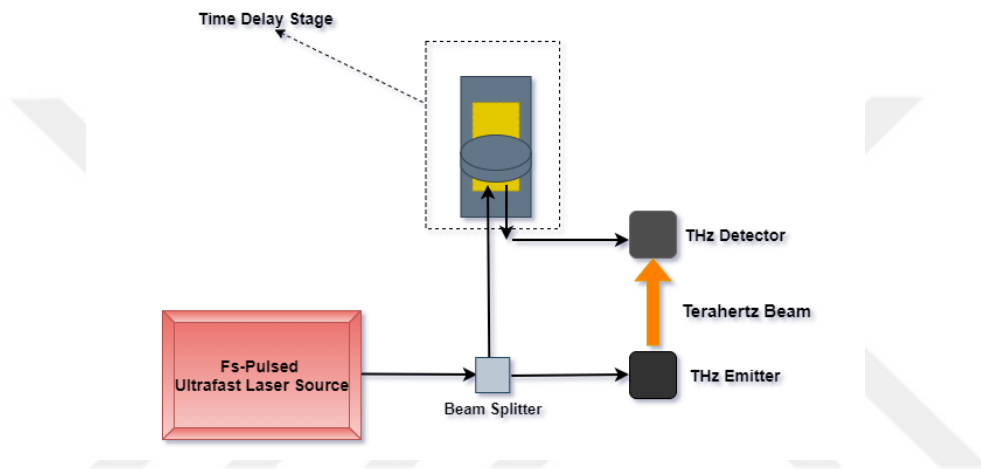
Figure 2.1: A Simplified illustration of THz Time Domain Spectroscopy Systems
