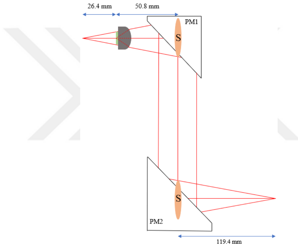
Figure 3.13: Behaviour of the emitted THz beam collimated and focused by parabolic mirrors PM1 and PM2.
