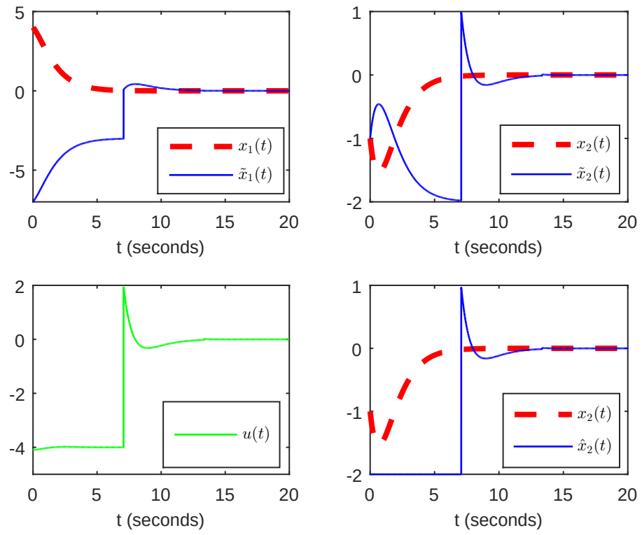
Figure 3.2: Simulation of the closed loop system: System (3.75) with controller (3.58) and continuous-discrete observer (3.57)
