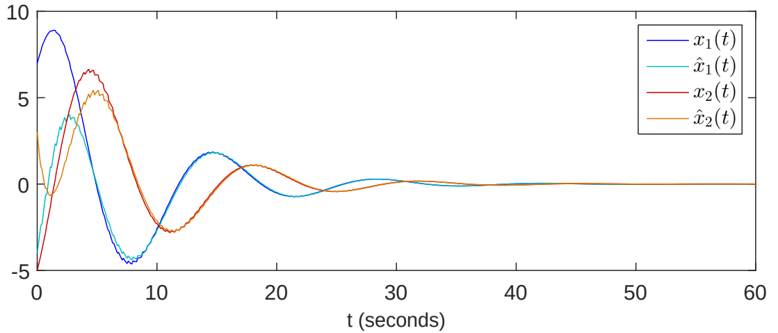
Figure 2.1: Simulation of the closed-loop system (2.16): State x and its estimate \hat{x}
