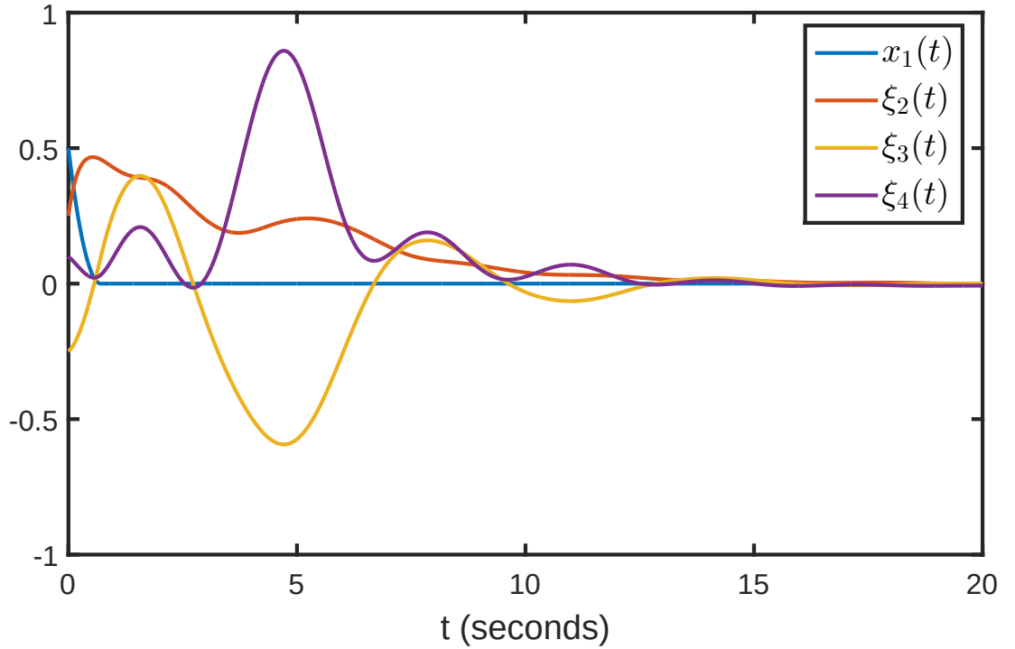
Figure 4.1: Simulation of the closed loop system: System (4.72) with input v_2 defined in (4.83)
