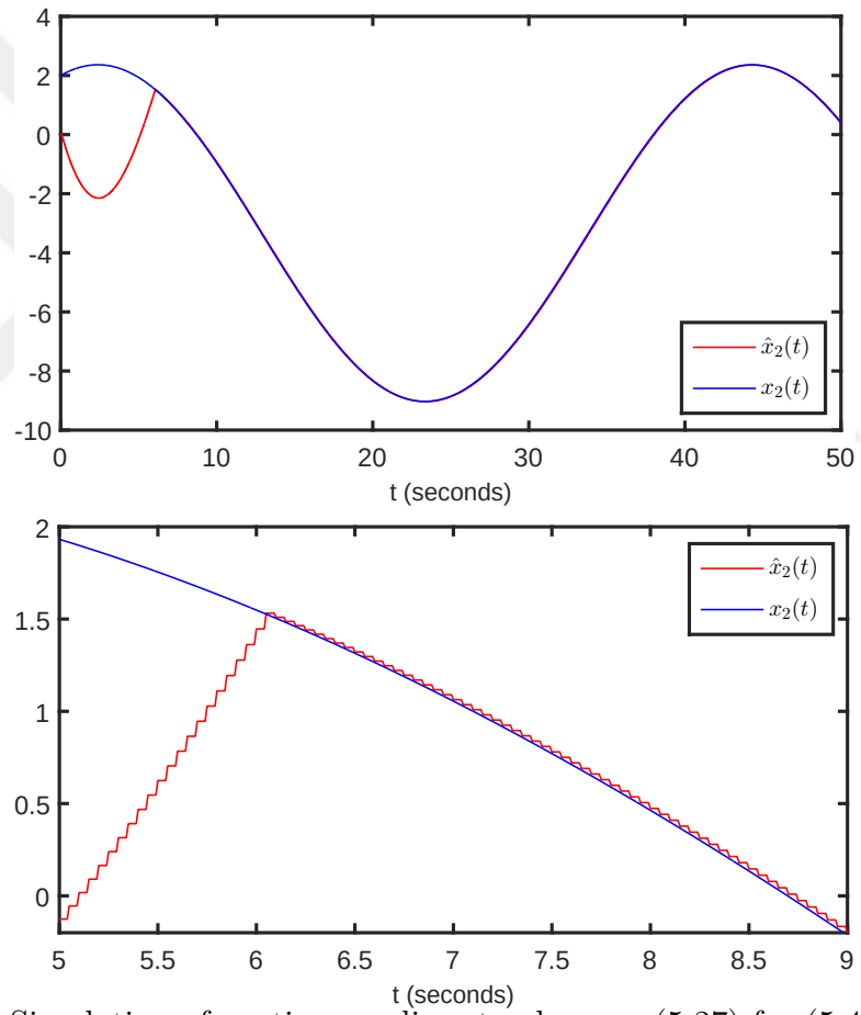
Figure 5.1: Simulation of continuous-discrete observer (5.27) for (5.44): Component x_2 and its estimate \hat{x}_2
