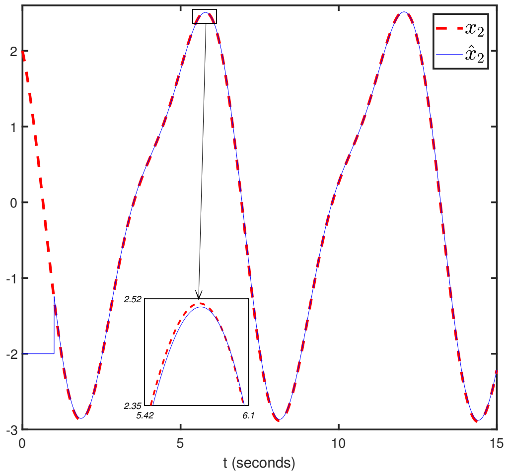
Figure 3.1: Simulation of finite-time observer (3.18) for (3.71): Component x_2 and its estimate \hat{x}_2
