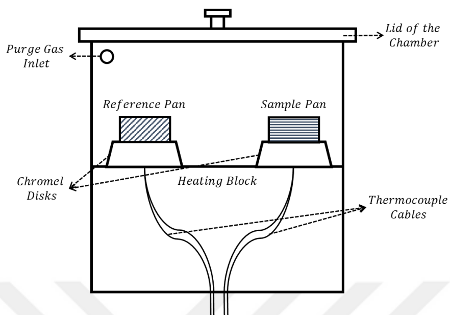
Figure 1.8. Heat flux DSC chamber drawing
