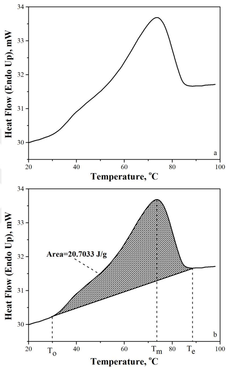
Figure 4.1. Representative thermogram for heating of crystallized honey sample (36 th hour) (a) and calculation of process temperatures and area under curve (b) where T_o , T_m and T_e denote onset, melting and end set temperature values, respectively
