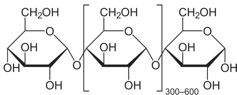
Figure 1.6. Amylose
