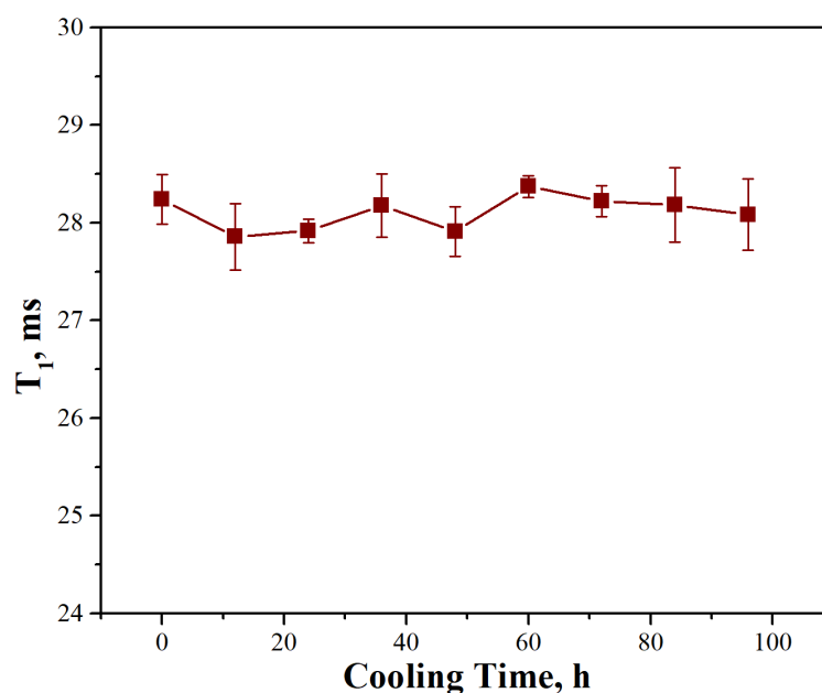
Figure 3.2. Change in T_1 relaxation time during crystallization
