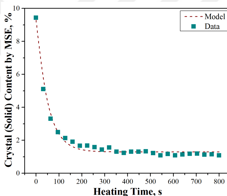
Figure 3.15. Crystallinity change during melting at 50°C
