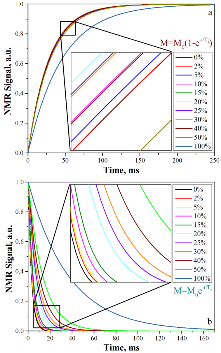
Figure 3.8. T 1 recovery (a) T 2 decay curves (b) of samples adulterated by HFCS
