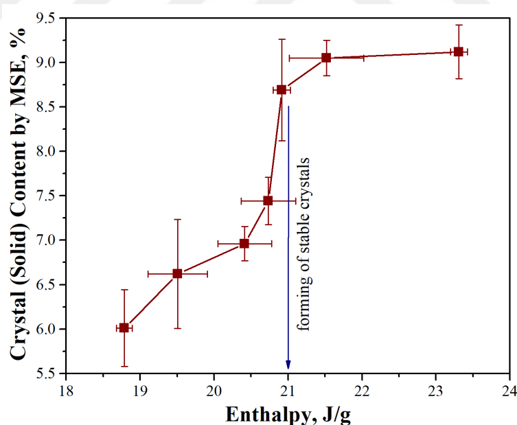
Figure 3.7. Crystal (solid) content by MSE vs. Melting enthalpy
