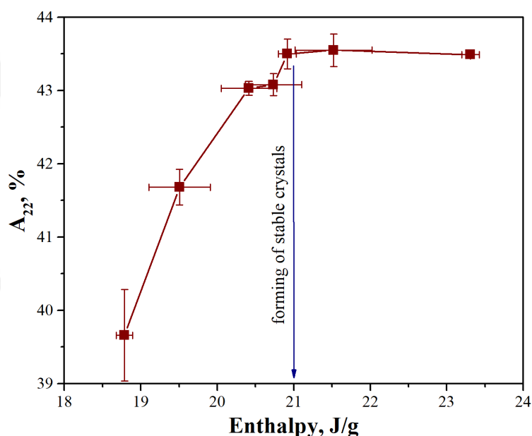
Figure 3.6. Contribution of the faster relaxing liquid into CPMG decay vs. melting enthalpy
