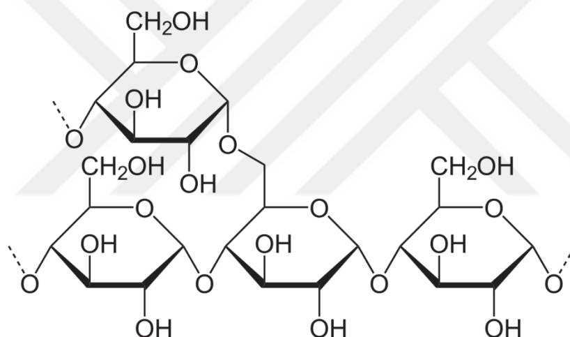
Figure 1.7. Amylopectin
