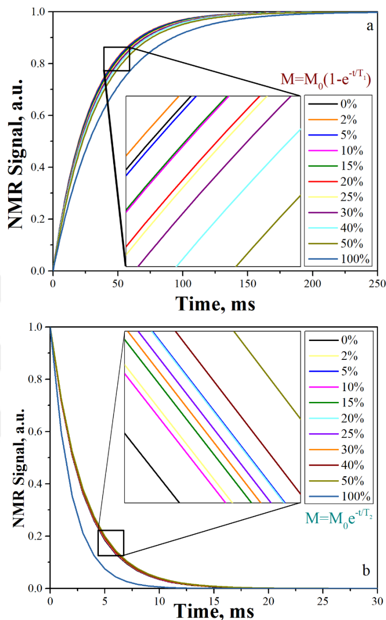
Figure 3.11. T 1 recovery curves (a) T 2 decay curves of samples (b) adulterated by GS
