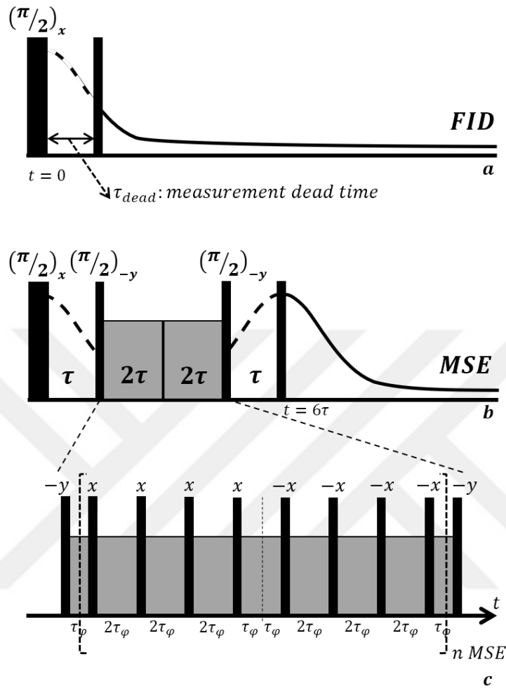
Figure 1.15. Comparison of FID (a) and MSE (b) sequences and MSE sequence pulse diagram (c)
