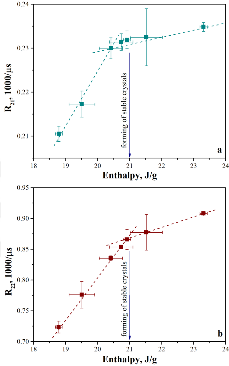
Figure 3.5. Spin-spin relaxation rate of the longer component (a) and the shorter component (b) of CPMG decay vs. melting enthalpy
