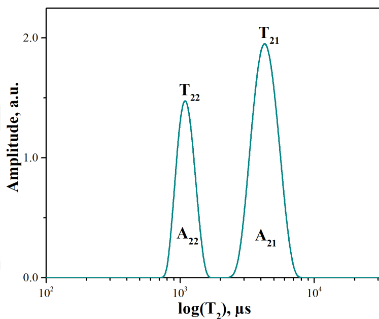
Figure 3.3. A representative T_2 relaxation spectrum showing the multiexponential nature of honey
