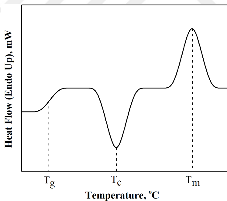
Figure 1.9. An example DSC thermogram; where T_g , T_c and T_m denote glass transition, crystallization and melting temperature values, respectively
