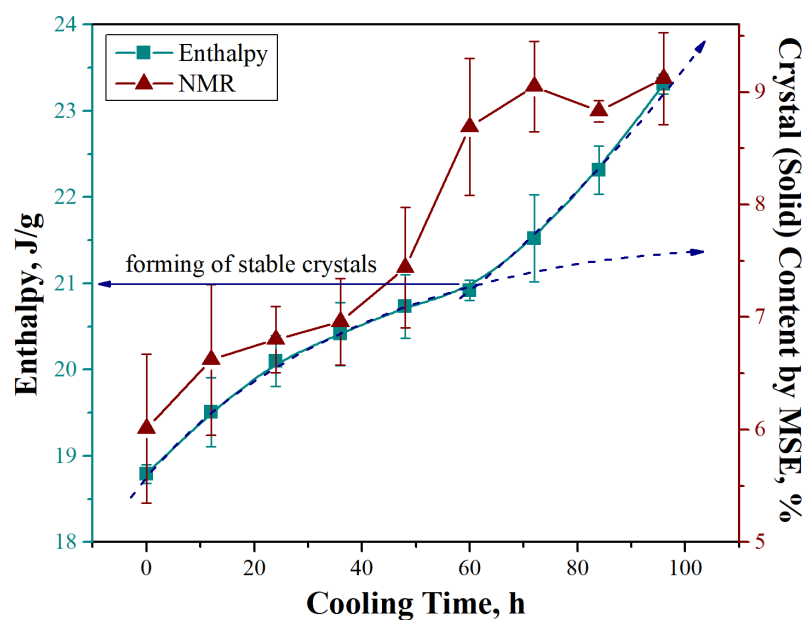
Figure 3.1. Change in the crystal melting enthalpy (by DSC) and crystal (solid) content by MSE experiments
