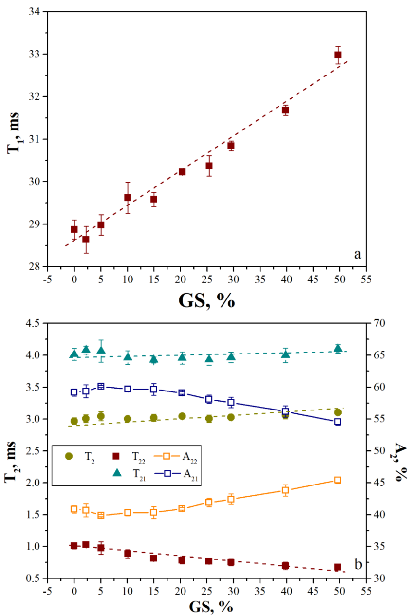
Figure 3.12. T_1 values of GS adulterated samples (a) mono and bi-exponential fitting results of T_2 times (b)
