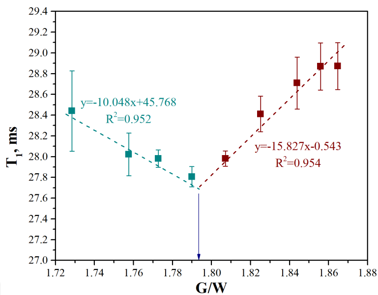
Figure 3.10. T 1 values of HFCS adulterated samples
