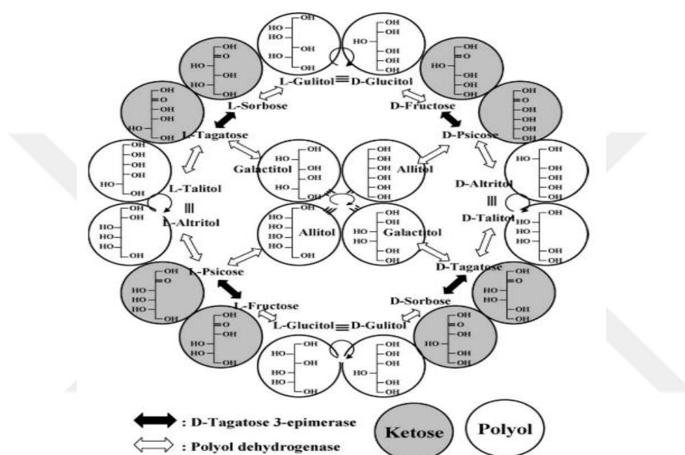
Figure 2.5. Linkage of ketohexoses by D-tagatose-3-epimerase (Izumori, 2006)
