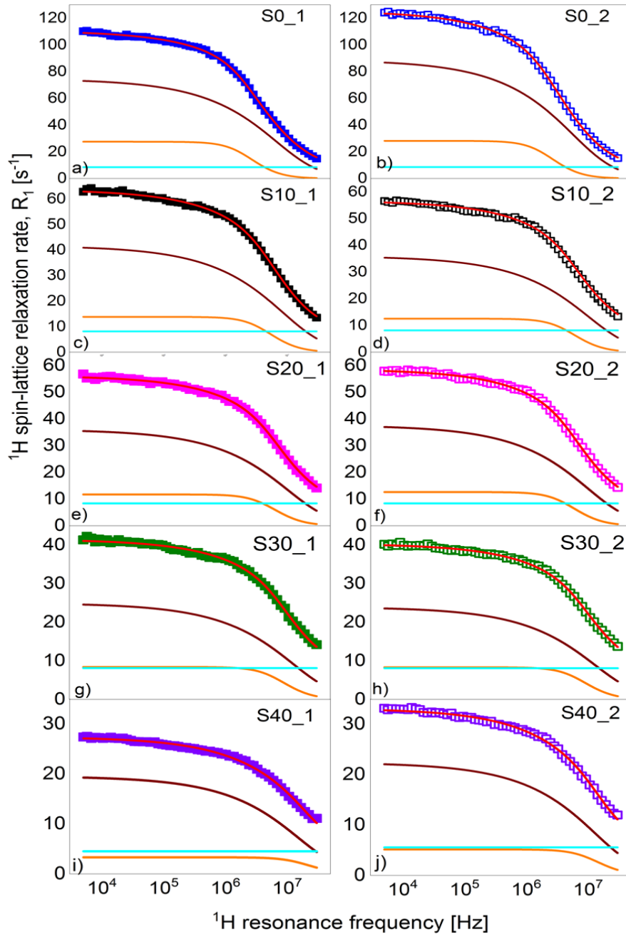
Figure 4.11. ^1\text{H} spin-lattice relaxation dispersion profiles, R_{1,H}(\omega) , for different gelatine composition. Red lines – theoretical fits decomposed into the individual contributions: R_{1,H}^{\text{confined,rot}}(\omega) (brown lines), R_{1,H}^{\text{confined,trans}}(\omega) (orange lines), A (light blue lines)
