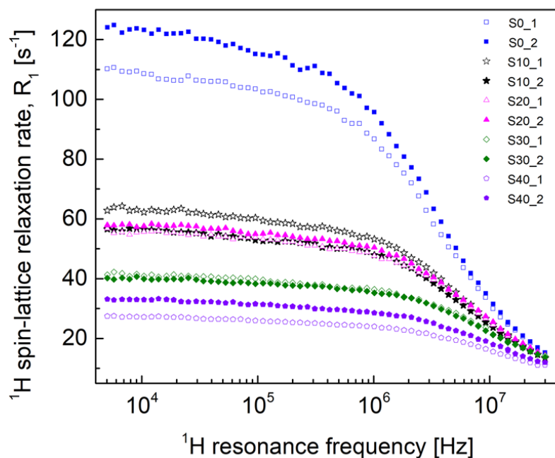
Figure 4.10. Representative NMRD profiles of gelatin based soft candies containing different amount of D-allulose; indices 1, 2 denote two replicates of each composition.
