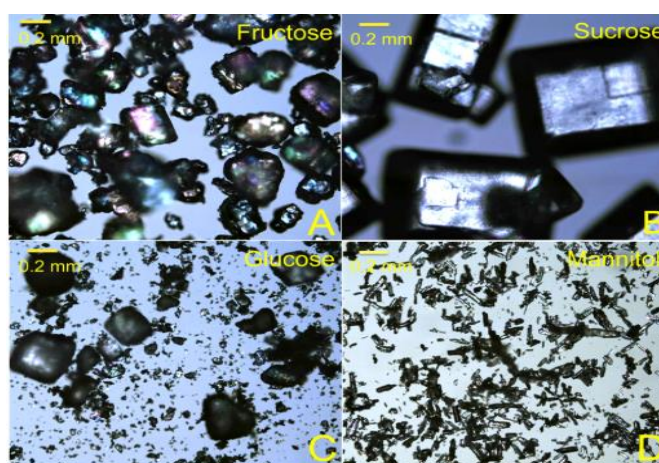
Figure 2.3. Crystals of fructose (A), sucrose (B), glucose (C), and Mannitol (D) (10x magnification) (Roos et al., 2012)
