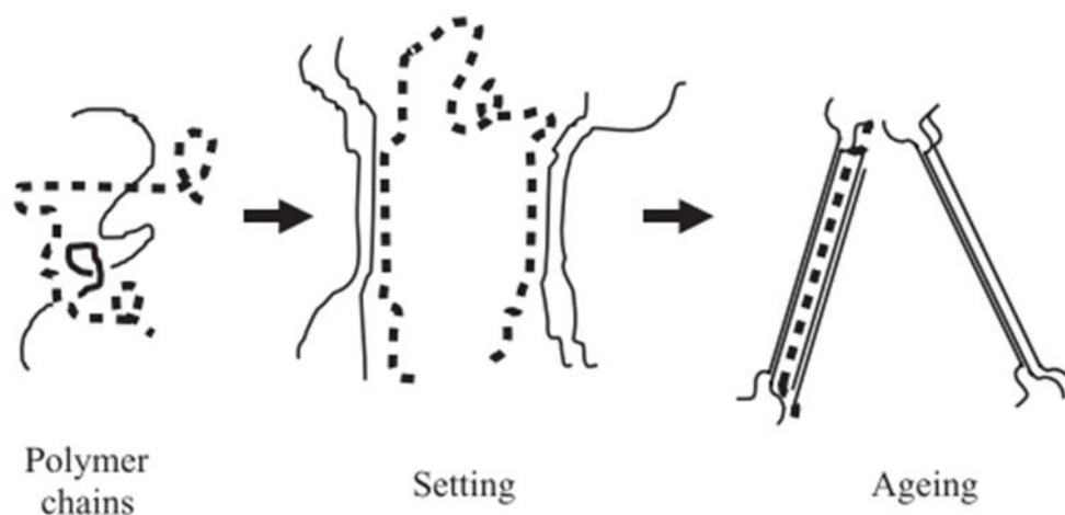
Figure 2.1. Sol-gel transition in gelatin system (Burey et al., 2009)
