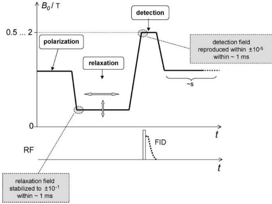
Figure 2.12. Schematic representation of a typical cycle of the main magnetic field B_0 employed with field-cycling NMR relaxometry (Kimmich & Anoardo, 2004)
