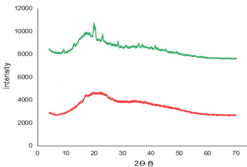
Figure 2.7. X -ray diffraction patterns of starch based confectioneries (Turkish delights) containing different type of sugar source (sucrose:— and corn syrup:—)
