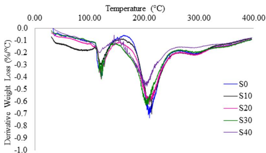
Figure 4.13. Derivative weight loss curves for different formulations
