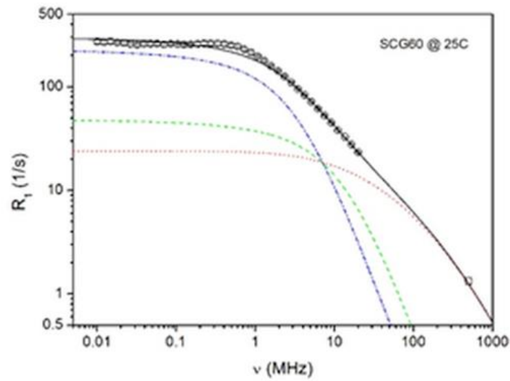
Figure 4.17. Proton spin-lattice relaxation dispersion profiles obtained at 25°C for SUC (a), SBF10 (b), SCG40 (c), and SCG60 (d); the solid lines are the best fits of equations (3), (6), (7) to the experimental data (see text); deconvolution of the overall
