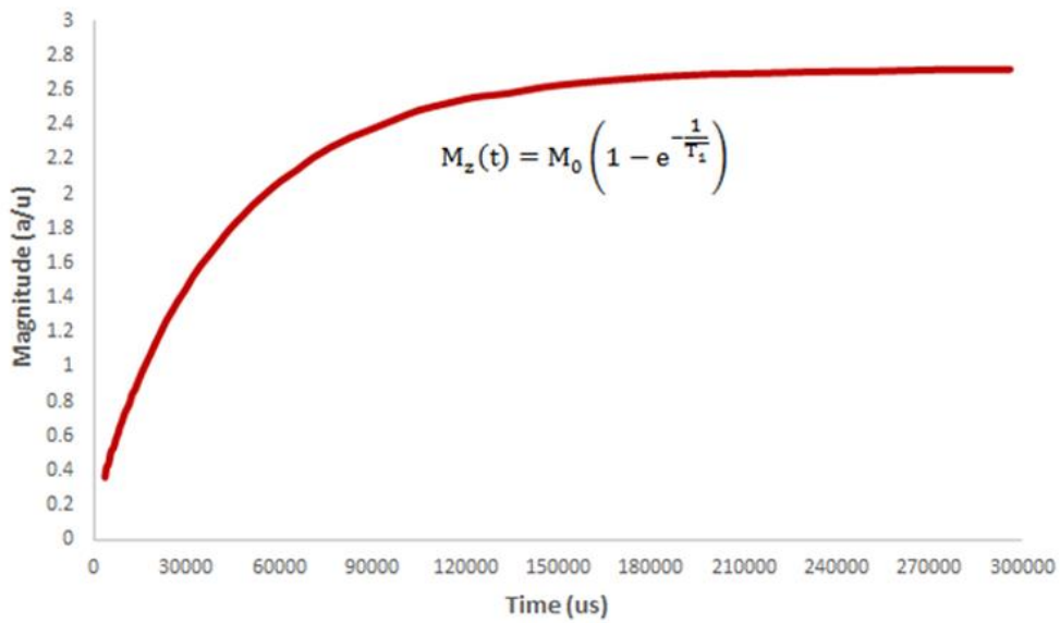
Figure 2.10. Representative graph for the magnetization recovery curve with the growth rate of T_1
