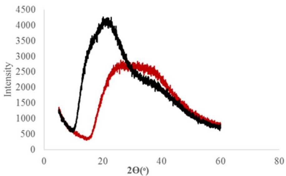
Figure 4.3. X-Ray Diffraction Pattern of gelatin based soft candies at the first day of storage: P0 (—) and P40 (—)
