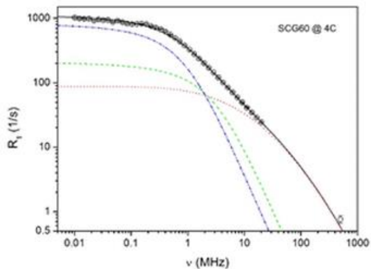
Figure 4.18. Proton spin-lattice relaxation dispersion profiles obtained at 4°C for SUC (a), SBF10 (b), SCG40 (c), and SCG60 (d); the solid lines are the best fits of equations (3), (6), (7) to the experimental data (see text); deconvolution of the
