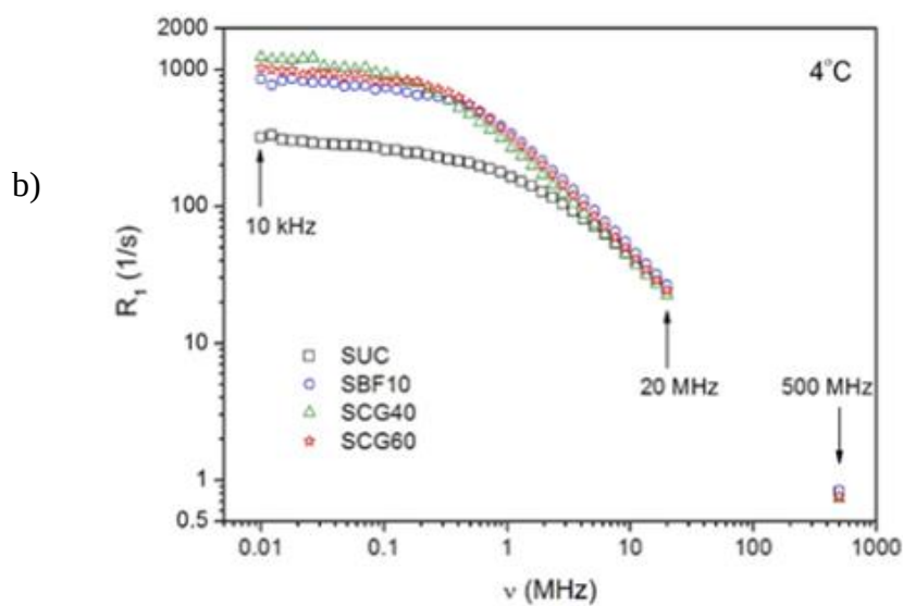
Figure 4.16. Proton spin-lattice relaxation dispersion profiles of Turkish delights formulated with different type of sugar source (corn syrup or sucrose) obtained with a FFC NMR relaxometer in the range of 10 kHz-20 MHz at 25°C (a) and 4°C (b); additional points were obtained at 500 MHz with a conventional NMR spectrometer
