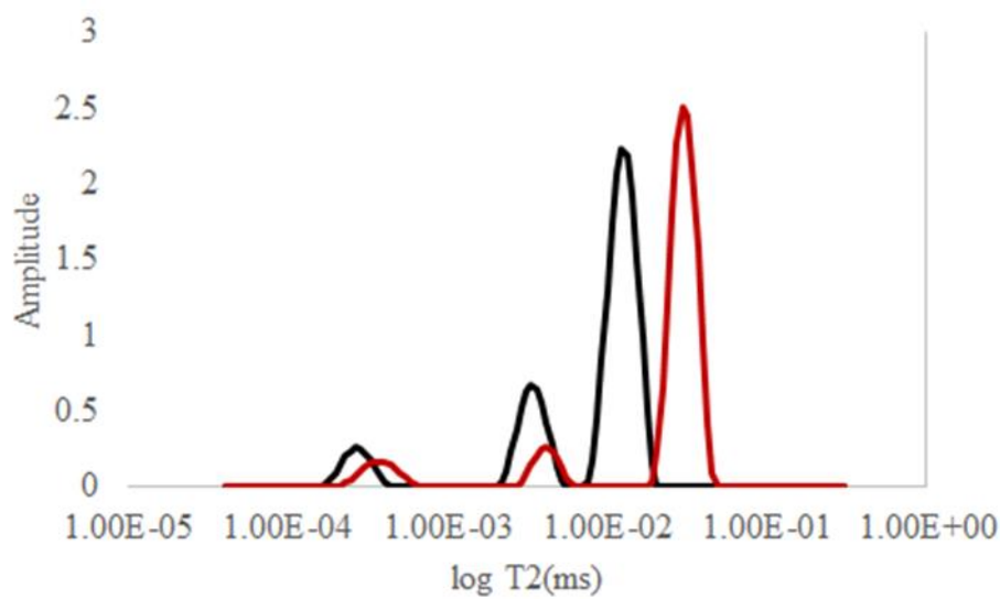
Figure 4.9. T_2 Relaxation Spectrum graph of gelatin based soft candies at the 28 th day of storage: P0 (—) and P40 (—)
