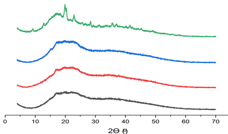
Figure 4.15. X-ray diffraction pattern of Turkish delights formulated with different type of sugar source (SUC: — , SCG60: — , SCG40: — , SBF10: — )
