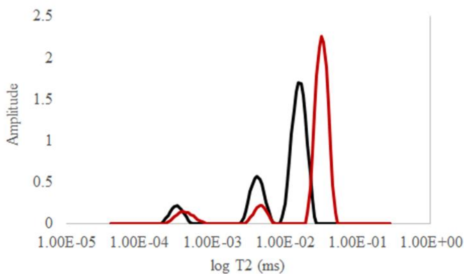
Figure 4.8. T_2 Relaxation Spectrum graph of gelatin based soft candies at the first day of storage: P0 (—) and P40 (—)
