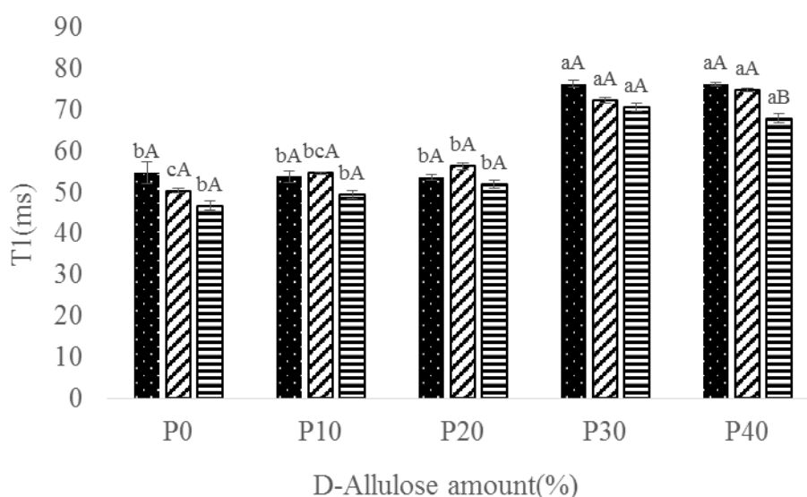
Figure 4.7. T_1 (spin-lattice) relaxation times of gelatin based soft candies at the first day (■), 14 th day (▨) and 28 th day (▤) of storage
