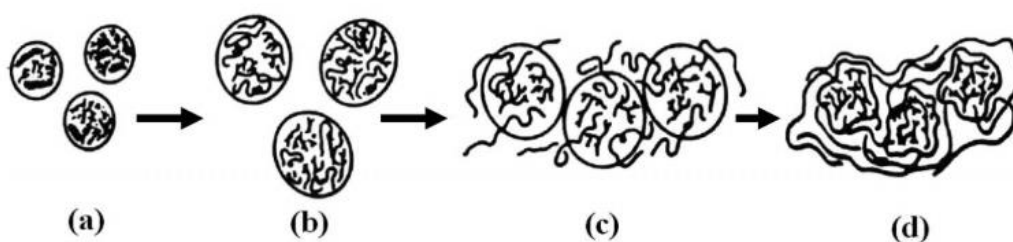
Figure 2.2. The mechanism of starch gelatinization a) Starch granules b) Swelling of starch granules upon exposing heat and moisture c) Leaching of amylose from the granules d) Formation of starch gel matrix (Burey et al., 2009)
