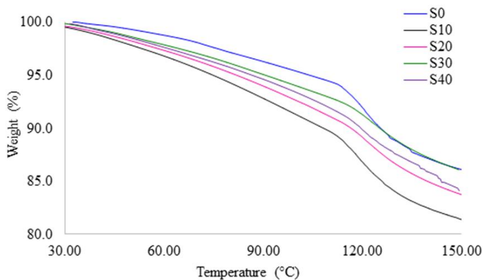
Figure 4.12. Thermogravimetric Analysis (TGA) thermogram of different formulations
