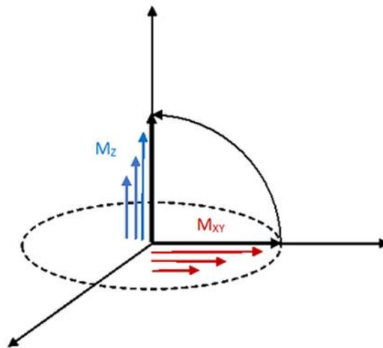
Figure 2.9. Decaying and recovering of transverse magnetization ( M_{xy} ) vector longitudinal magnetization vector ( M_z ), respectively after RF pulse is turned OFF (Hashemi et al., 2010)
