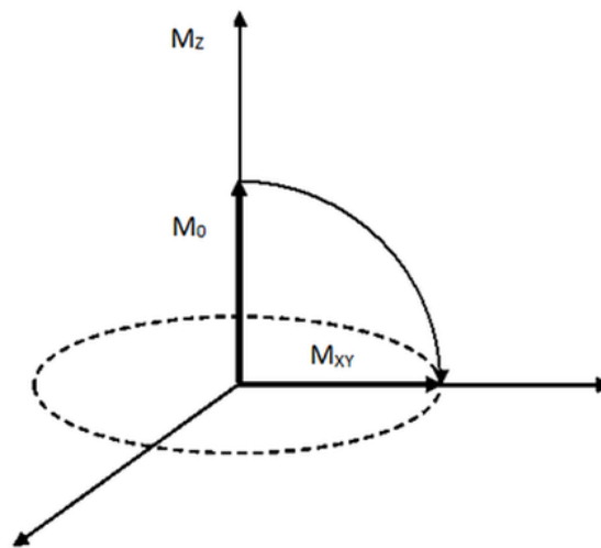
Figure 2.8. Flipping of M_0 (longitudinal magnetization 90^\circ into x-y plane leading to formation of M_{xy} (transverse magnetization) after RF pulse is turned ON (Hashemi et al., 2010)
