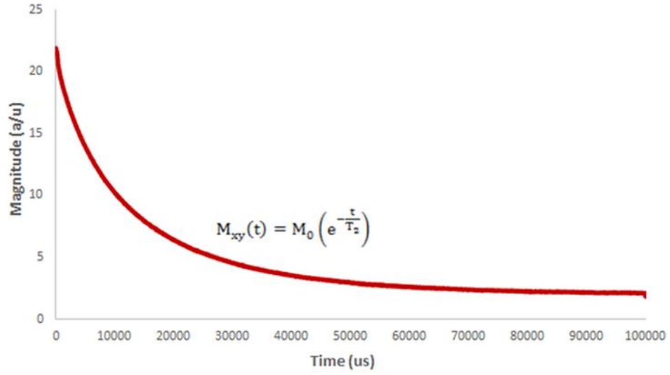
Figure 2.11. Representative graph for the magnetization decaying curve with the decay rate of T_2
