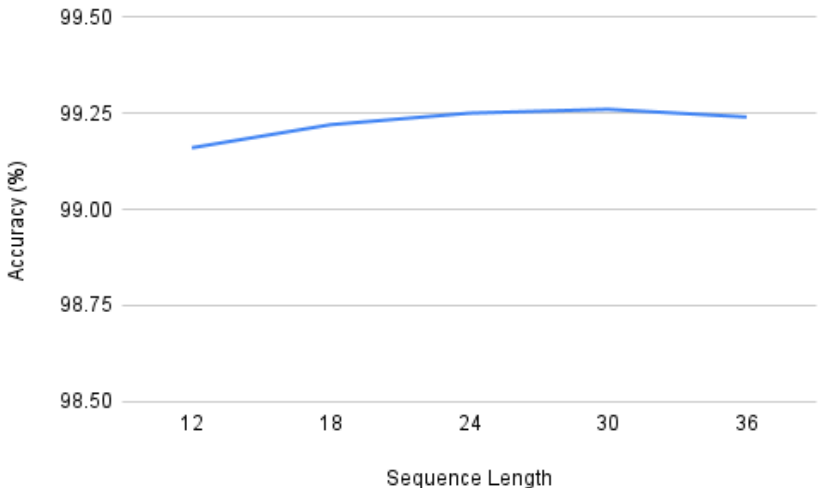
Figure A.5: Accuracy-Sequence Length
