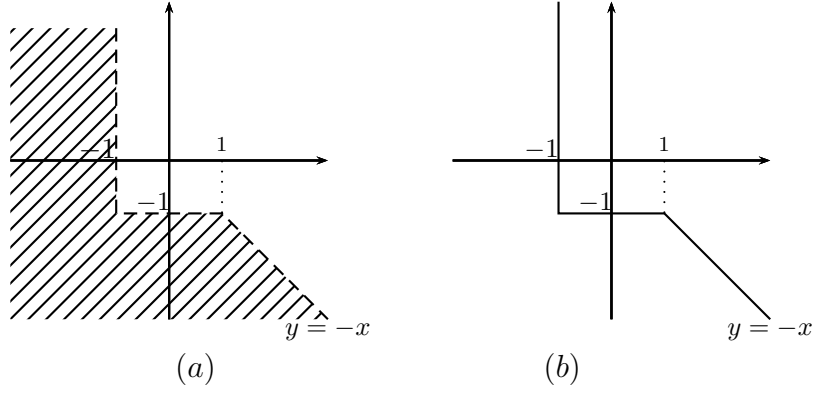
Şekil 3.12: (a) \bigcup_{(a,b,d) \in \mathbb{R}^2 \times \mathbb{R}_+} \inf_{x_0 \geq -1} [(ax_0, bx_0) + (d|x_0|, d|x_0|) - f^w(x_0, a, b, d)] kümesinin alt noktaları kümesi (b) \sup_{(a,b,d) \in \mathbb{R}^2 \times \mathbb{R}_+} \inf_{x_0 \geq -1} [(ax_0, bx_0) + (d|x_0|, d|x_0|) - f^w(x_0, a, b, d)] kümesi
