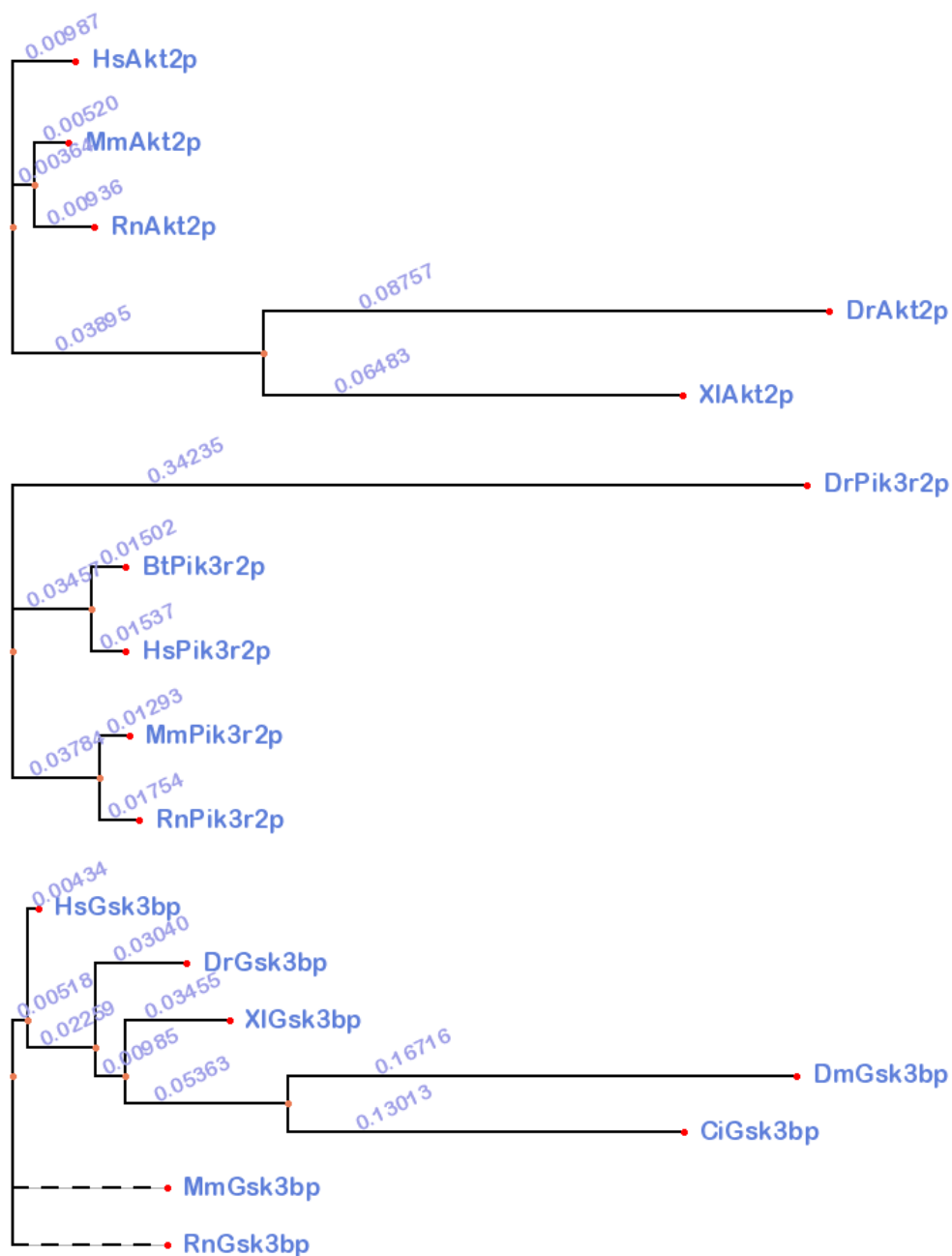
Fig. 4.9.2. Phylogenetic trees obtained from multiple alignment of amino acid sequences shown in Fig. 4.9.1a-c. Trees were generated by phyfi ( http://cgi-www.daimi.au.dk/cgi-chili/phyfi/go ).
