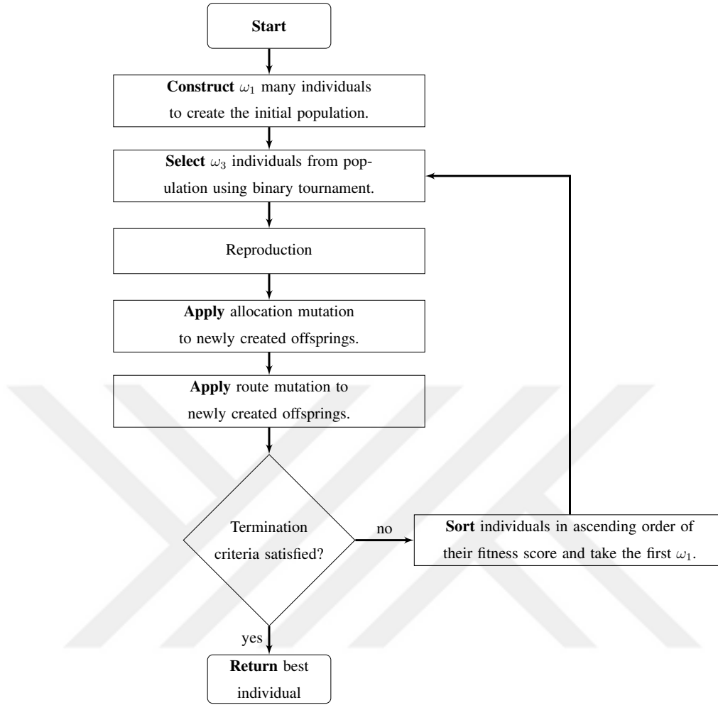
Figure 4.1: The main steps of the proposed evolutionary algorithm
