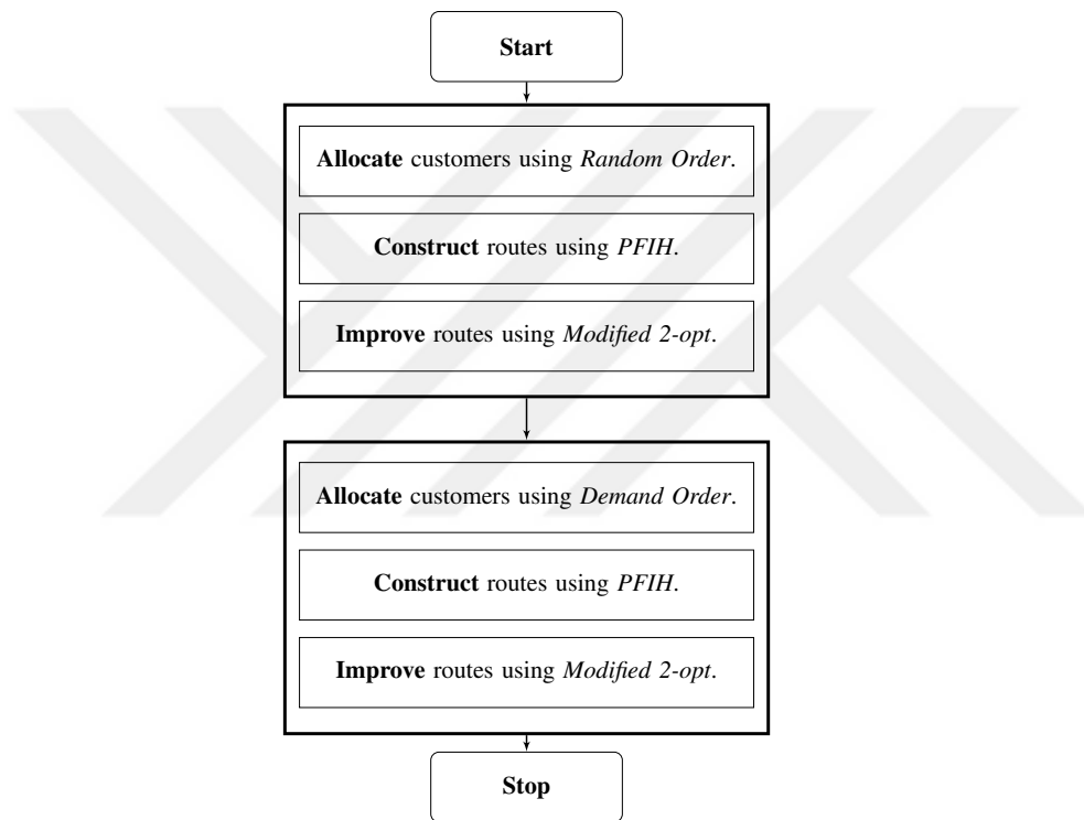
Figure 4.5: Initialization procedure
