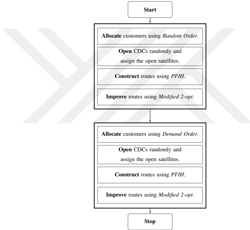
Figure 5.2: Initialization procedure
