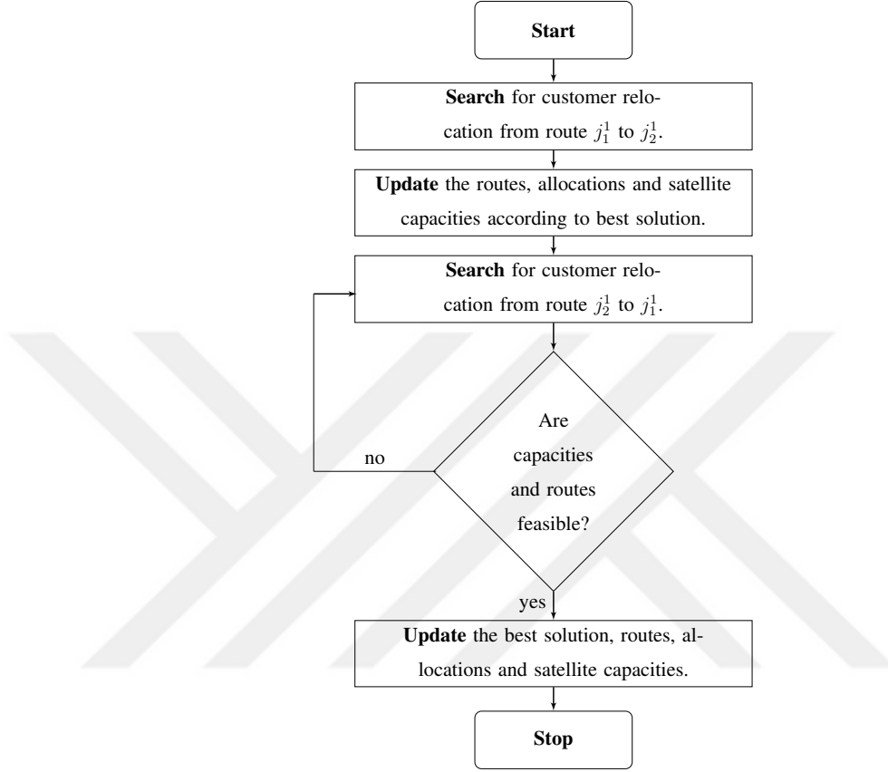
Figure 4.8: The main steps of Improve Allocation
