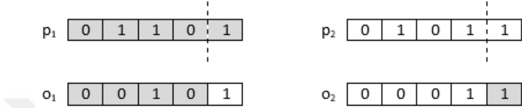
Figure 5.3: One-point crossover
