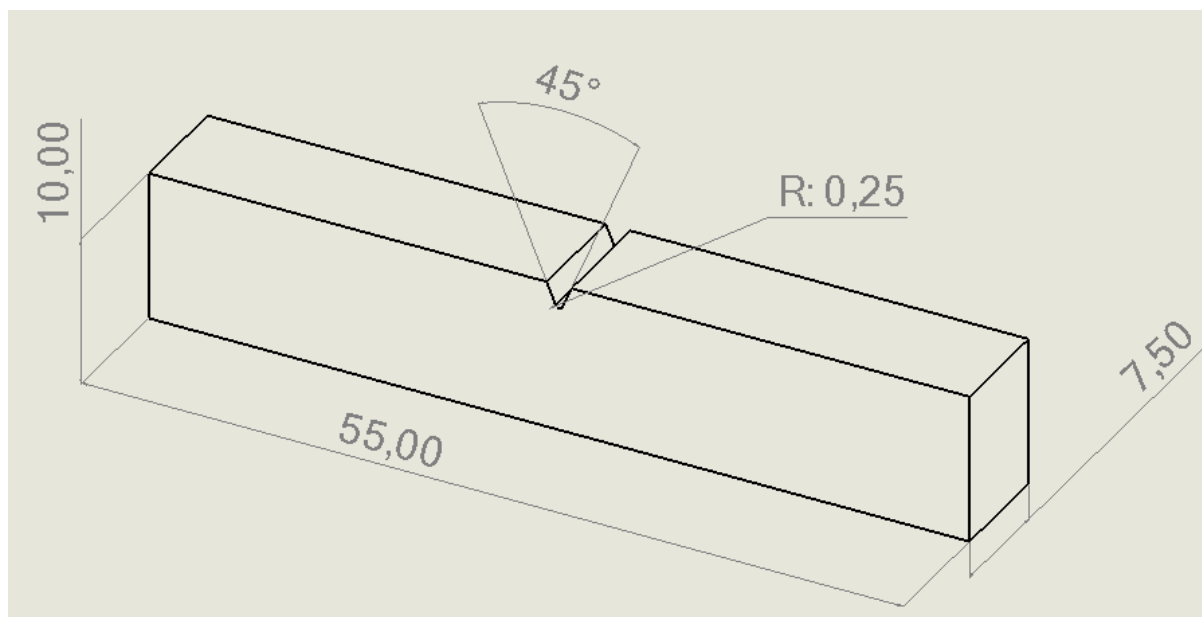
Figure 4.16 The dimensions of armor steel-1 and armor steel-2 impact test specimens in mm.
