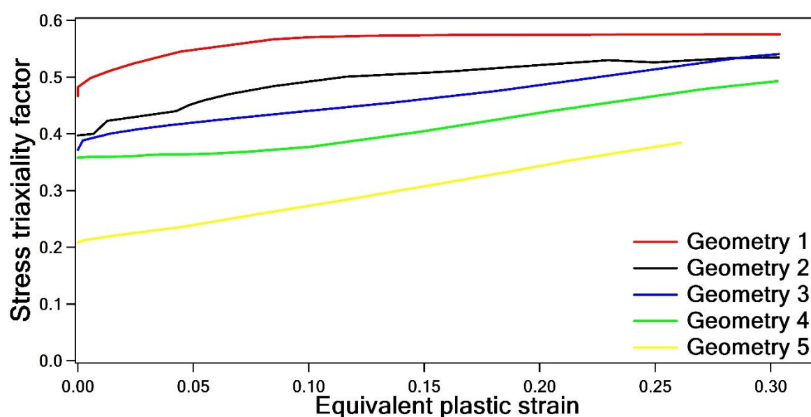
Figure 4.29 Evolution of the STF with respect to equivalent plastic strain for armor steel-1.
