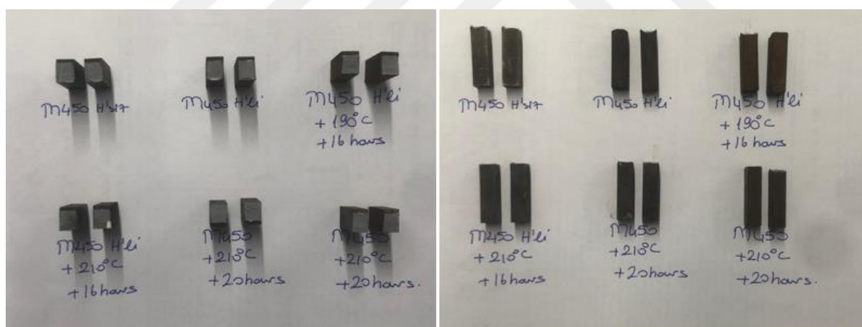
Figure 4.18 The fracture surfaces of all experiments carried out with armor steel-1
