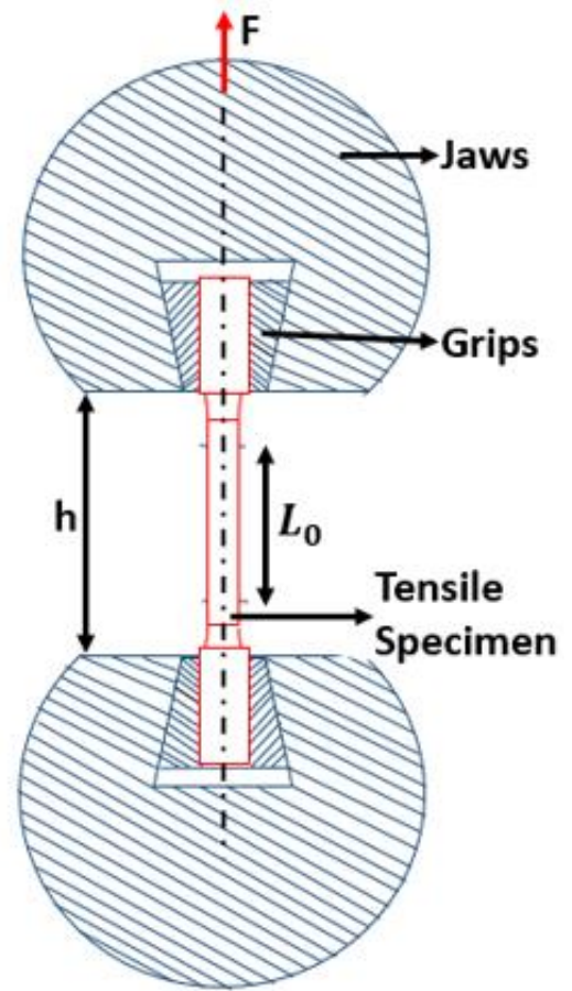
Figure 4.3 10 kN universal Shimadzu AGS-X and schematic representation of universal tensile testing machine (on the right)
