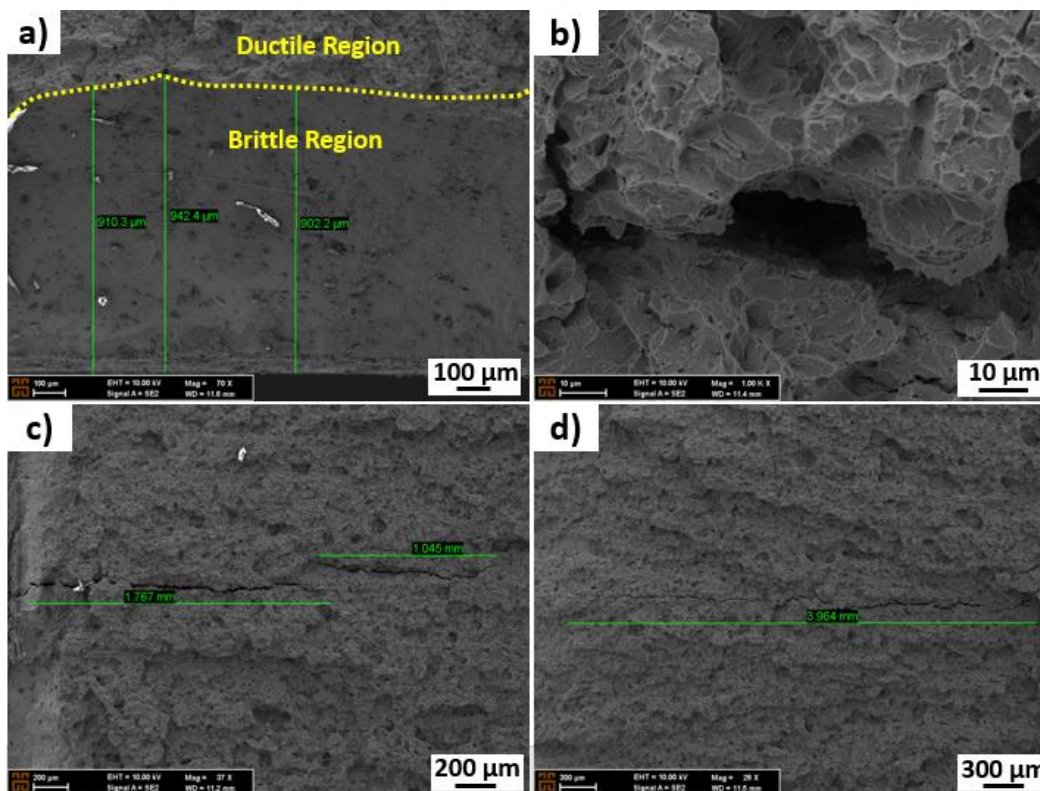
Figure 4.46 Fracture surface overview of armor steel-2 with hydrogen-charging condition.
